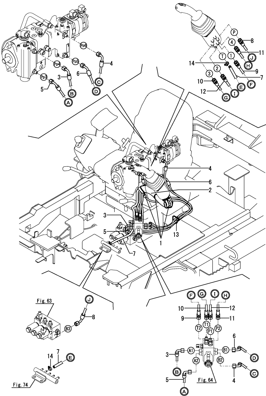
Fig.80. CONTROL PIPING(LEFT)
