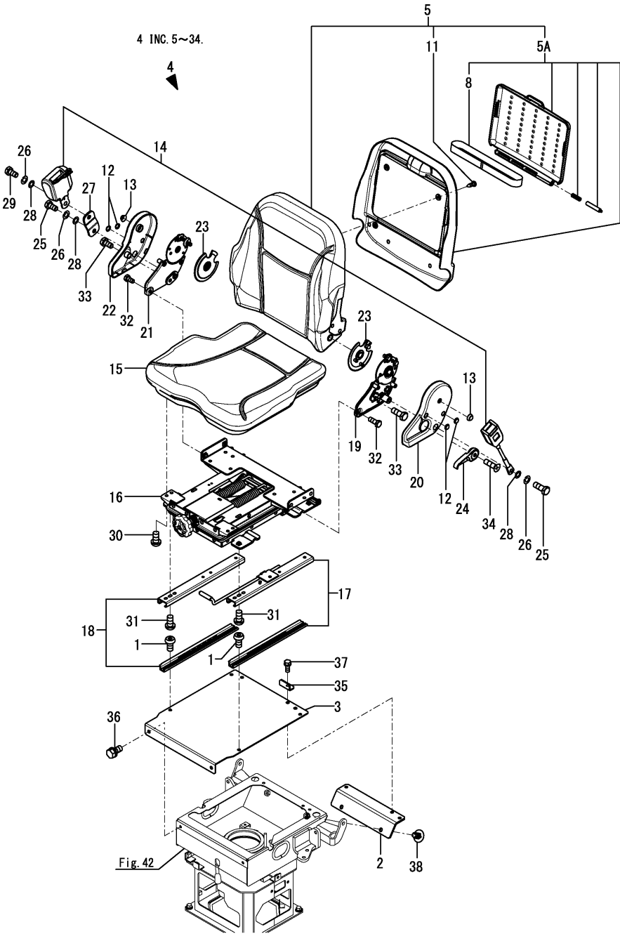
Fig.44. SEAT
