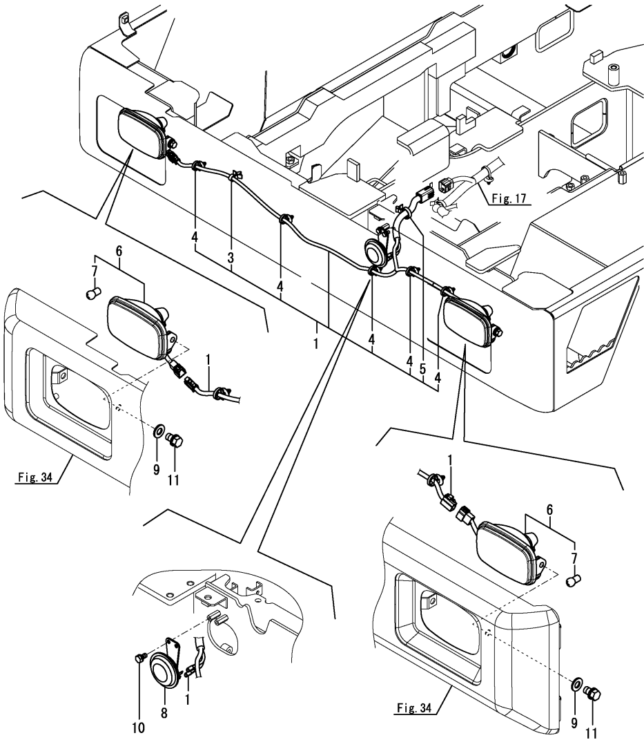
Fig.21. FRONT LAMP
