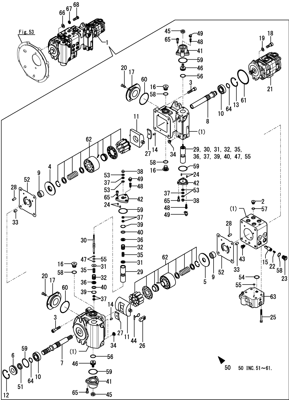
Fig.55. HYDRAULIC PUMP
