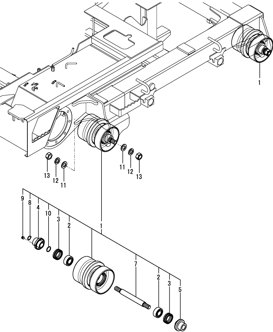
0CK50-M00830 TRAVELING Fig.27. TRACK ROLLER(2)
