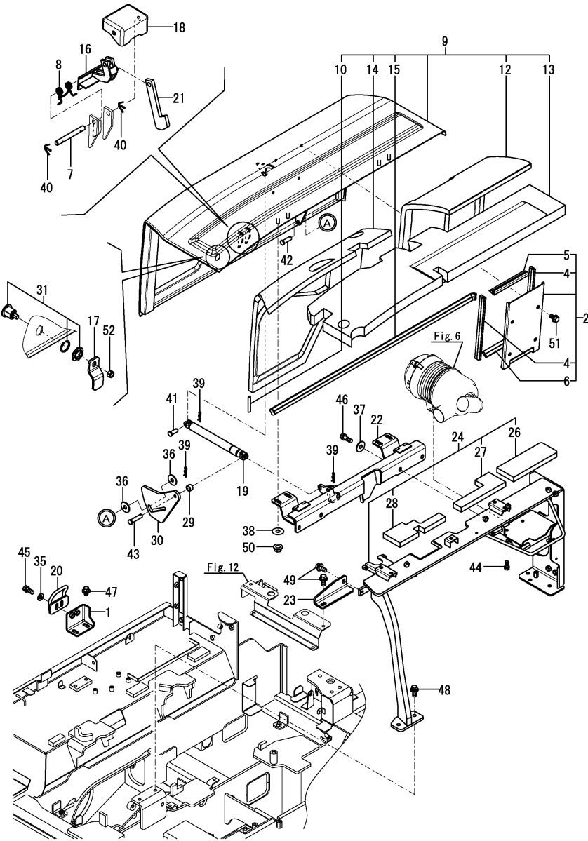
Fig.48. BONNET(RIGHT)
