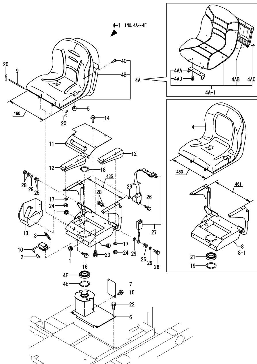
Fig.38. SEAT & MOUNT
