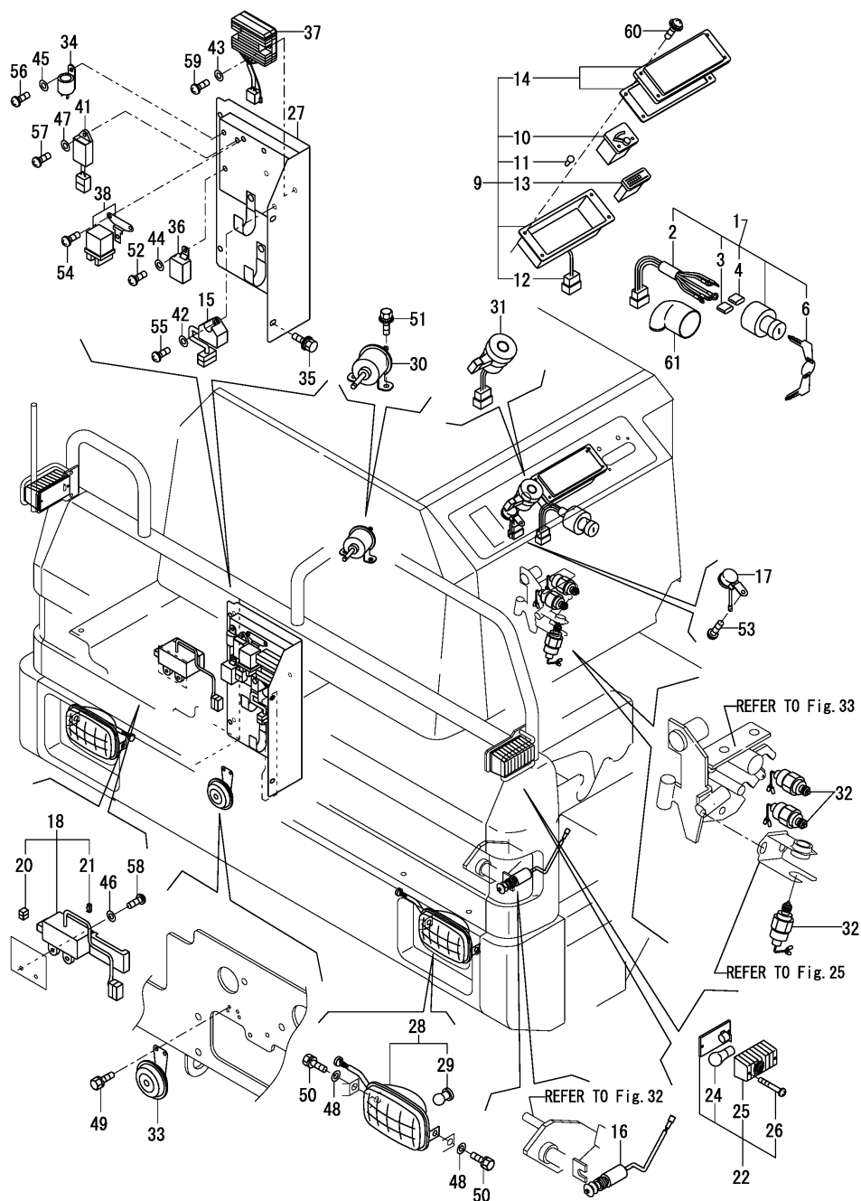
Fig.14. ELECTRIC PART(EQUIPMENT)
