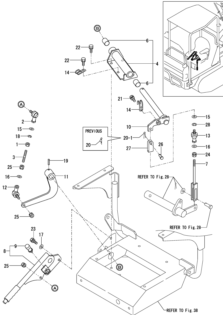
Fig.27. BRAKE(PARKING)
