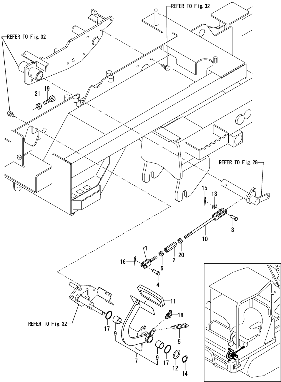
Fig.29. BRAKE(PEDAL & ROD)(FRONT)
