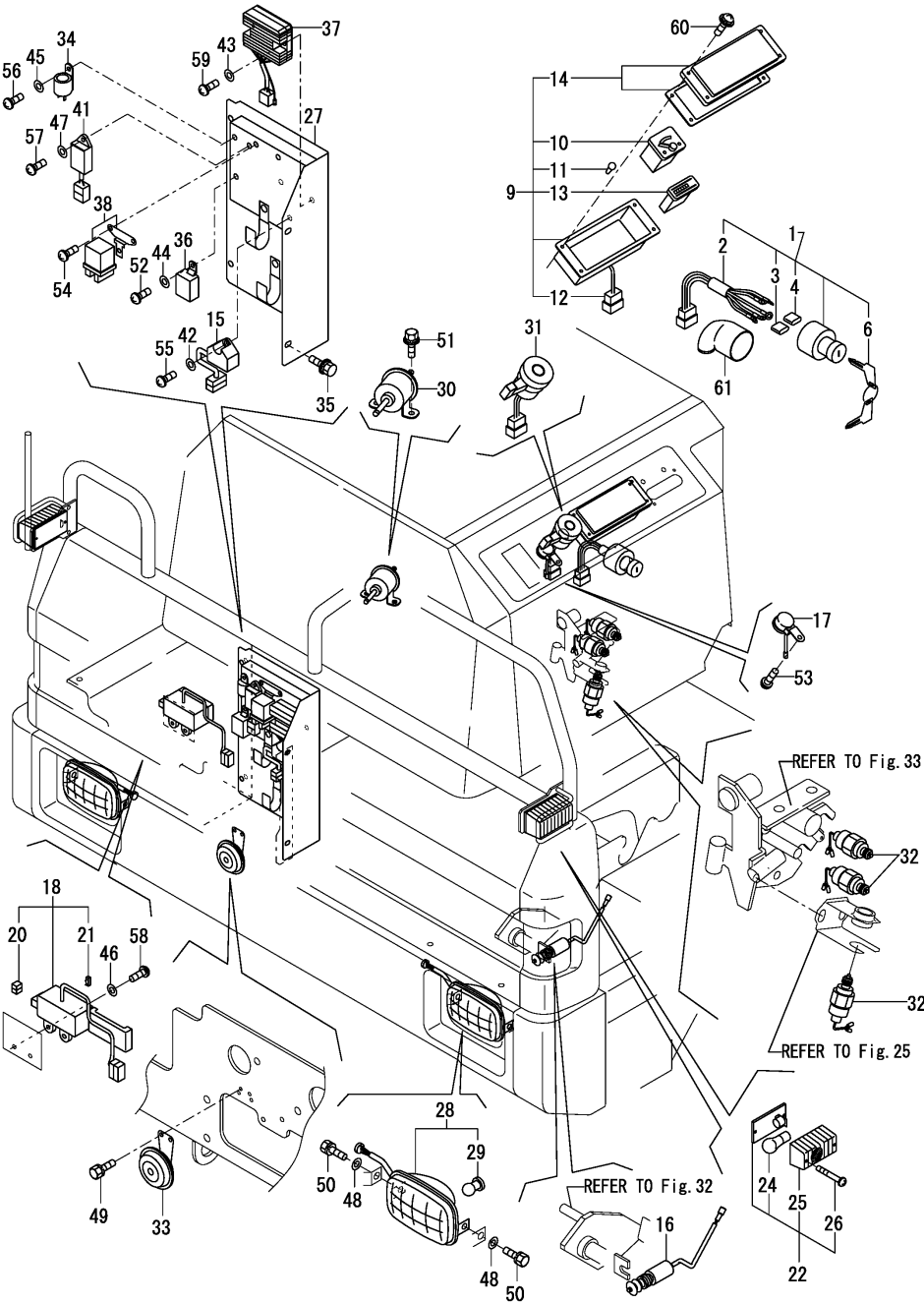
Fig.14. ELECTRIC PART(EQUIPMENT)
