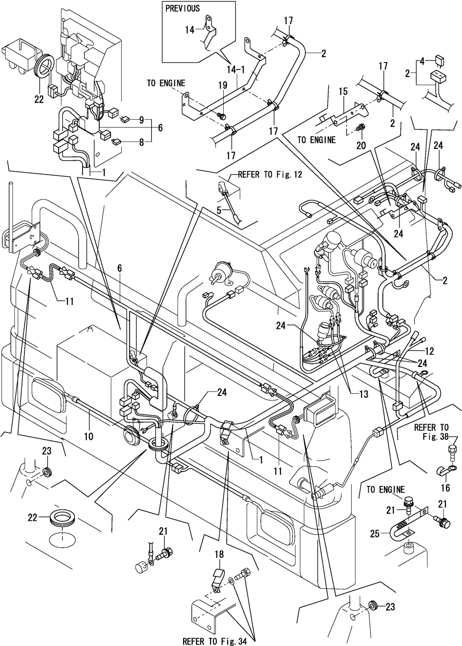
Fig.13. ELECTRIC PART(WIRING)
