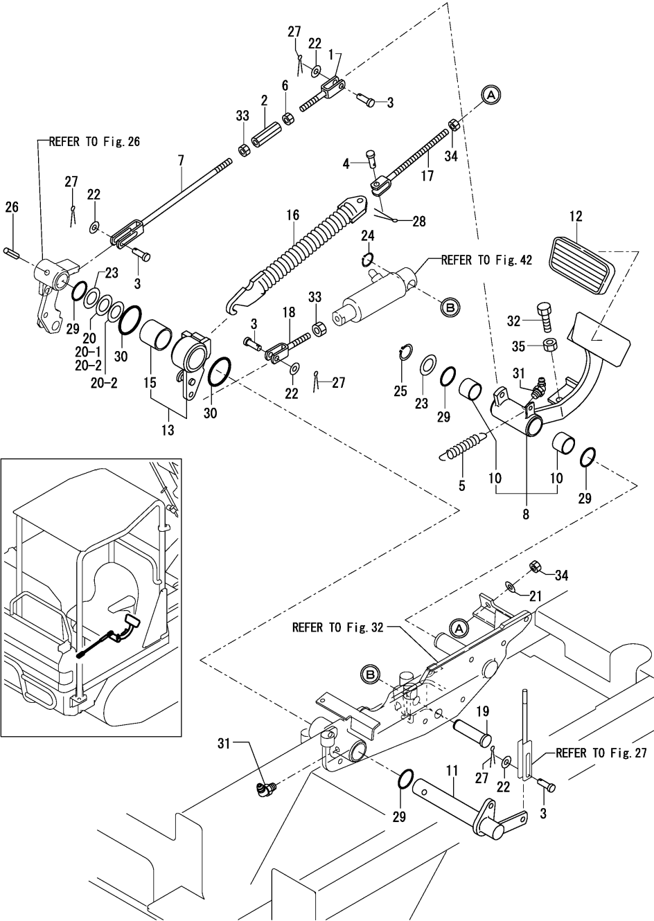
Fig.28. BRAKE(PADAL & ROD)(REAR)
