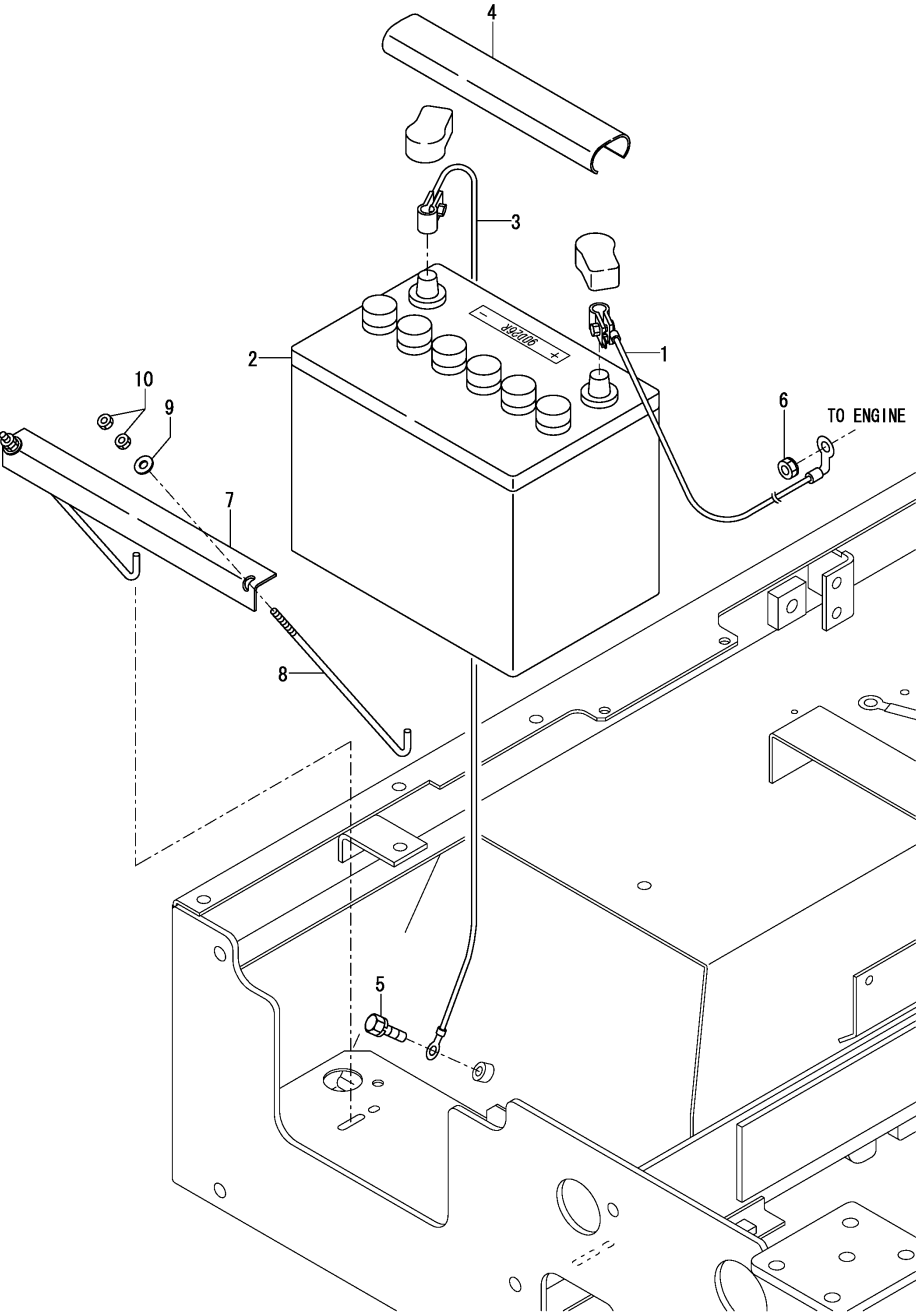
Fig.12. BATTERY
