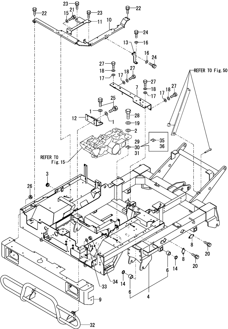
Fig.35. FRAME & BUMPER
