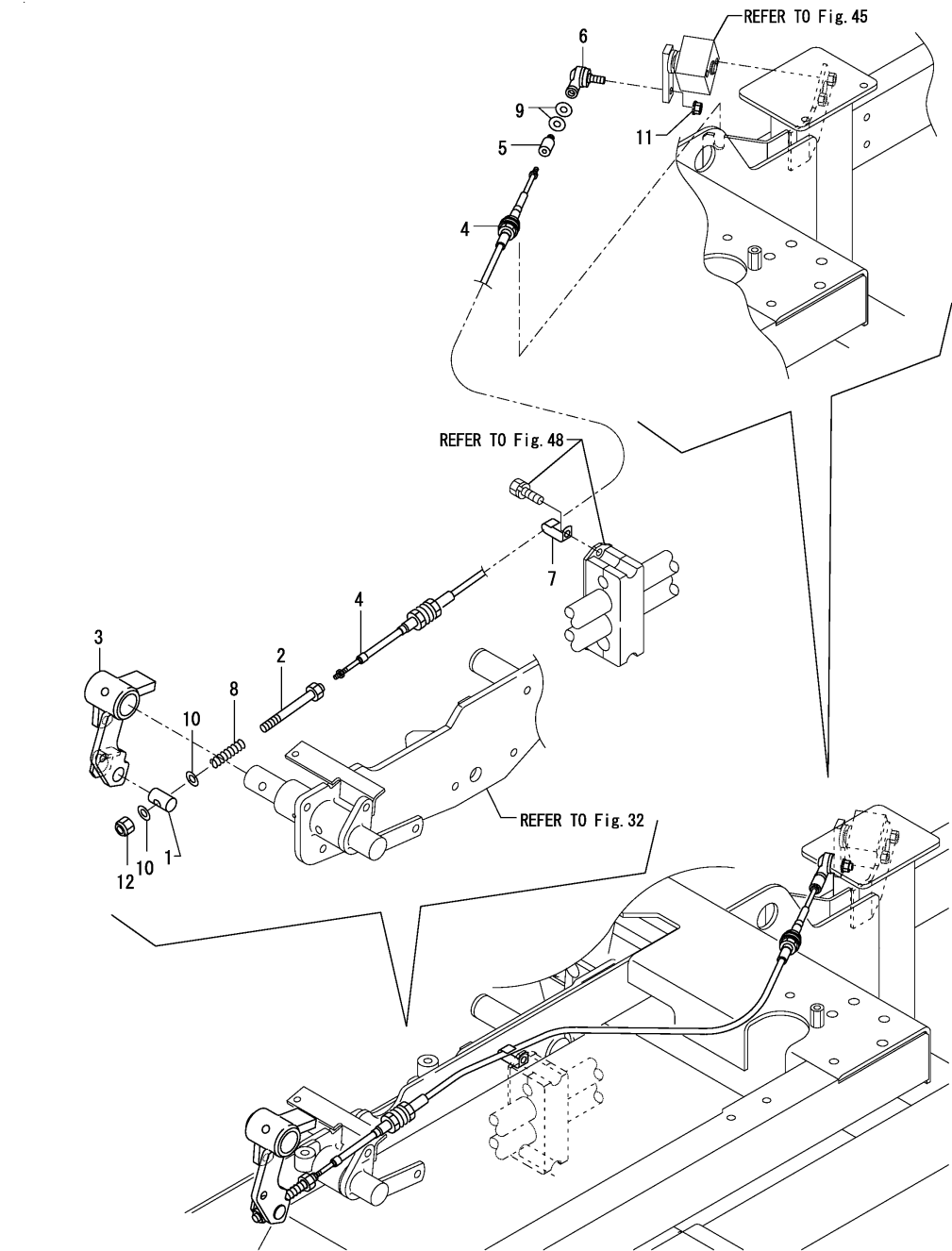
Fig.26. INCHING LINK
