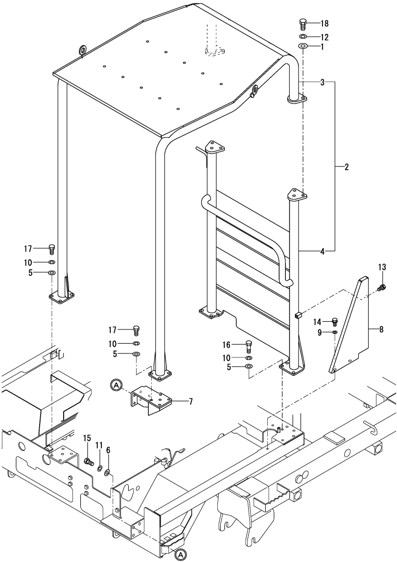
Fig.40. CANOPY(ROPS)
