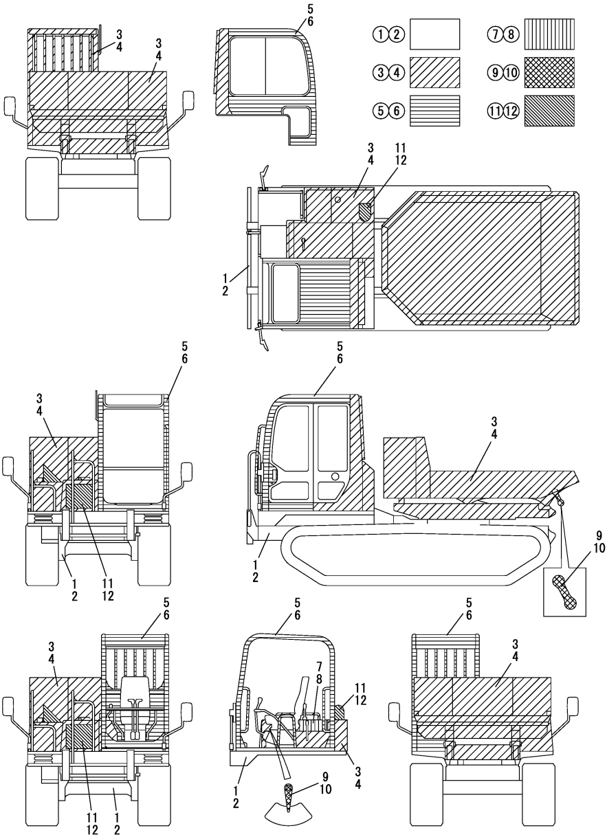
Fig.85. PAINTED COLOR(TURNING)
