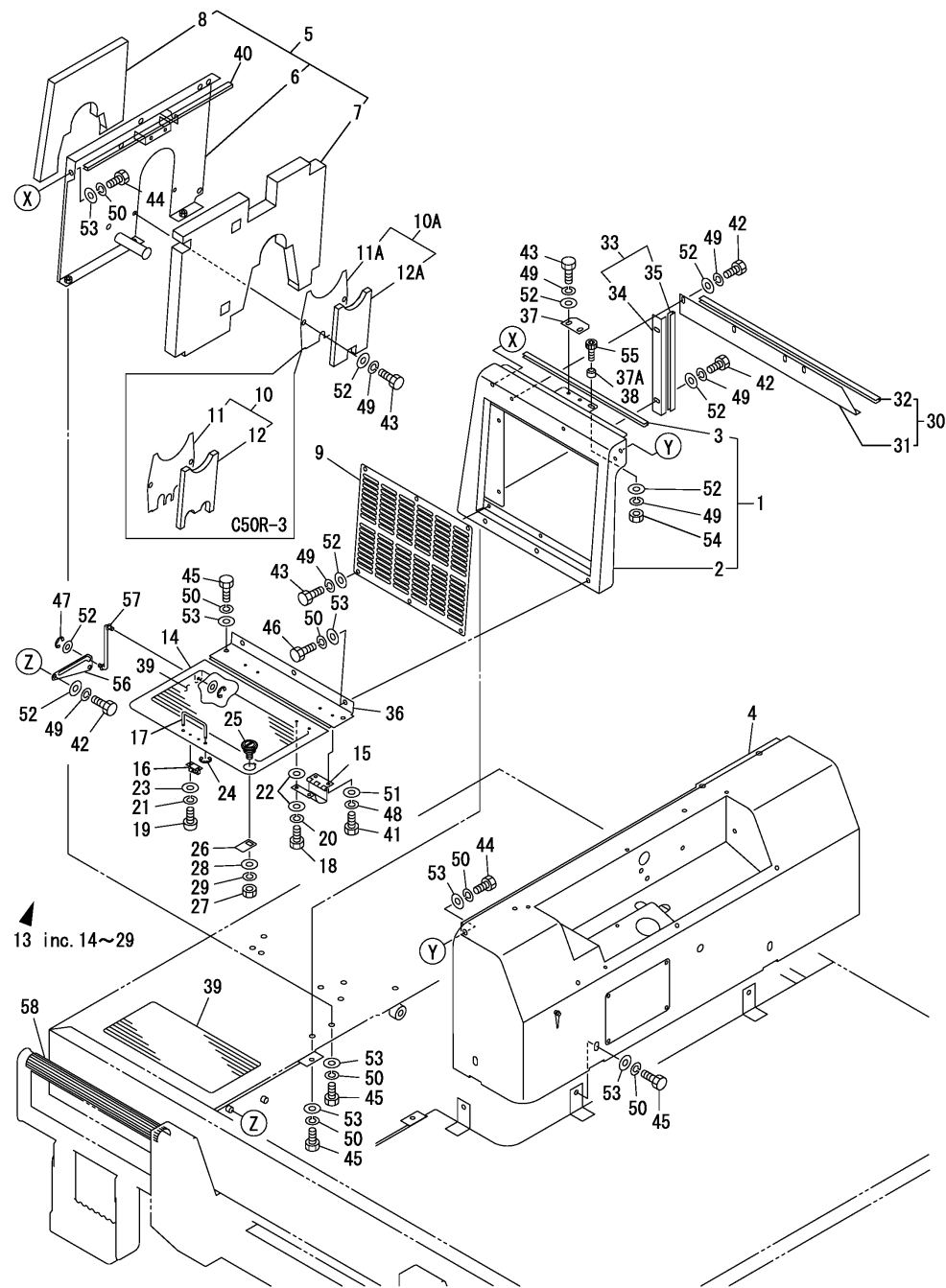
OCK30-M38102 C50R-3(A) Fig.44. COVER(1)
