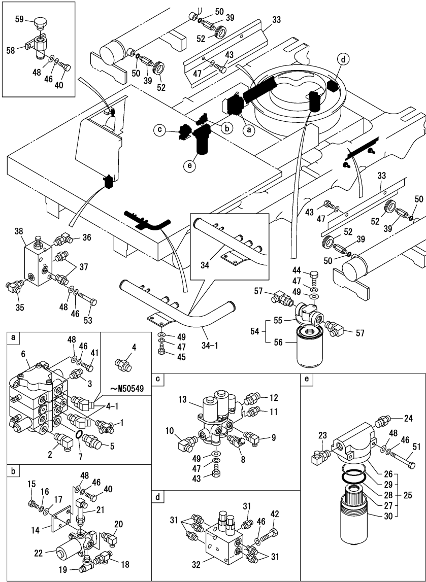
Fig.33. VALVE(TURNING)
