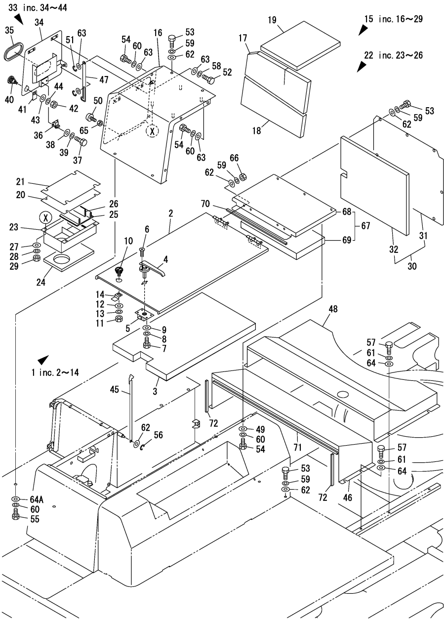
Fig.46. COVER(2)(FROM M40563)
