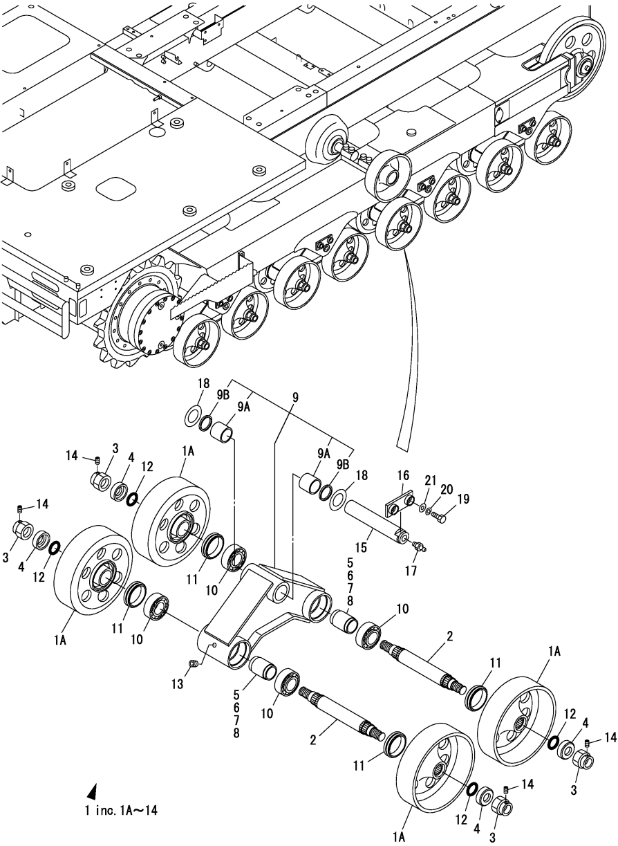
Fig.5. TRUCK ROLLER
