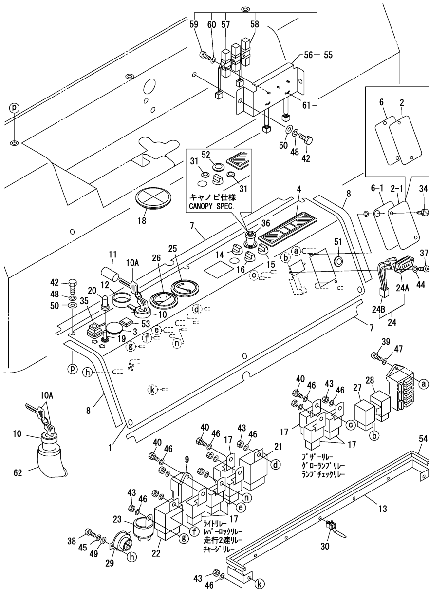
Fig.19. CONTROL BOX
