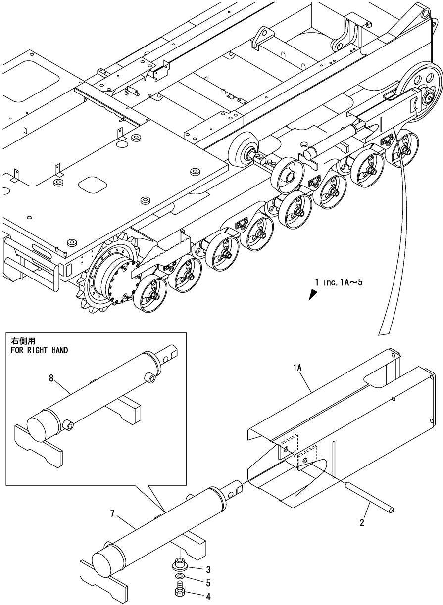
Fig.7. TRUCK ADGUSTA
