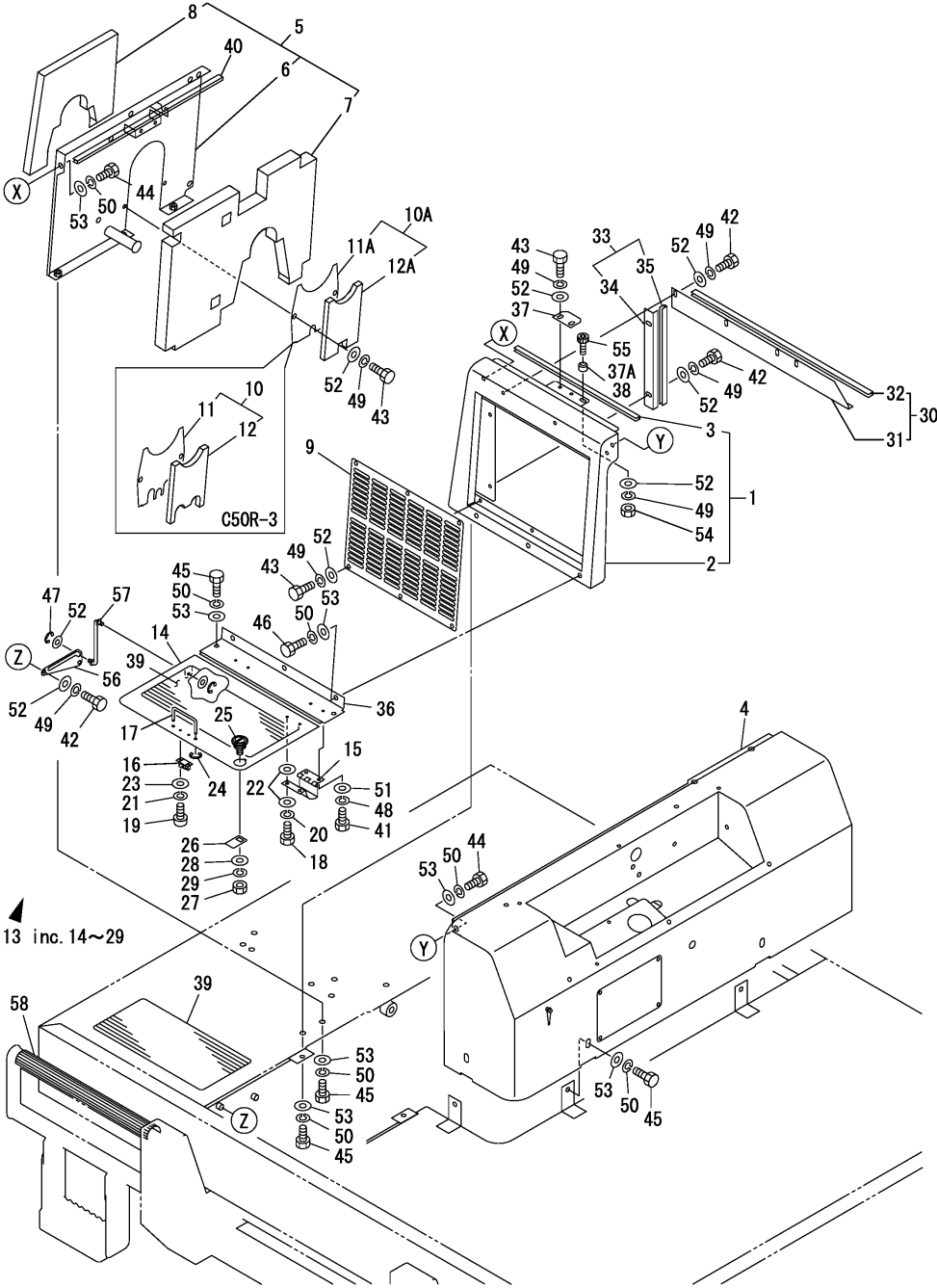
Fig.44. COVER(1)
