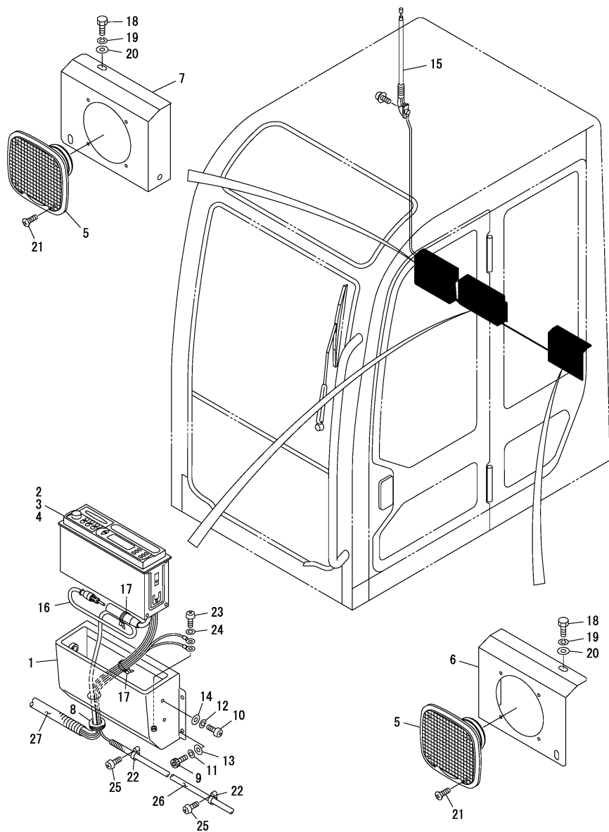
Fig.28. RADIO
