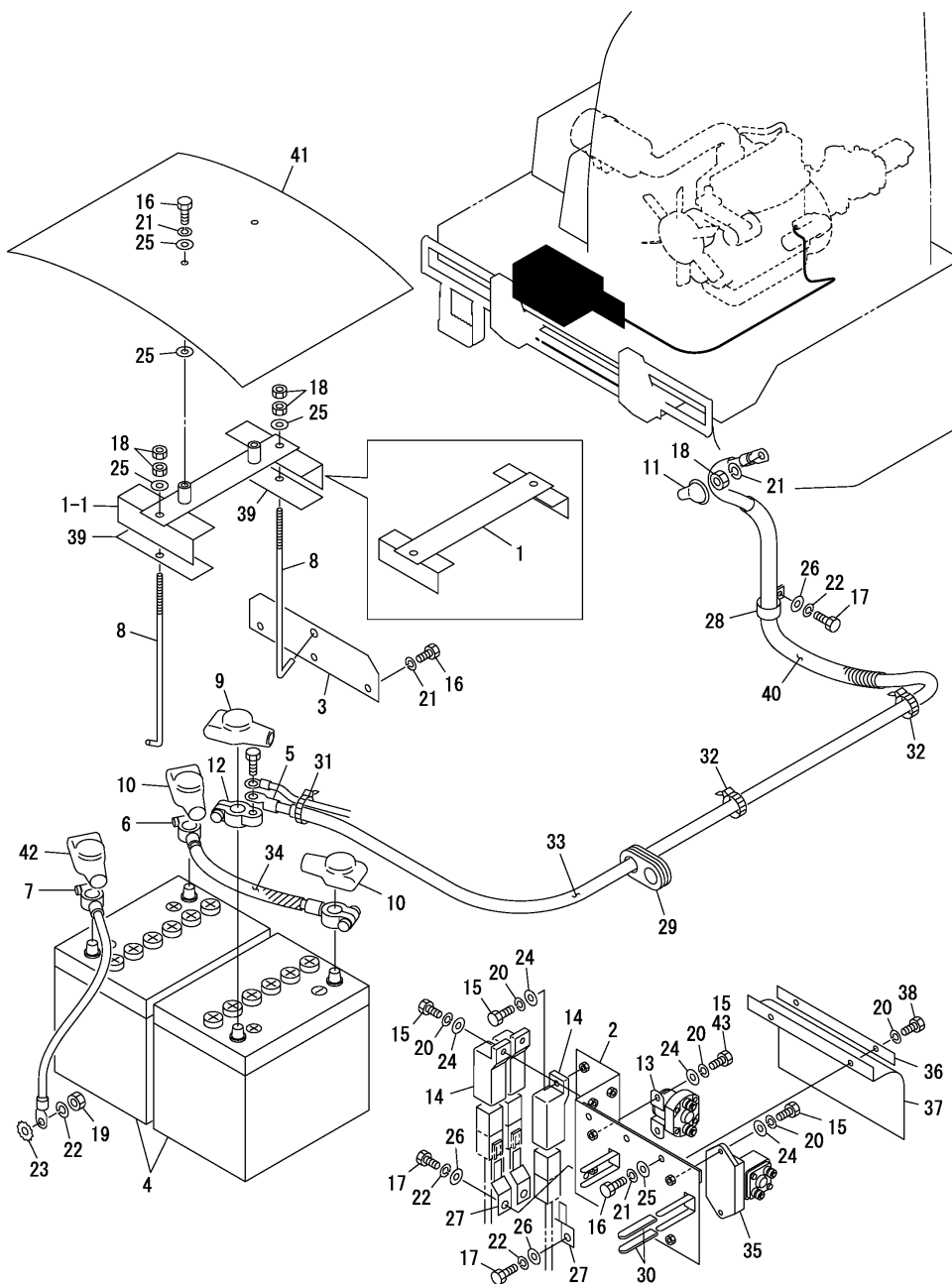
Fig.22. BATTERY(C50R-3)
