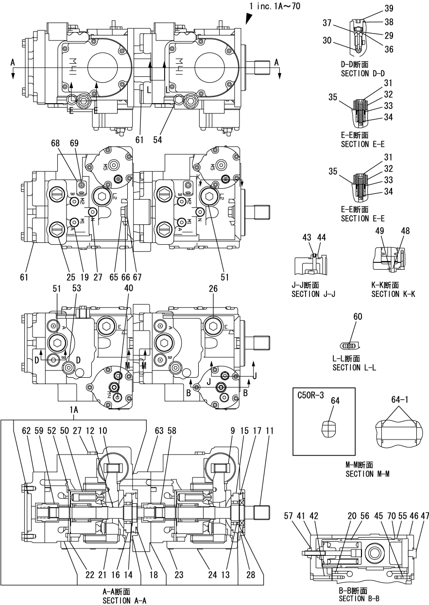
Fig.104. HYD. OIL PUMP
