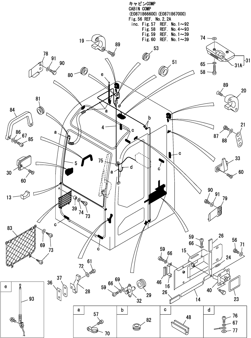
Fig.58. CABIN(3)
