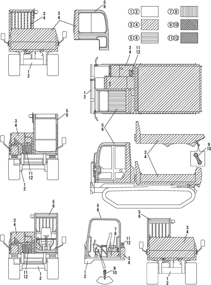
Fig.84. PAINTED COLOR
