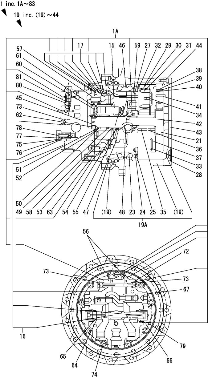
Fig.102. TRAVEL MOTOR
