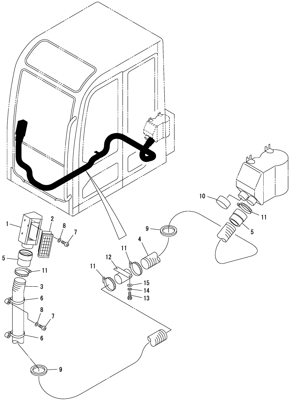
Fig.64. DEFROSTER
