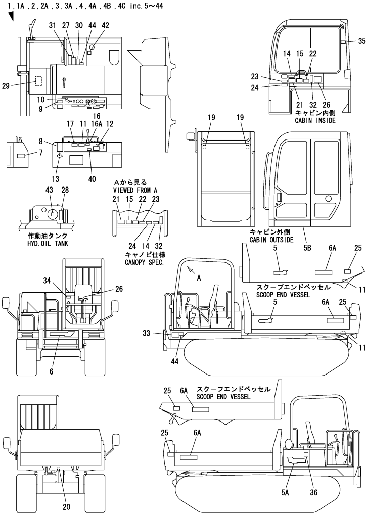
Fig.81. LABEL(EX)
