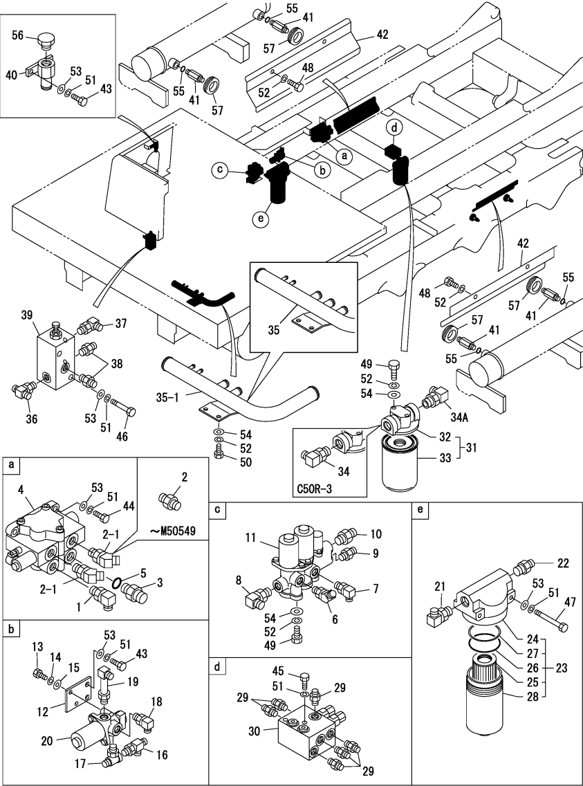
Fig.32. VALVE
