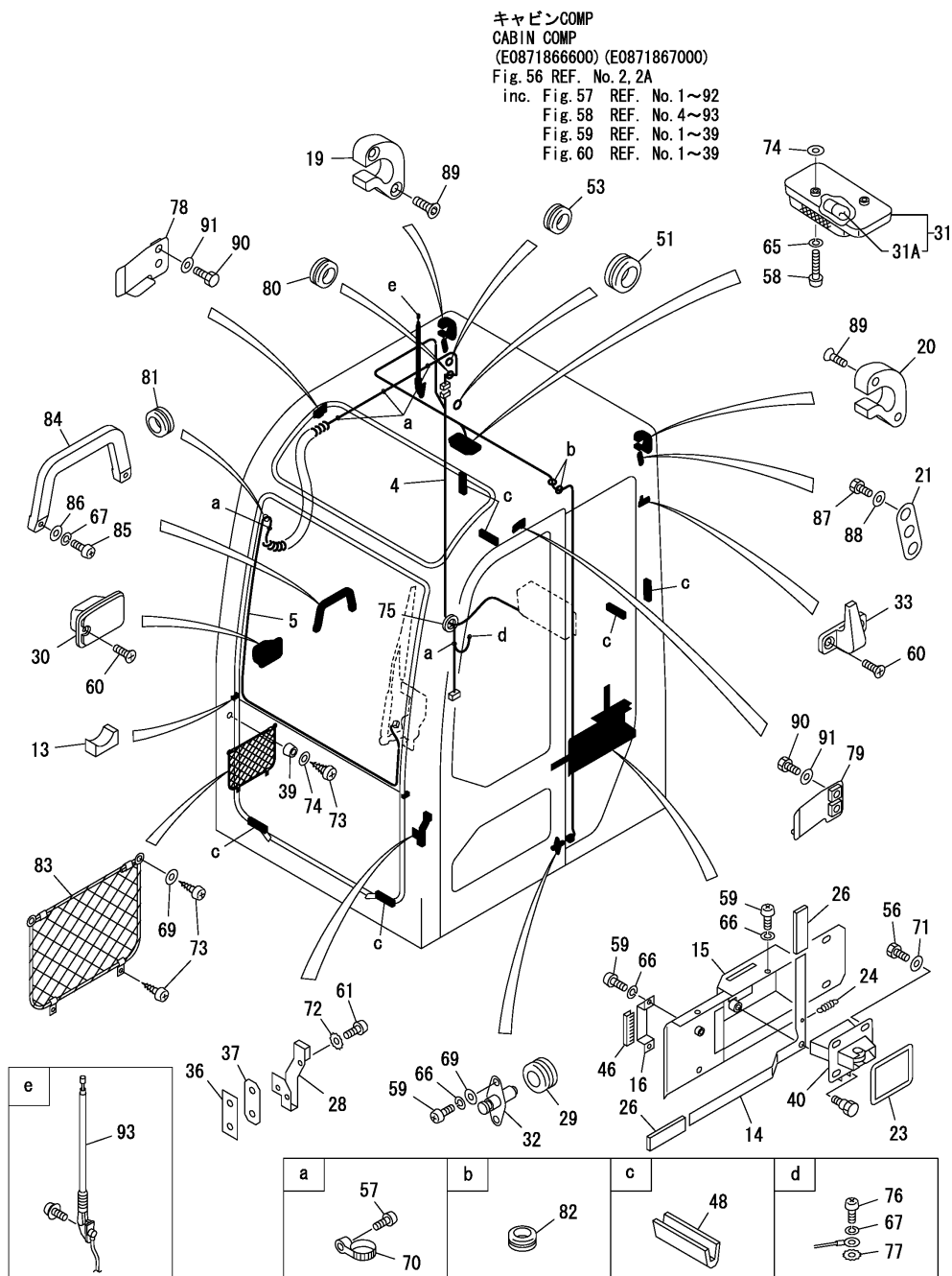
Fig.58. CABIN(3)
