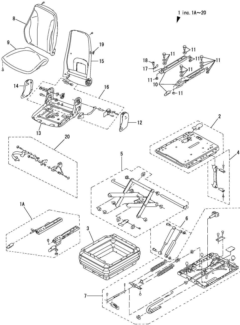
Fig.54. SEAT(COMPONENT PART)(OVER SAE)
