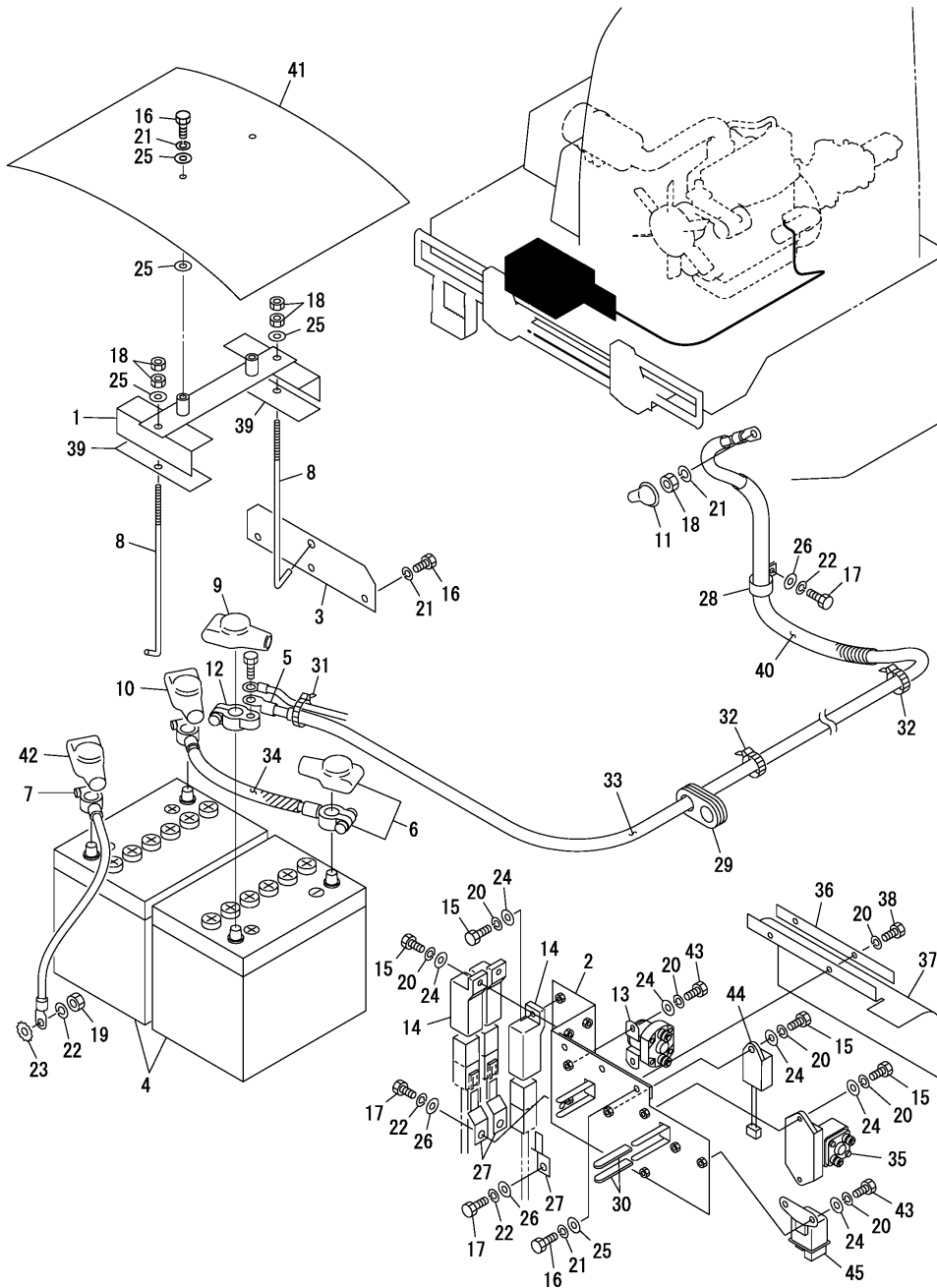
Fig.23. BATTERY(C50R-3A)
