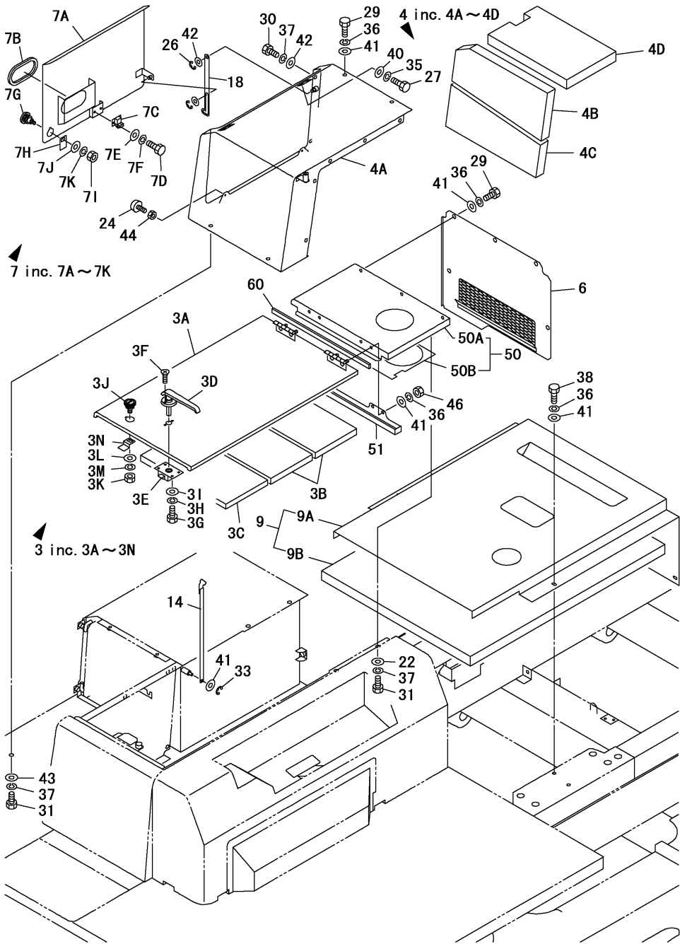
Fig.44. COVER(2/4)
