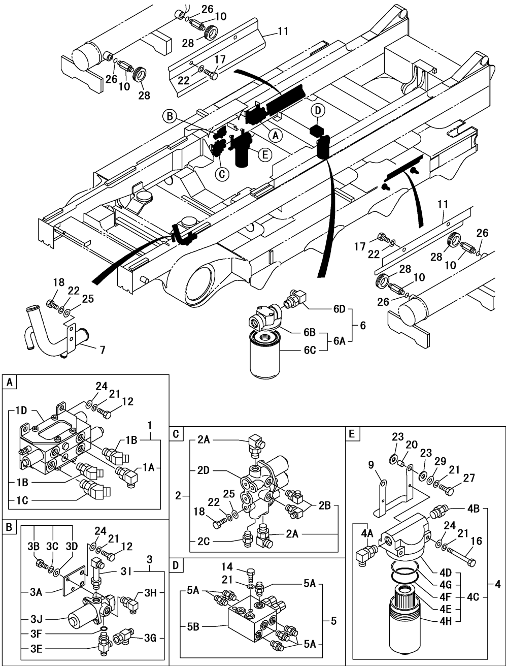
Fig.32. VALVE
