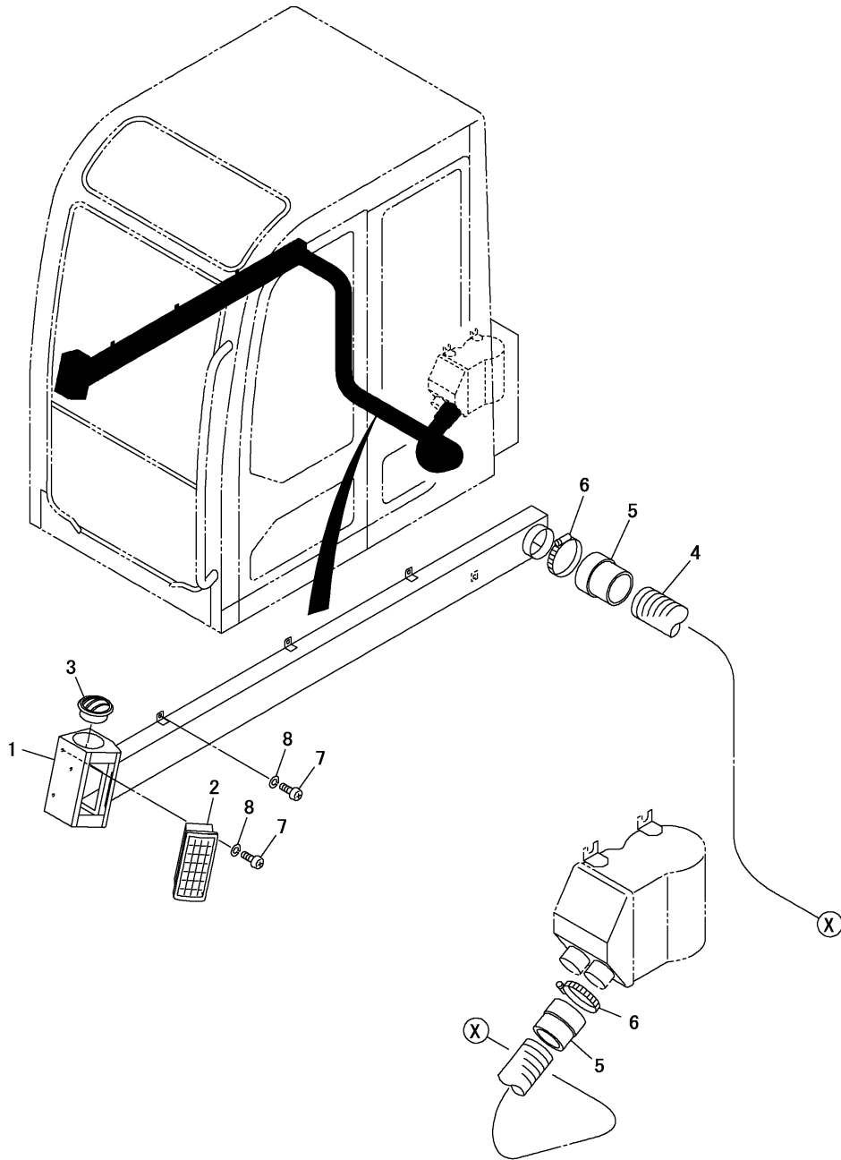
Fig.60. DEFROSTER
