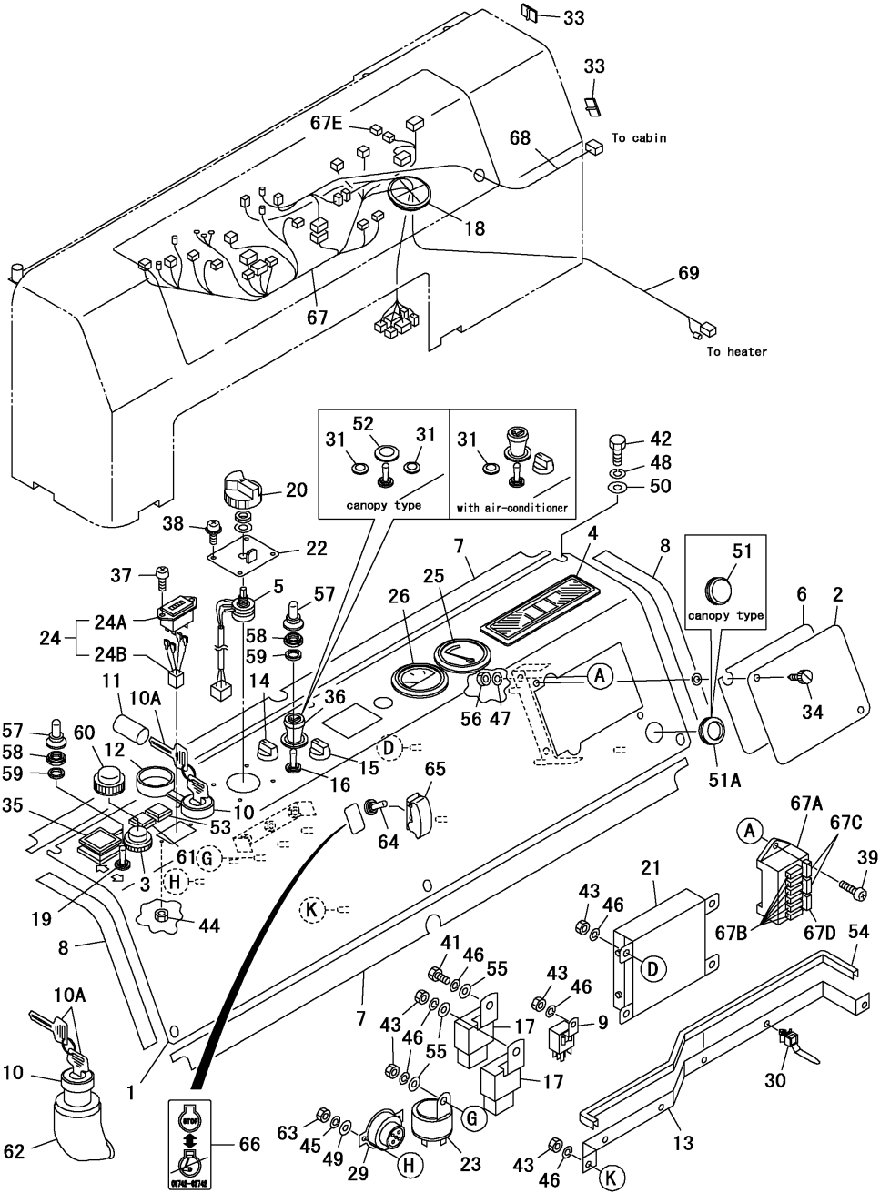
Fig.19. CONTROL BOX
