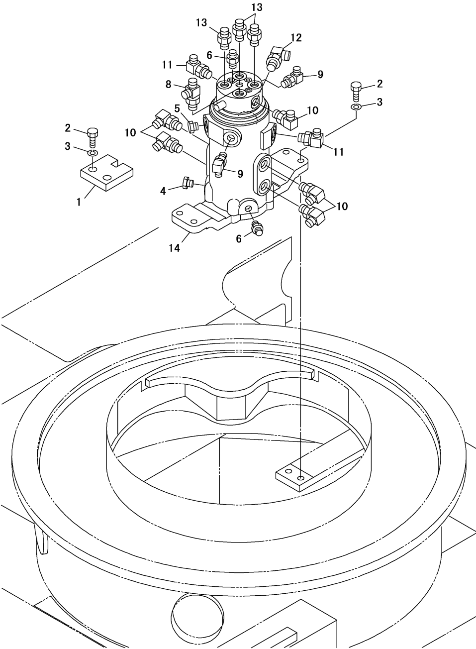
Fig.10. SWIVEL JOINT
