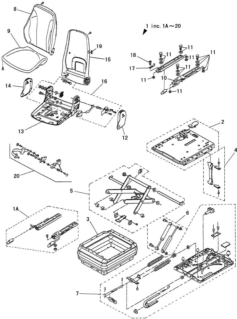
Fig.51. SEAT(2/2)
