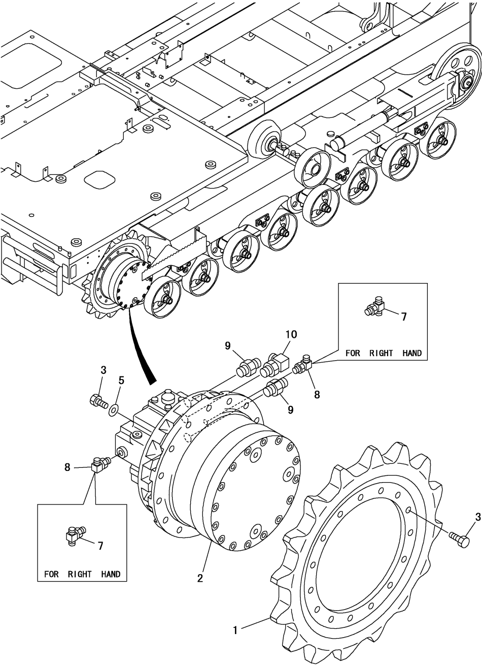
Fig.8. TRAVEL DEVICE
