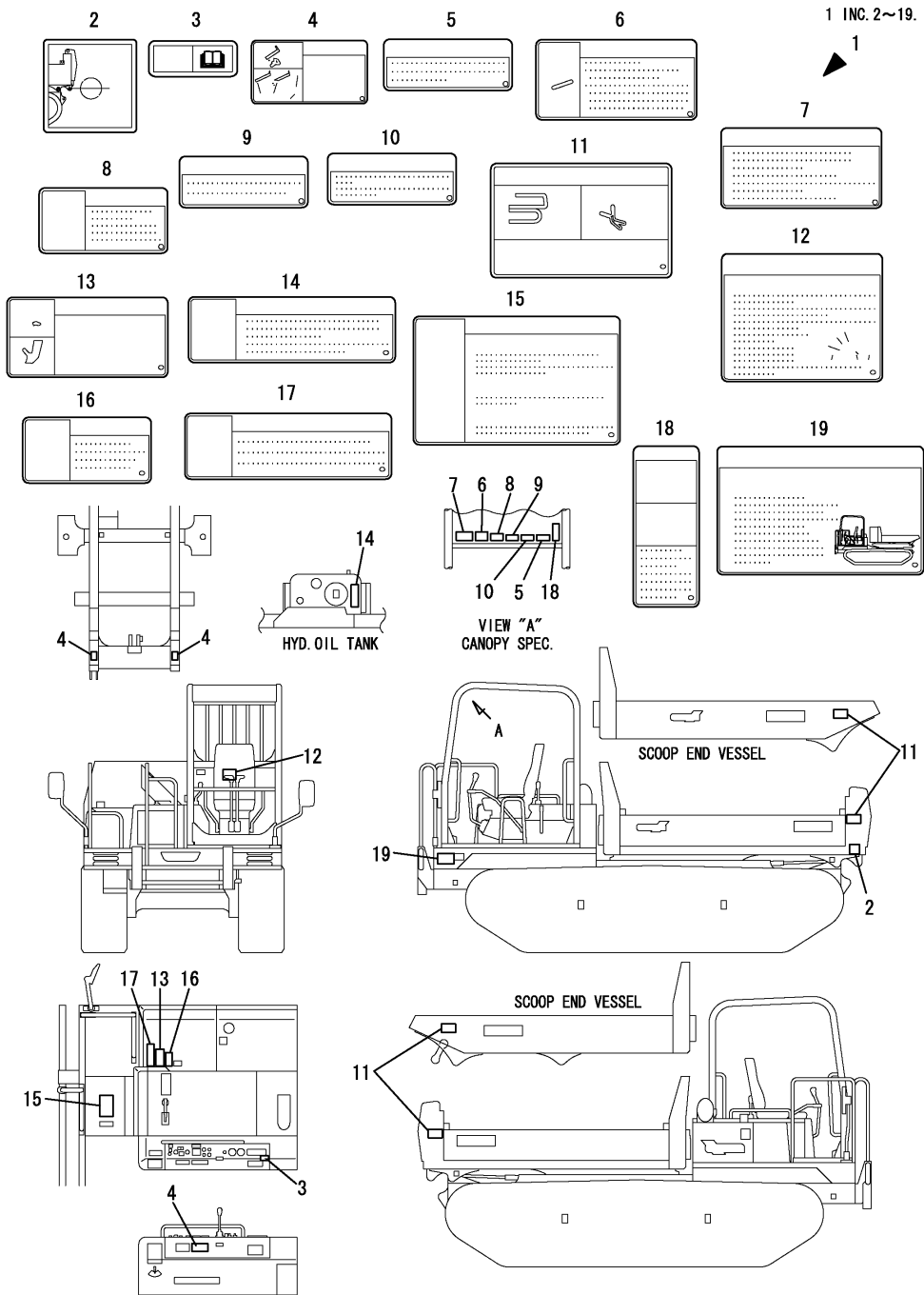
Fig.103. (73A)SAFETY LABEL(CANOPY)
