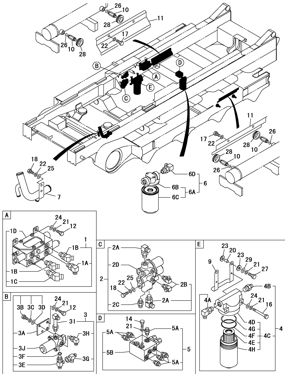
Fig.32. VALVE
