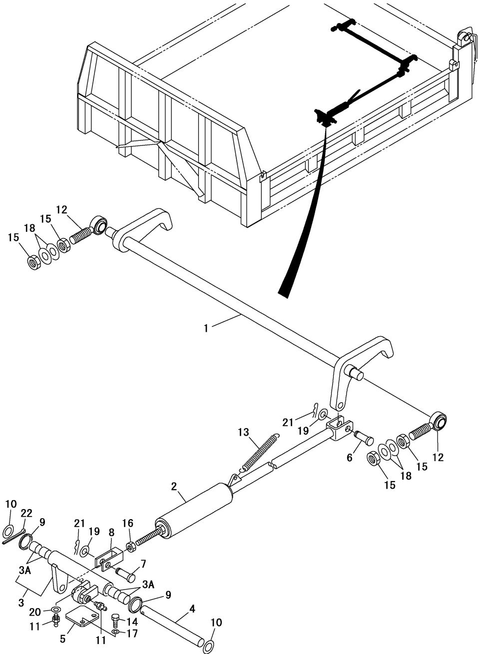
Fig.70. REAR LINK
