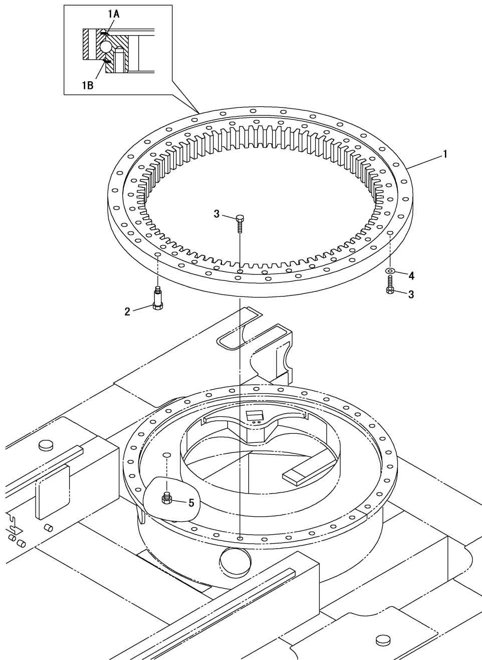
Fig.9. TURNING BEARING
