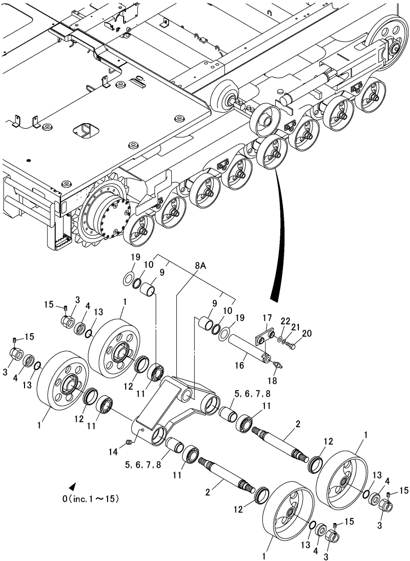
Fig.5. TRUCK ROLLER
