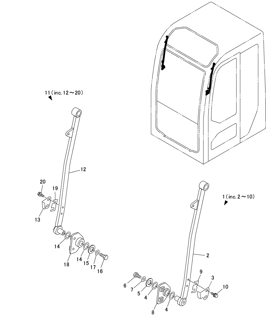
Fig.64. CAB(4/5)(FRONT SASH ASSIST)
