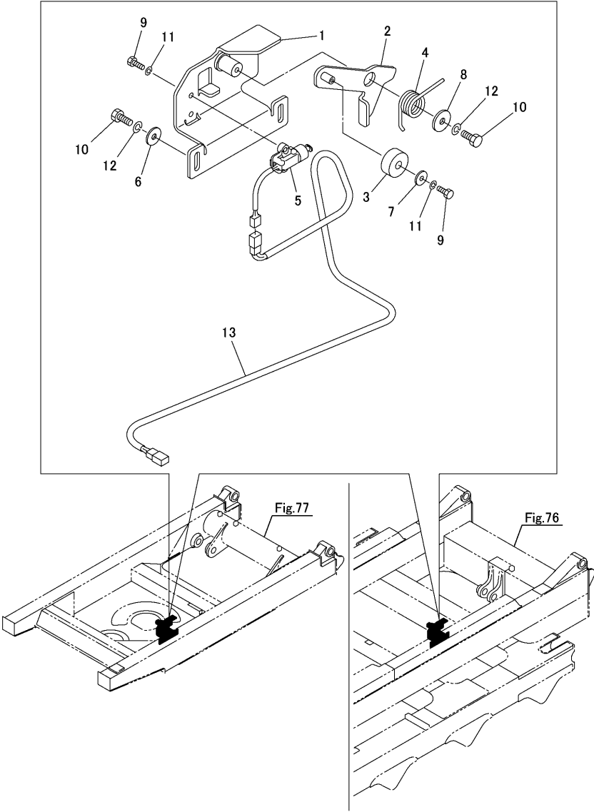
Fig.80. LIMIT SENSOR
