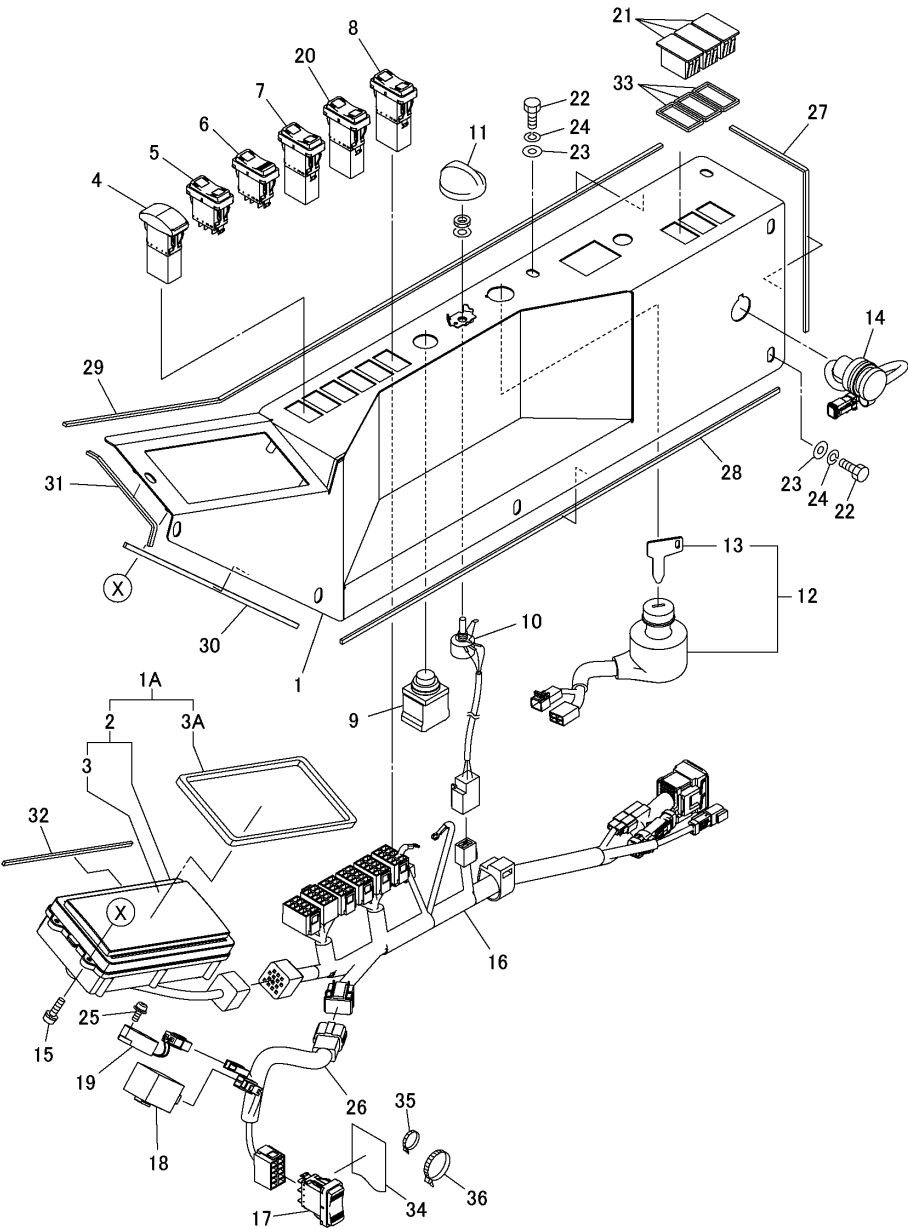
Fig.24. CONTROL BOX(CAB)(AIR CONDITIONER)
