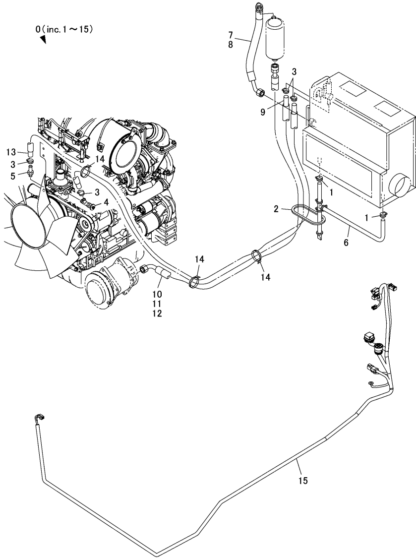
Fig.73. AIR CONDITIONER(3/4)(UNIT-2)
