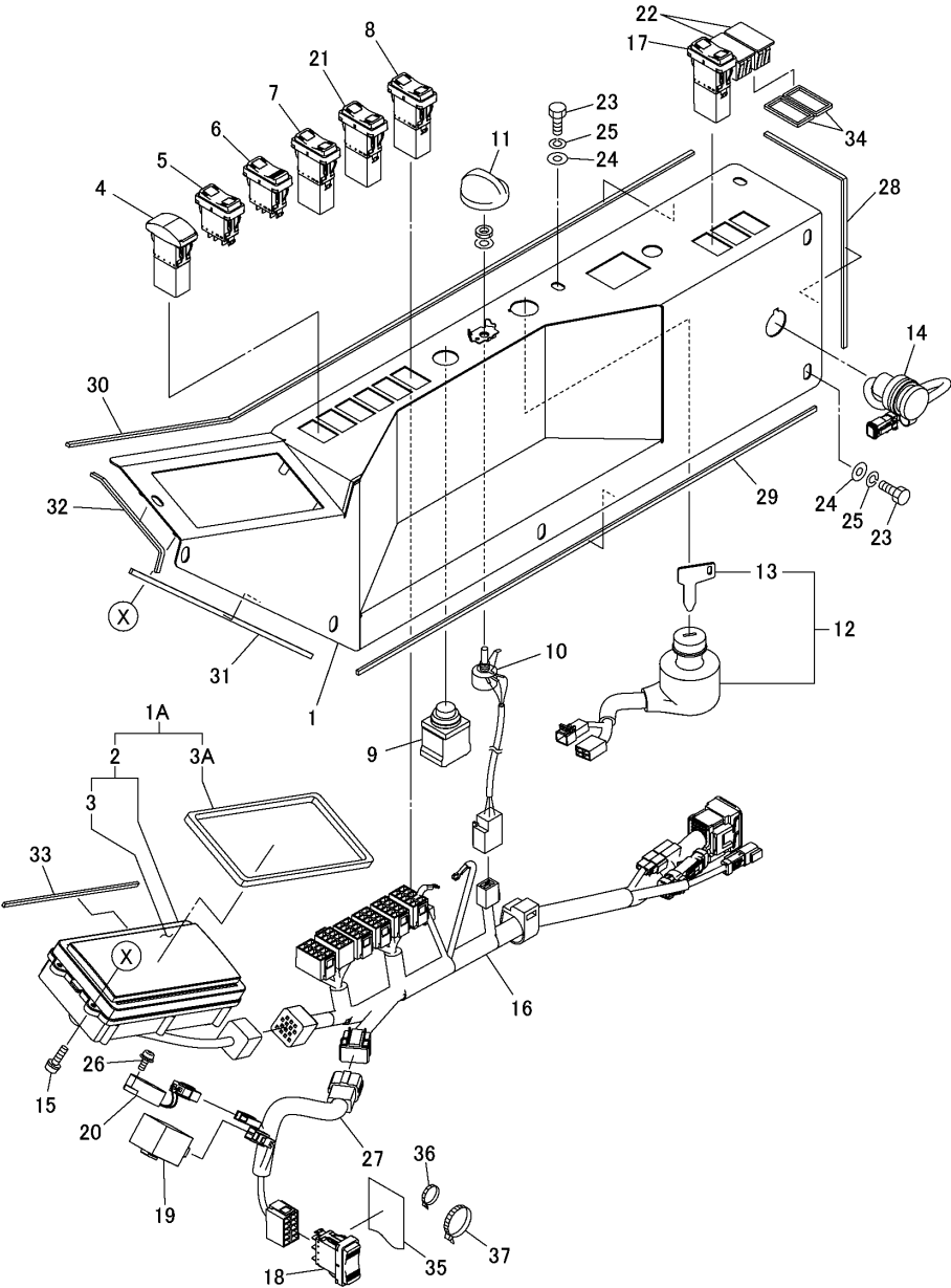
Fig.23. CONTROL BOX(CAB)
