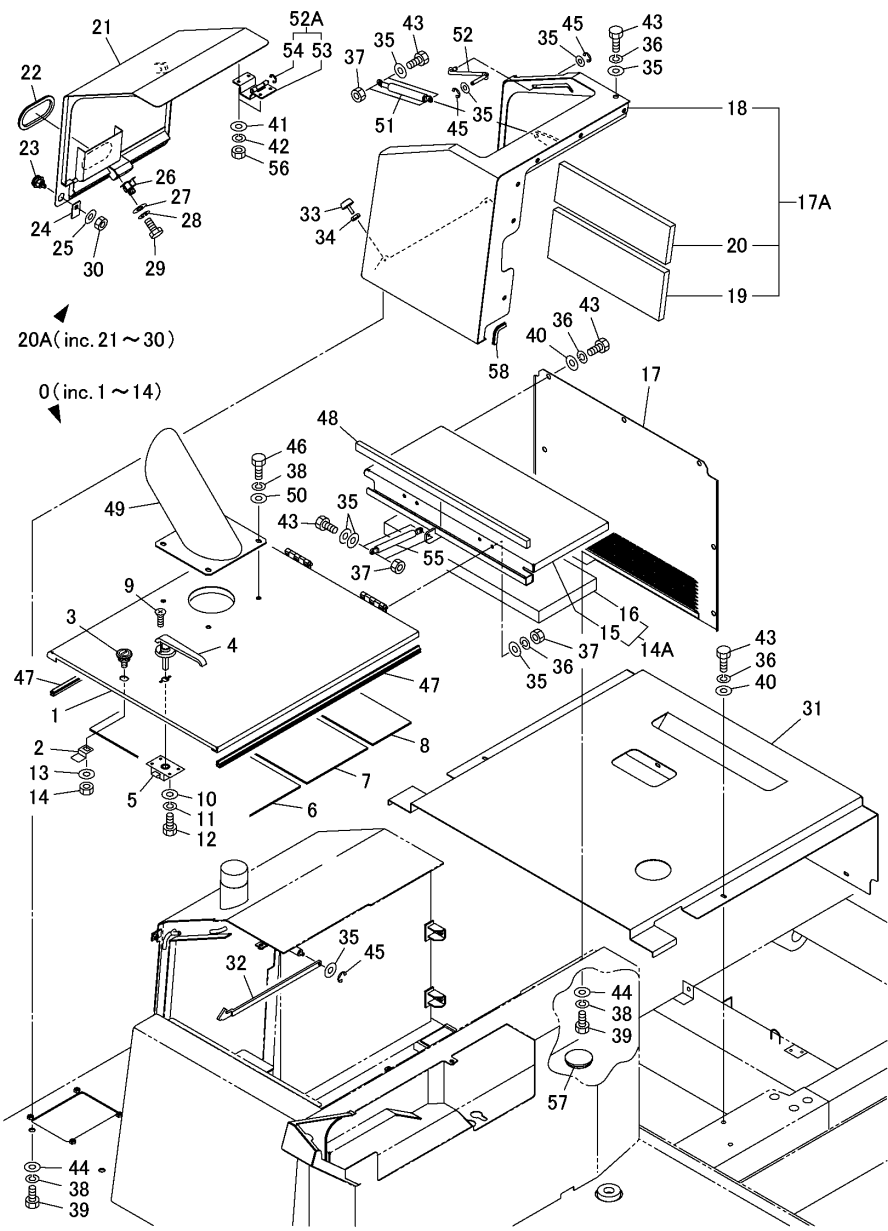
Fig.50. COVER(2/3)(CANOPY)
