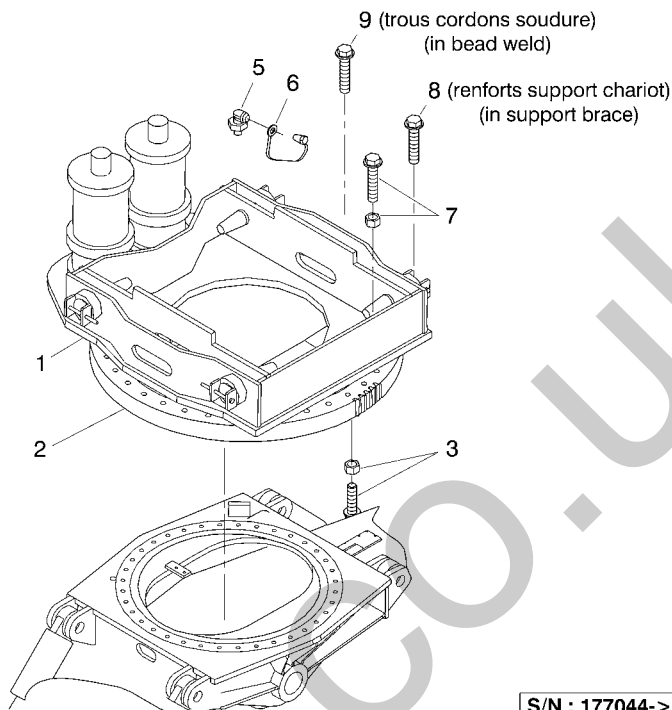
TOP-PICK+TILT
