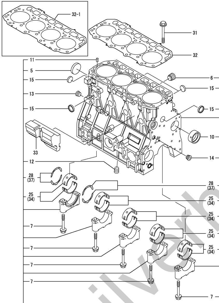
Fig.1. CYLINDER BLOCK
