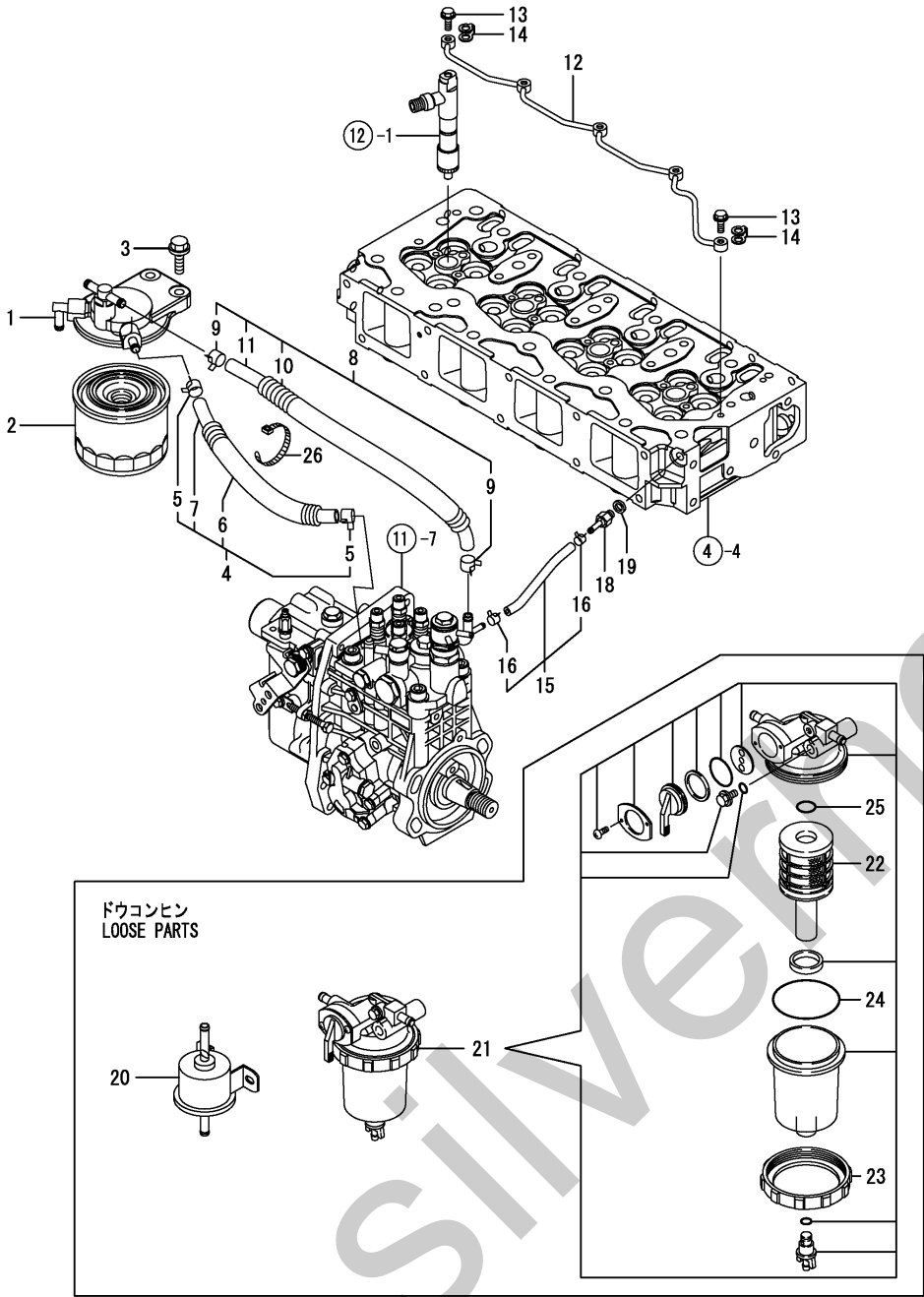
Fig.13. FUEL LINE
