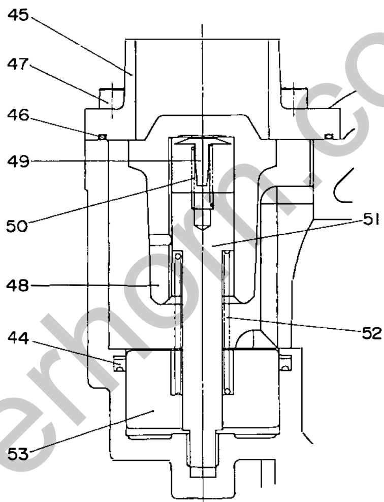
VIEW - Z
