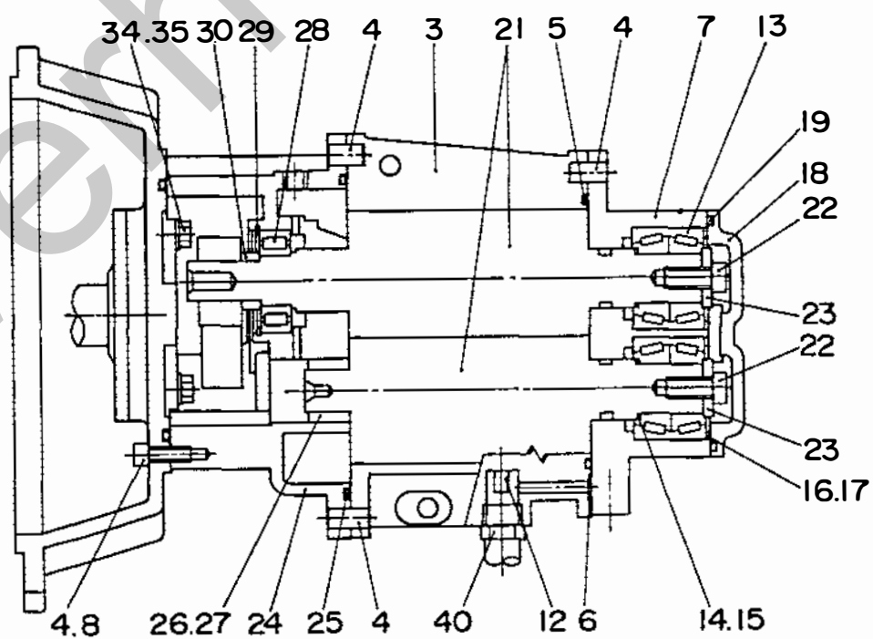
SECTION Y-Y
