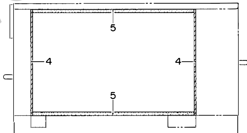
SECTION Z-Z
