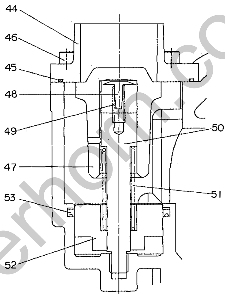
VIEW - Z
