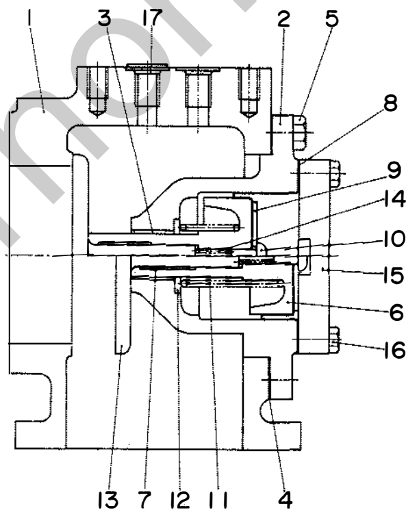
SECTION X-X
