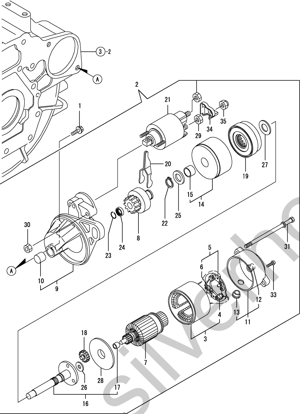
Fig.13. STARTING MOTOR
