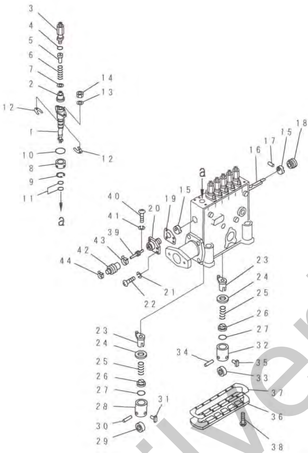
FIG. A4010-C7B1Z FUEL INJECTION PUMP (PUMP) (L.H.) (2/2) (FOR DCA800-SPK. SSKE) (INNER PARTS) (#12305-)
