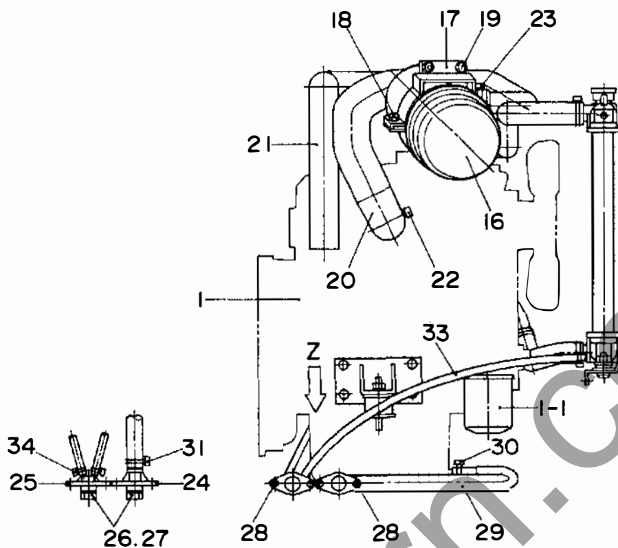
VIEW - Z
