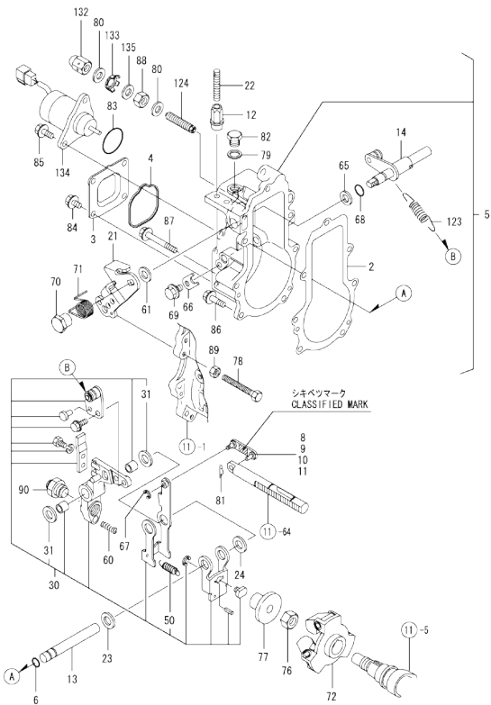
Fig.12. GOVERNOR
