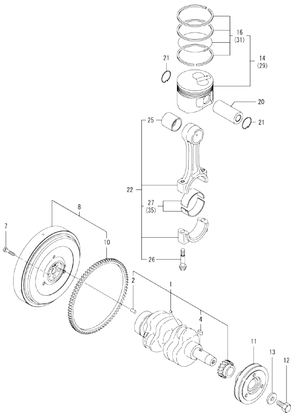
Fig.8. CRANKSHAFT & PISTON
