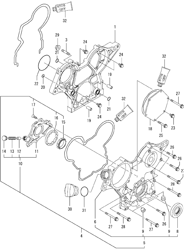
OCD10-M85401 3TNV70-QIK Fig.2. GEAR HOUSING
