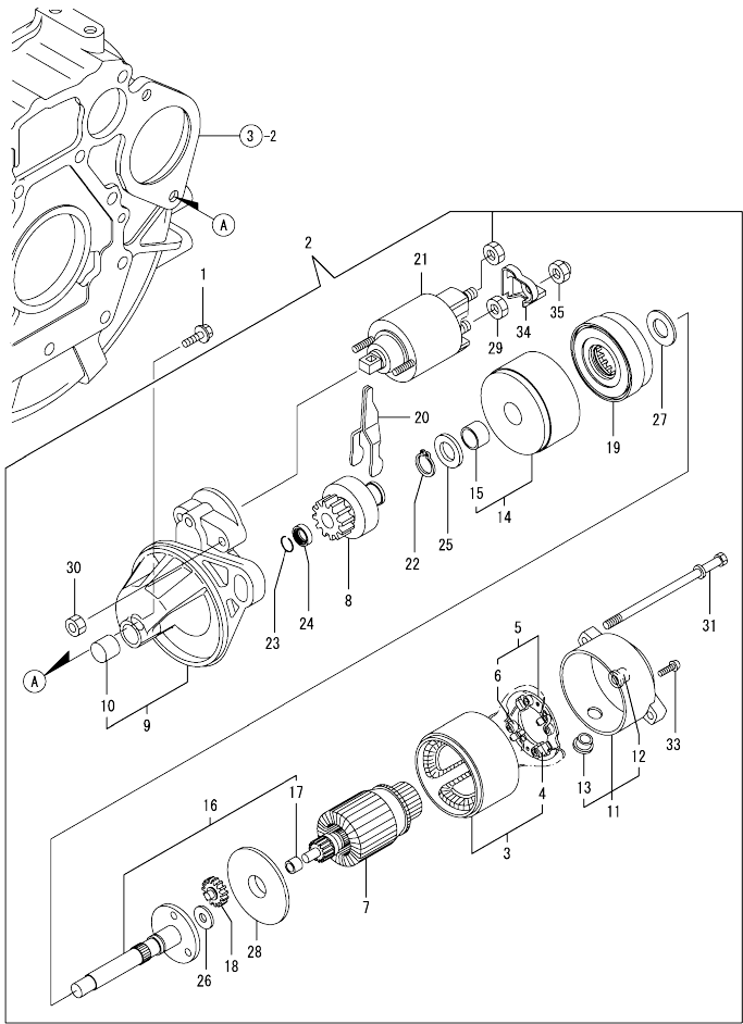
OCD10-M85401 3TNV70-QiK Fig.15. STARTING MOTOR
