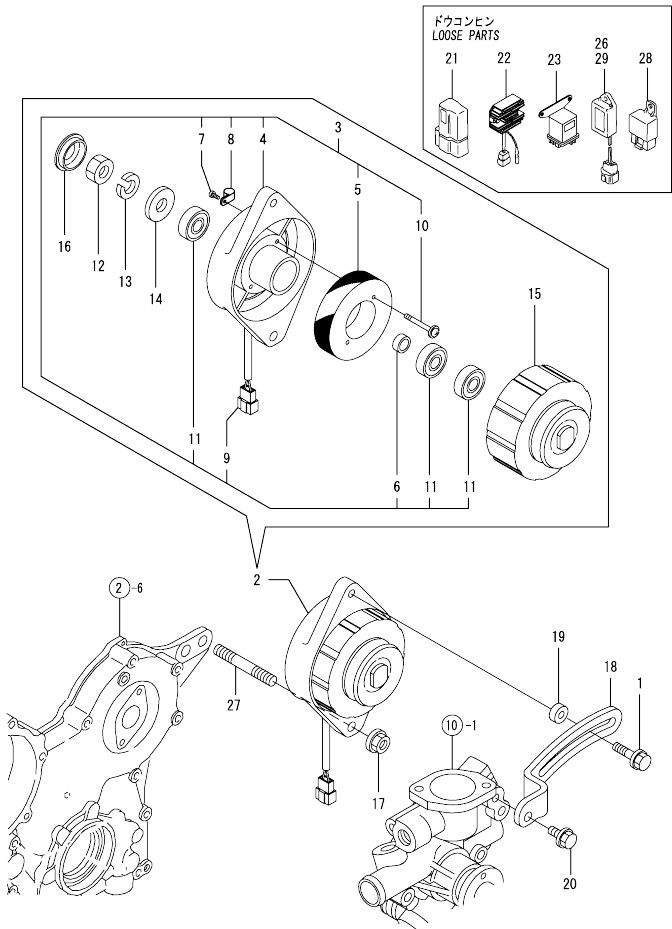
OCD10-M85401 3TNV70-QIK Fig.16. GENERATOR
