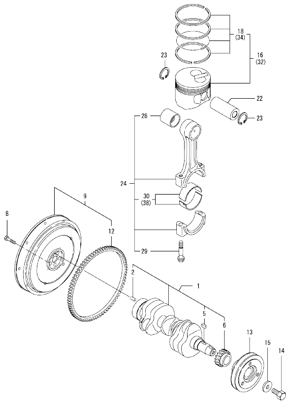
Fig.8. CRANKSHAFT & PISTON
