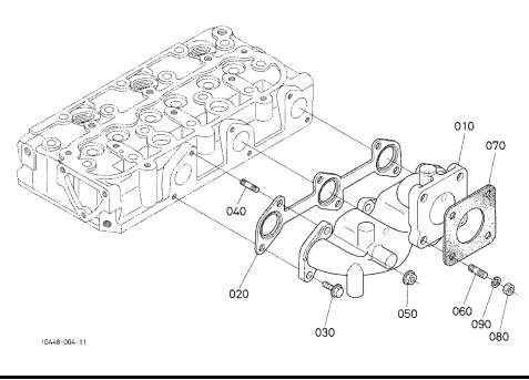
060200 ESCAPE COLECTOR
