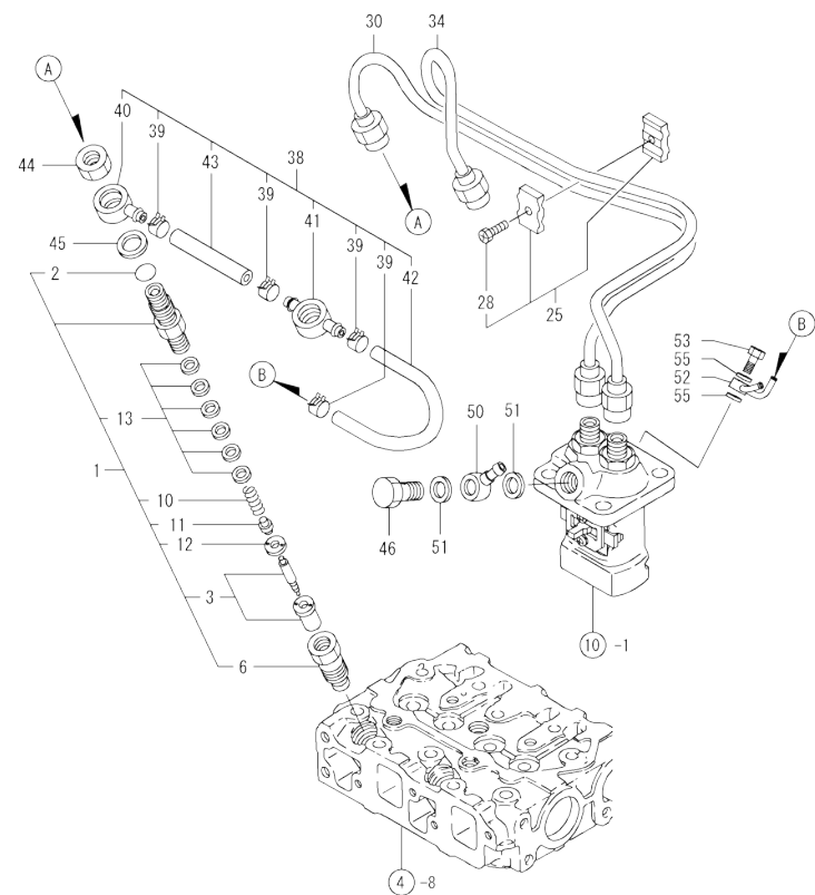
Fig.12. FUEL INJECTION VALVE
