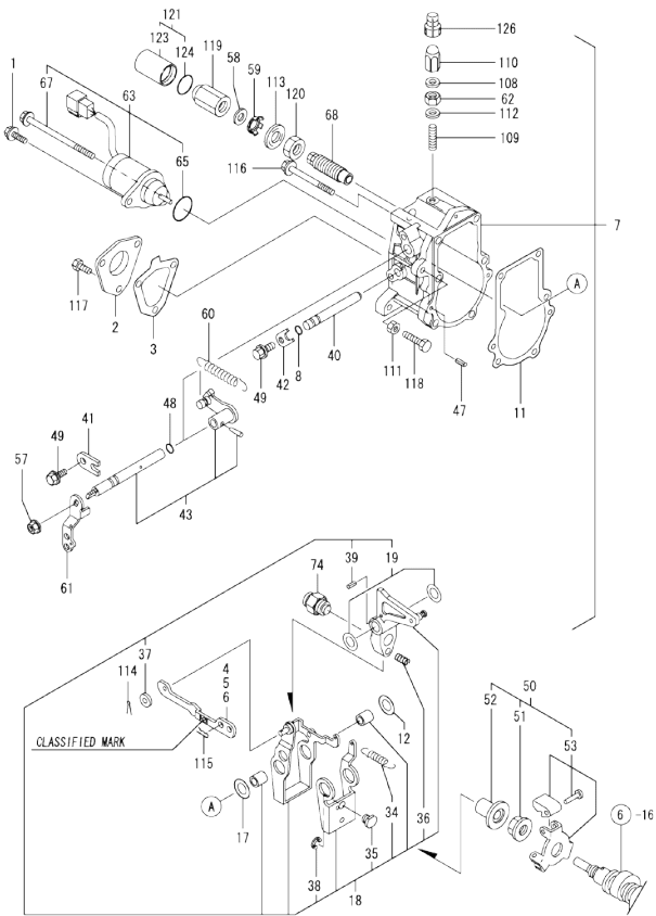
Fig.11. GOVERNOR
