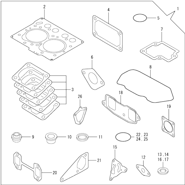
Fig.14. GASKET SET
