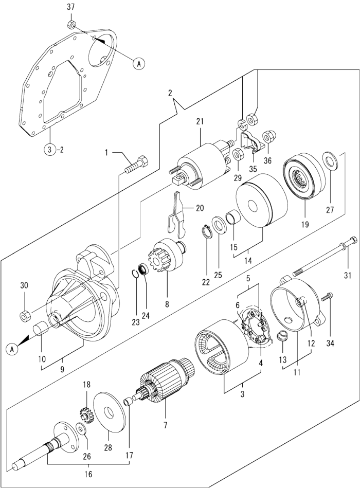
Fig.13. STARTING MOTOR
