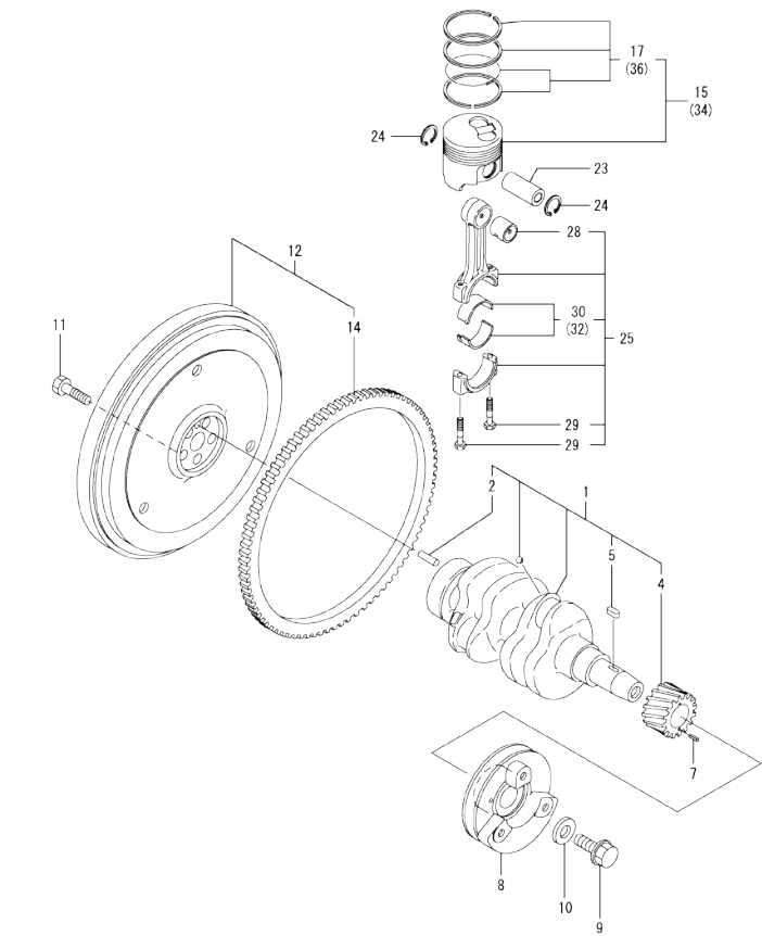
Fig.7. CRANKSHAFT & PISTON
