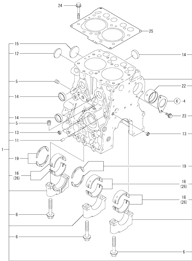
Fig.1. CYLINDER BLOCK
