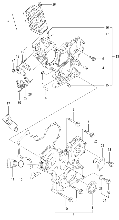
Fig.2. GEAR HOUSING
