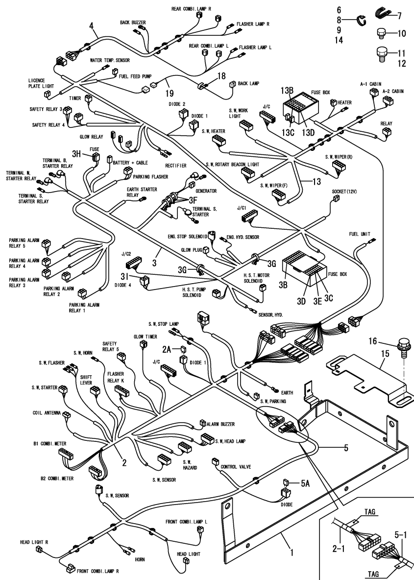
Fig.72. (11A)WIRING(FROM M61069)
