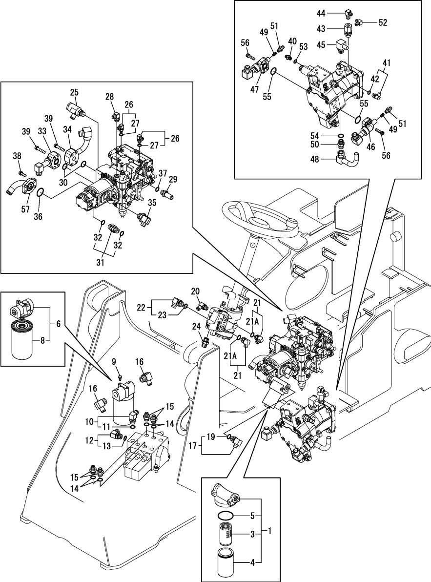
OCS10-M53302 V3-6(US)(AS)(NZ) Fig.55. FILTER & PIPE FITTING
