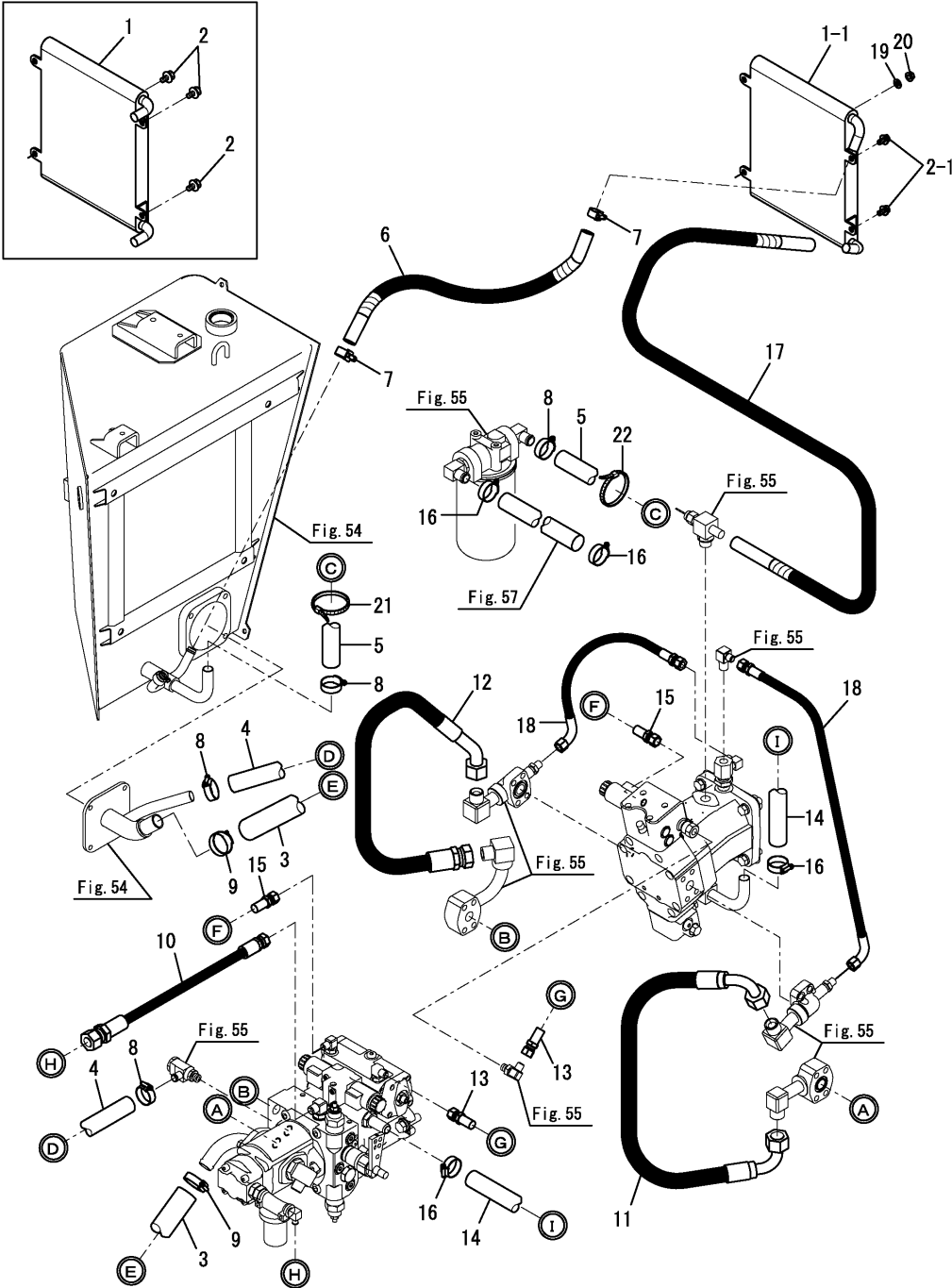
OCS10-M53302 V3-6(US)(AS)(NZ) Fig.56. HYD.OIL PIPING(HST)
