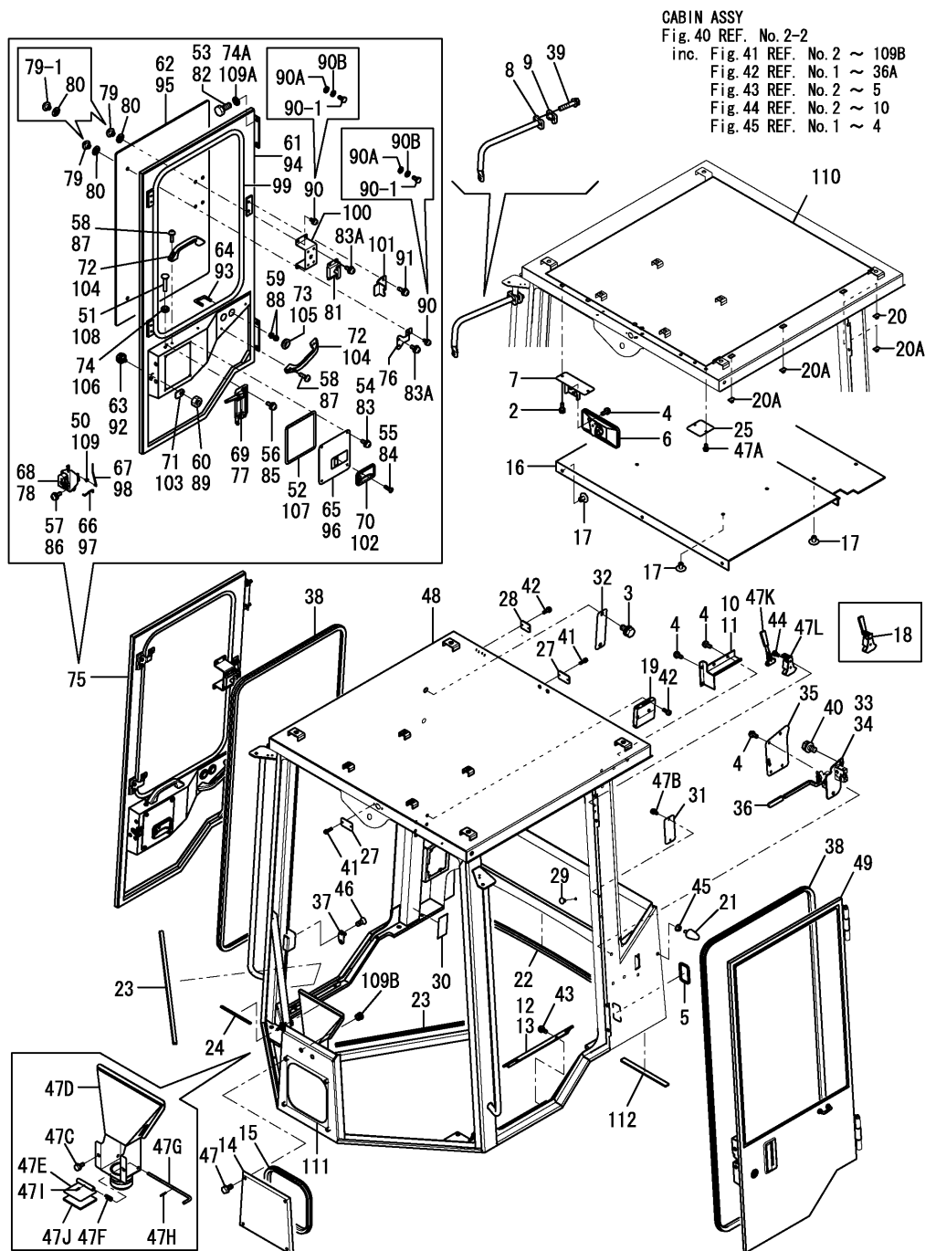
Fig.41. CABIN(DOOR)(CENTER DEFROSTER SPEC.)
