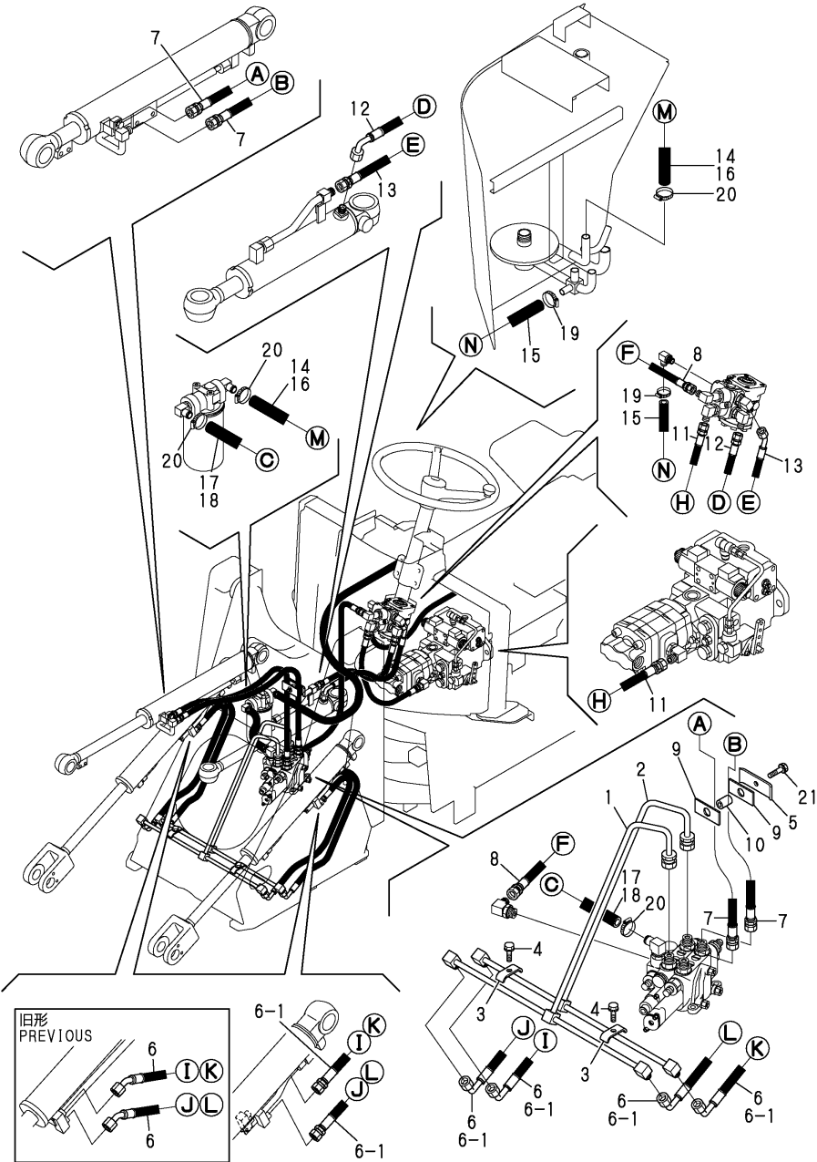
OCK20-M36003 V3/V4-5(A),V5(-A)(JP) Fig.99. HYD.OIL PIPING(LOADER 1)
