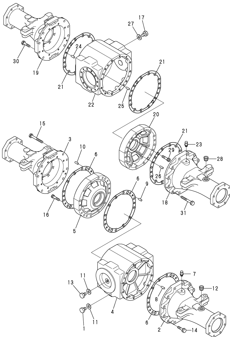
Fig.33. AXLE CASE(2)
