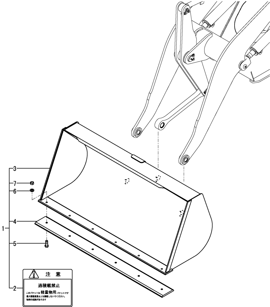
Fig.123. BUCKET(0.9)(PLATING) KIT(OPTIONAL)
