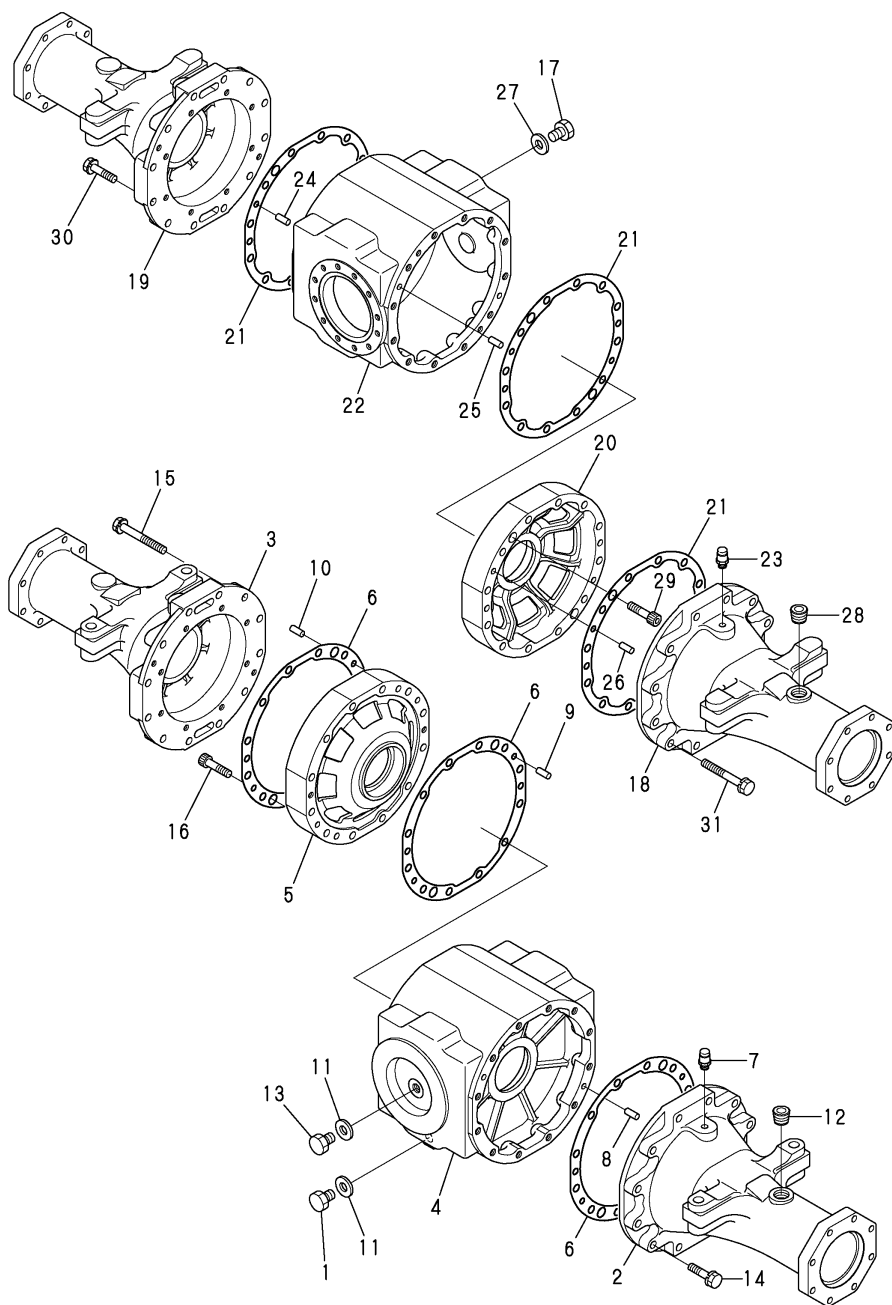
Fig.32. AXLE CASE(1)
