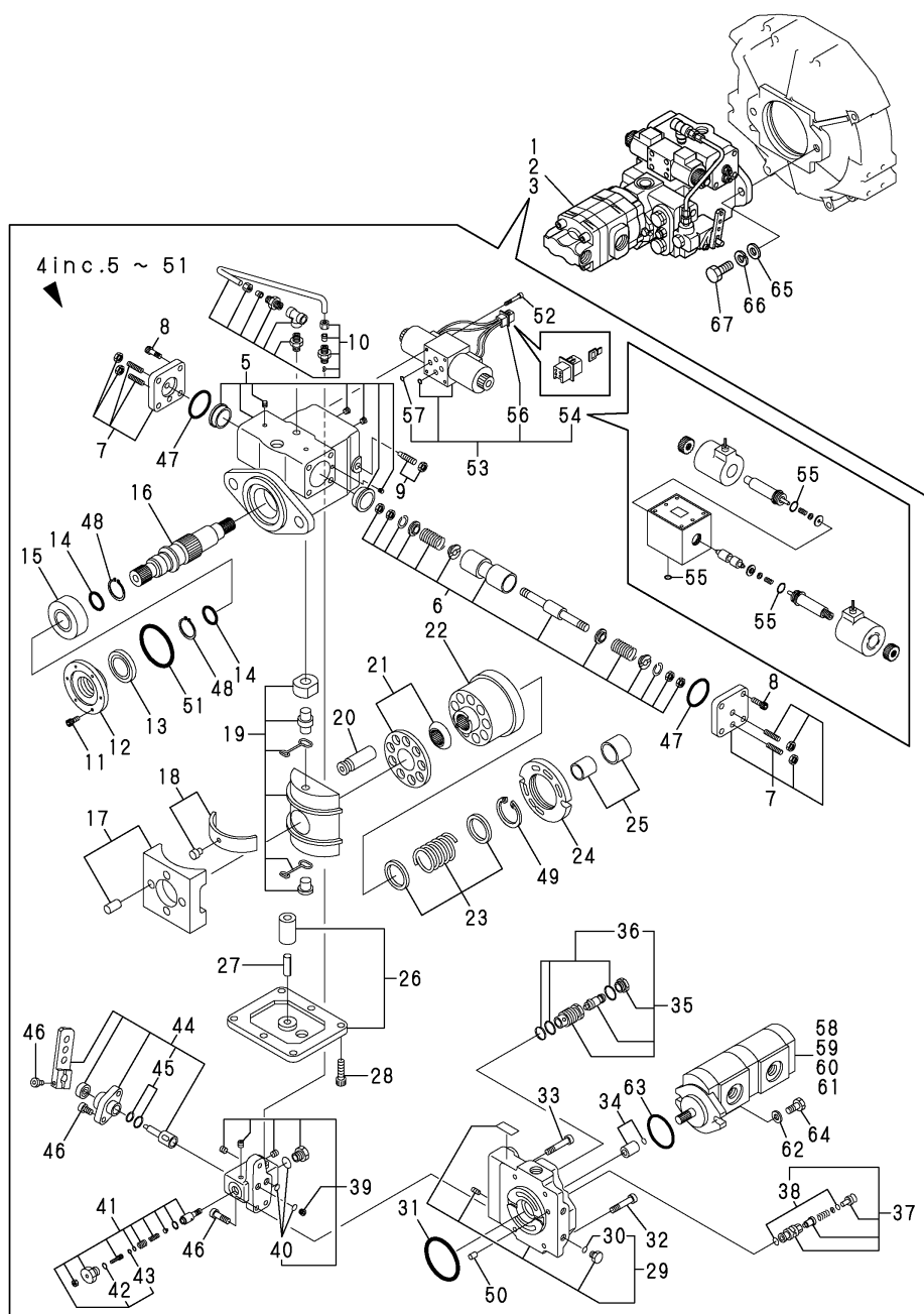
Fig.82. HST PUMP
