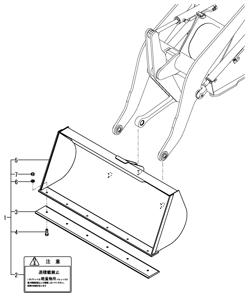
0CK20-M36003 V3/V4-5(A),V5(-A)(JP) Fig.117. BUCKET(0.5) KIT(OPTIONAL)
