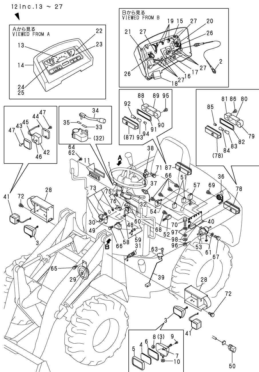
Fig.19. ELECTRIC PART(1)
