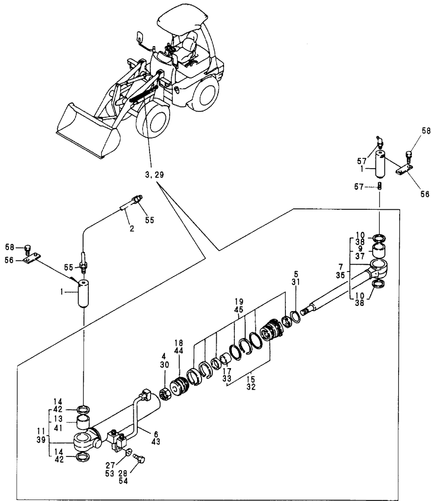
Fig.53 PSシリンダ POWER STEERING CYLINDER
