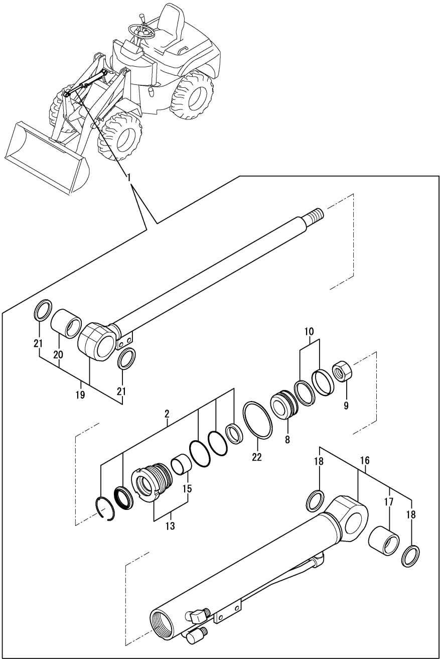
Fig.43. DUMP CYLINDER
