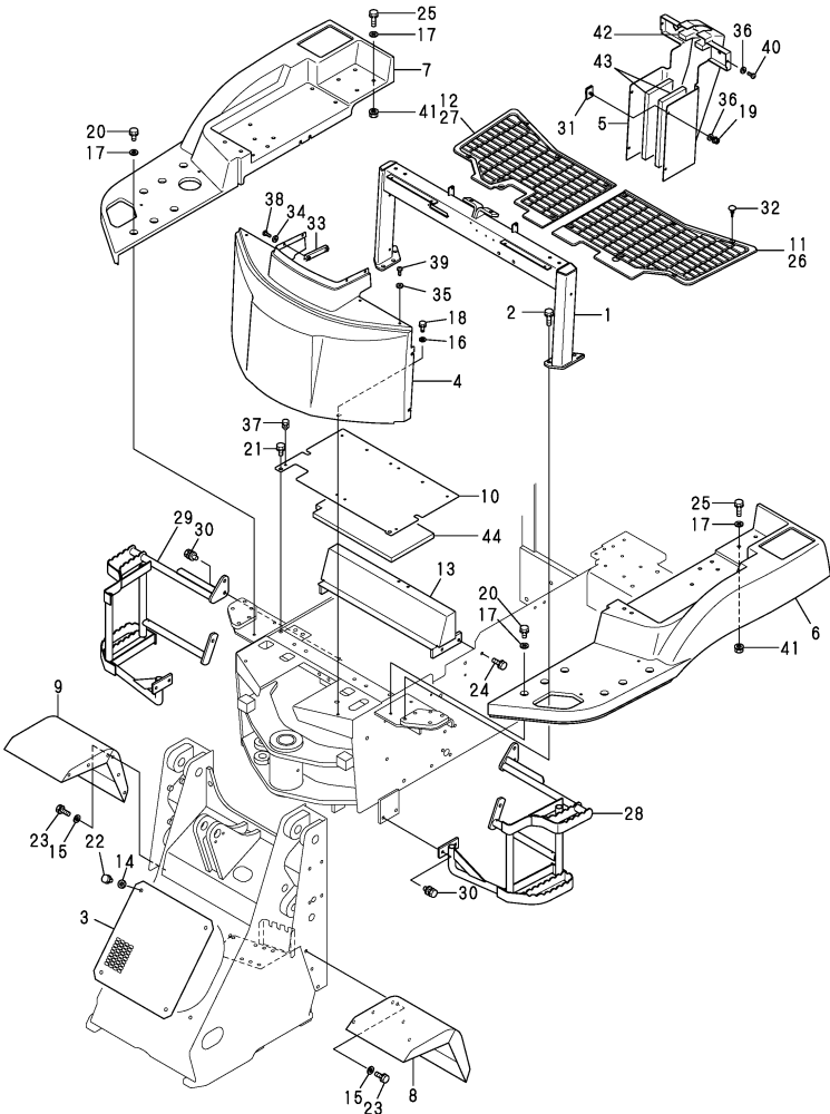
Fig.32. OPERATION FRAME & COVER
