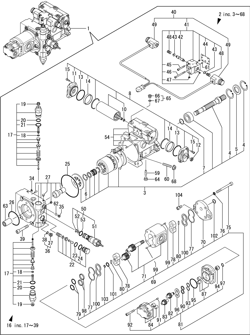
Fig.53. HYDRAULIC PUMP(INNER PARTS)
