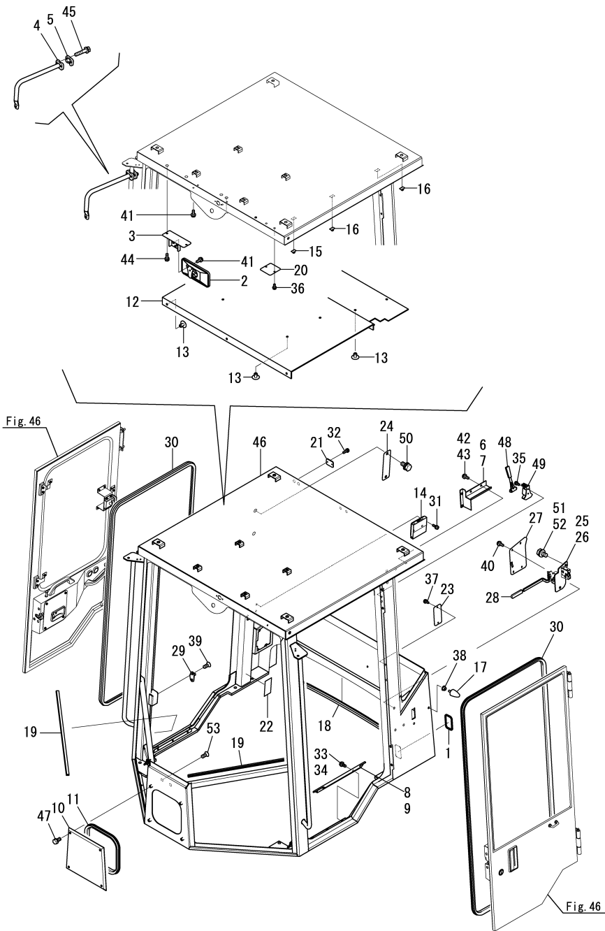
OCK50-M00410 CABIN Fig.45. CABIN FRAME
