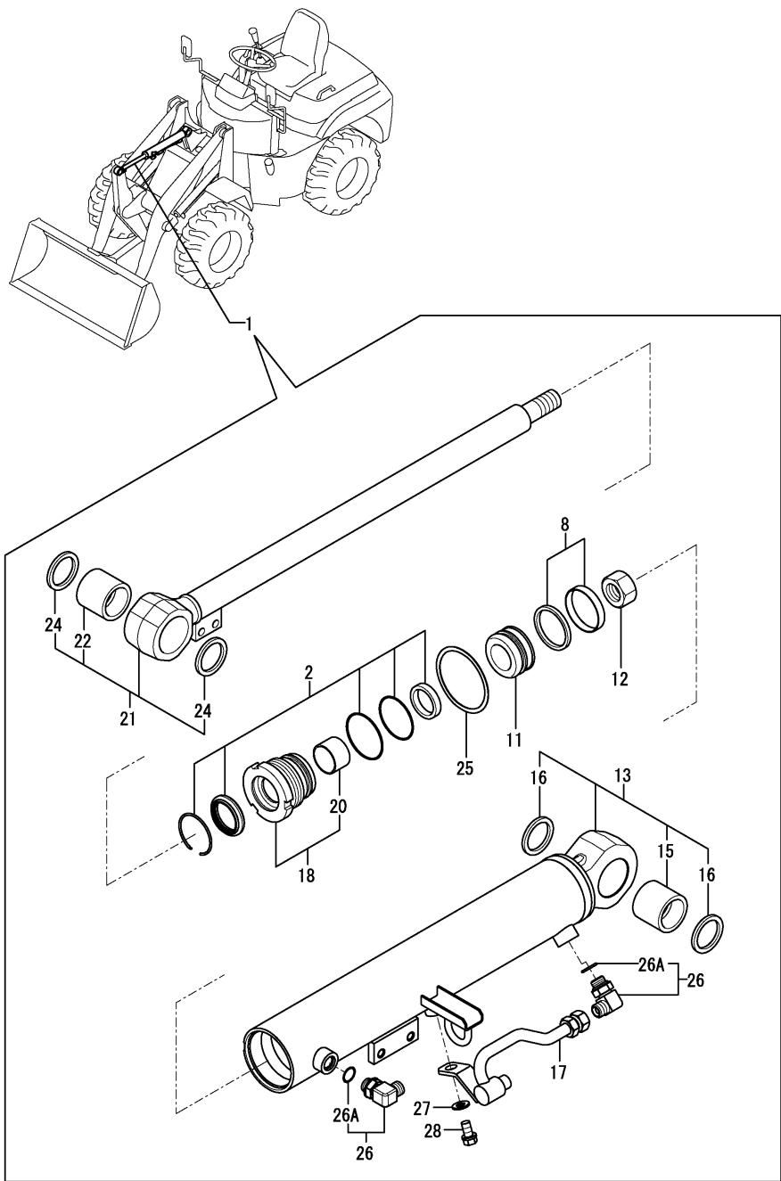
Fig.50. DUMP CYLINDER
