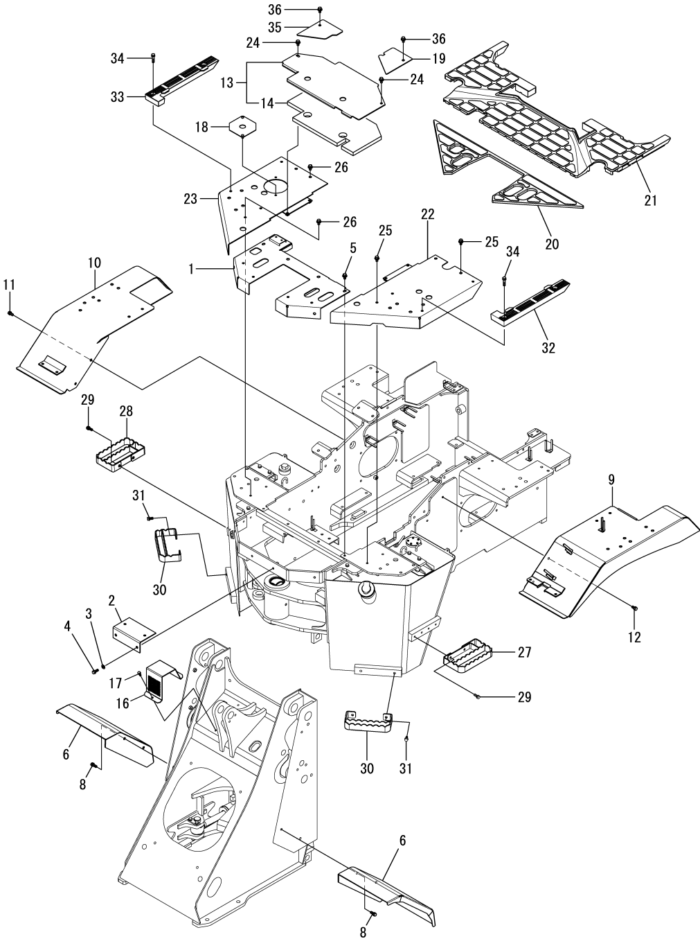
Fig.39. COVER & STEP(AIR CONDITIONER SPEC.)
