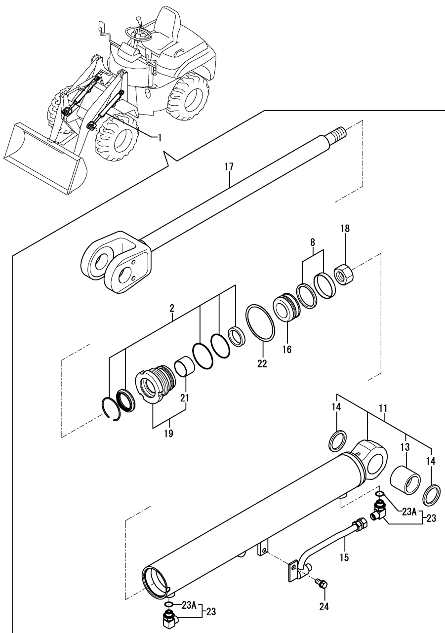
Fig.49. LIFT CYLINDER
