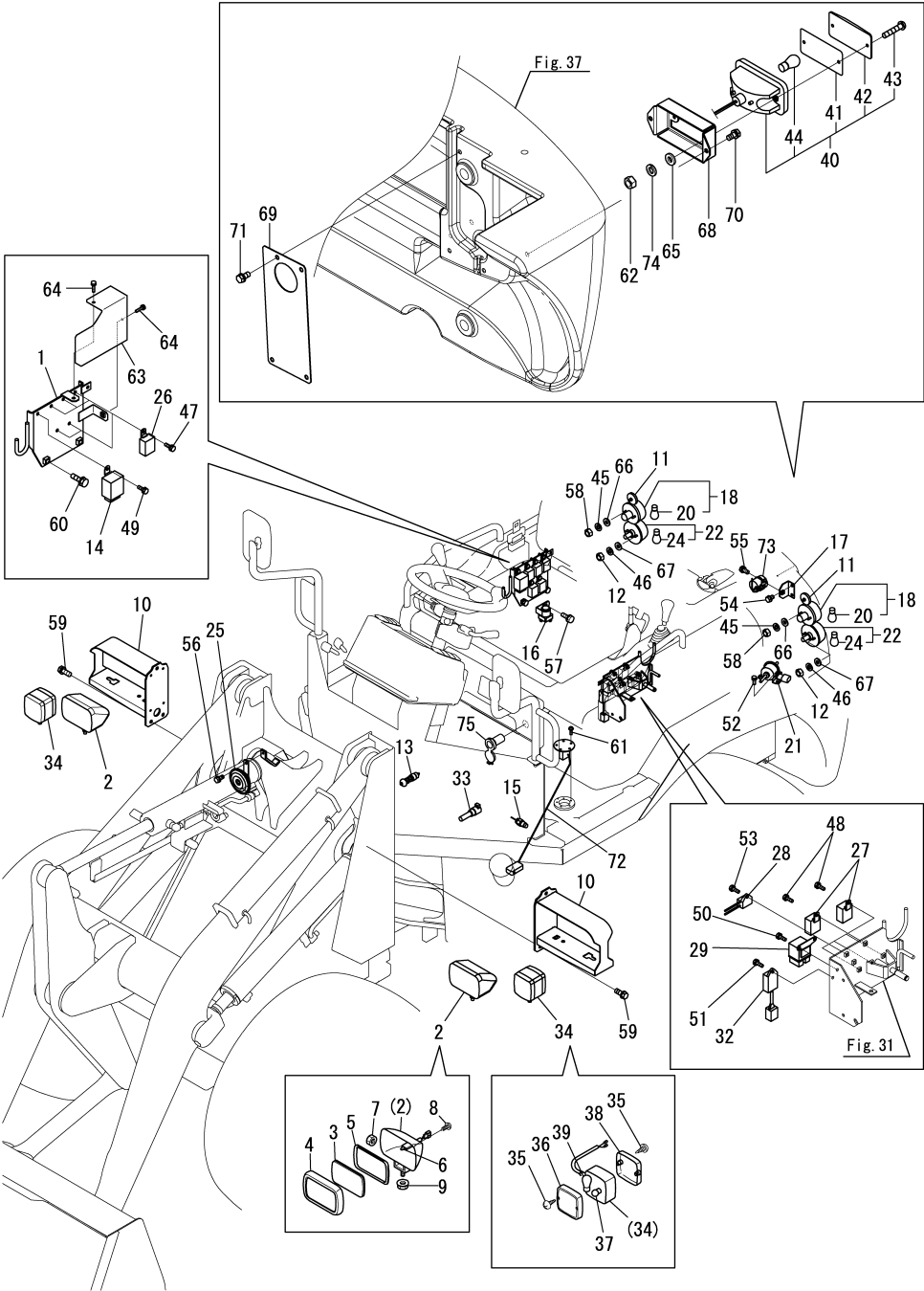
Fig.12. ELECTRIC PARTS(1)
