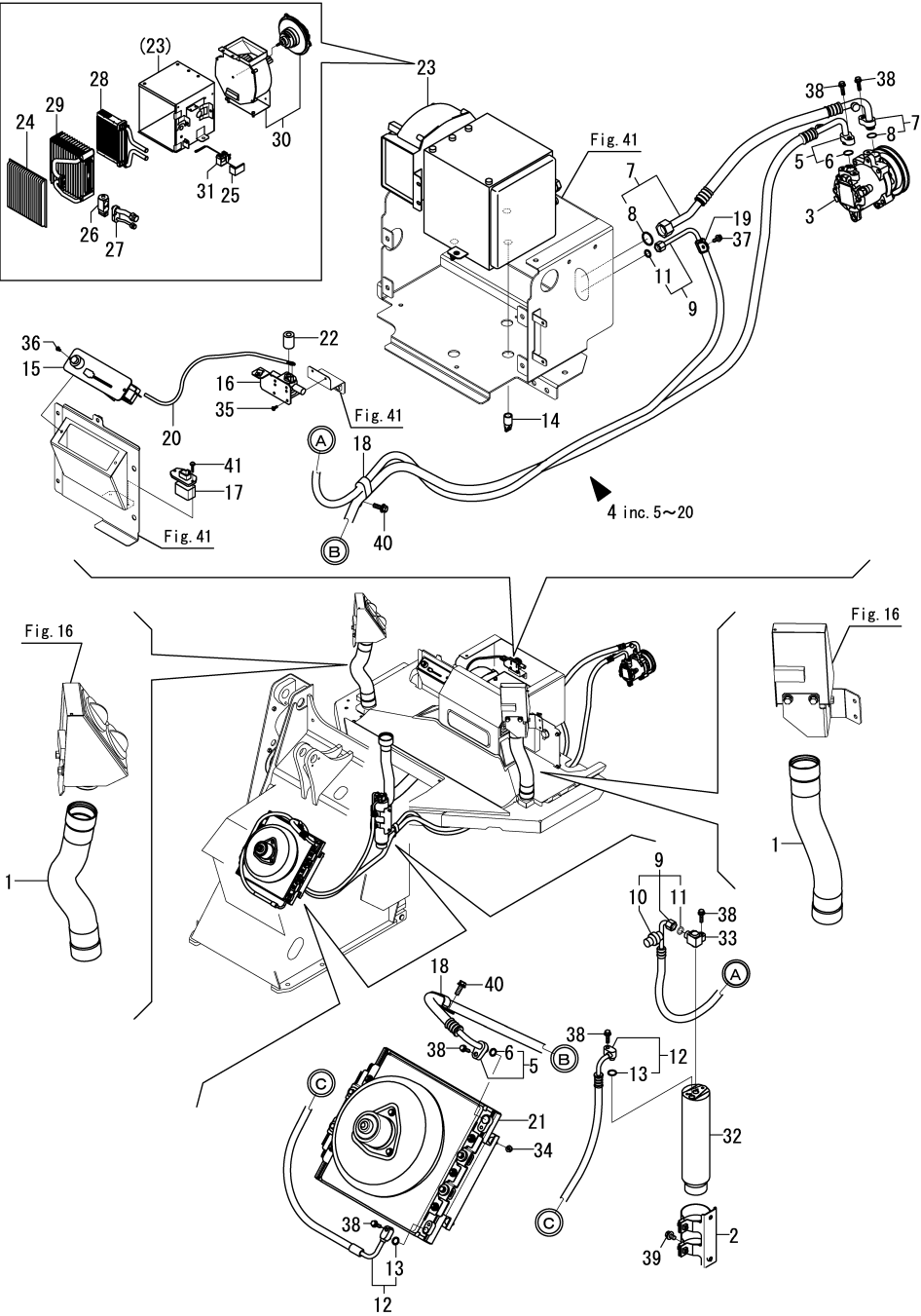
Fig.18. AIR CONDITIONER(ELECTRIC PARTS)
