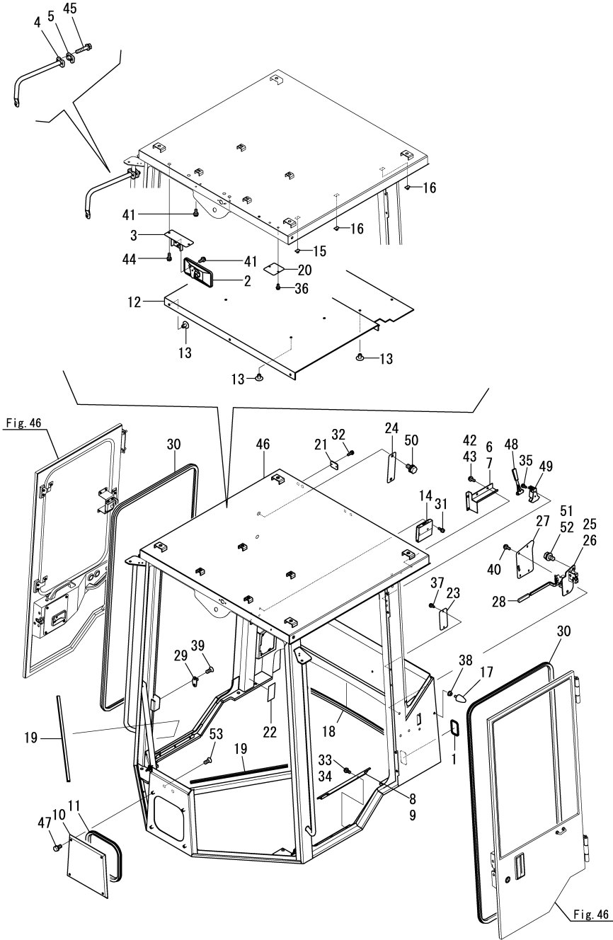
Fig.45. CABIN FRAME
