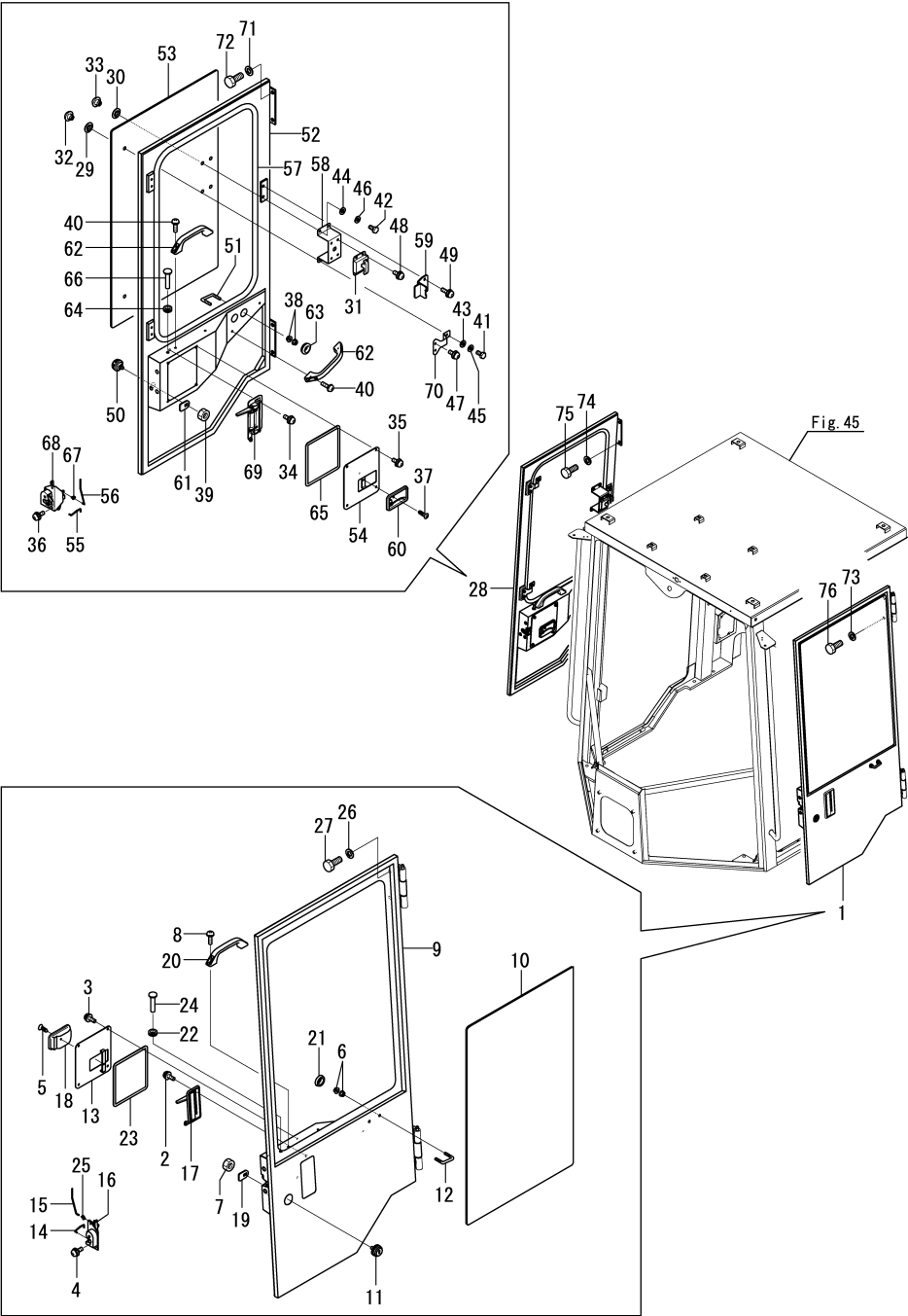
Fig.46. CABIN DOOR
