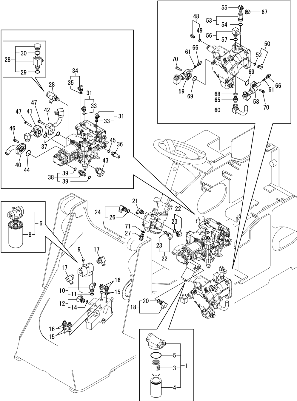
Fig.59. FILTER & FITTING
