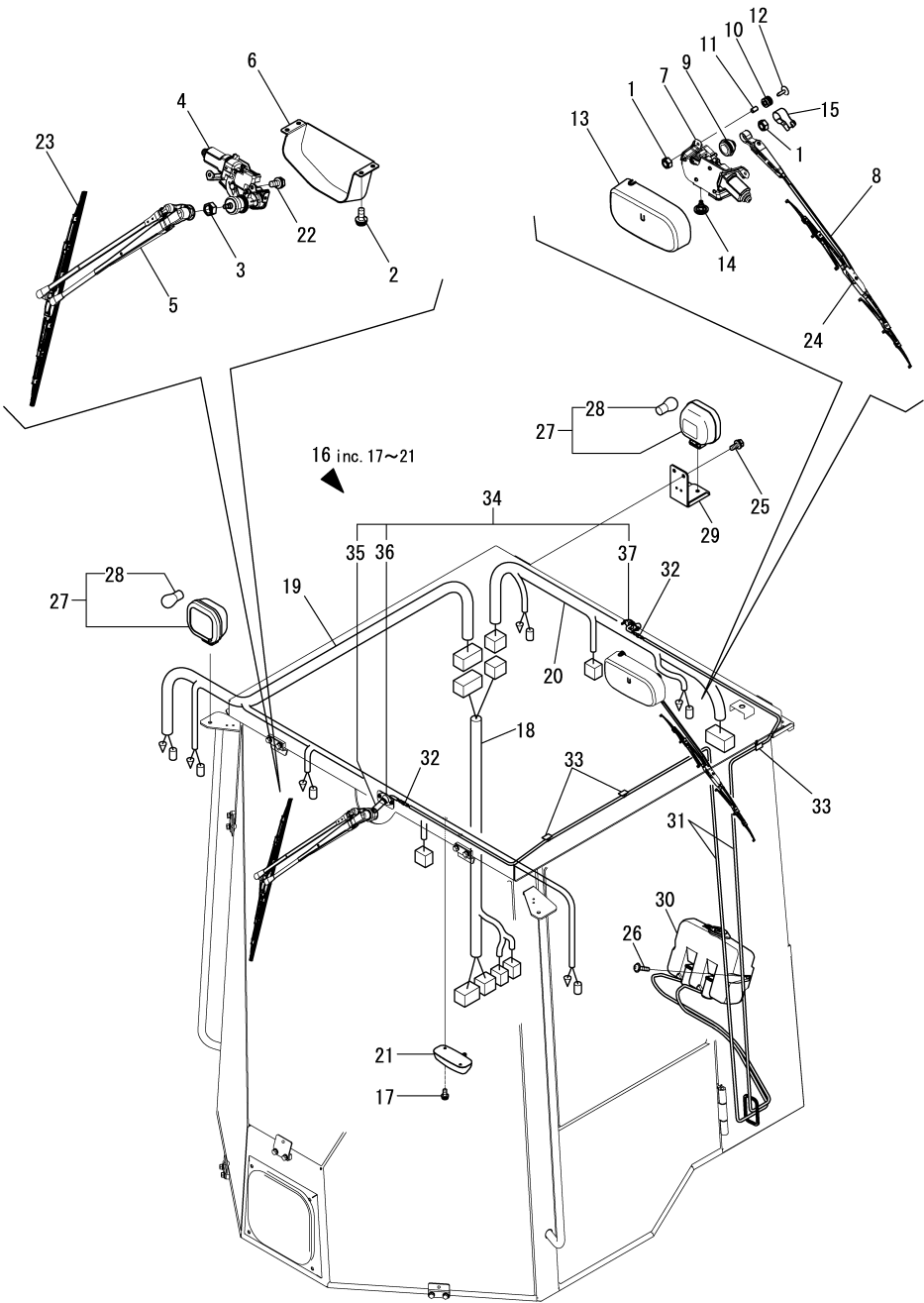
Fig.48. CABIN(ELECTRIC PARTS)
