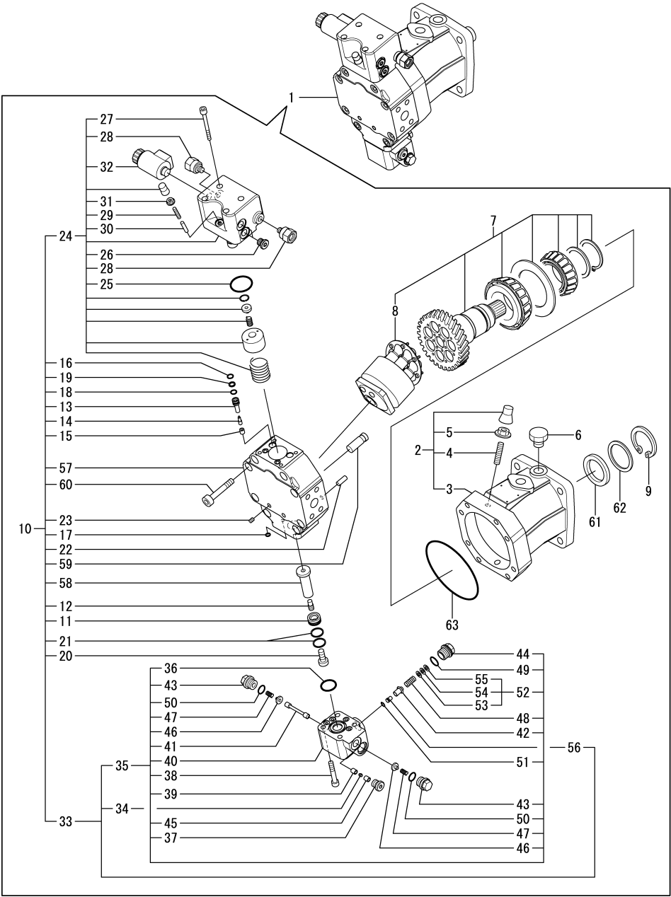
Fig.55. HYDRAULIC MOTOR(INNER PARTS)
