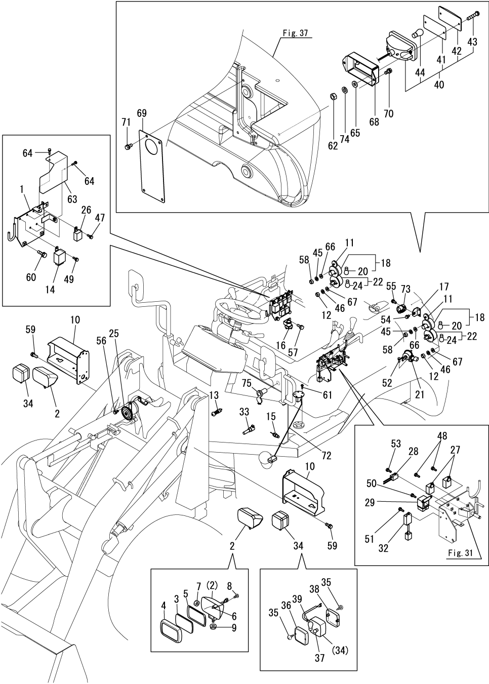
Fig.12. ELECTRIC PARTS(1)
