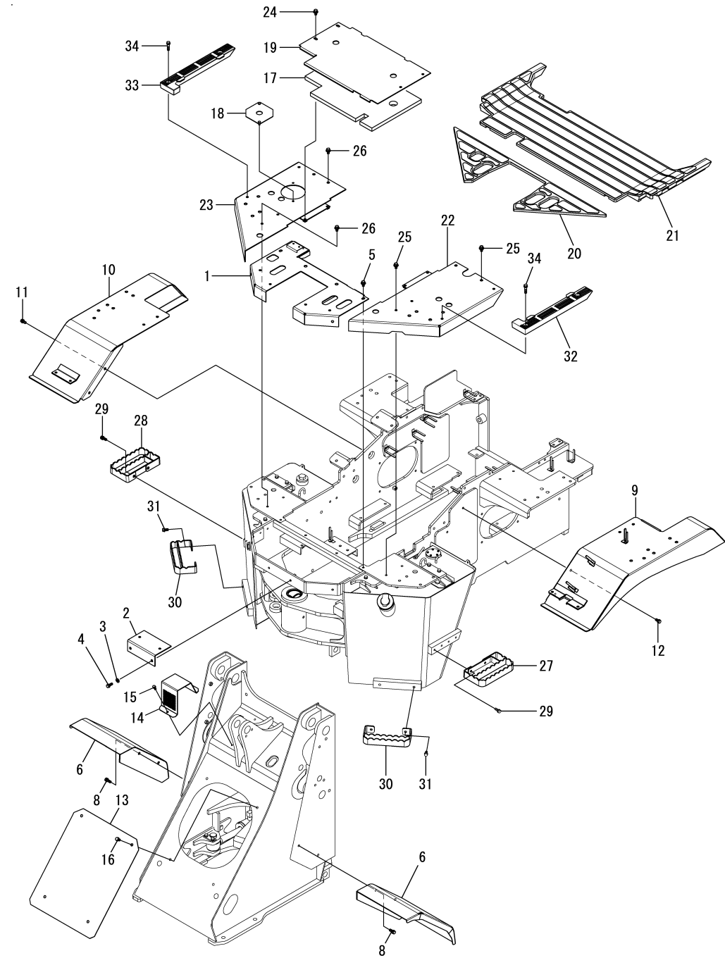
Fig.38. COVER & STEP
