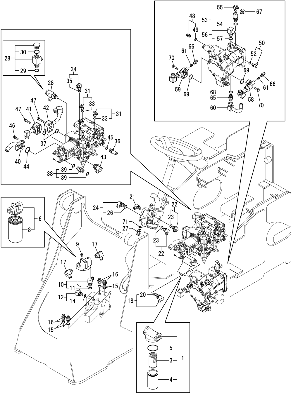
Fig.59. FILTER & FITTING
