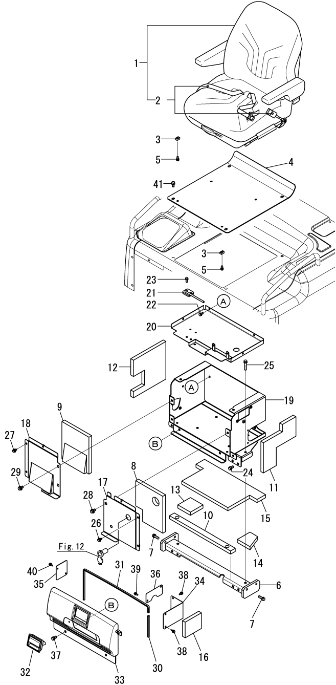
Fig.40. SEAT & SEAT MOUNT
