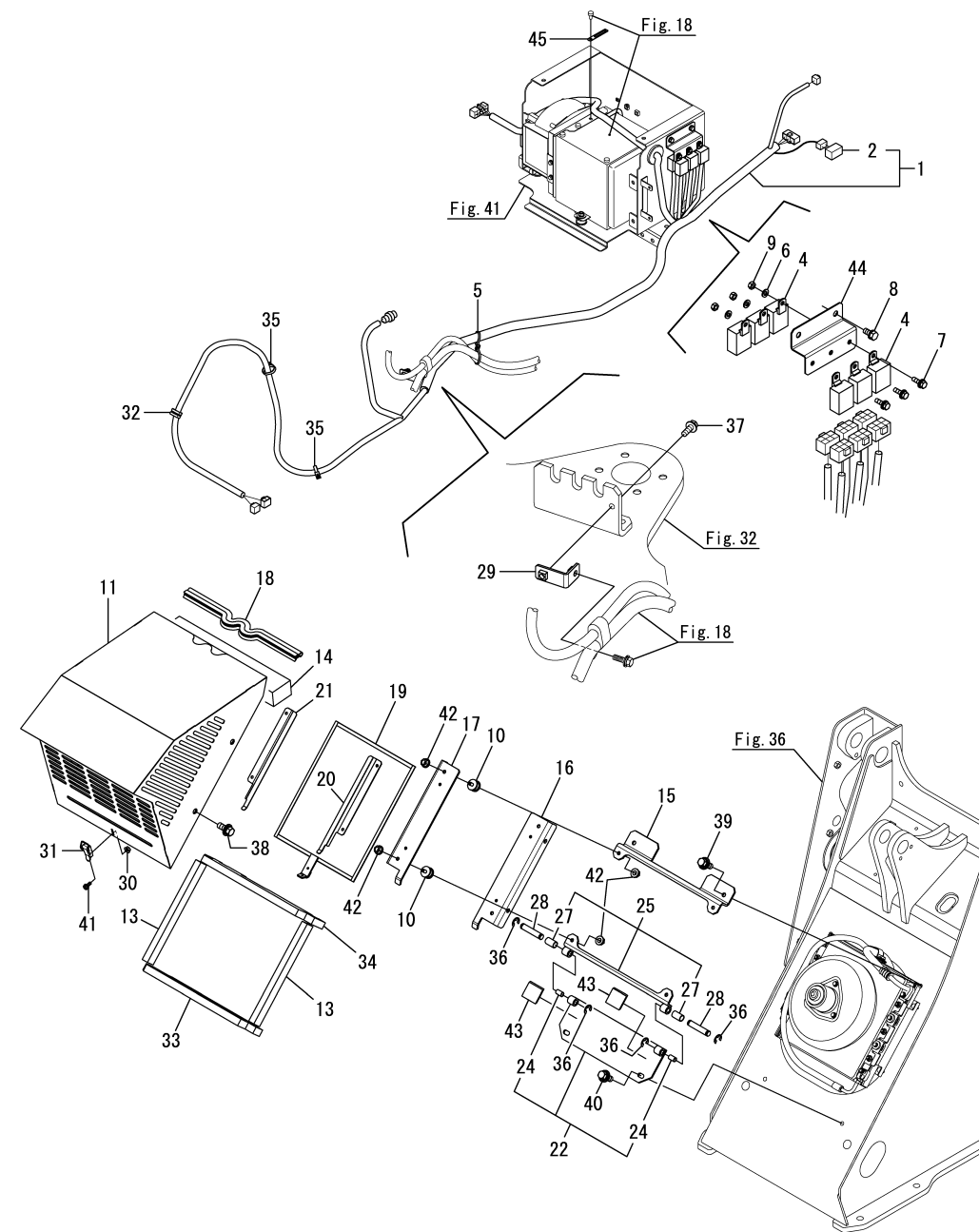
Fig.15. AIR CONDITIONER(FRONT)
