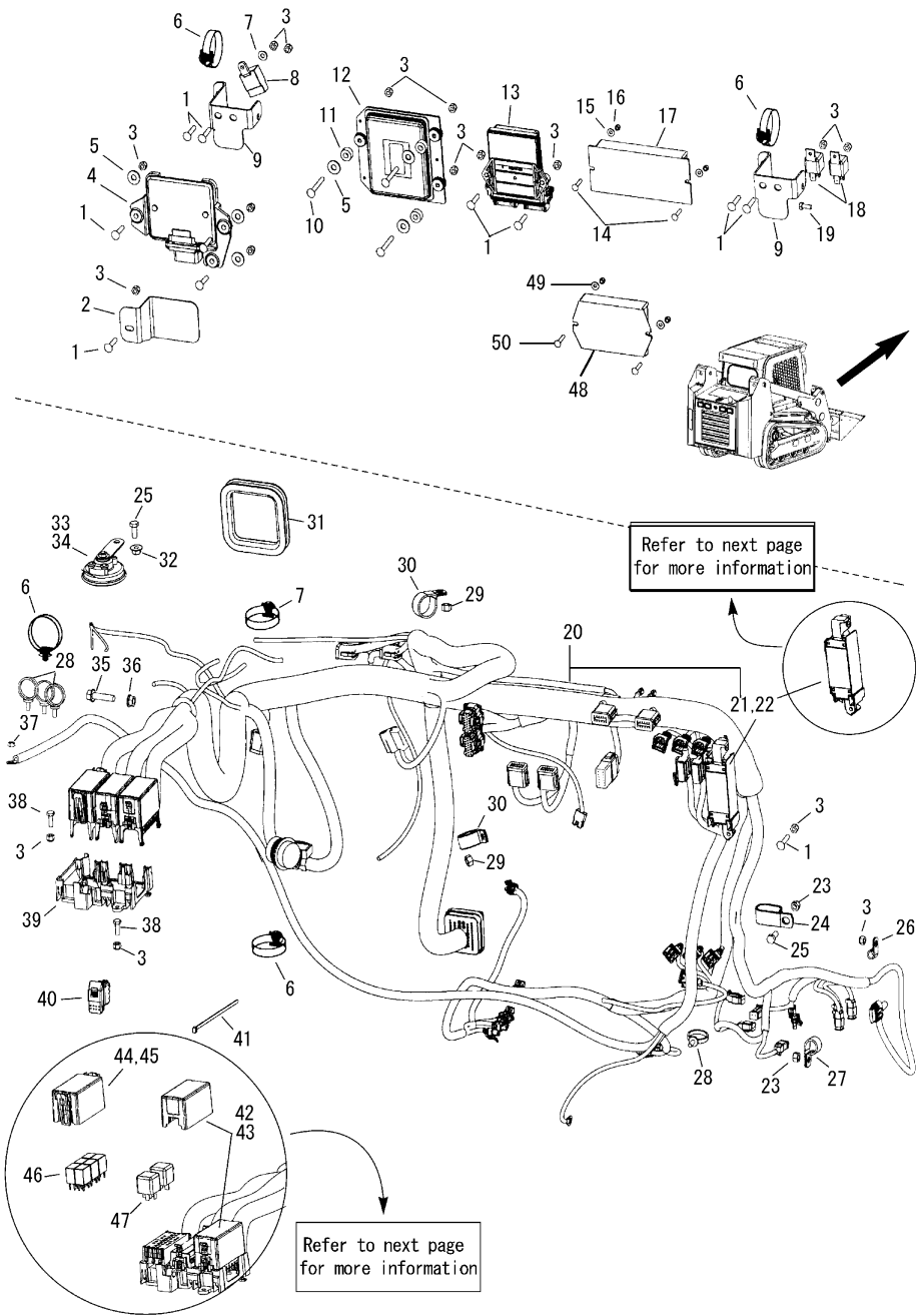
Fig.27. CHASSIS,WIRE HARNESS,COMPONENT
