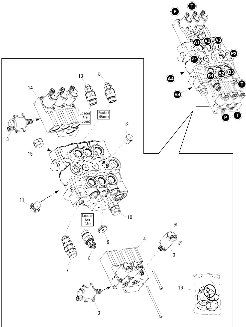
Fig.69. HYDRAULIC MAIN VALVE(HIGH FLOW
