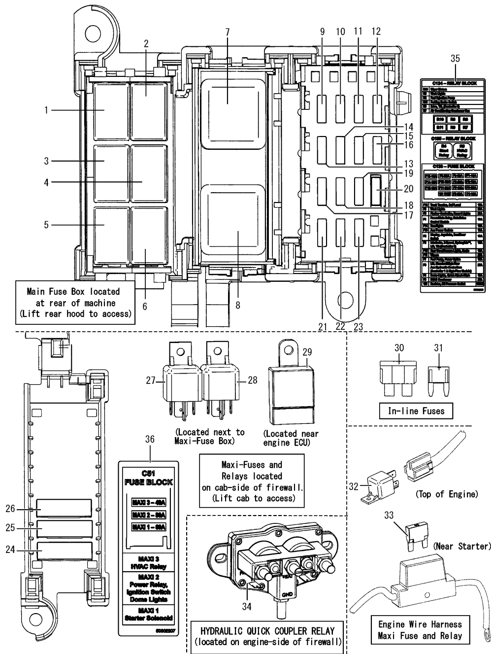
Fig.28. FUSE BOXES,FUSES,RELAYS
