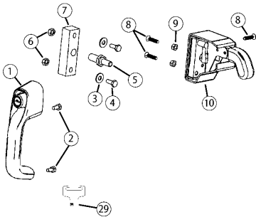
SERIES II and III DOOR LATCH
