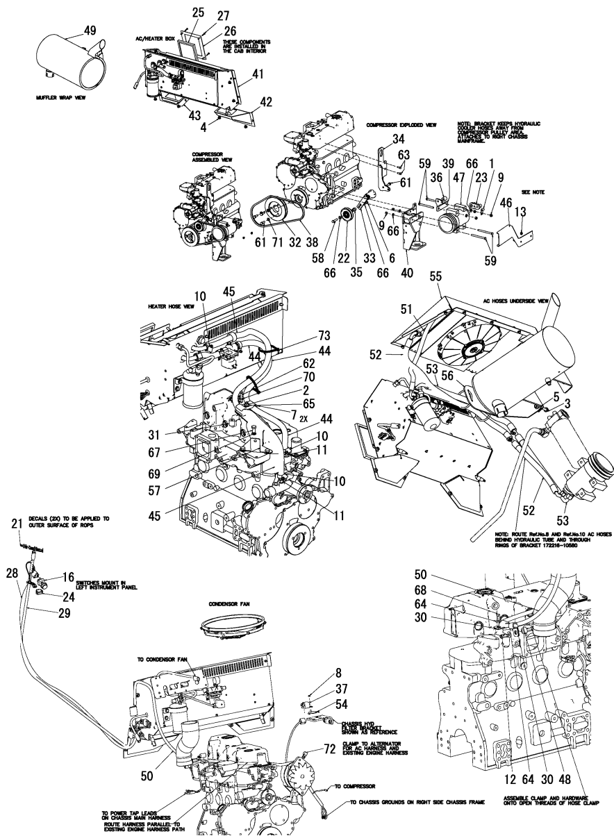
OCS10-M56600 MAIN LOADER COMPONENTS Fig.2. CHASSIS(HVAC COMPLETING)
