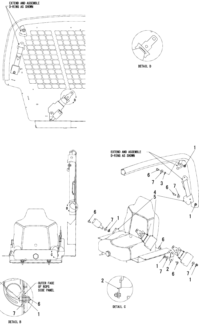
Fig.15. SEATS-THREE-POINT RESTRAINT SEAT BELT OPTION
