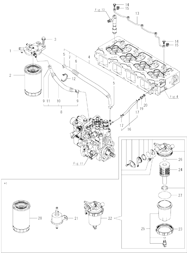
Fig.14. FUEL PIPING
