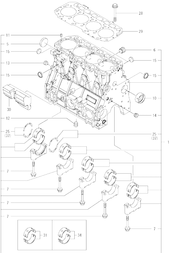
Fig.1. CYLINDER BLOCK
