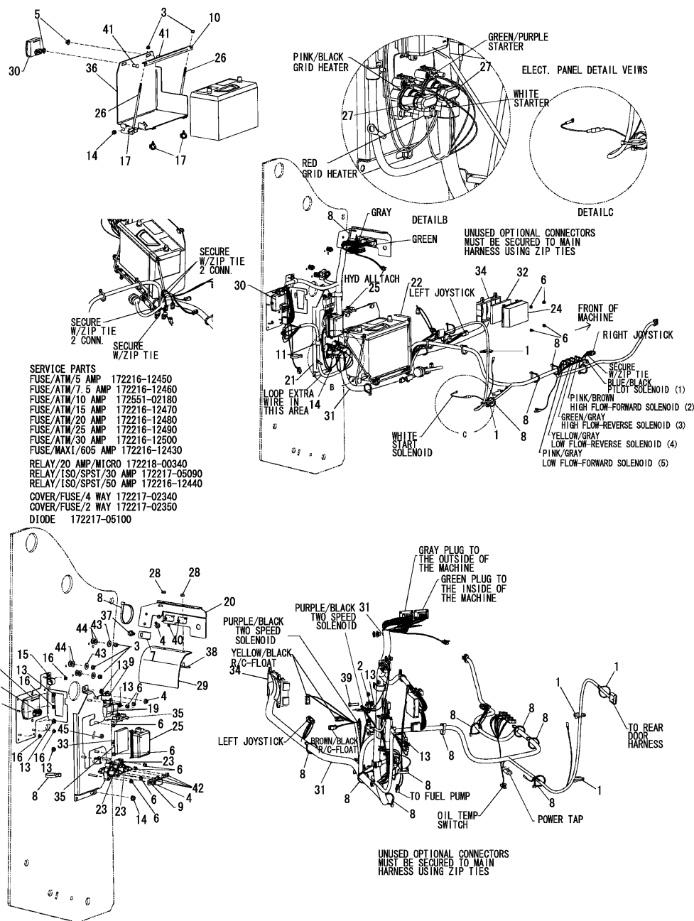
Fig.42. ELECTRICAL - CHASSIS
