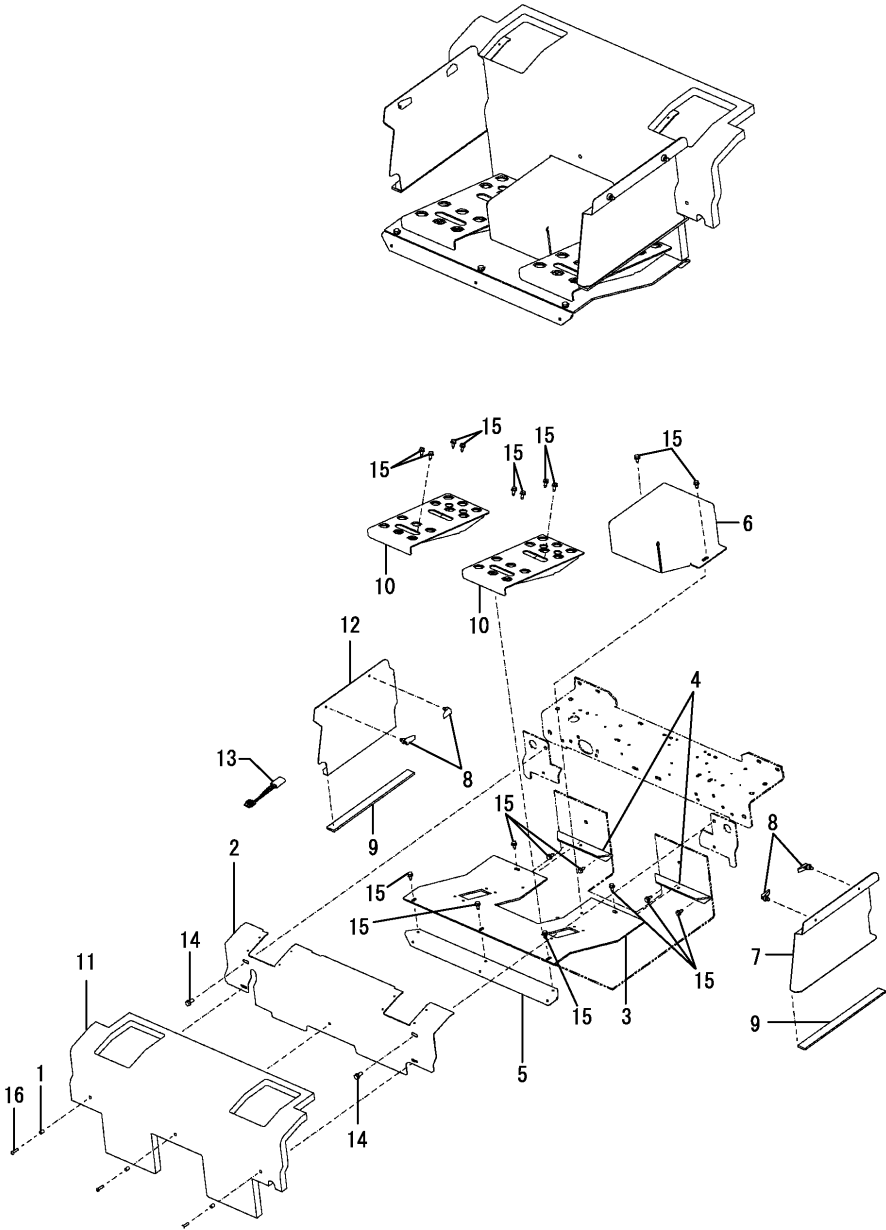
Fig.7. CHASSIS(COVERS - DUAL JOYSTICK CONTROLS)
