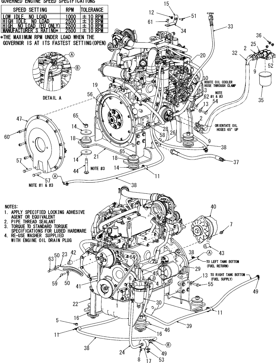
Fig.21. ENGINE
