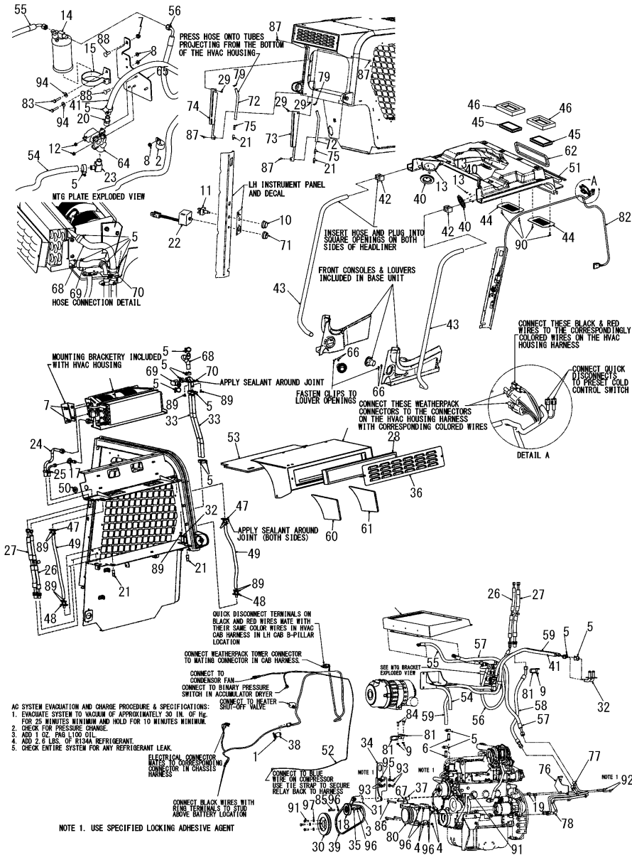
OCS10-M56800 MAIN LOADER COMPONENTEN Fig.2. CHASSIS(HVAC COMPLETING)
