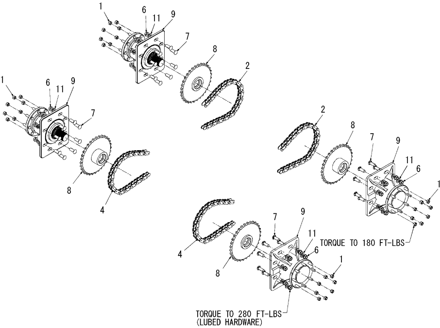
Fig.19. WHEEL DRIVES
