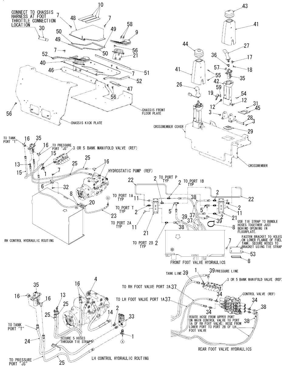
Fig.32. CONTROLS - LIFT/TILT AND TRACTION(HAND/FOOT CONTROLS)
