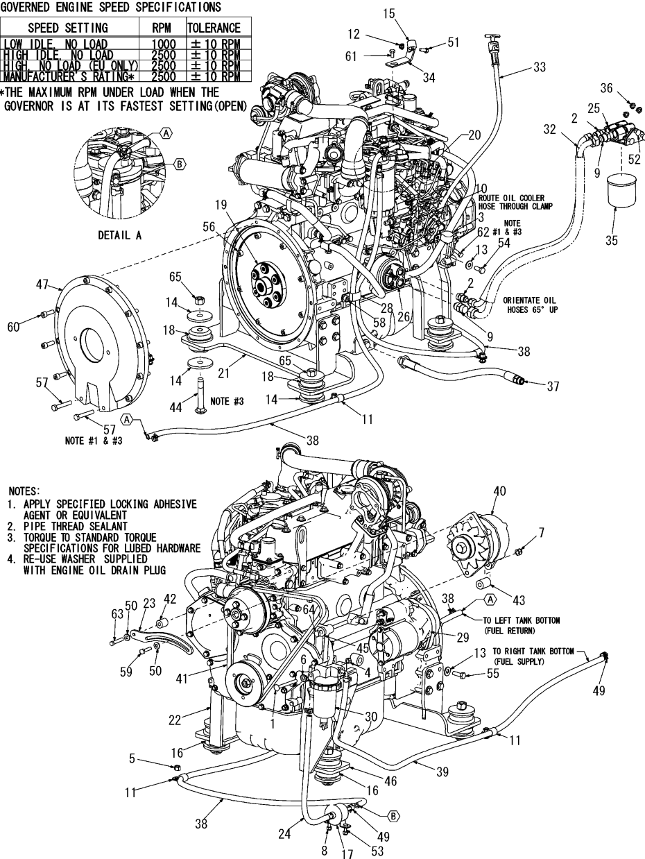
Fig.21. ENGINE
