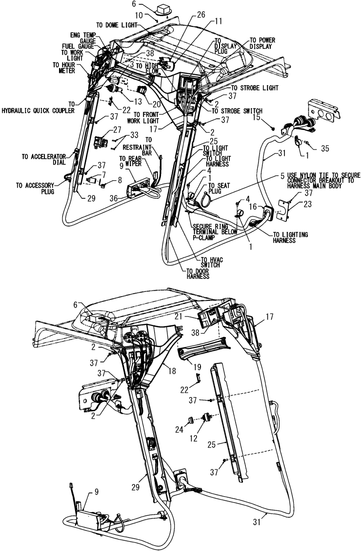
OCS10-M56800 MAIN LOADER COMPONEN Fig.37. ELECTRICAL - ROPS/FOPS
