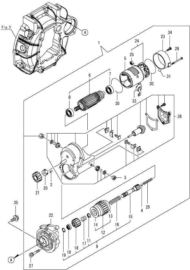
Fig.15. STARTER MOTOR
