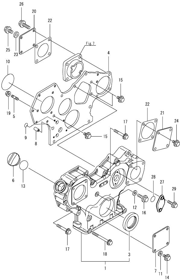
Fig.2. GEAR HOUSING
