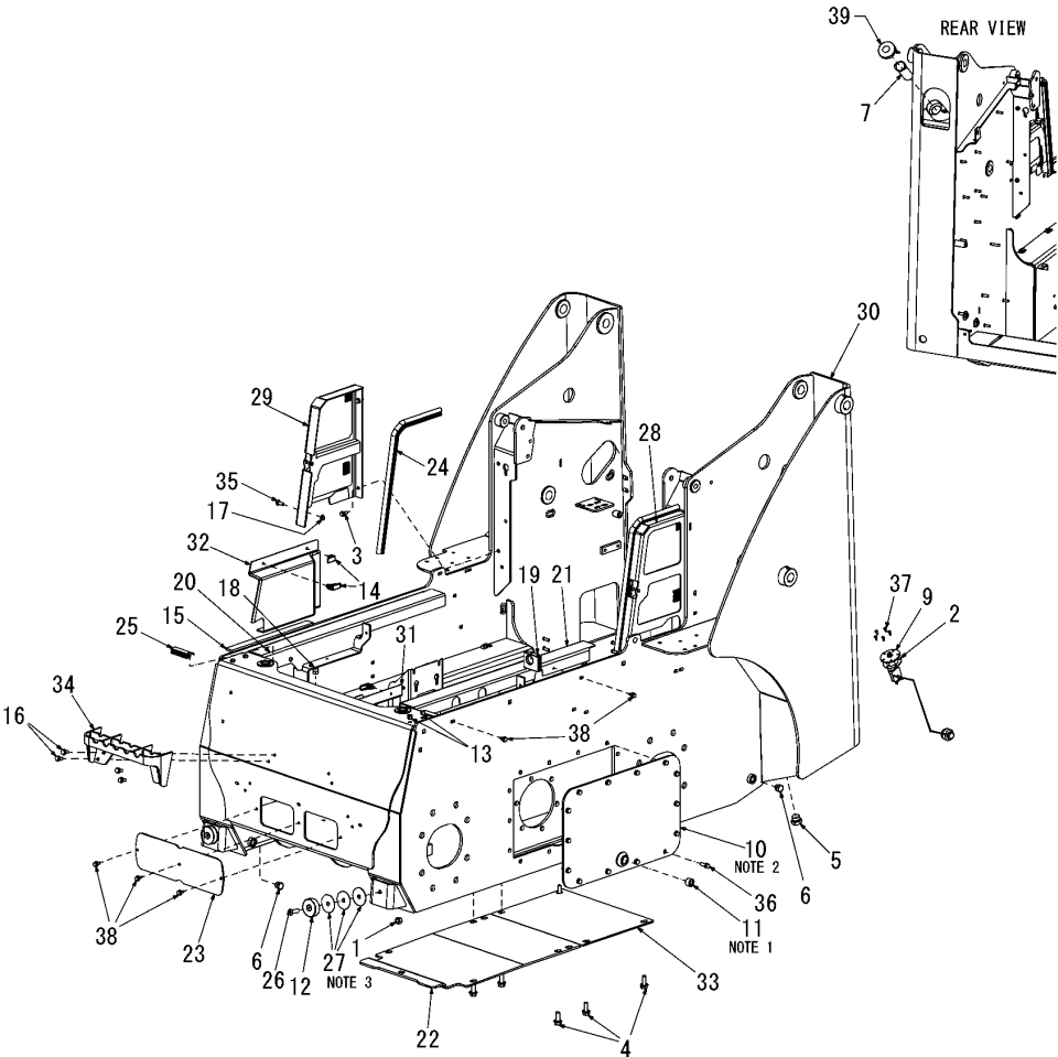
Fig.1. CHASSIS(S190R
