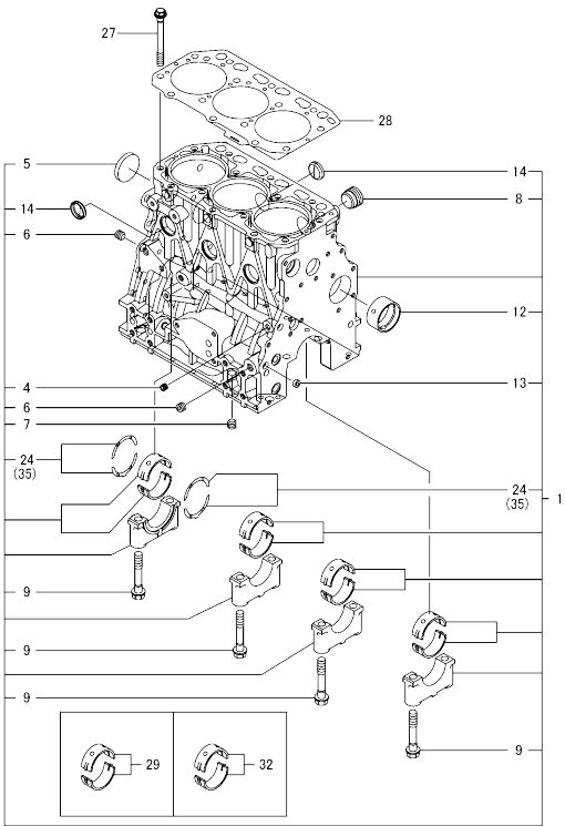
Fig.1. CYLINDER BLOCK
