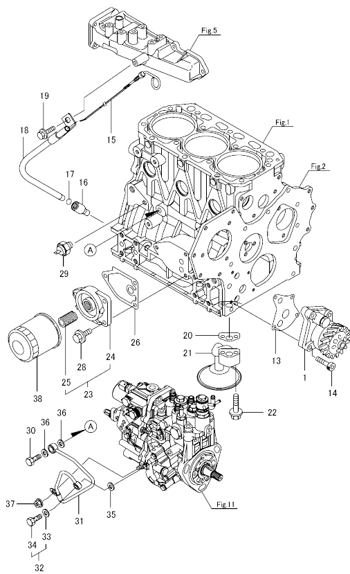
Fig.9. LUB. OIL SYSTEM
