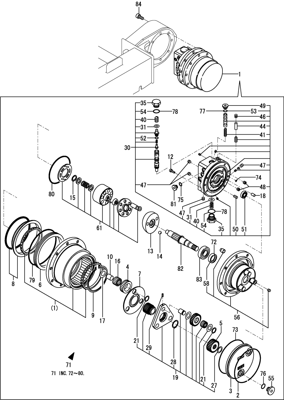
Fig.56. TRAVEL MOTOR
