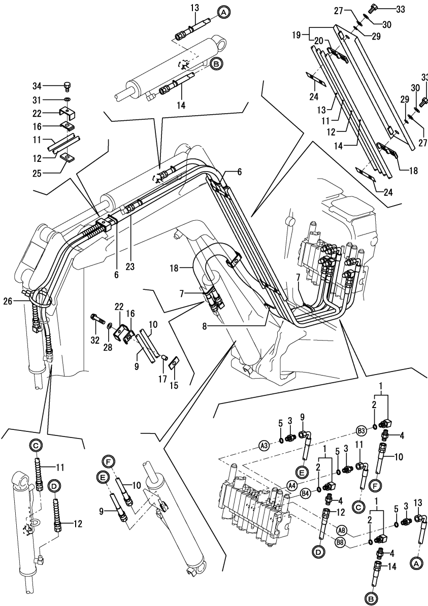
Fig.72. CONTROL VALVE - BOOM
