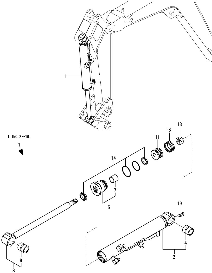
Fig.52. BUCKET CYLINDER
