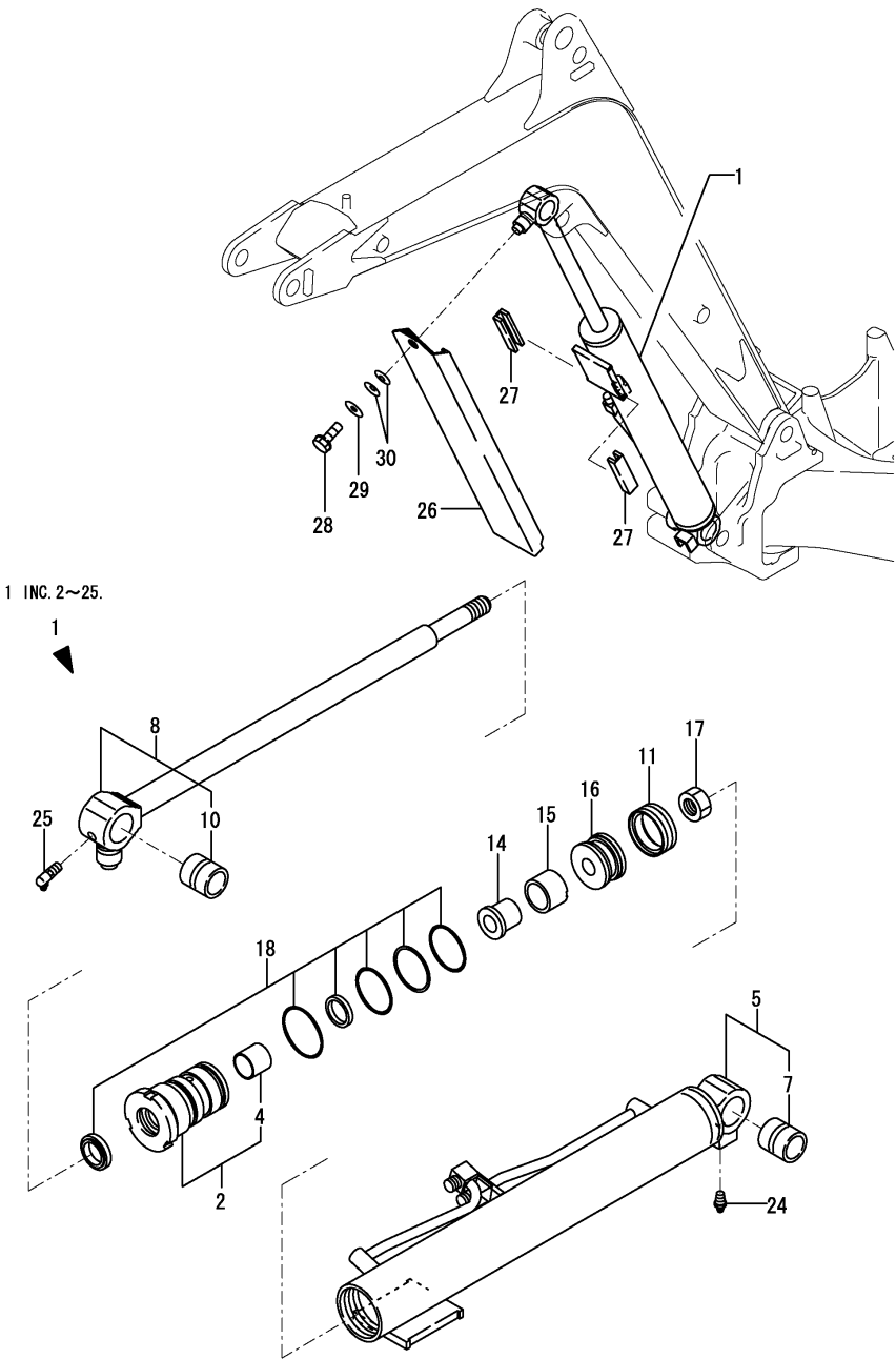
Fig.50. BOOM CYLINDER
