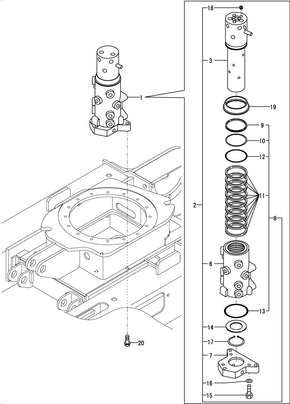
Fig.58. SWIVEL JOINT
