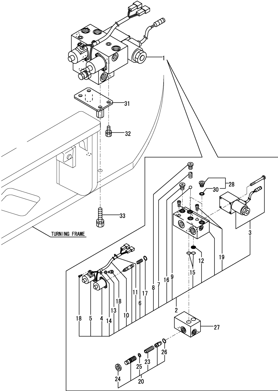
OCS10-M45602 VEHILCE SV100 Fig.66. SOLENOID VALVE
