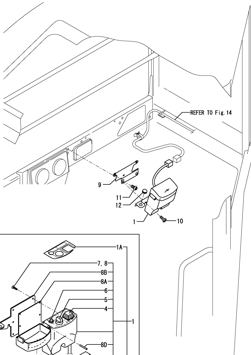
Fig.16. ELECTRIC PART(SWITCH BOX : QUICK COUPLER)
