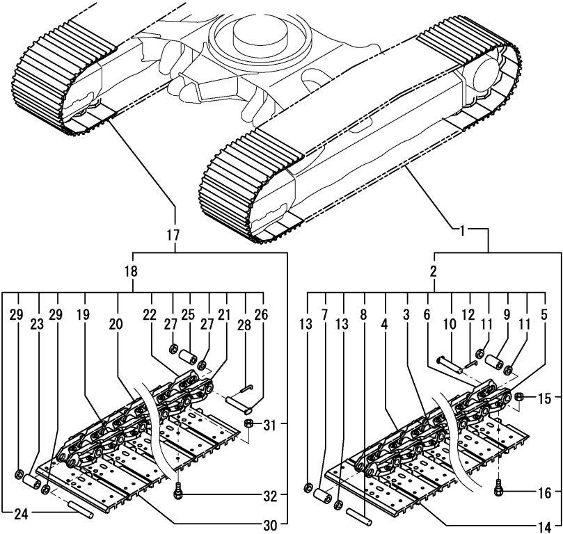
Fig.27. CRAWLER
