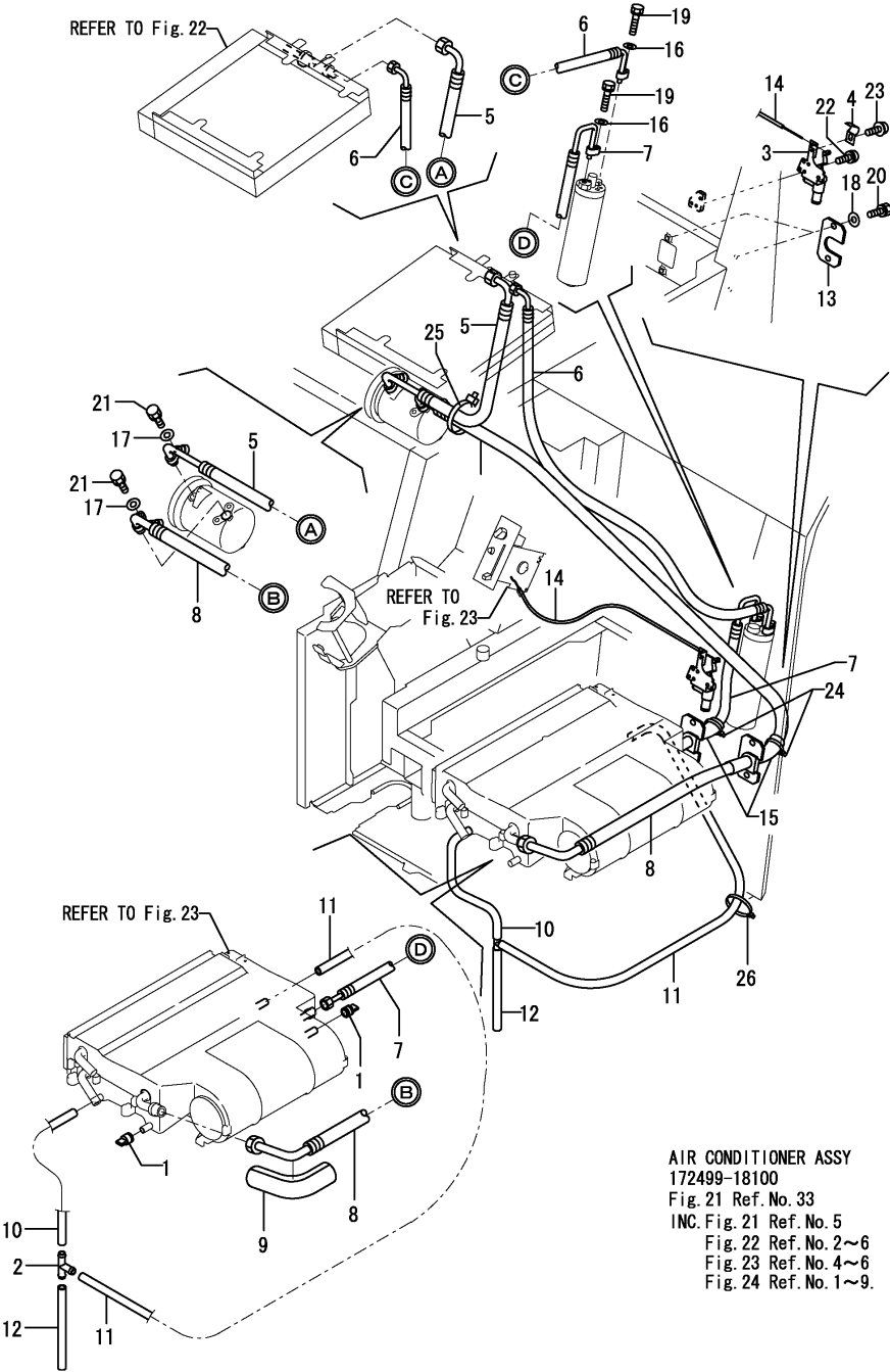
Fig.24. AIR CONDITIONER(PIPING)
