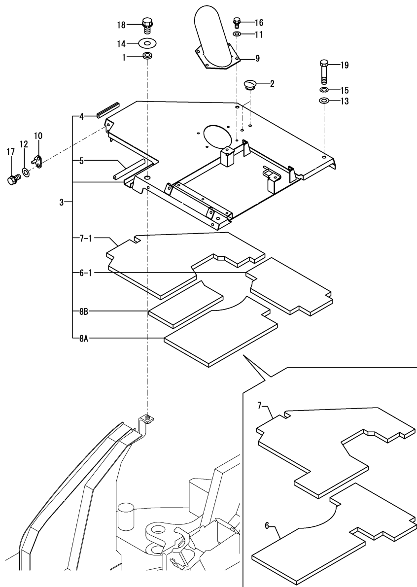
Fig.43. HOOD(UPPER COVER)
