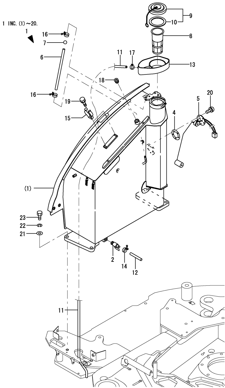
Fig.9. FUEL TANK
