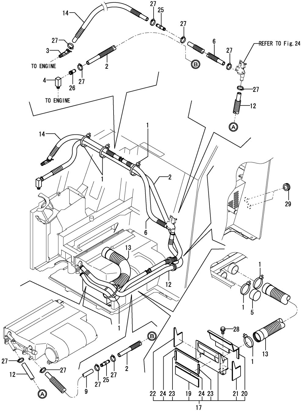
Fig.20. HEATER
