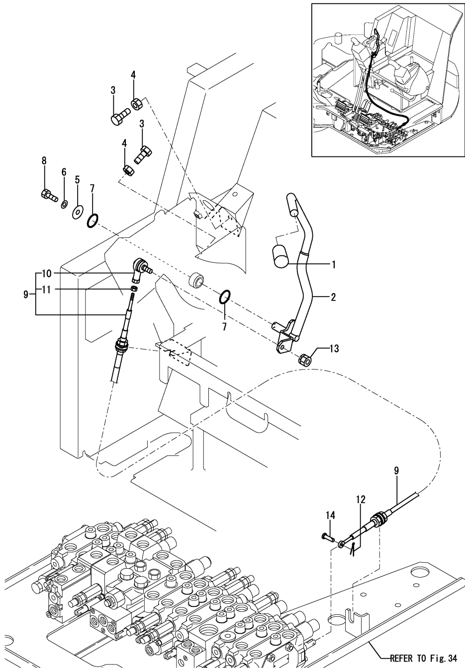
Fig.30. CONTROL EQUIPMENT(BLADE LEVER)
