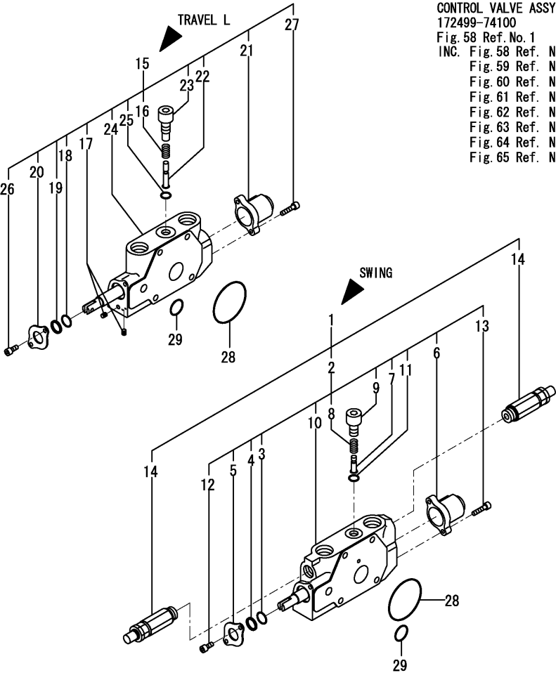
Fig.62. CONTROL VALVE(5/8)
