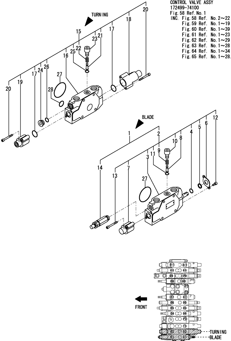
Fig.65. CONTROL VALVE(8/8)
