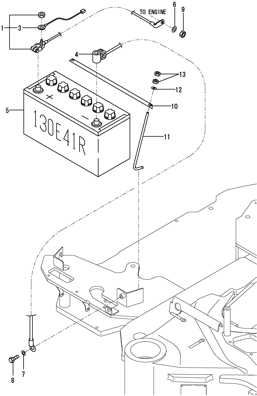
Fig.11. BATTERY
