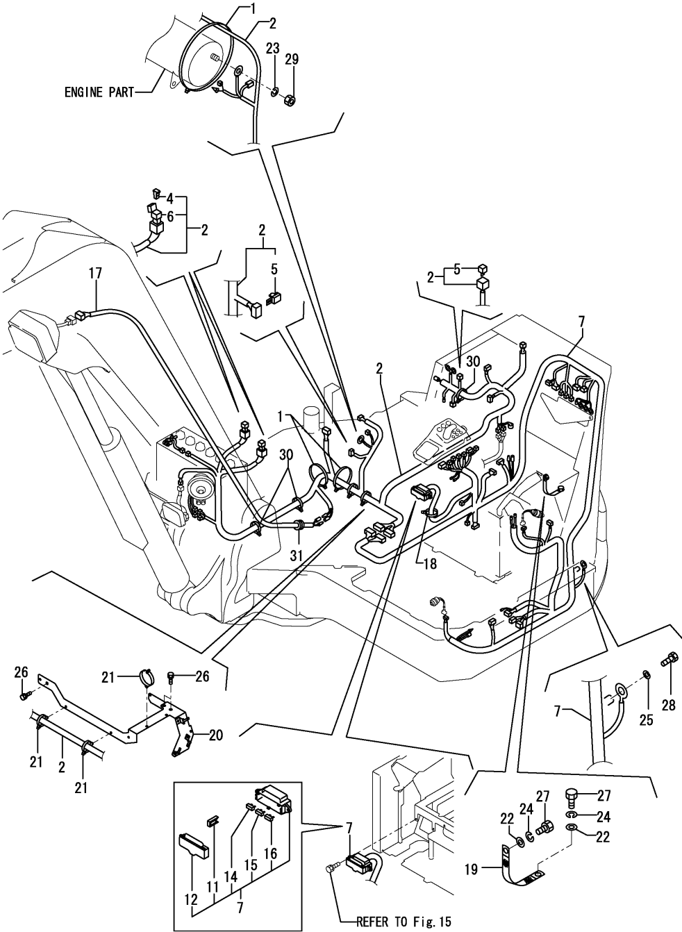
Fig.12. ELECTRIC PART(WIRING)
