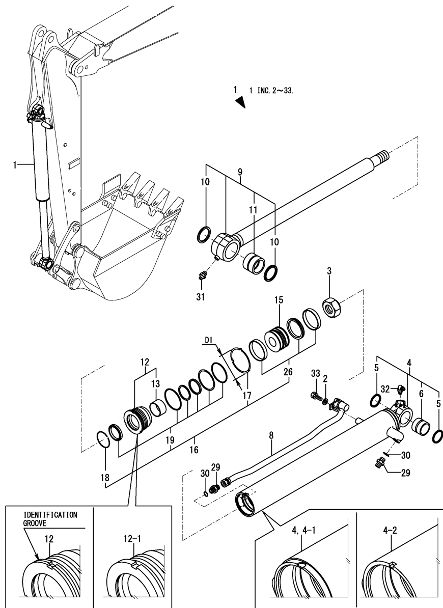
Fig.51. BUCKET CYLINDER
