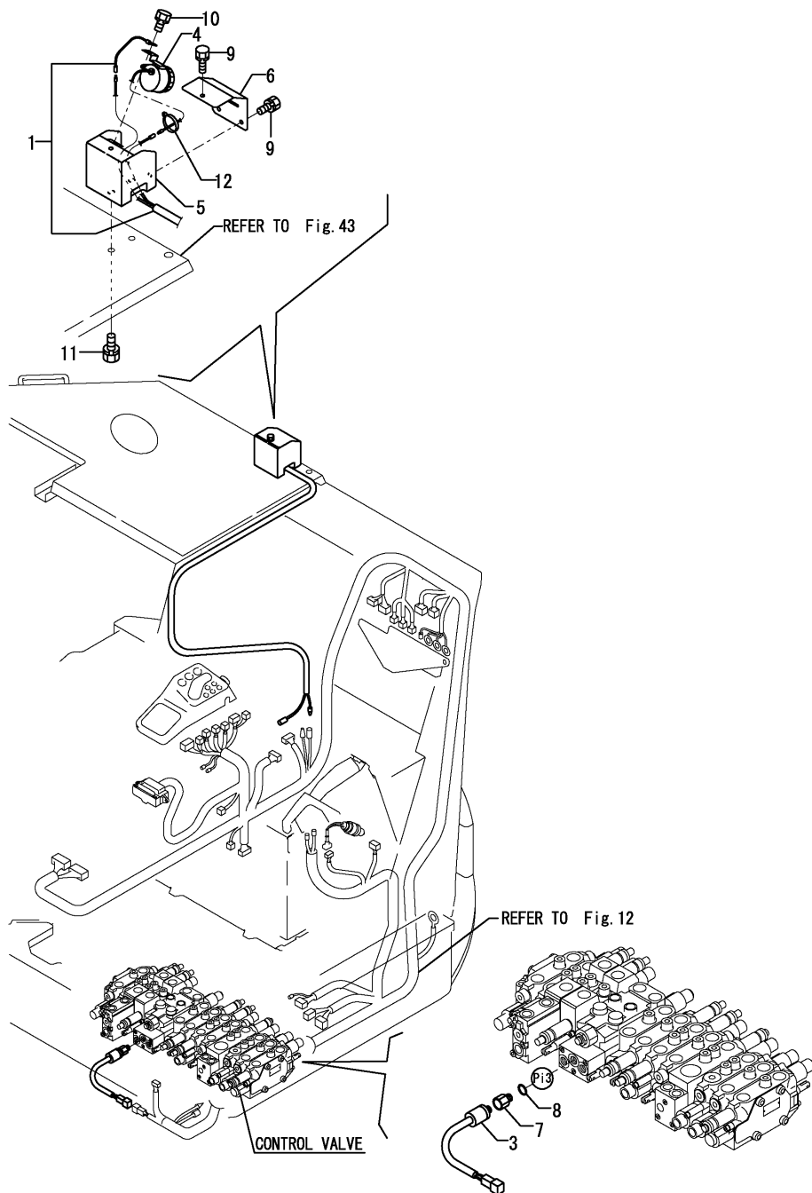
Fig.18. TRAVEL ALARM
