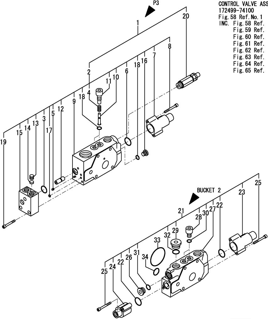
Fig.64. CONTROL VALVE(7/8)
