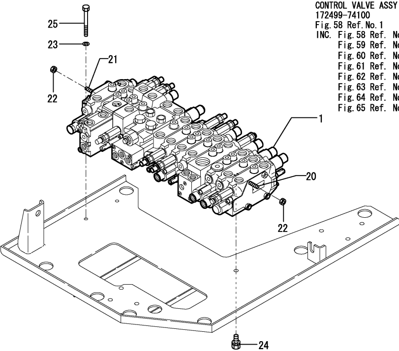
Fig.58. CONTROL VALVE(1/8)
