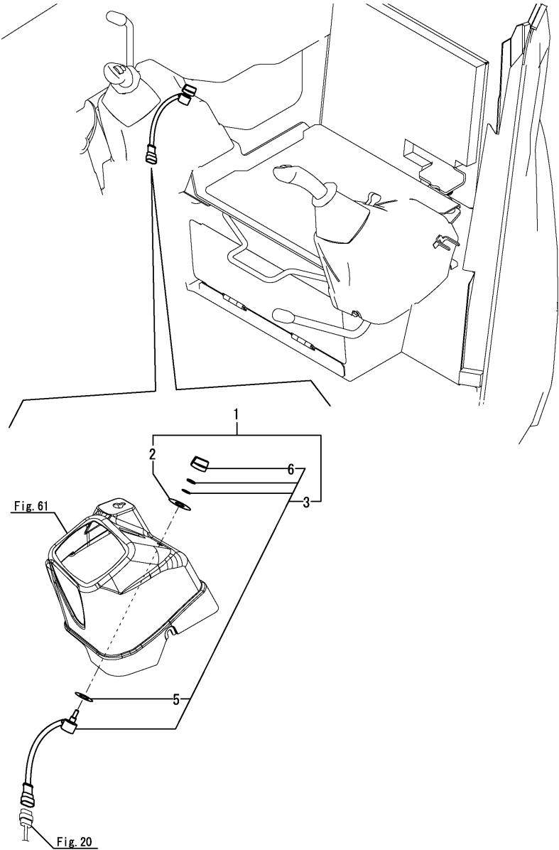
Fig.154. DIAL KIT FOR P.T.O. FLOW RATE ADJUSTMENT(OPTIONAL)
