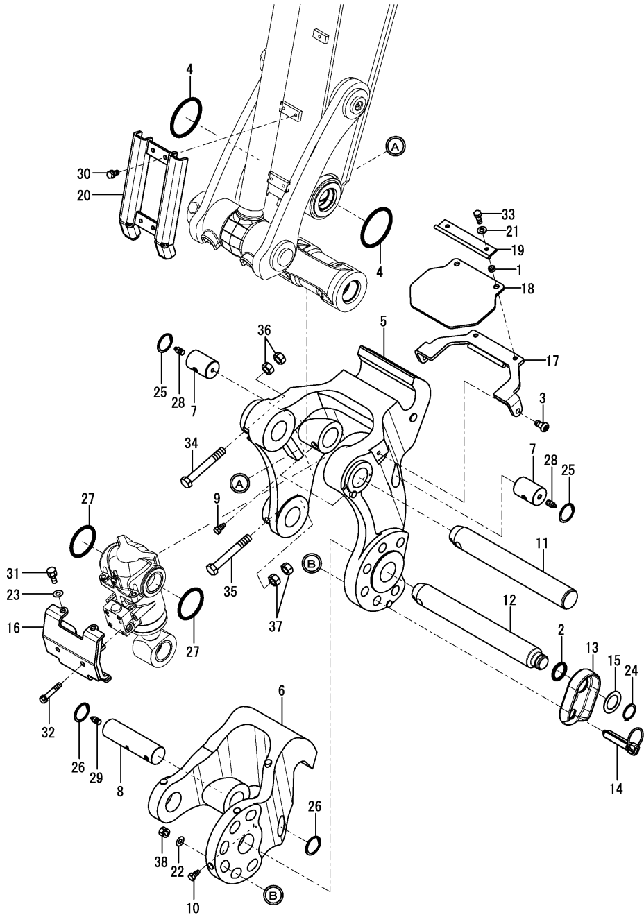
OCK50-M00650 IMPLEMENT Fig.150. QUICK COUPLER
