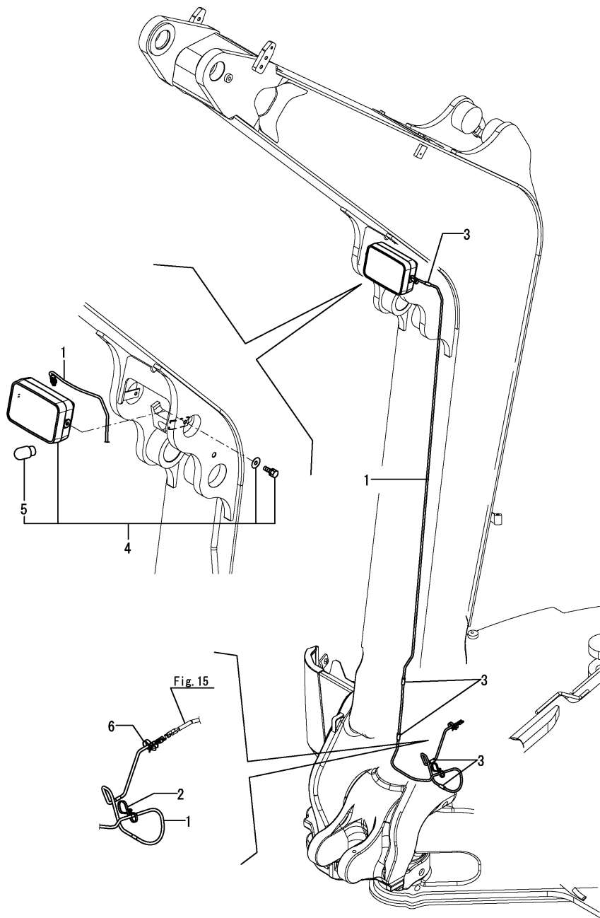
Fig.26. WORK LAMP
