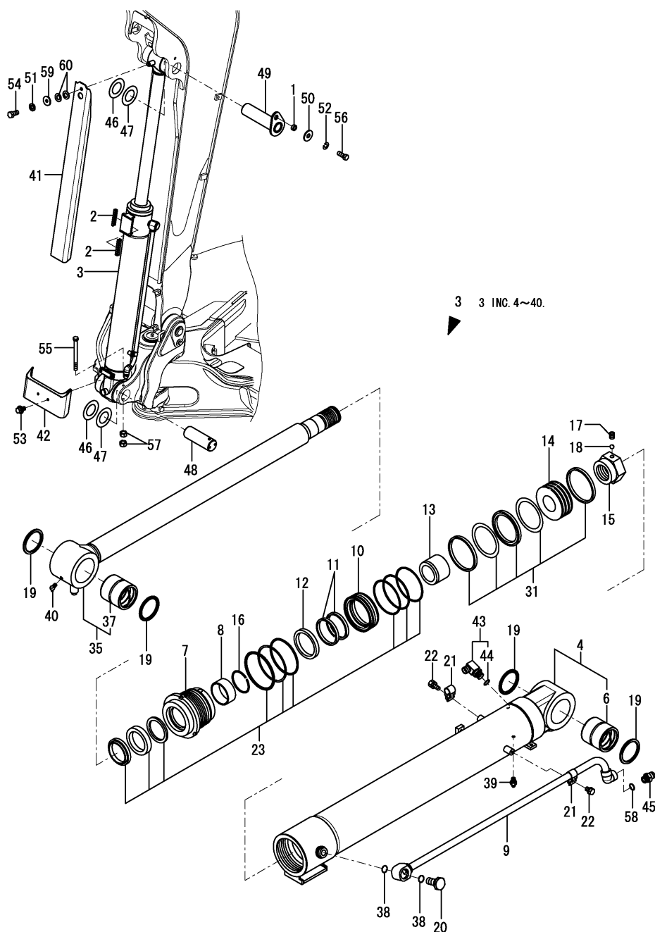
Fig.89. BOOM CYLINDER
