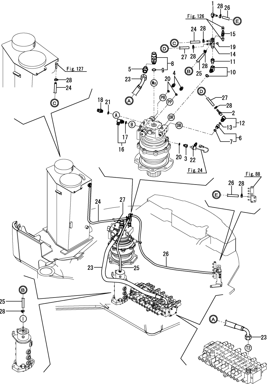
Fig.122. CONTROL VALVE - TURNING MOTOR
