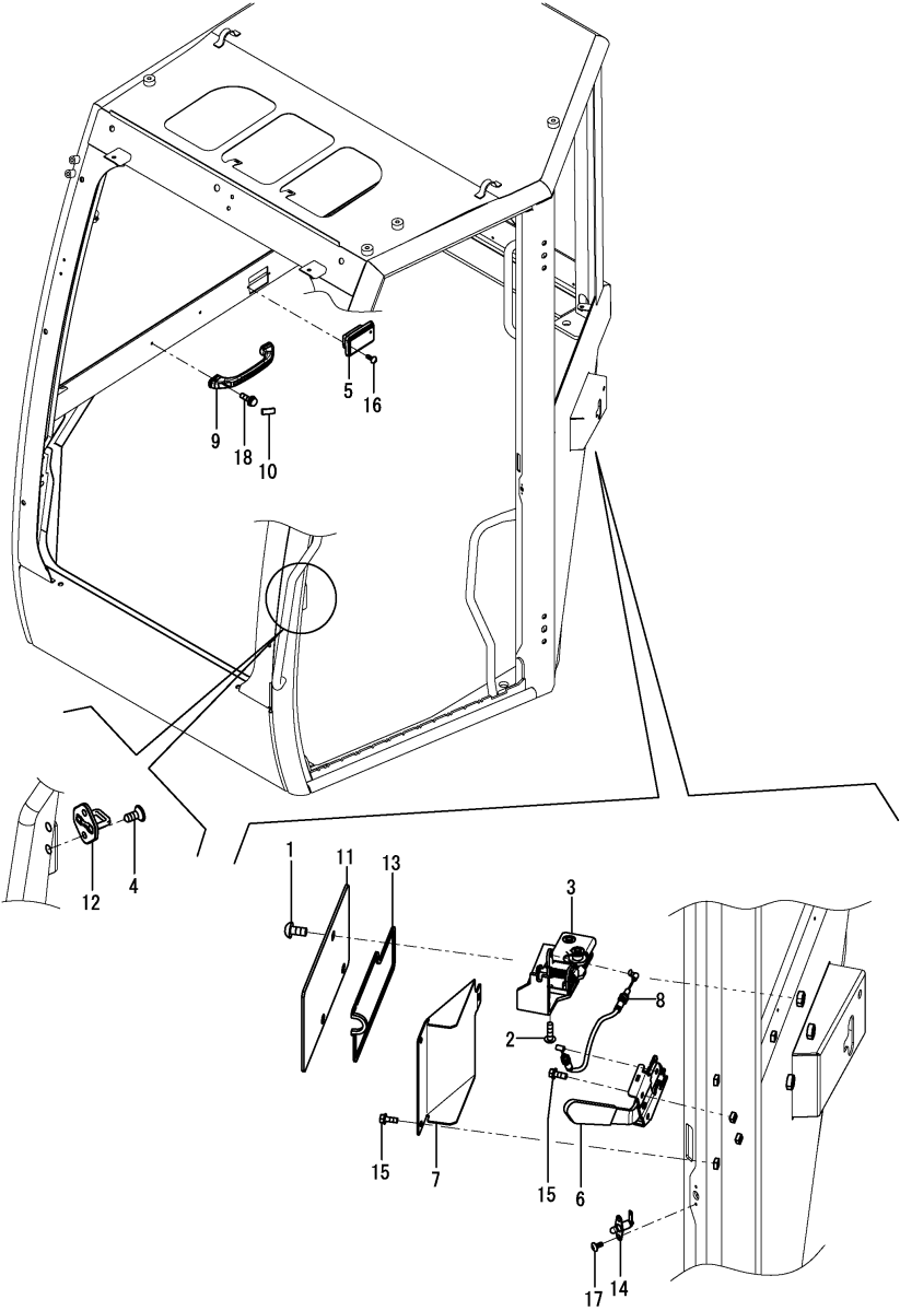
Fig.74. CABIN(ACCESSORY)(2)
