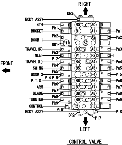
Fig.124. CONTROL VALVE(FITTING)(2)
