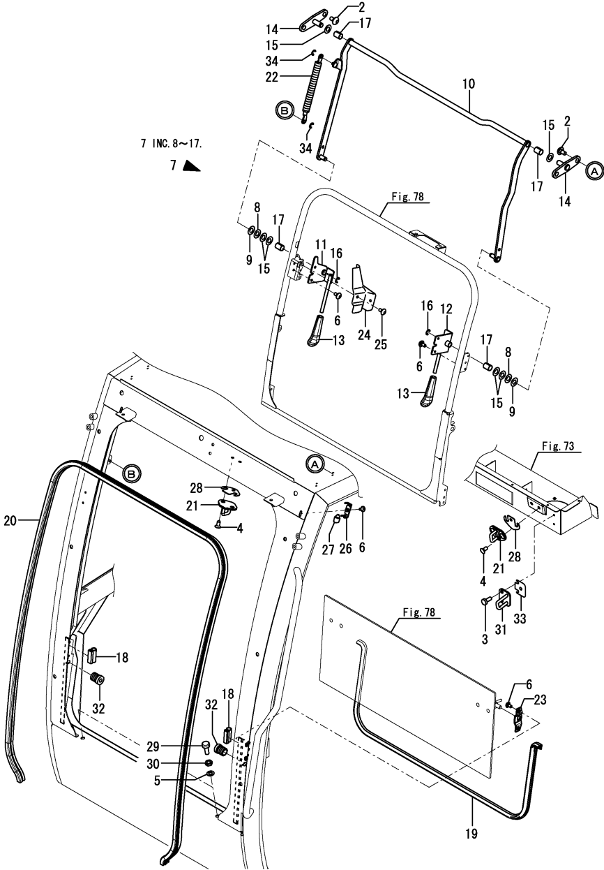
Fig.79. CABIN(FRONT WINDOW)(2)
