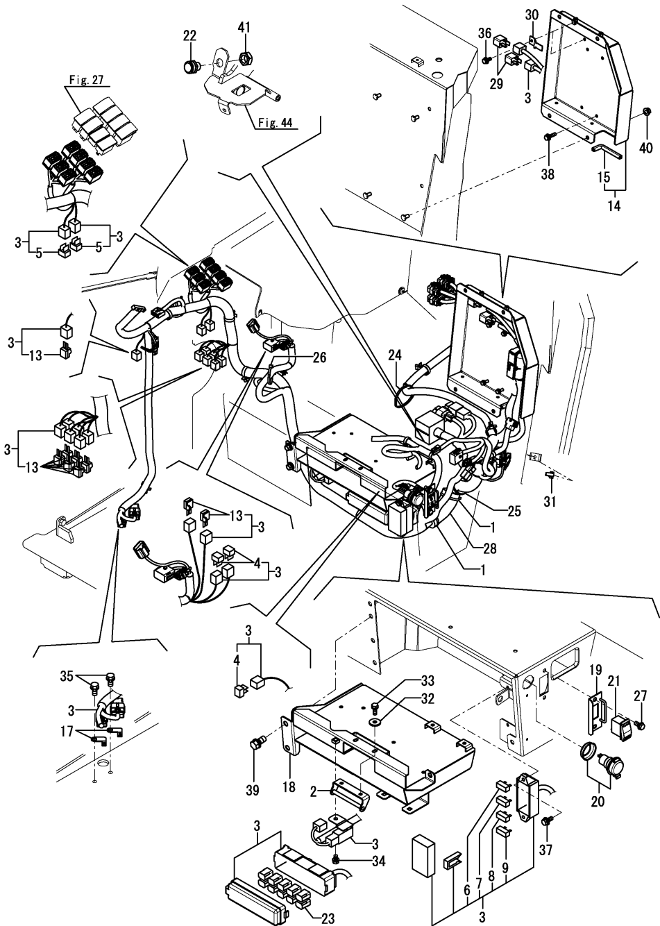
Fig.20. SEAT MOUNT
