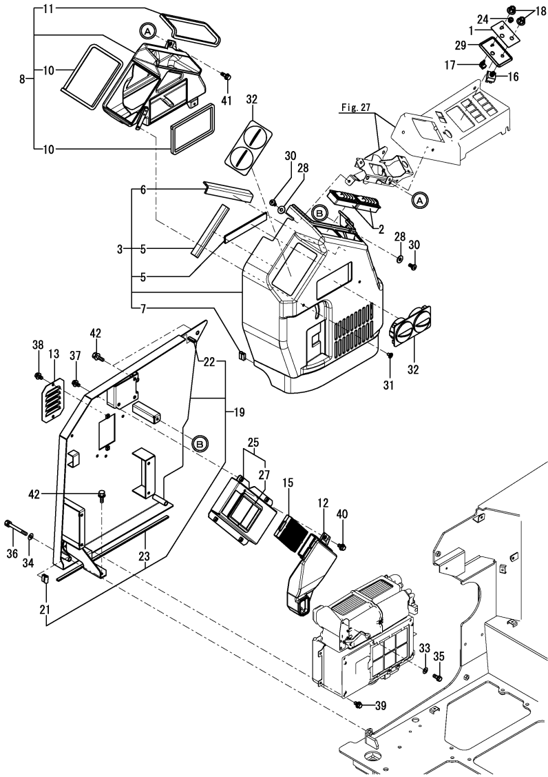
Fig.29. AIR CONDITIONER(CABIN RELATED)
