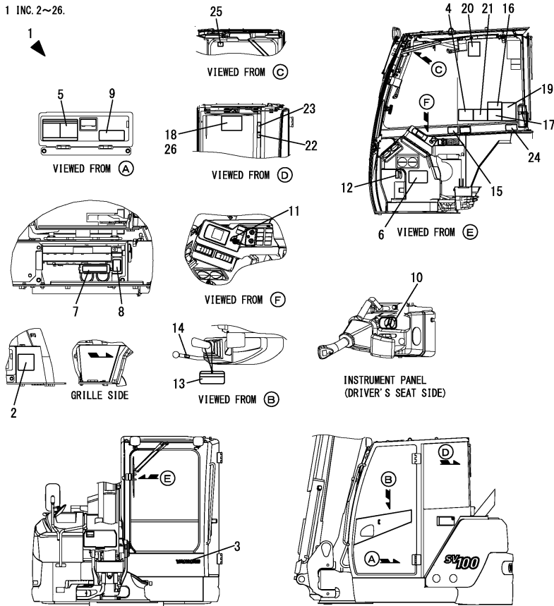
Fig.183. (3A)LABEL(CABIN)(FROM MAF001)
