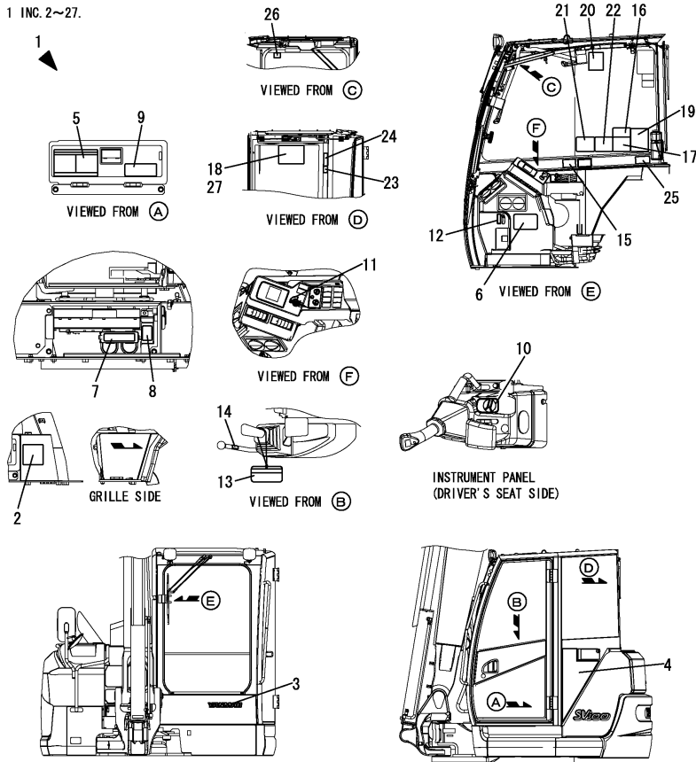
Fig.3. LABEL(CABIN)(TO MAF000)
