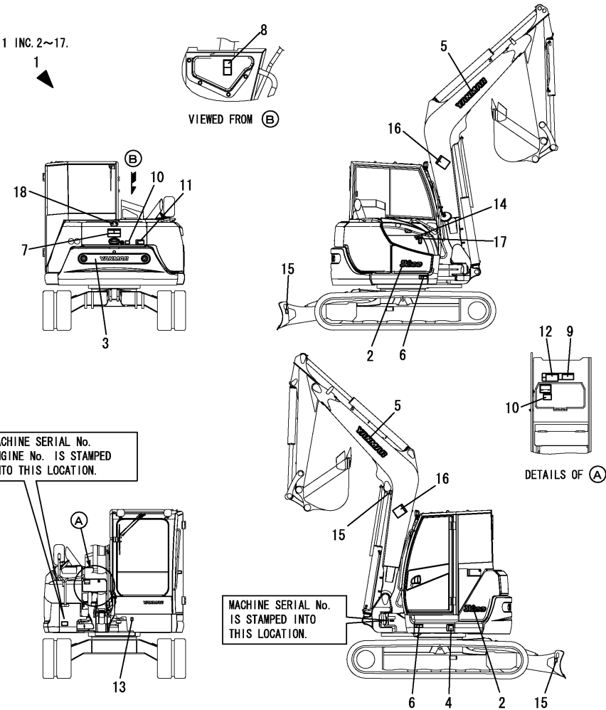
Fig.1. LABEL(EXTERIOR)(TO MAF000)
