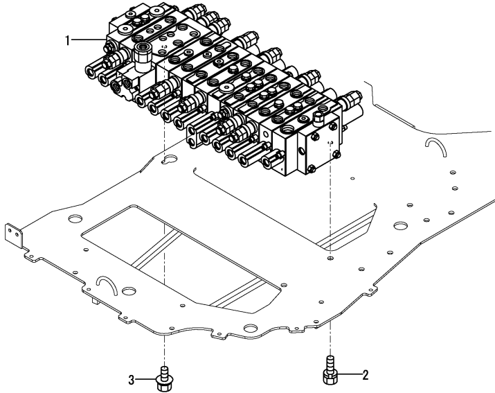
CONTROL VALVE ASSY Fig. 100 Ref. No. 1 INC. Fig. 101~108.
