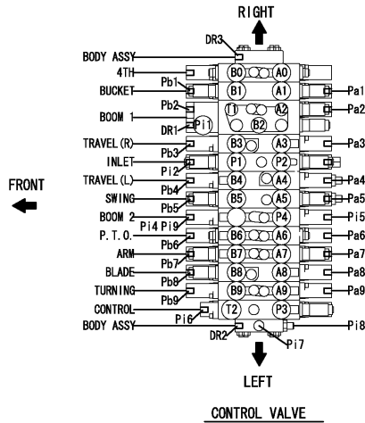
Fig.123. CONTROL VALVE(FITTING)(1)
