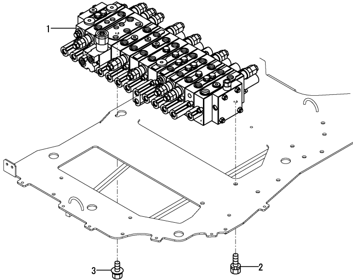
CONTROL VALVE ASSY Fig. 171 Ref. No. 1 INC. Fig. 172~179.
