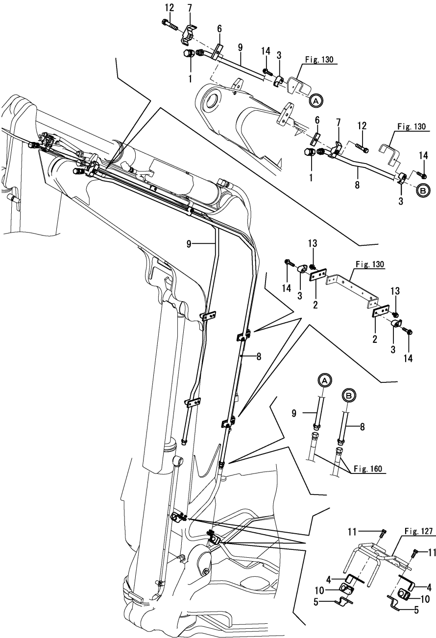
Fig.161. P.T.O. 2 KIT(BOOM END)(OPTIONAL)(7/7)
