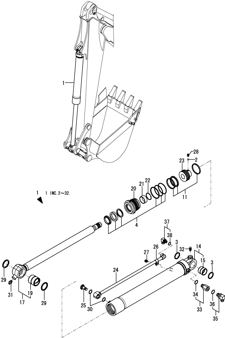
Fig.91. BUCKET CYLINDER
