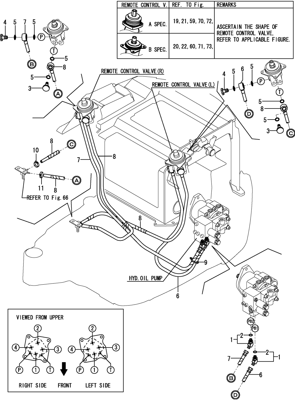
Fig.71. CONTROL PIPING(PUMP - CONTROL VALVE - RETURN : B-SPEC.)
