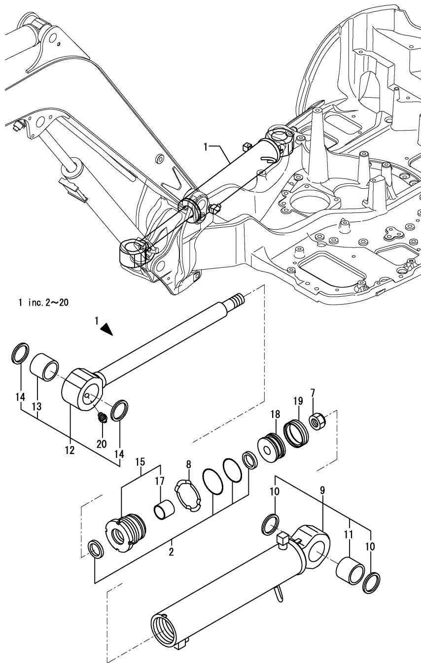
Fig.46. SWING CYLINDER
