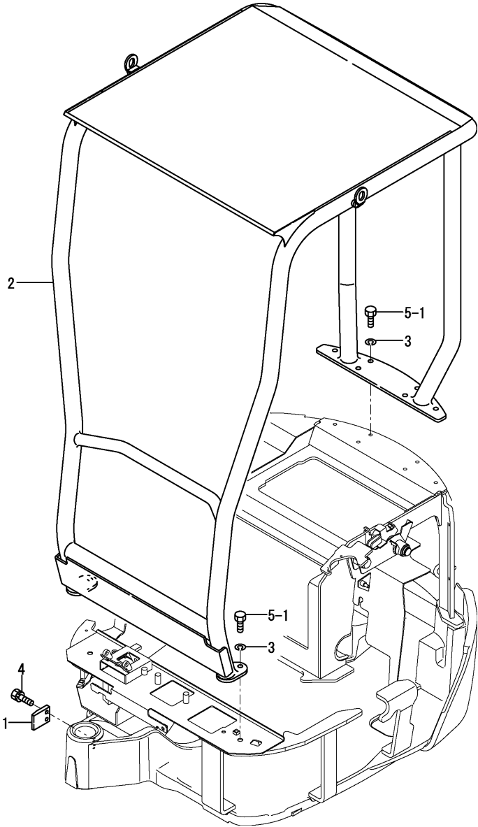
Fig.40. ROPS CANOPY
