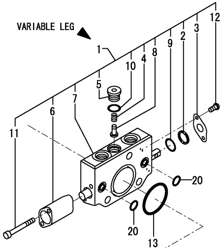
Fig.58. CONTROL VALVE(7/7)
