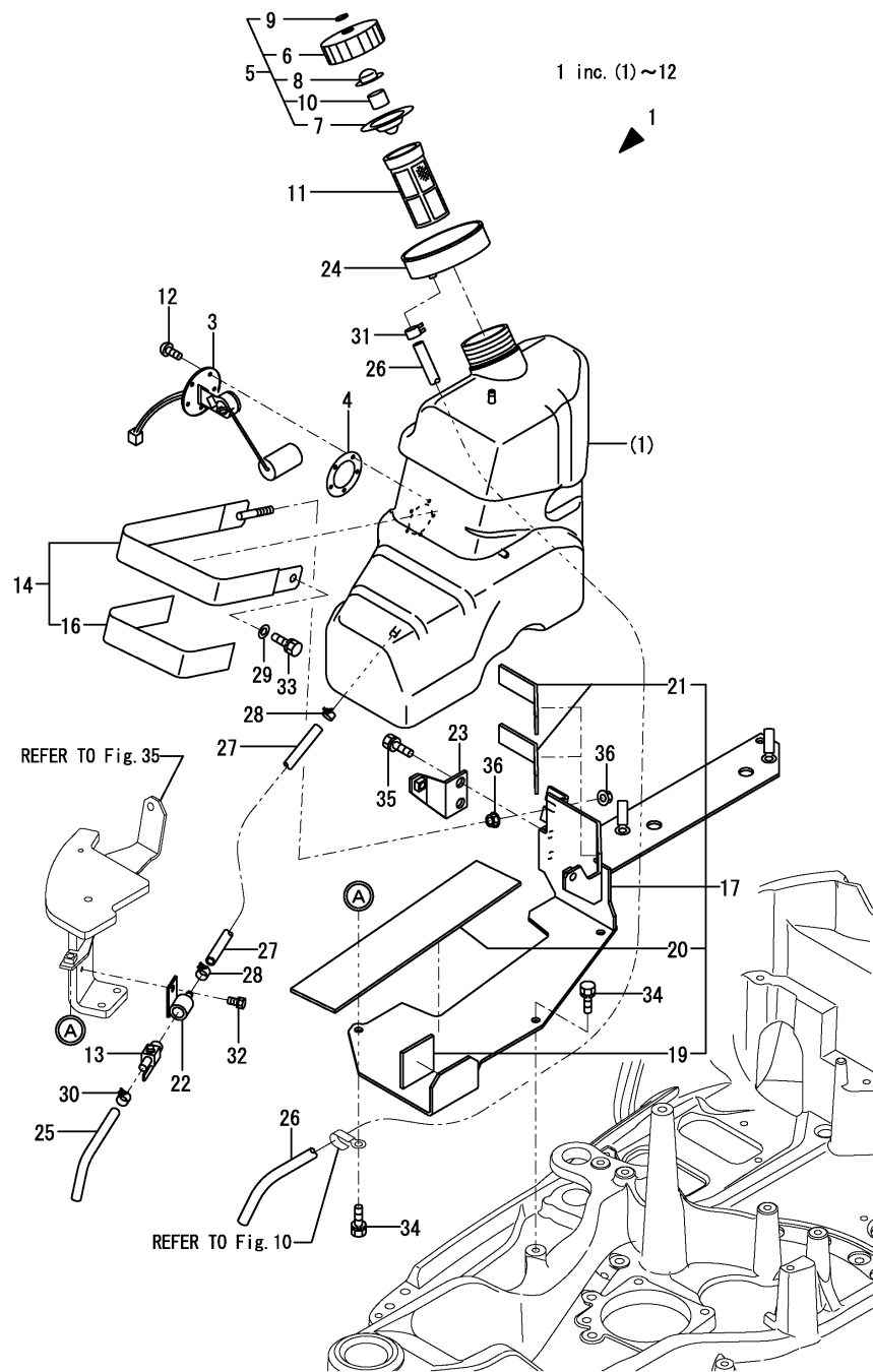
Fig.9. FUEL TANK
