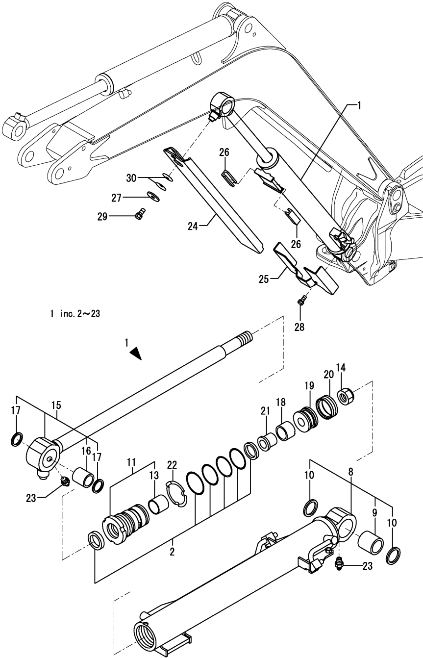
Fig.43. BOOM CYLINDER
