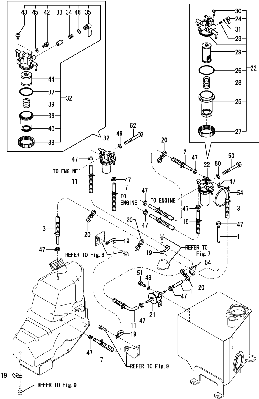
Fig.10. FUEL LINE
