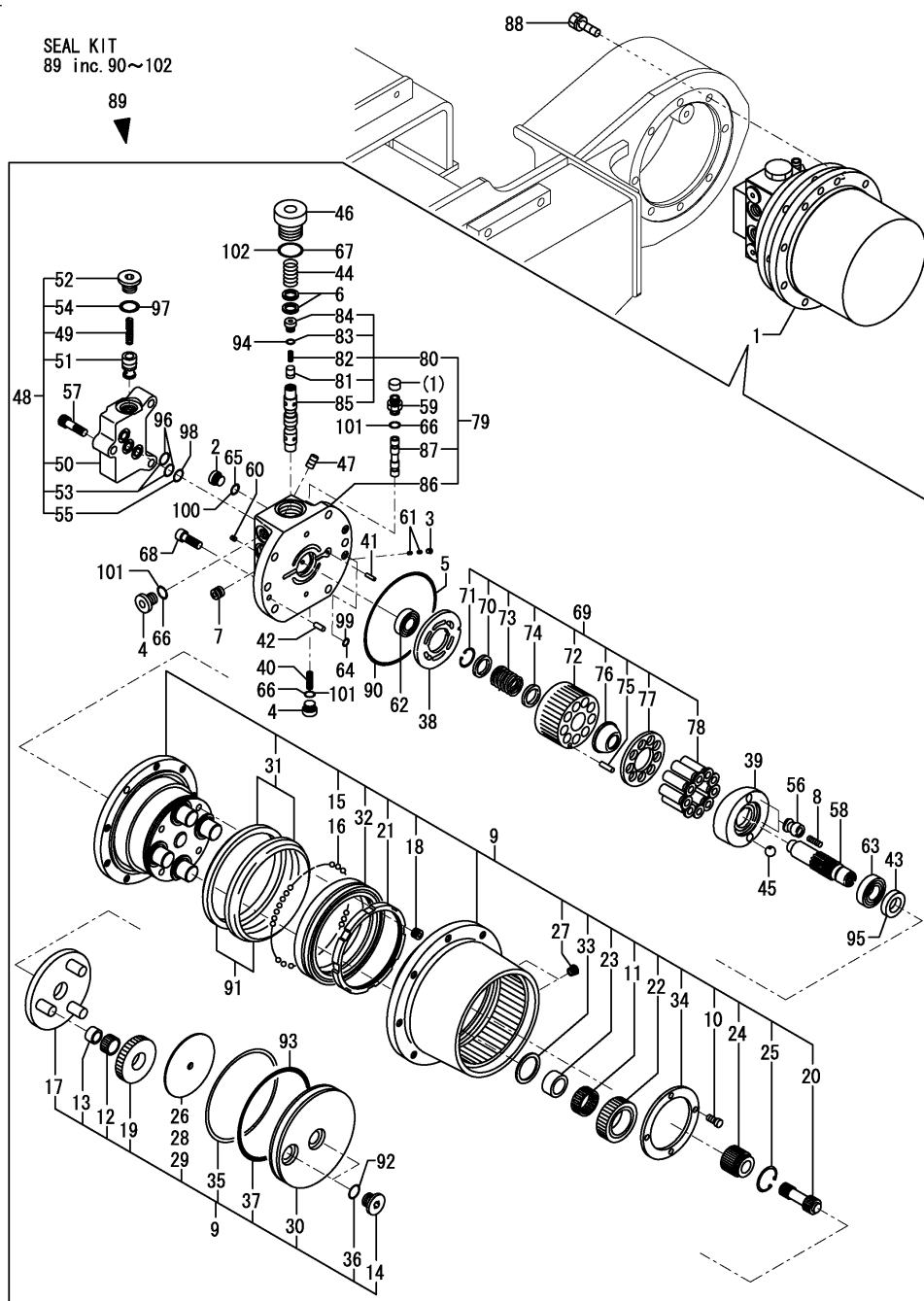
Fig.49. TRAVEL MOTOR
