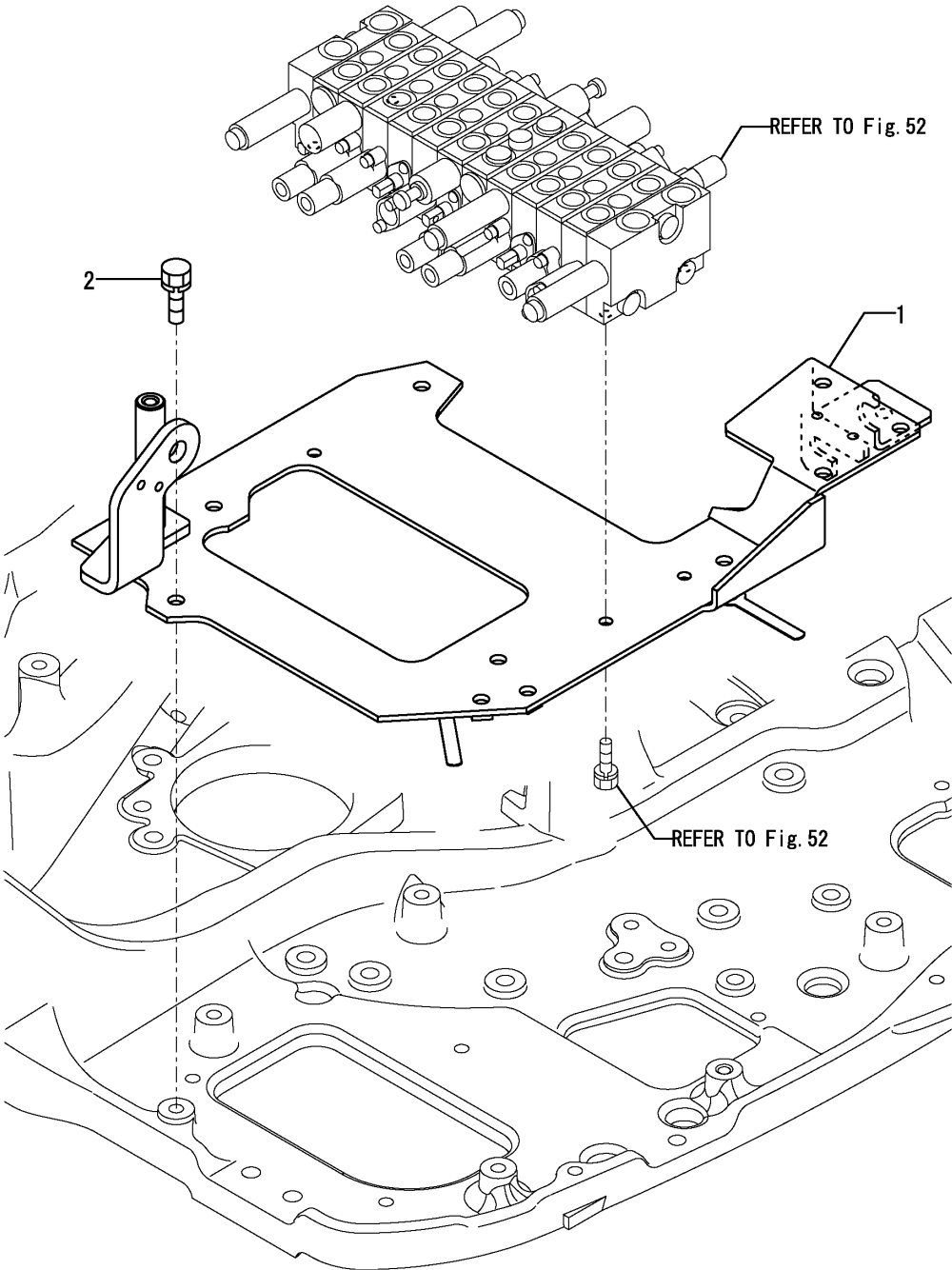
Fig.31. VALVE PLATE
