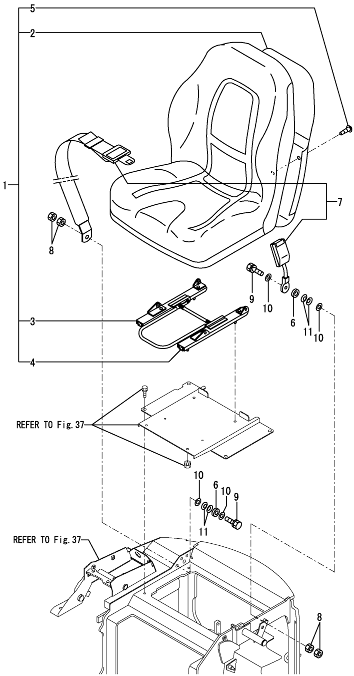
OCS10-M41801 AROUND SEAT Fig.36. SEAT & SEAT BELT
