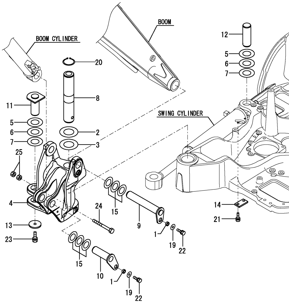
Fig.75. BOOM BRACKET
