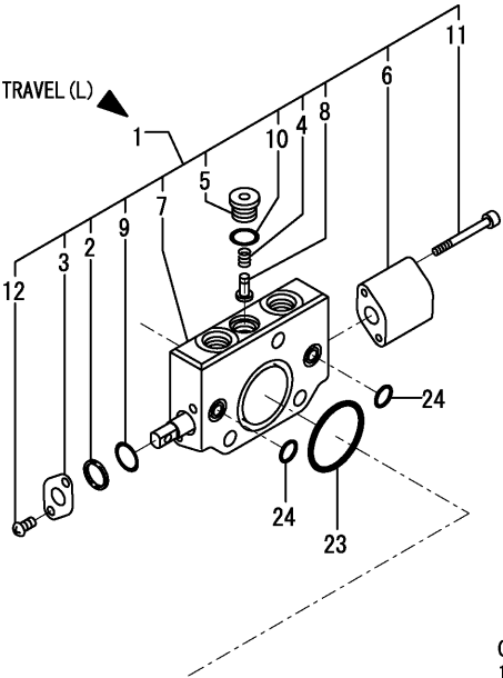
Fig.57. CONTROL VALVE(6/7)
