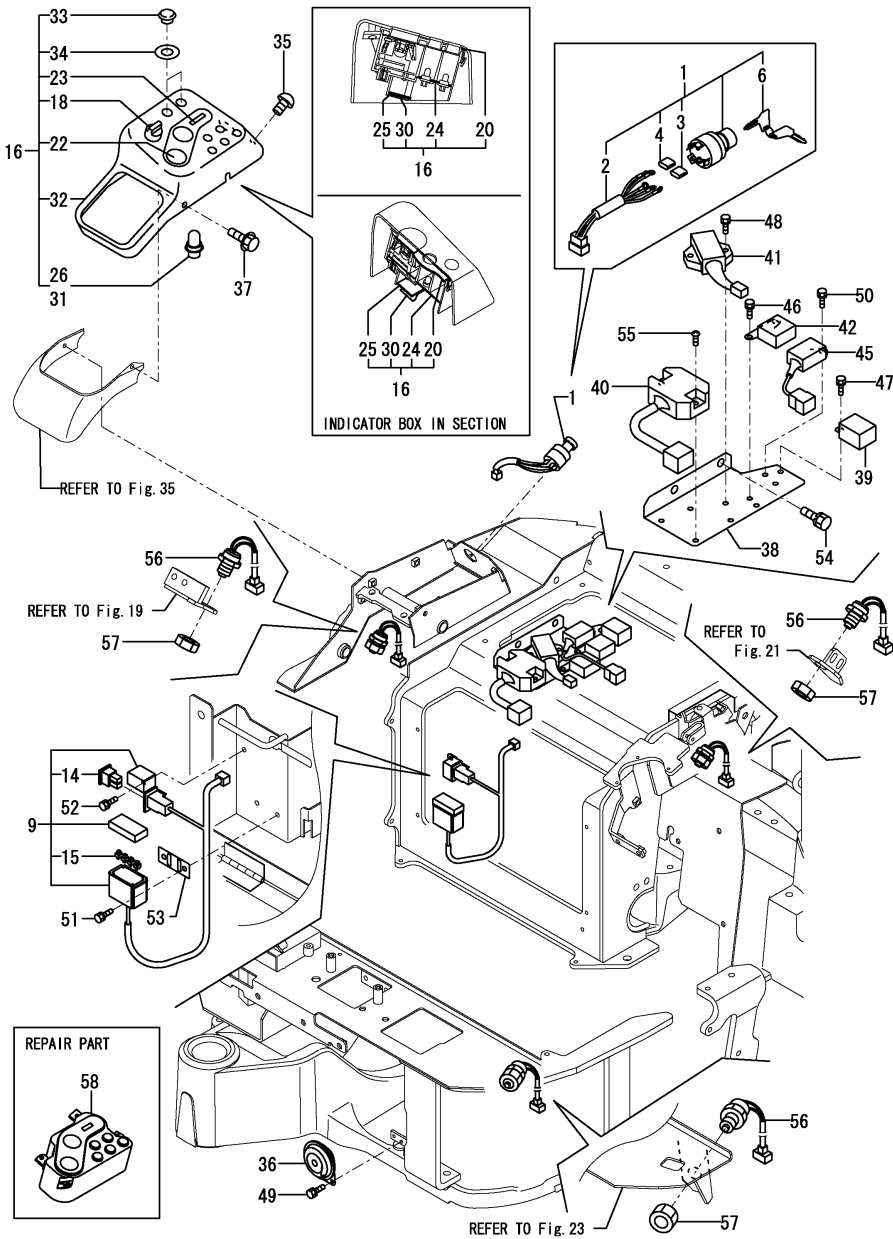
Fig.13. ELECTRIC PART(EQUIPMENT)
