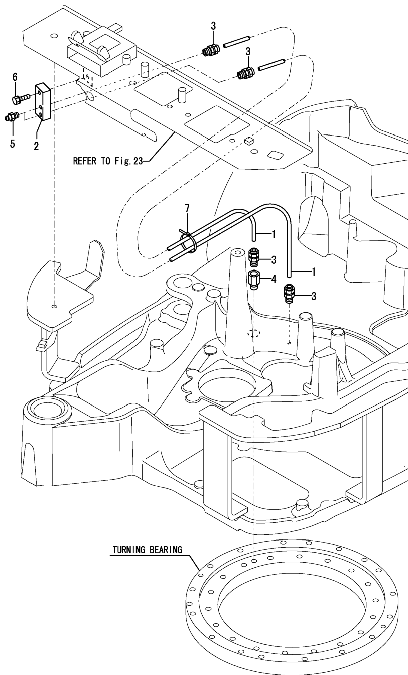
Fig.74. GREASING
