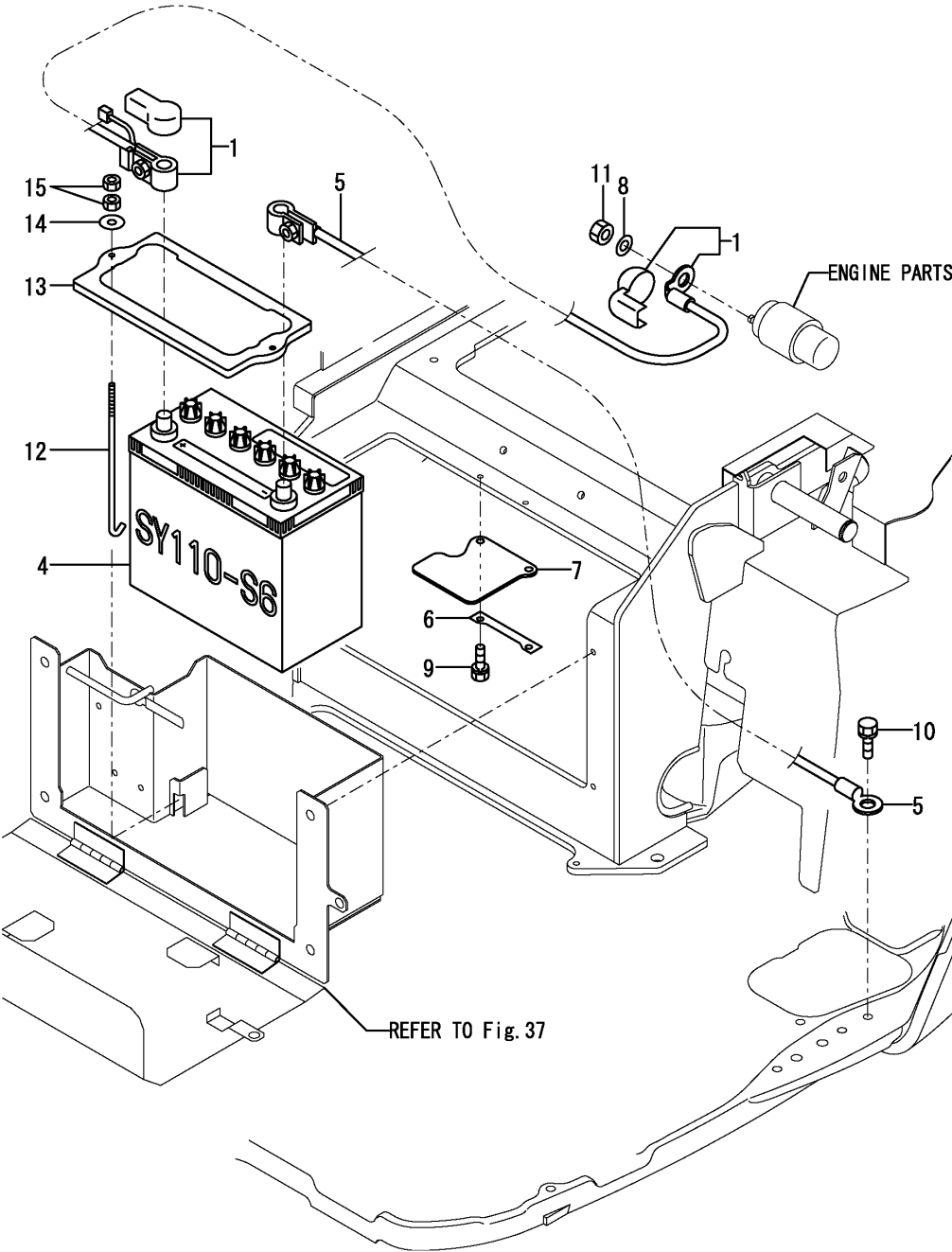
Fig.11. BATTERY
