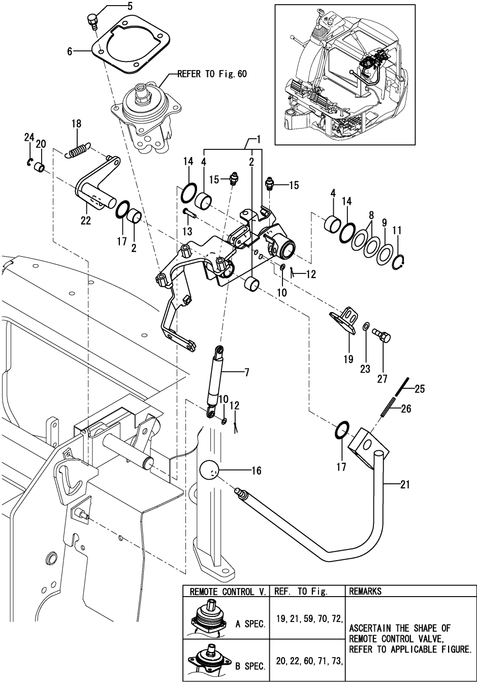
Fig.22. CONTROL EQUIPMENT(LOCK LEVER & STAND: LEFT)(B-SPEC.)
