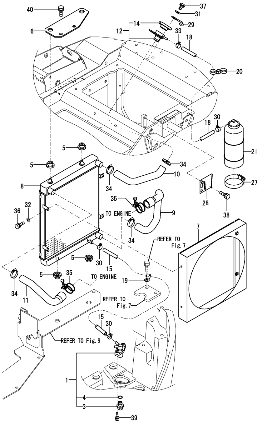
OCS10-M41801 ENGINE RELATED Fig.8. RADIATOR & MOUNT
