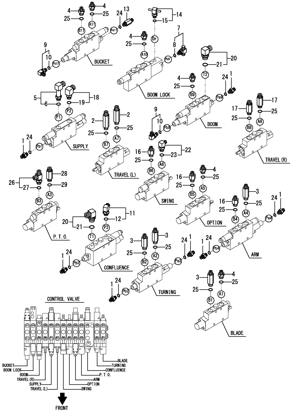
Fig.85. CONTROL VALVE(FITTING)
