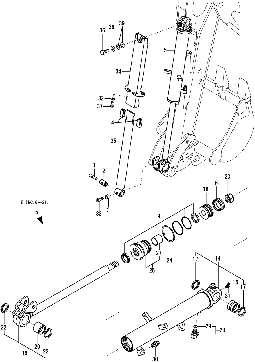
Fig.58. BUCKET CYLINDER
