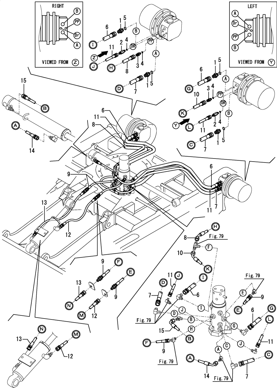
Fig.78. TRAVEL FRAME
