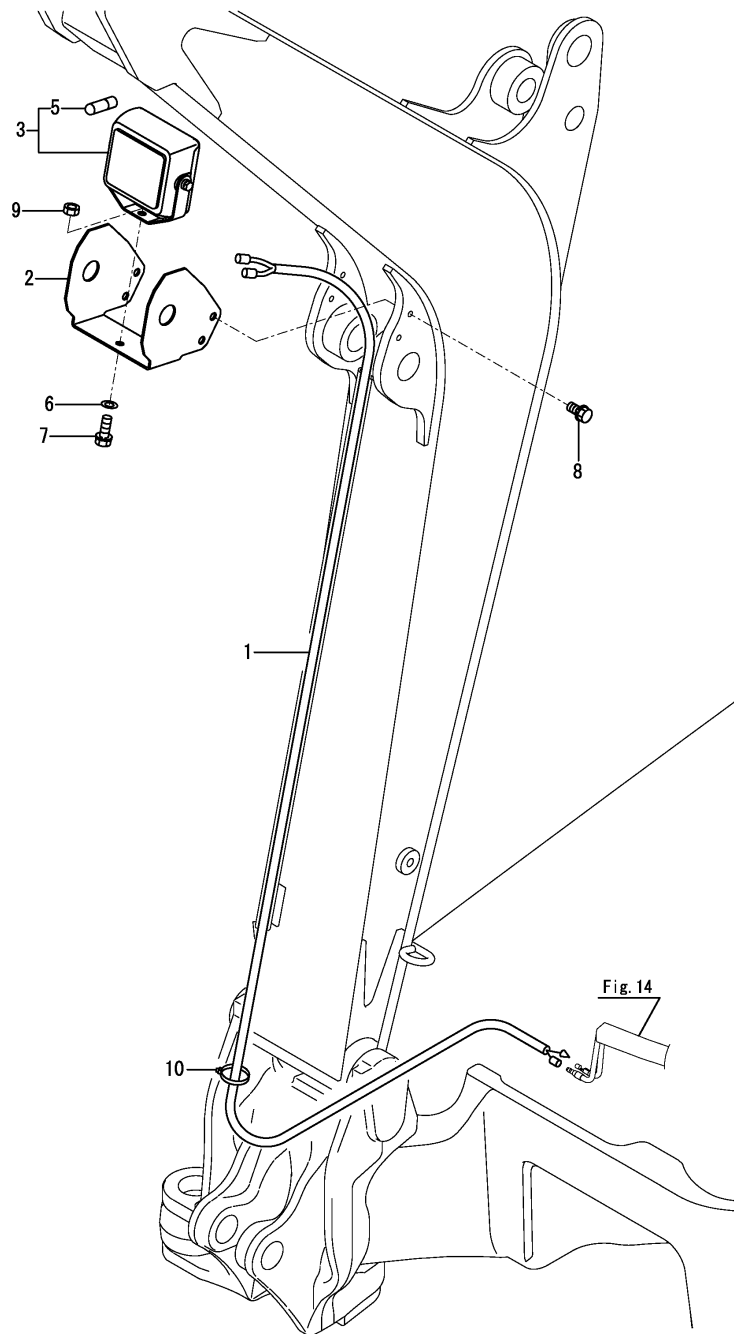
Fig.21. WORK LAMP
