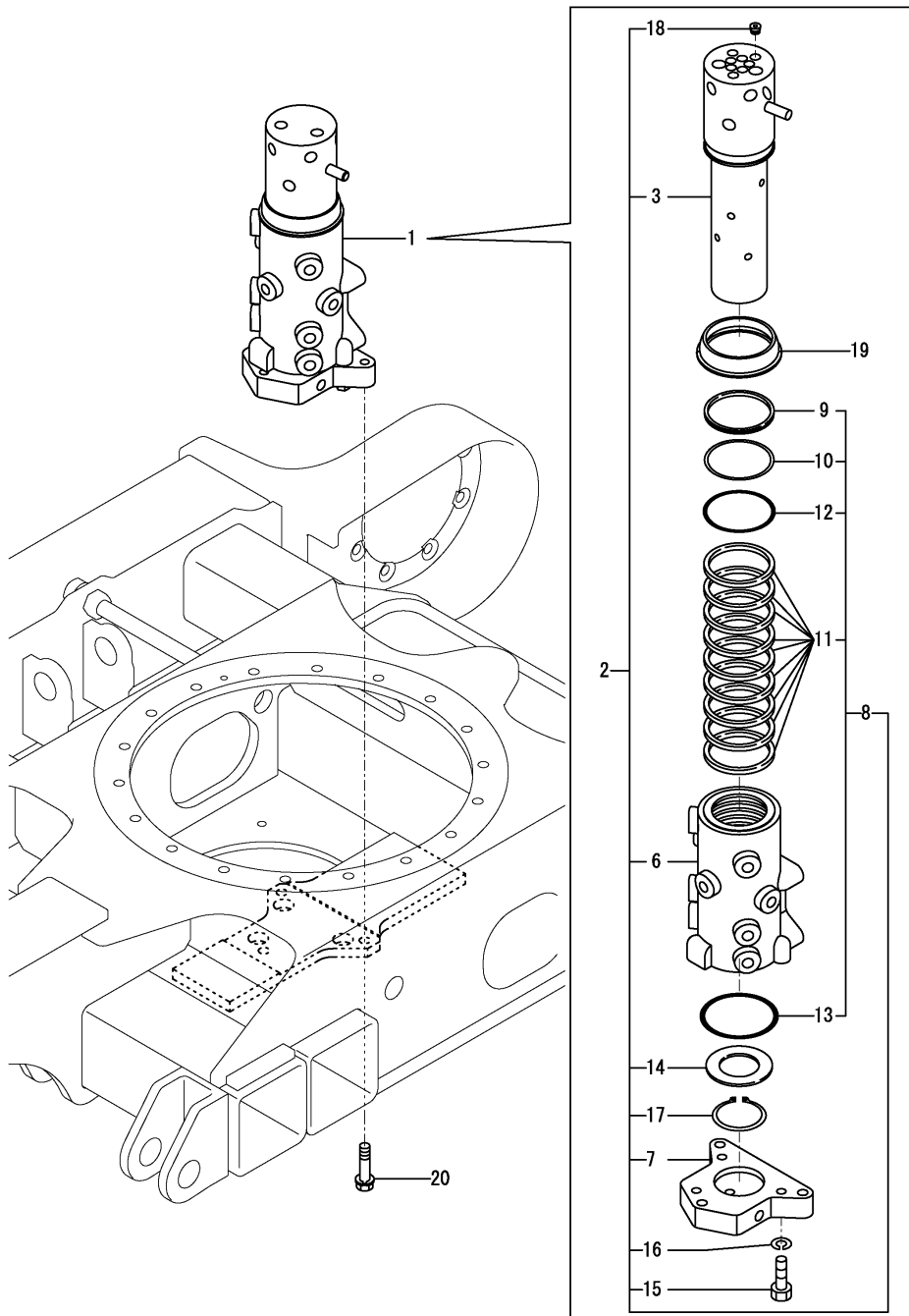
Fig.64. SWIVEL JOINT
