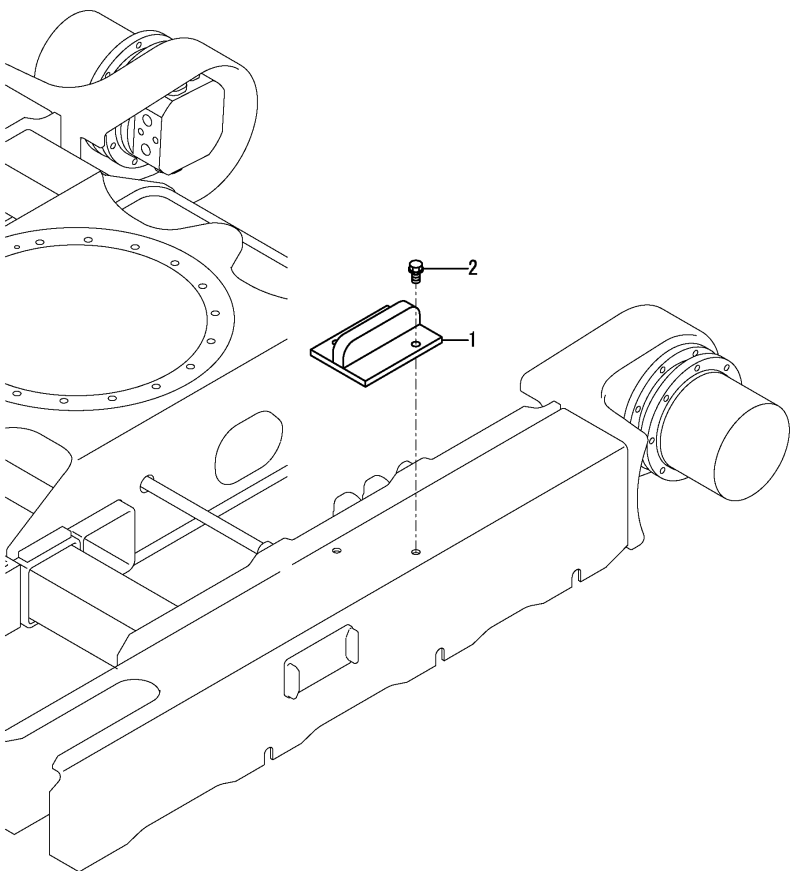
Fig.26. SHOE SLIDE PLATE
