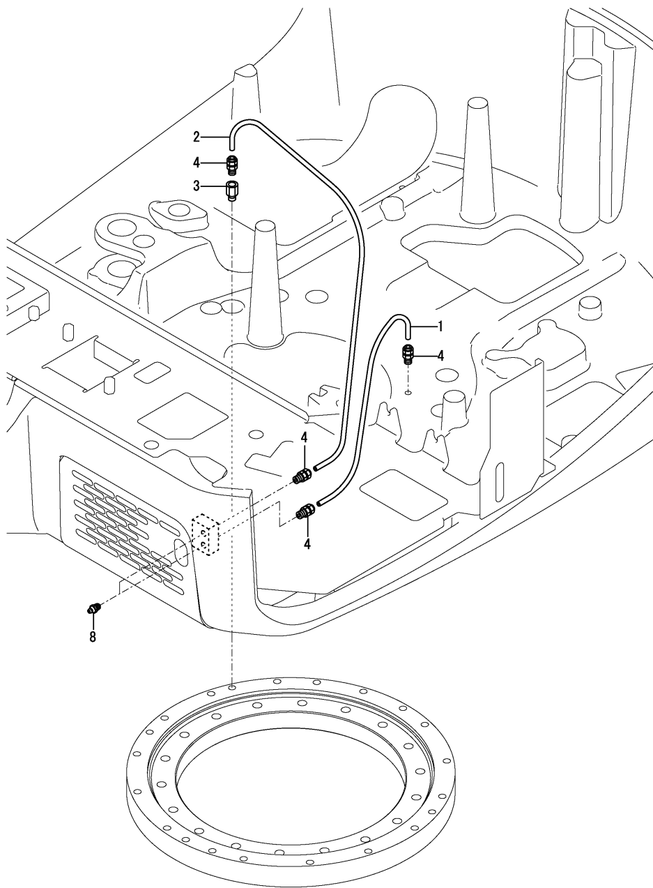
Fig.89. GREASING
