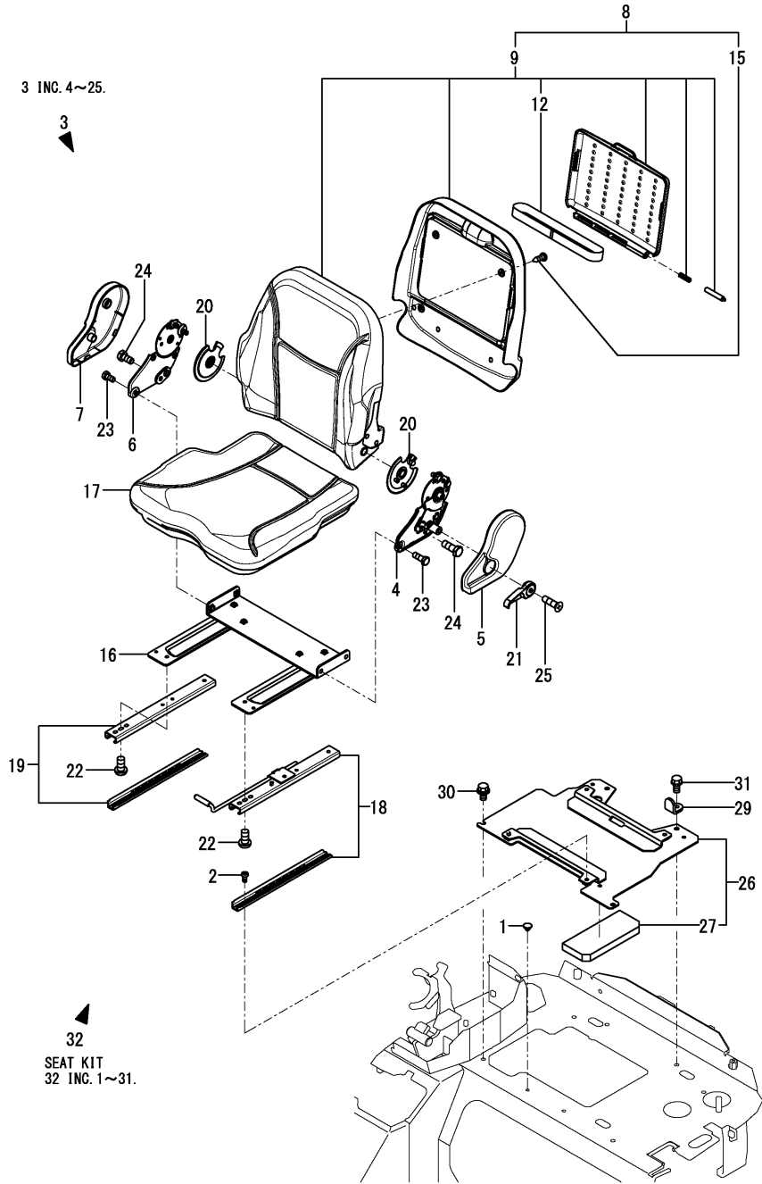
Fig.98. (49A)SEAT(FROM MAF183)
