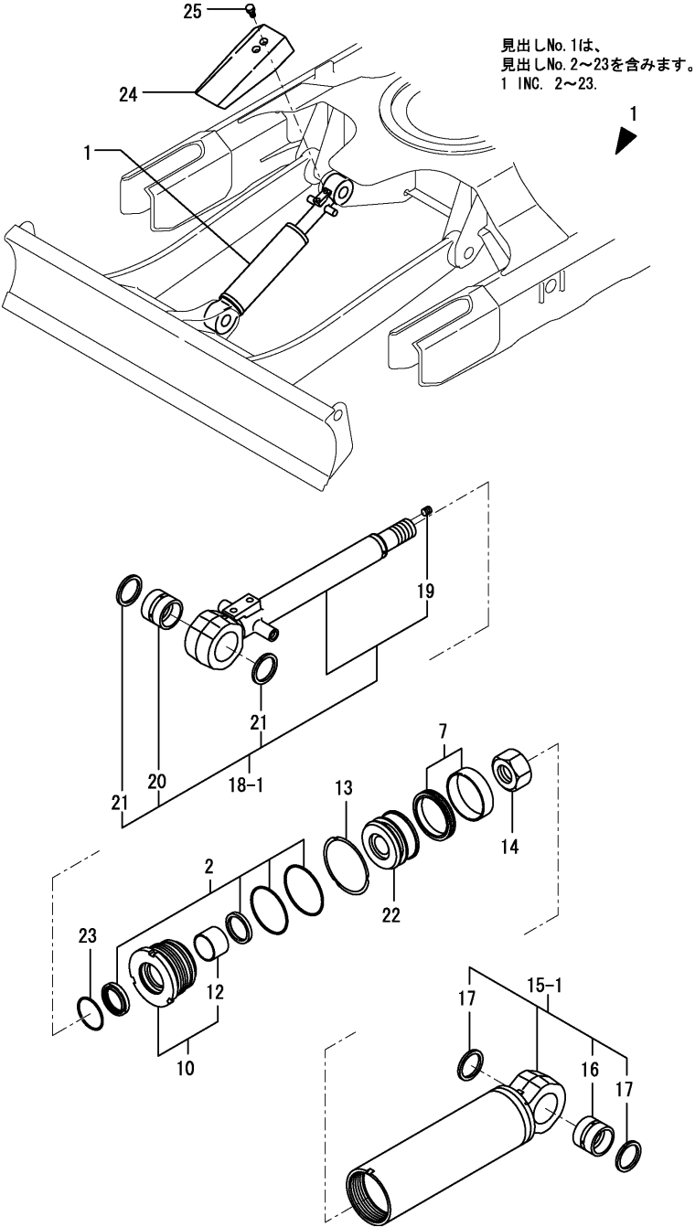
Fig.74. BLADE CYLINDER
