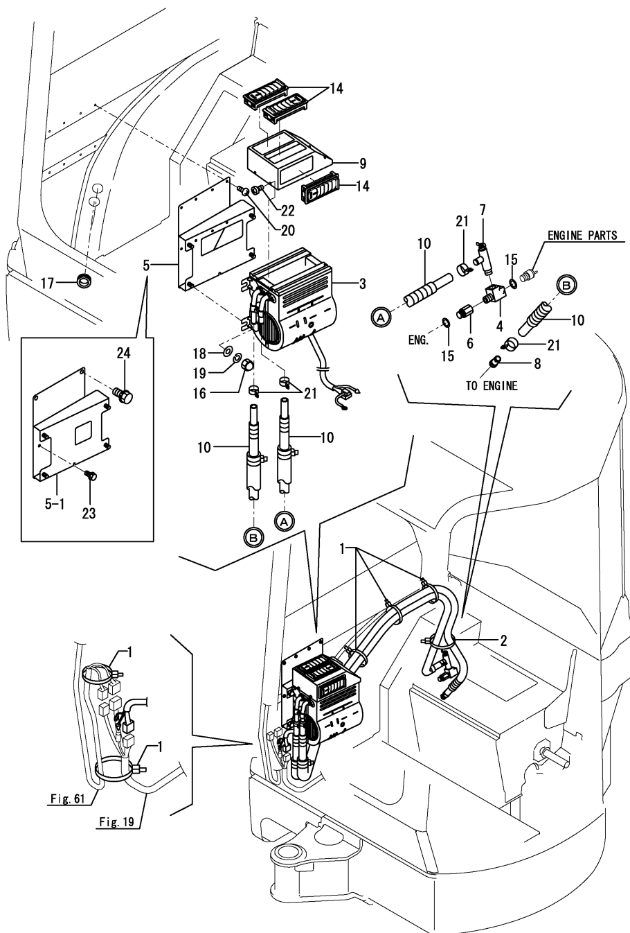
Fig.29. HEATER
