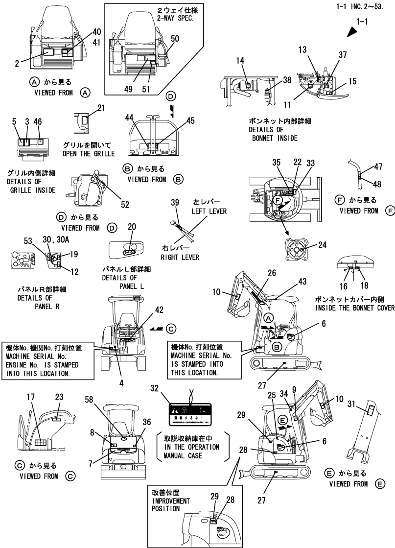
Fig.2. LABEL(CANOPY)(JP)(TO M3F000)
