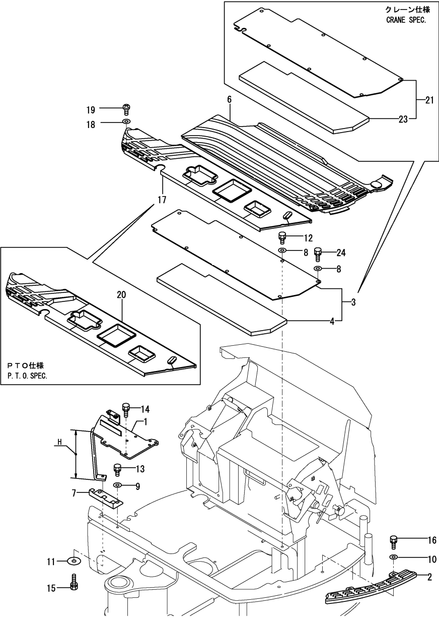
OCK10-M39703 AROUND SEAT Fig.52. STEP(CANOPY SPEC.)
