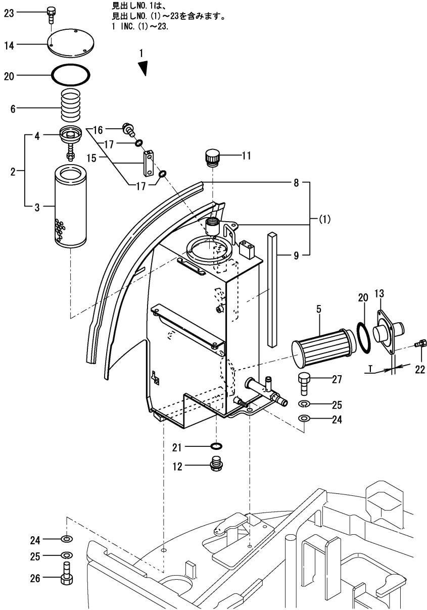
Fig.91. HYD.OIL TANK
