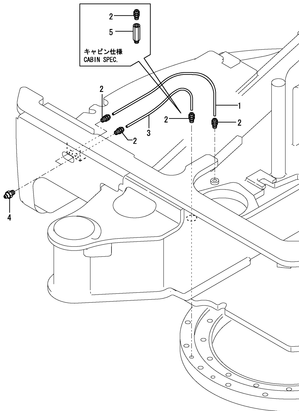
Fig.107. GREASING
