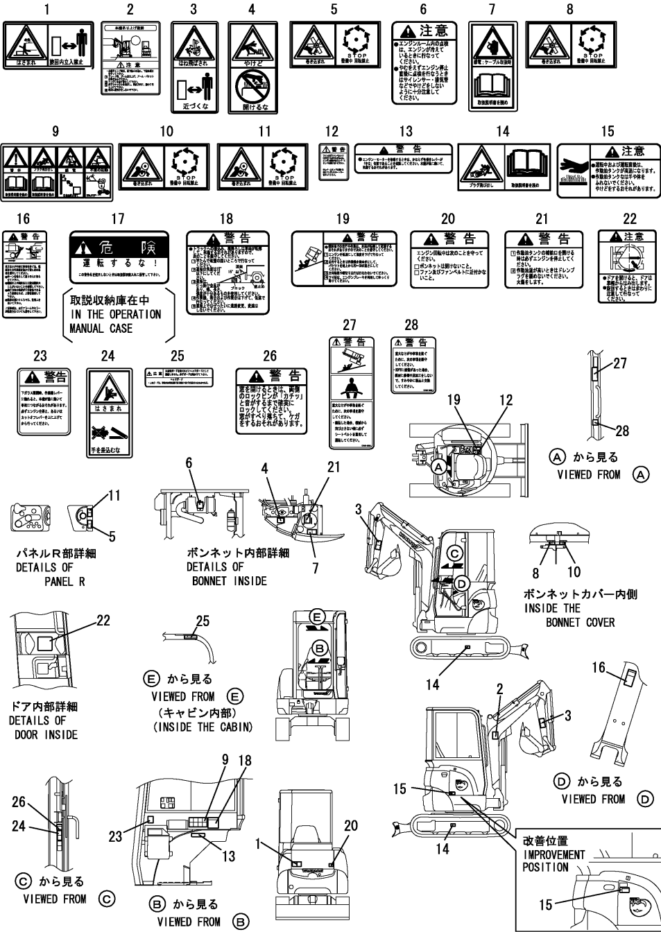
Fig.6. SAFETY LABEL(CABIN)(JP)
