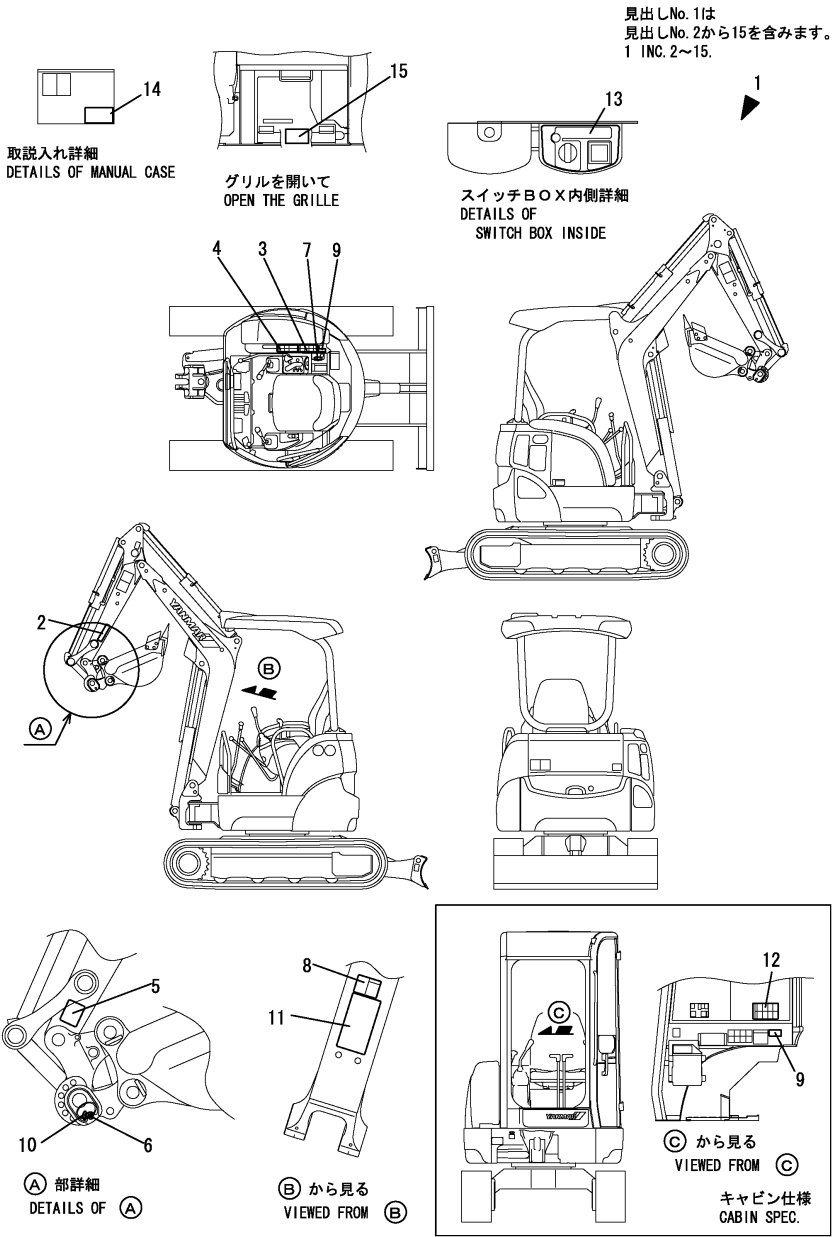
Fig.3. LABEL(QUICK COUPLER)(JP)
