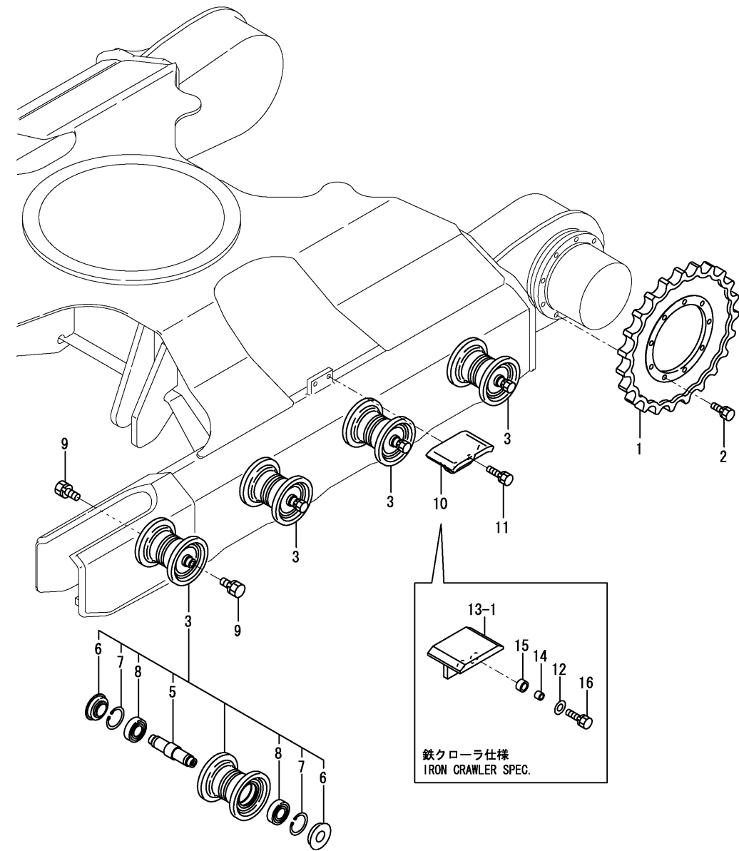
OCK10-M39703 TRAVELING Fig.30. SPROCKET & ROLLER
