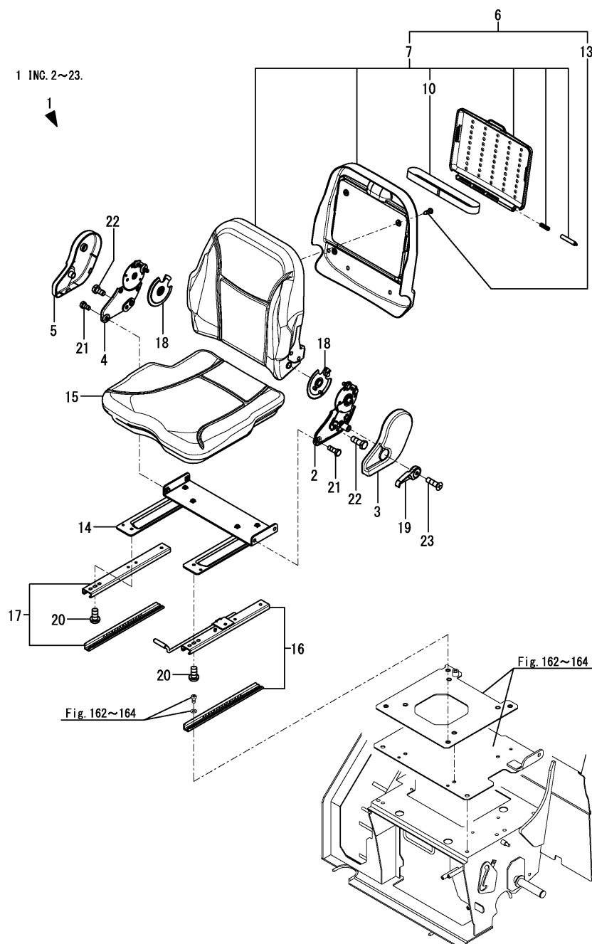
Fig.161. (56A)SEAT(FROM M3F495)
