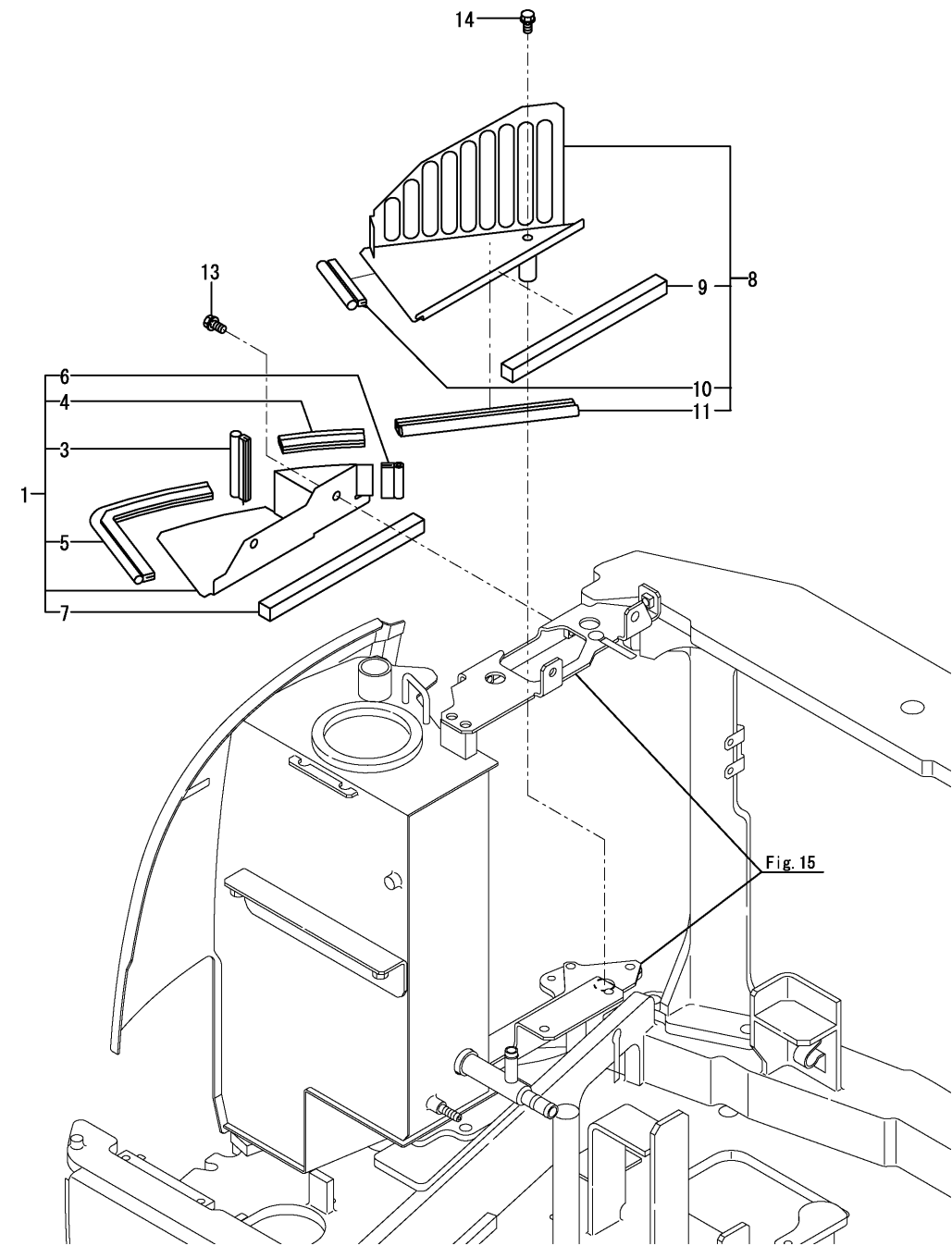
Fig.59. DUCT
