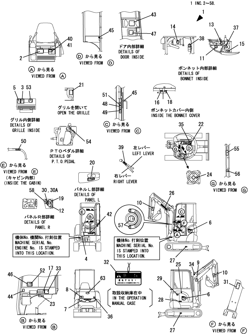
Fig.1. LABEL(CABIN)(JP)(TO M3F000)
