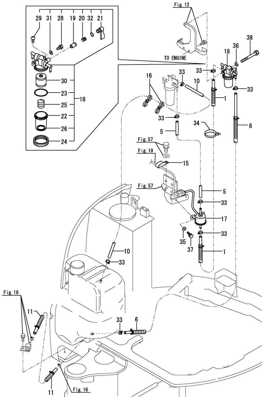
Fig.17. FUEL LINE
