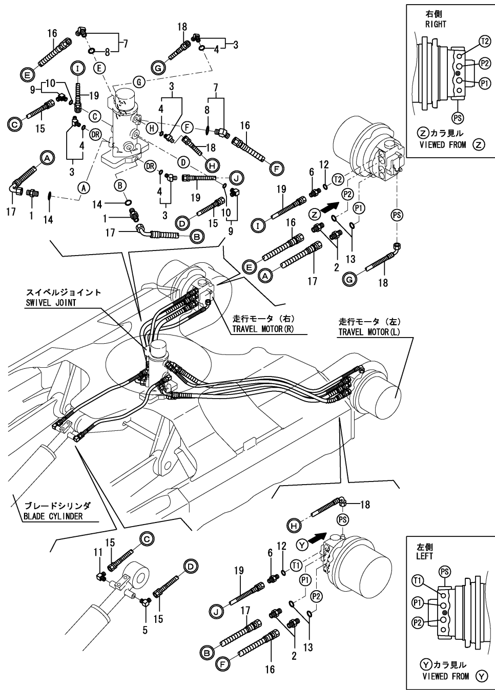
OCK10-M39703 HYDRAULIC OIL PIPING Fig.97. HYD.OIL PIPING(TRACK FRAME)
