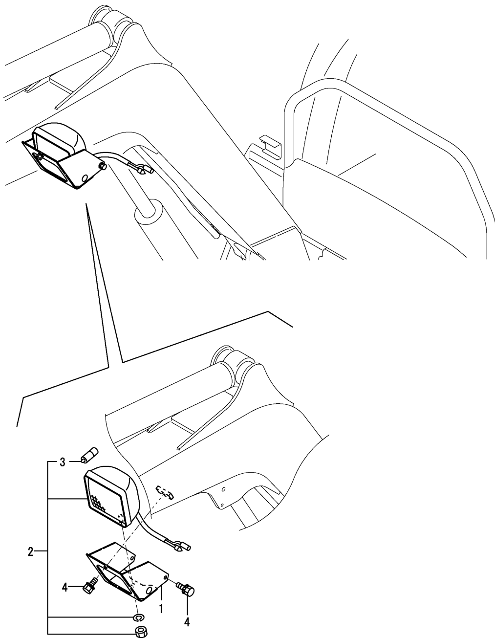
Fig.27. WORK LAMP
