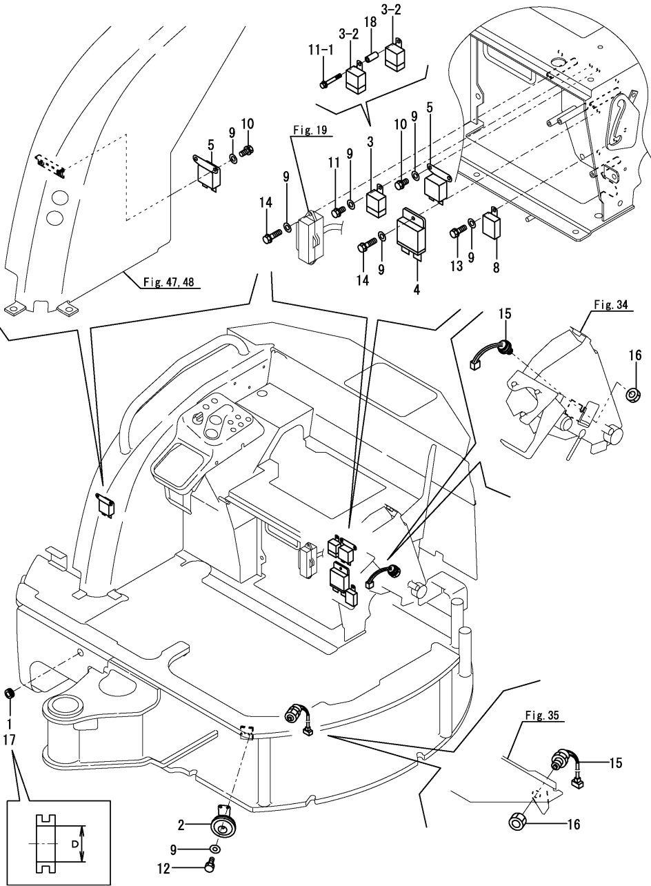
Fig.21. EQUIPMENT
