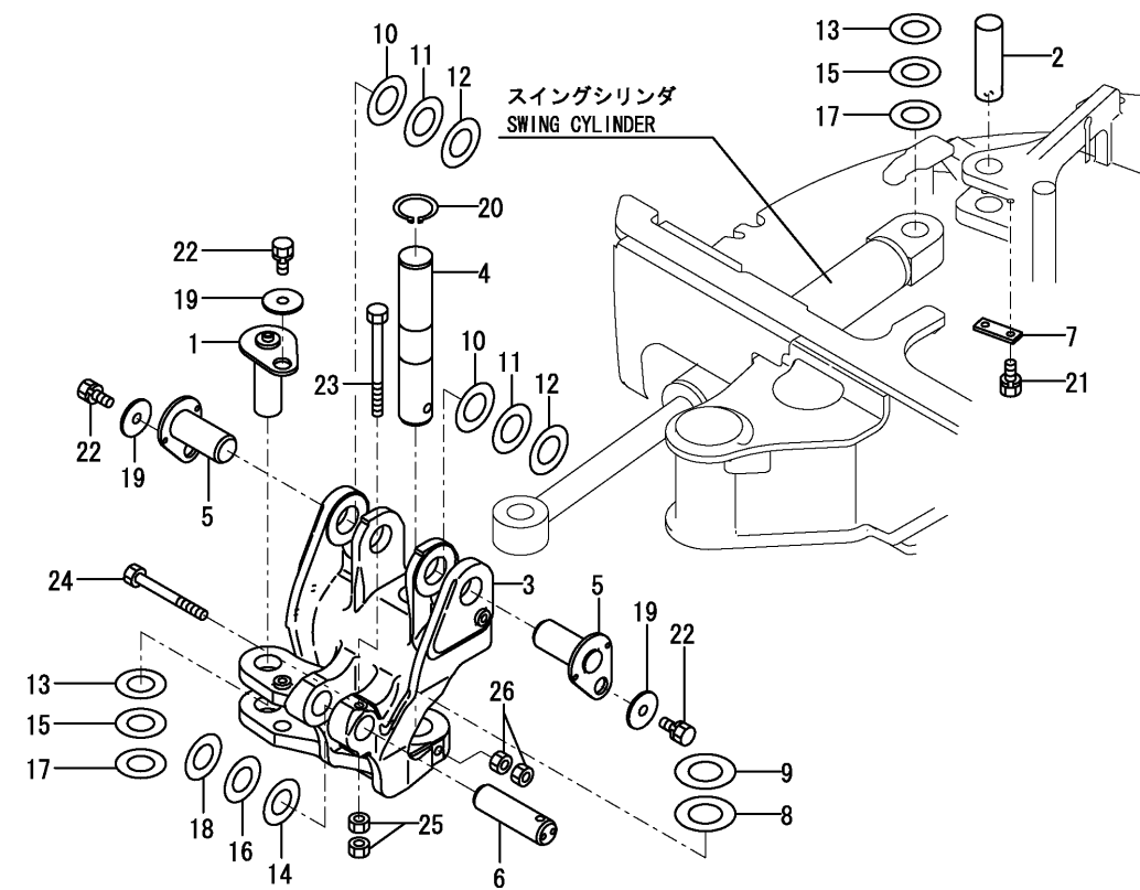
OCK10-M39703 IMPLEMENT Fig.110. BOOM BRACKET
