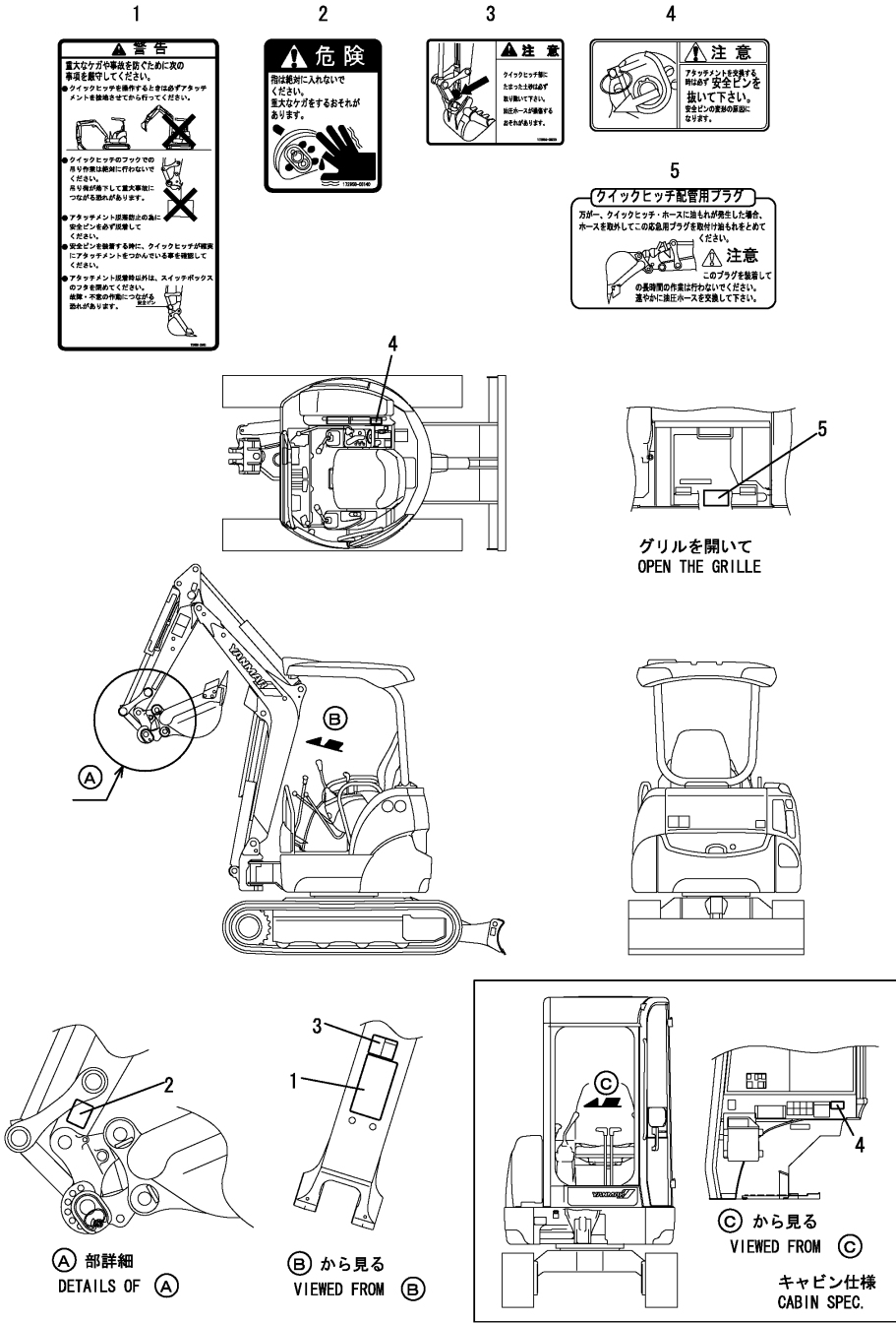
Fig.8. SAFETY LABEL(QUICK COUPLER)(JP)
