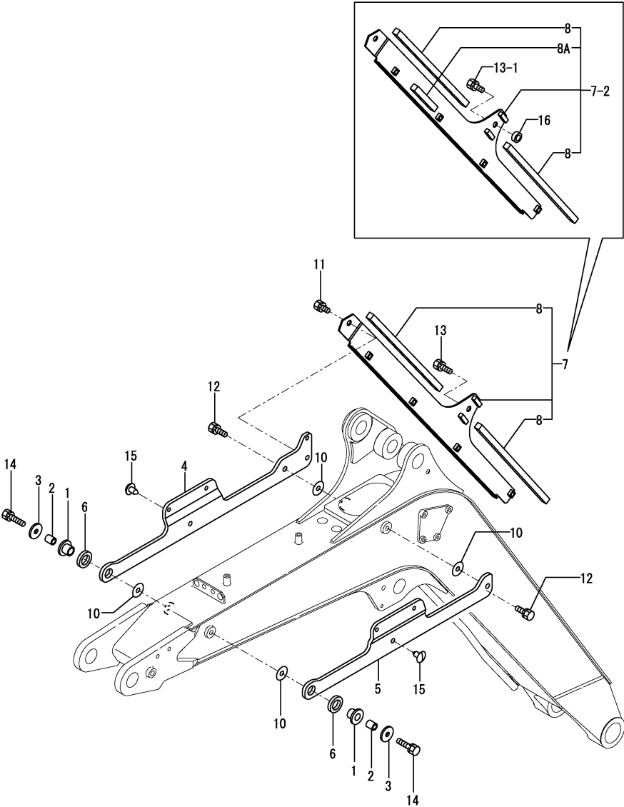
OCK10-M39703 IMPLEMENT Fig.119. STAY(CRANE SPEC.)
