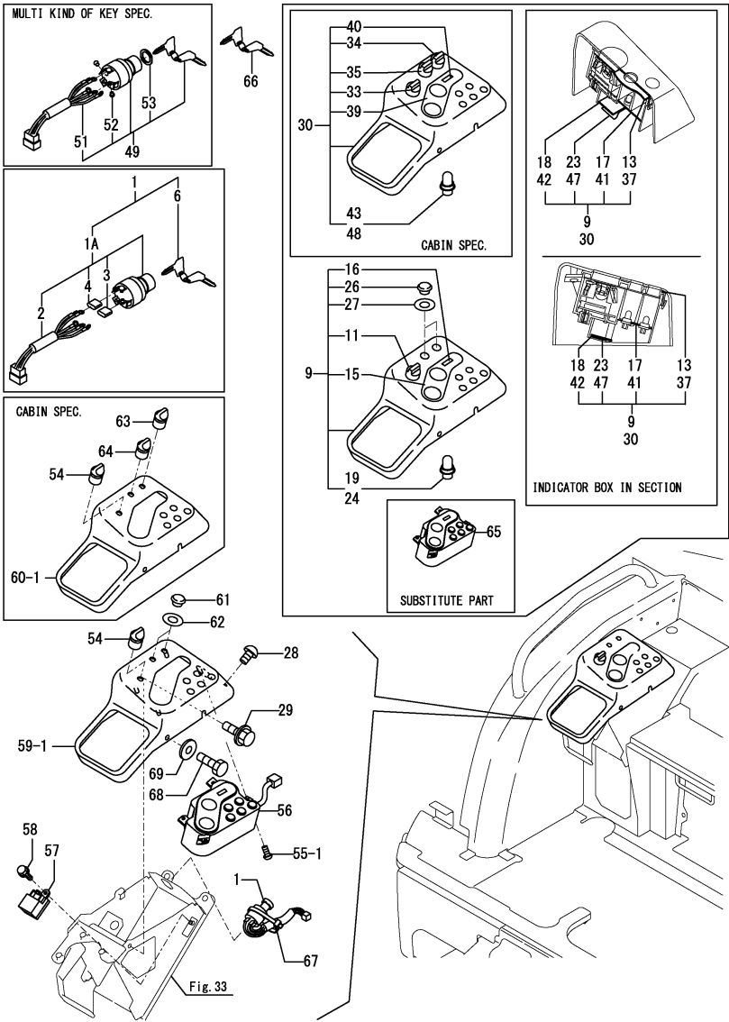
Fig.22. EQUIPMENT(INDICATOR BOX)
