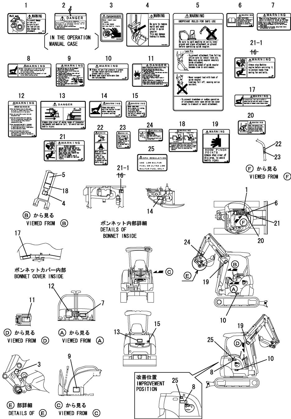
Fig.9. SAFETY LABEL(CANOPY)(EX)
