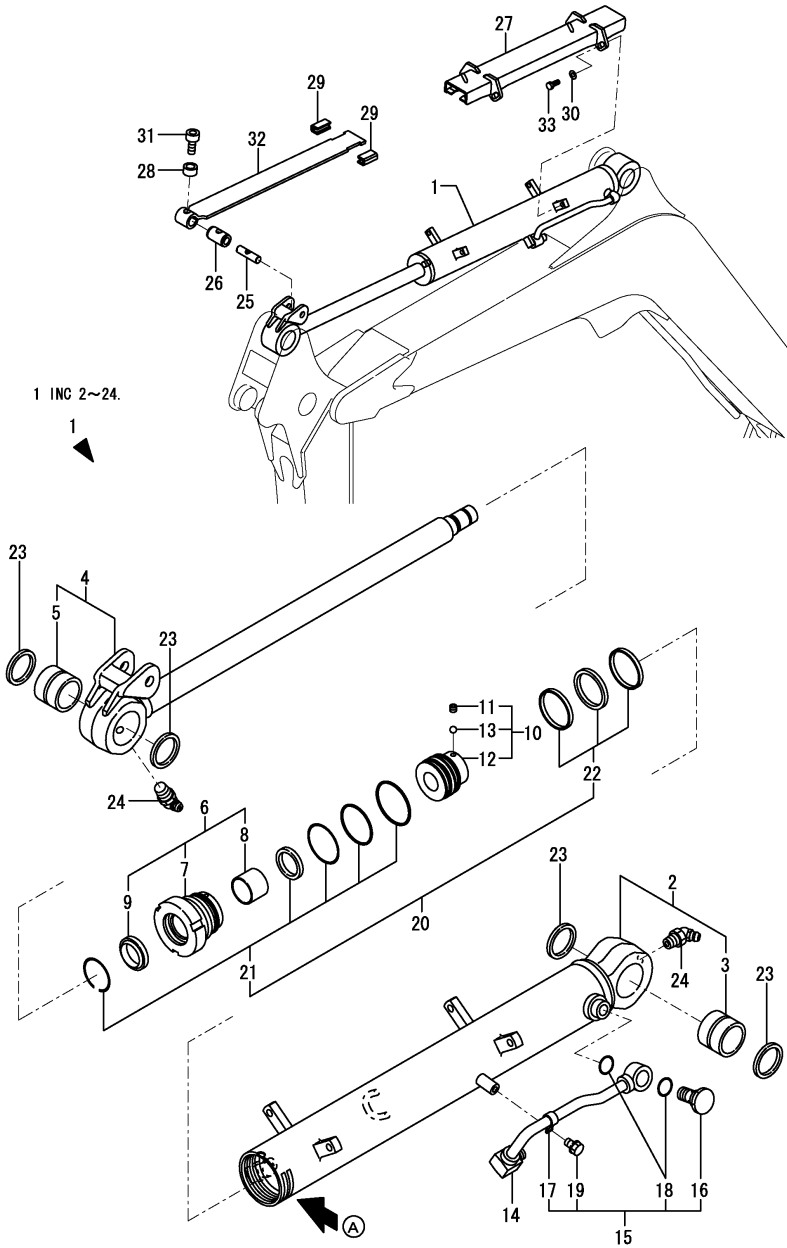
Fig.135. (70A)ARM CYLINDER(K SPEC.)
