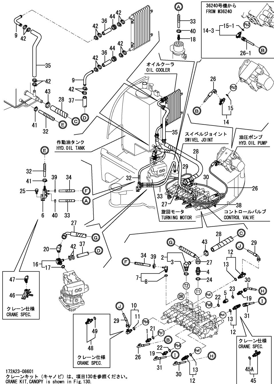
Fig.95. HYD.OIL PIPING(RETURN)
