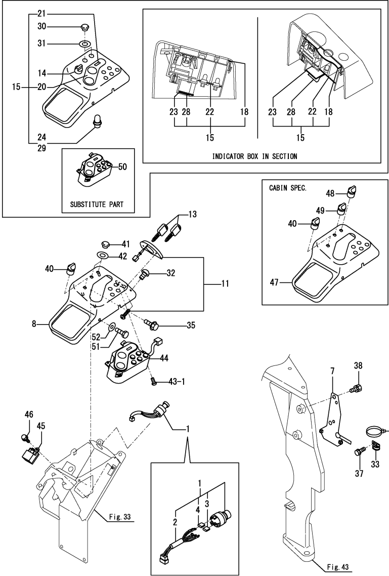
OCK10-M39703 ELECTRICAL PARTS Fig.23. EQUIPMENT(INDICATOR BOX)(IMMOBILIZER SPEC.)
