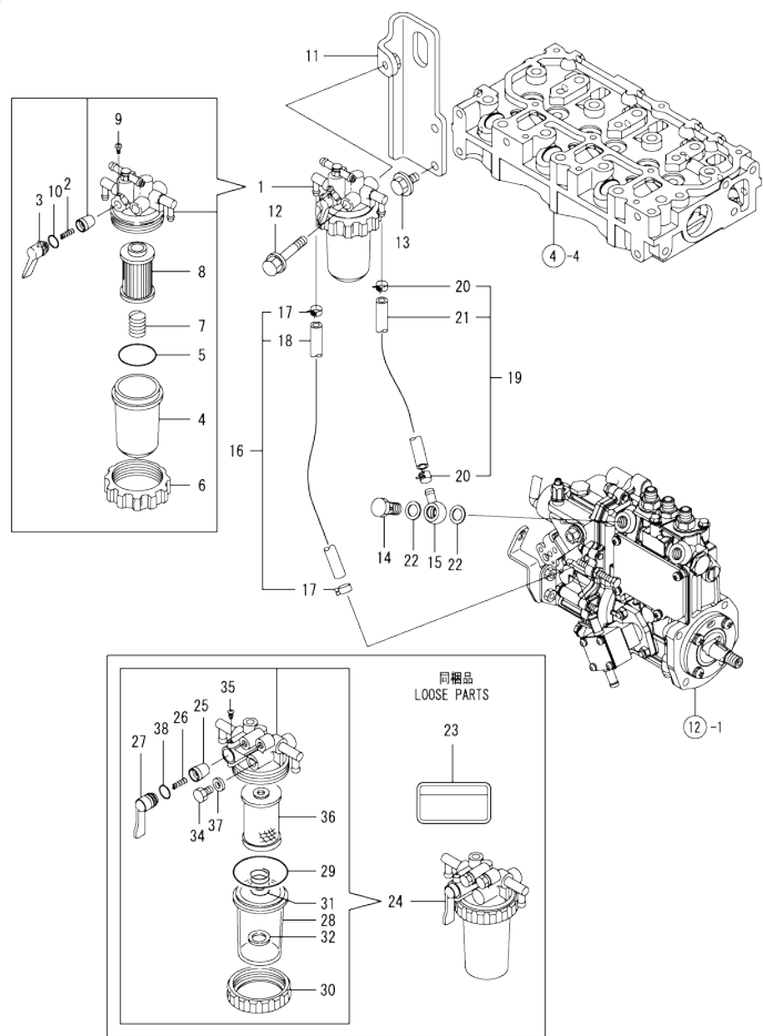
Fig.15. FUEL LINE
