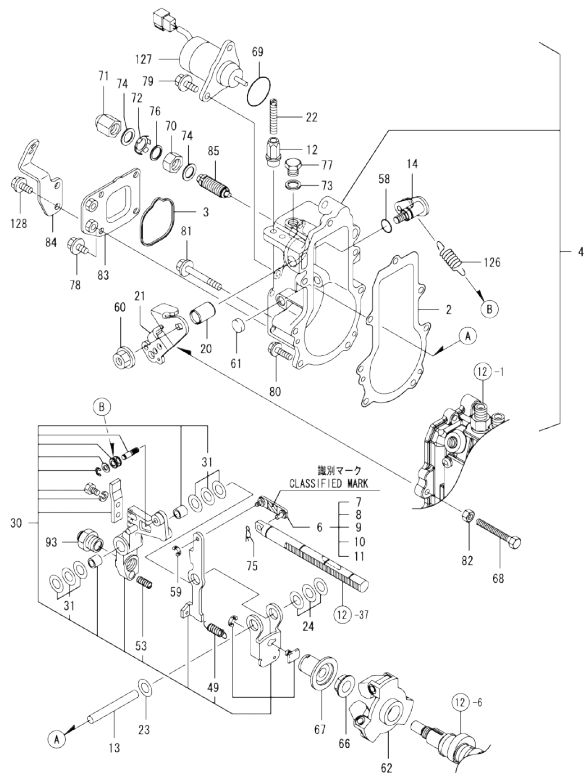
Fig.13. GOVERNOR
