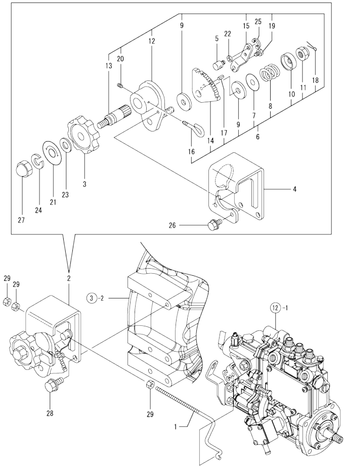
Fig.16. ENGINE CONTROL DEVICE
