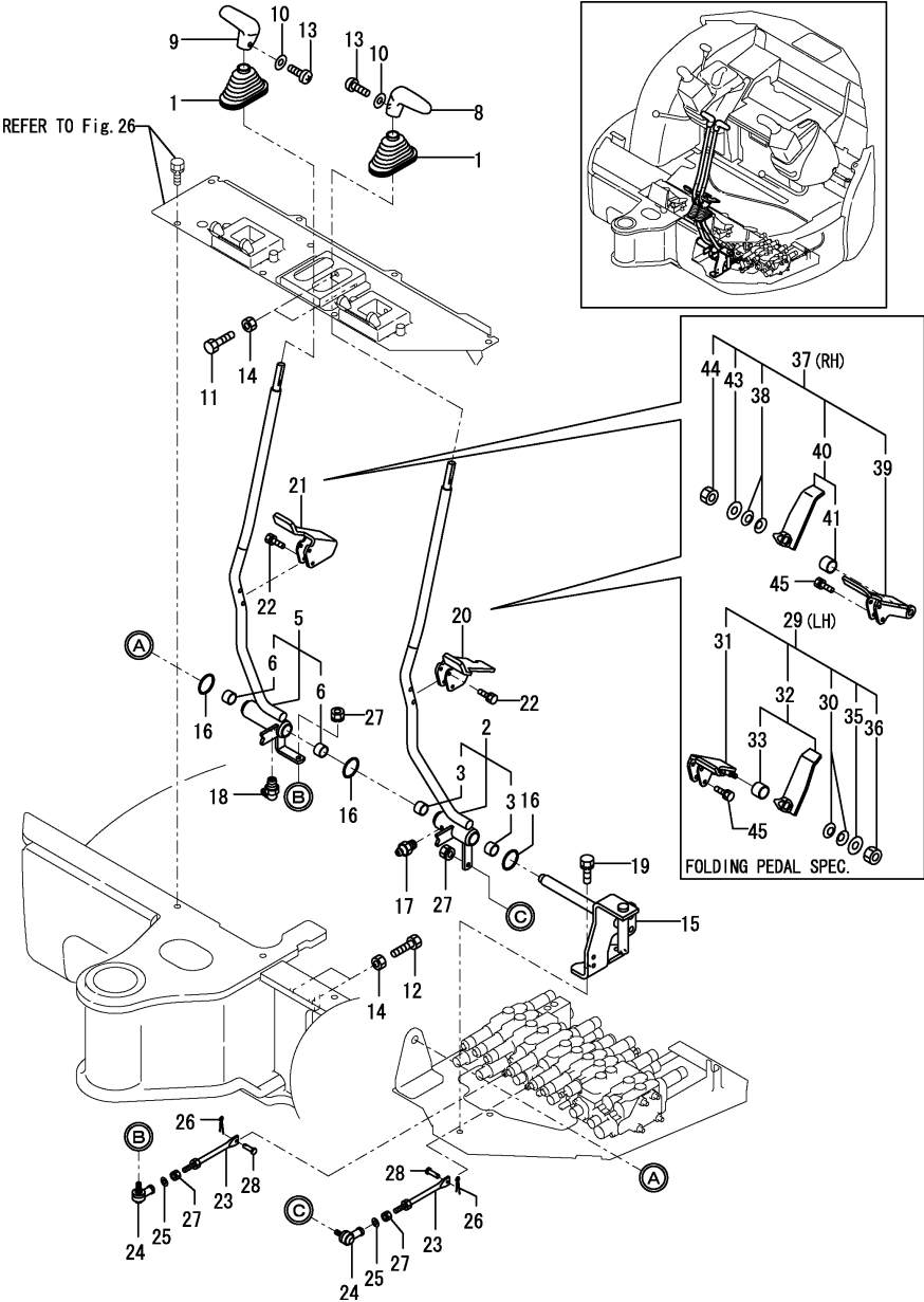
Fig.28. TRAVEL LEVER
