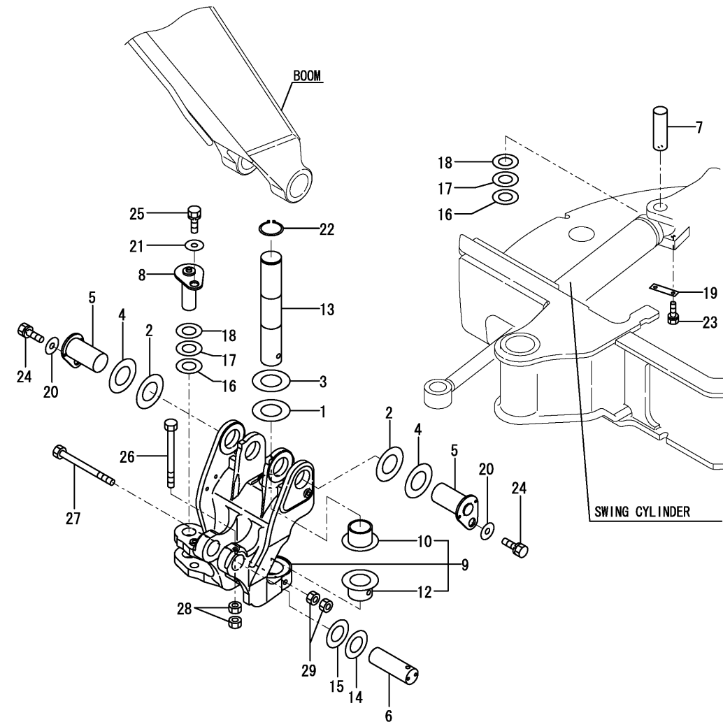
OCS10-M44901 IMPLEMENT Fig.95. BOOM BRACKET
