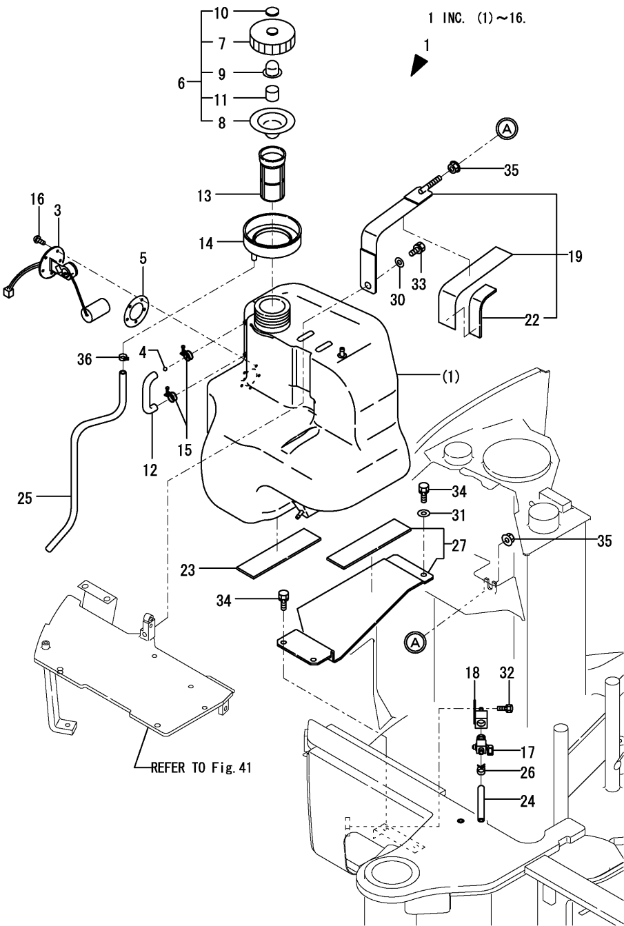
Fig.11. FUEL TANK
