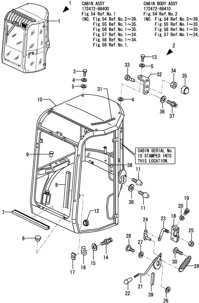
Fig.54. TIM CABIN(BODY)
