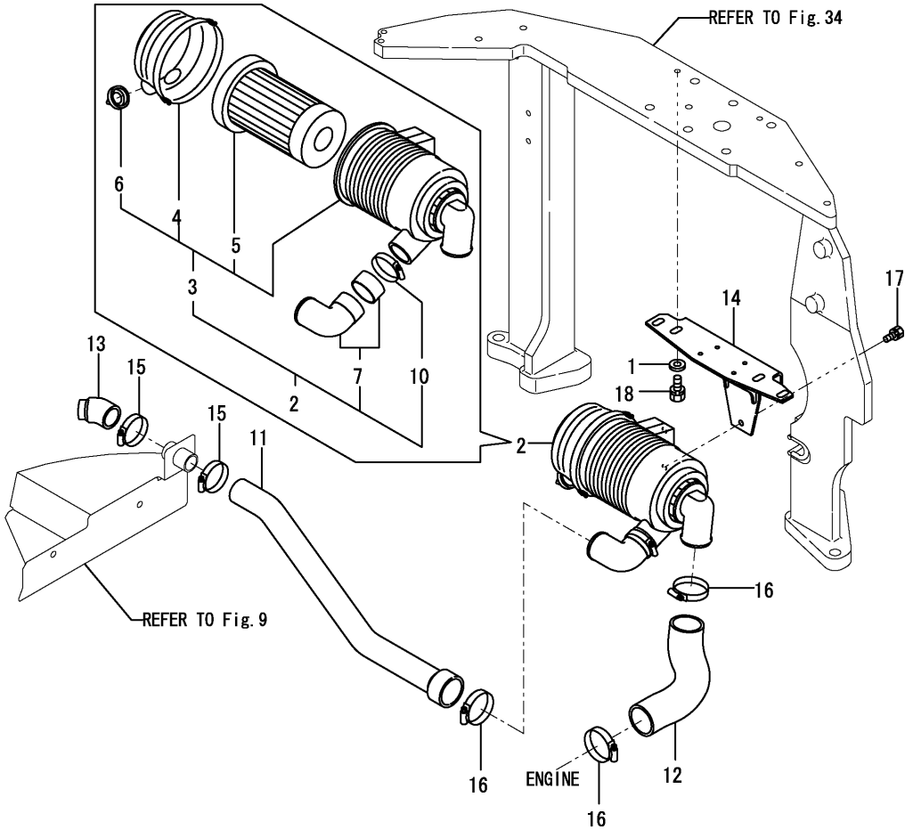
Fig.6. AIR CLEANER
