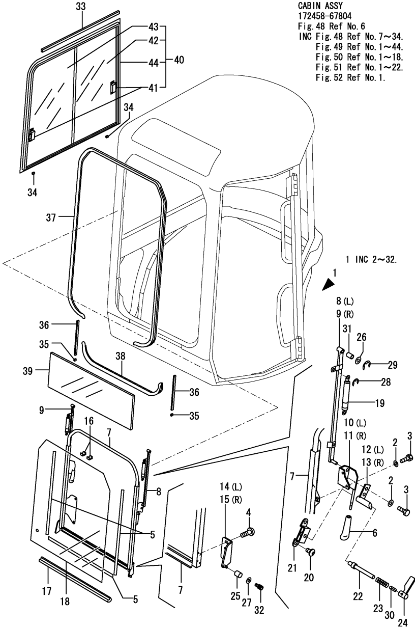
Fig.49. CABIN(GLASS)
