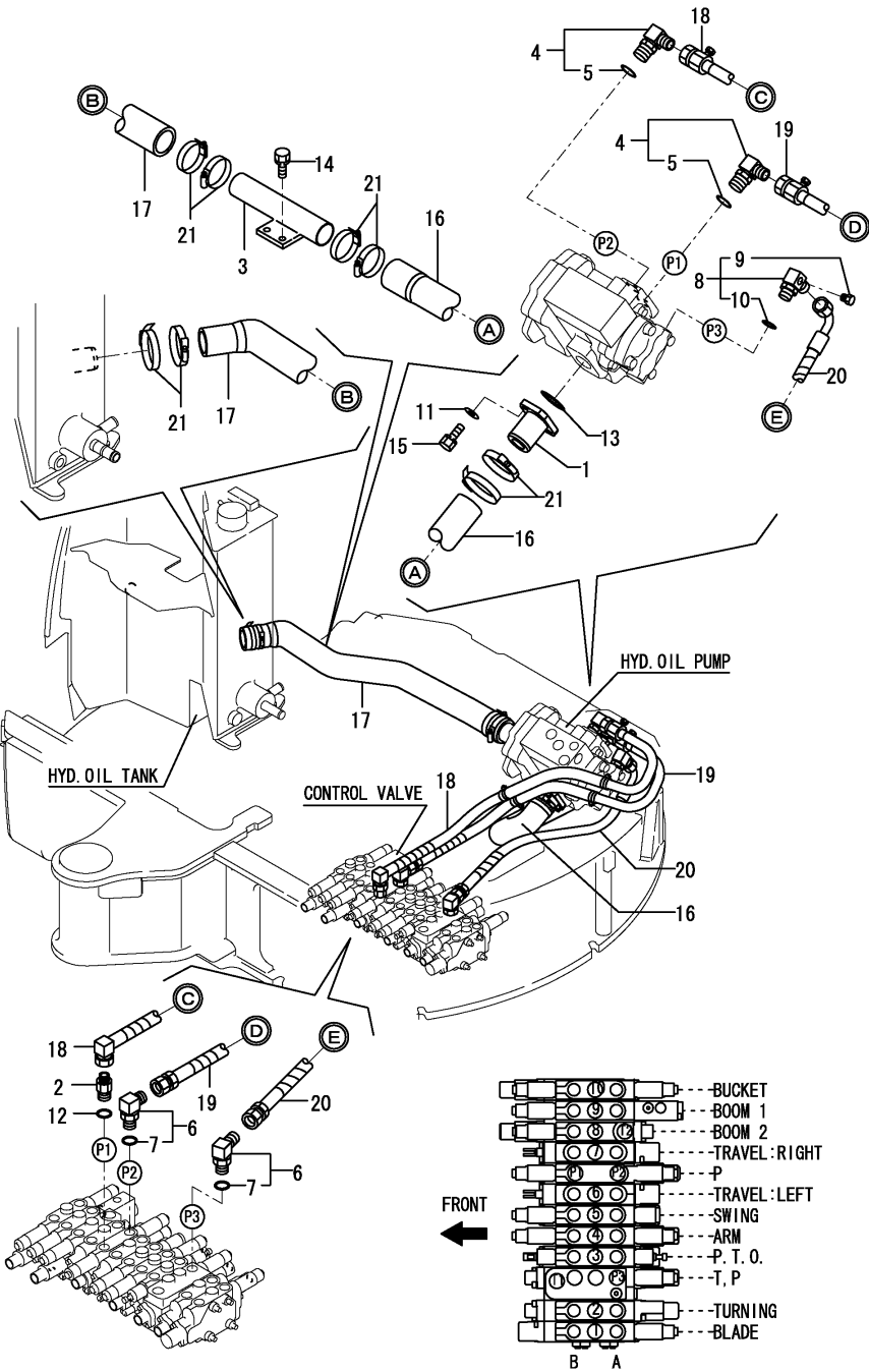
OCS10-M44901 HYDRAULIC OIL PIPING Fig.83. TANK - PUMP - CONTROL VALVE
