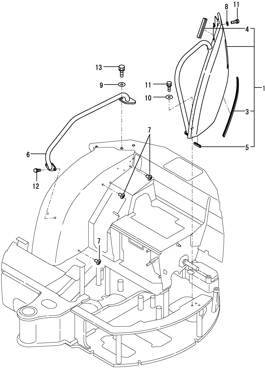
Fig.40. COVER(CANOPY)
