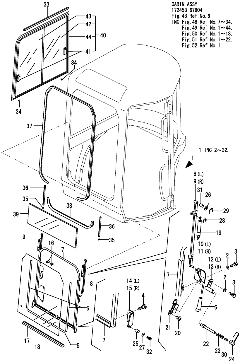
Fig.49. CABIN(GLASS)
