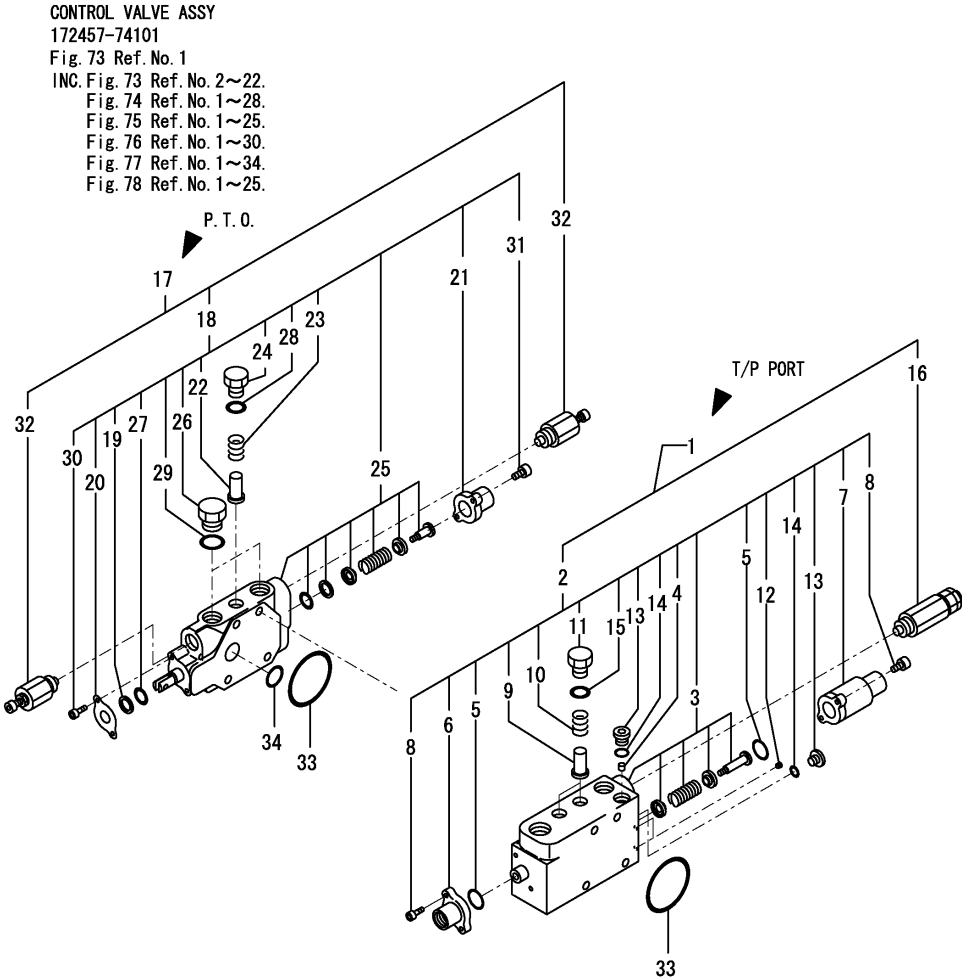
Fig.77. CONTROL VALVE(5/6)
