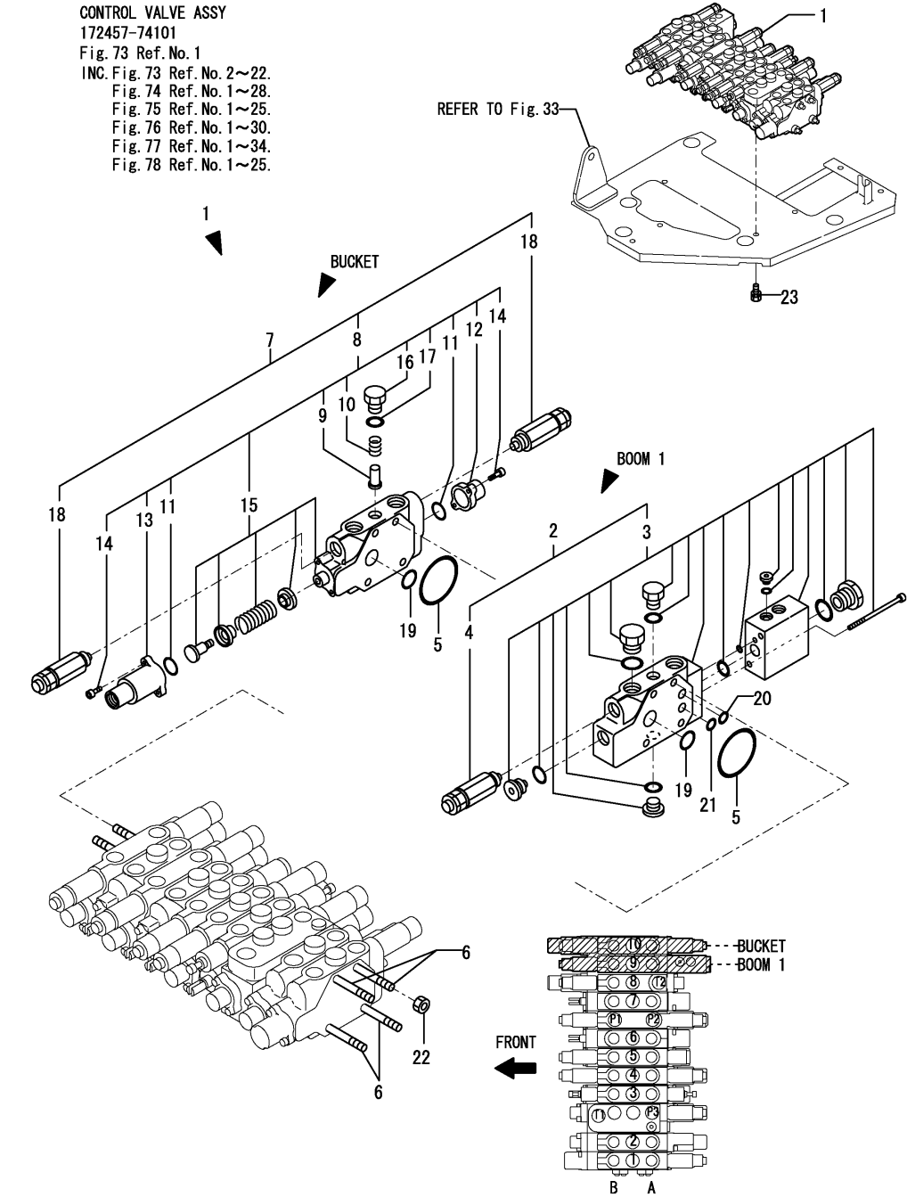
Fig.73. CONTROL VALVE(1/6)
