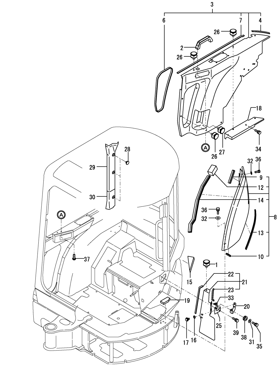
Fig.39. COVER(CABIN)
