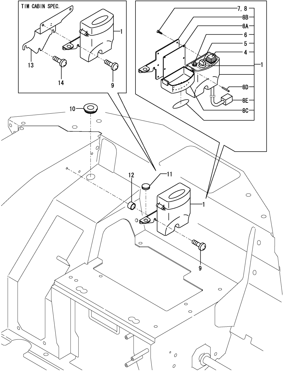
OCS10-M44901 ELECTRICAL PARTS Fig.17. QUICK COUPLER(SWITCH BOX)
