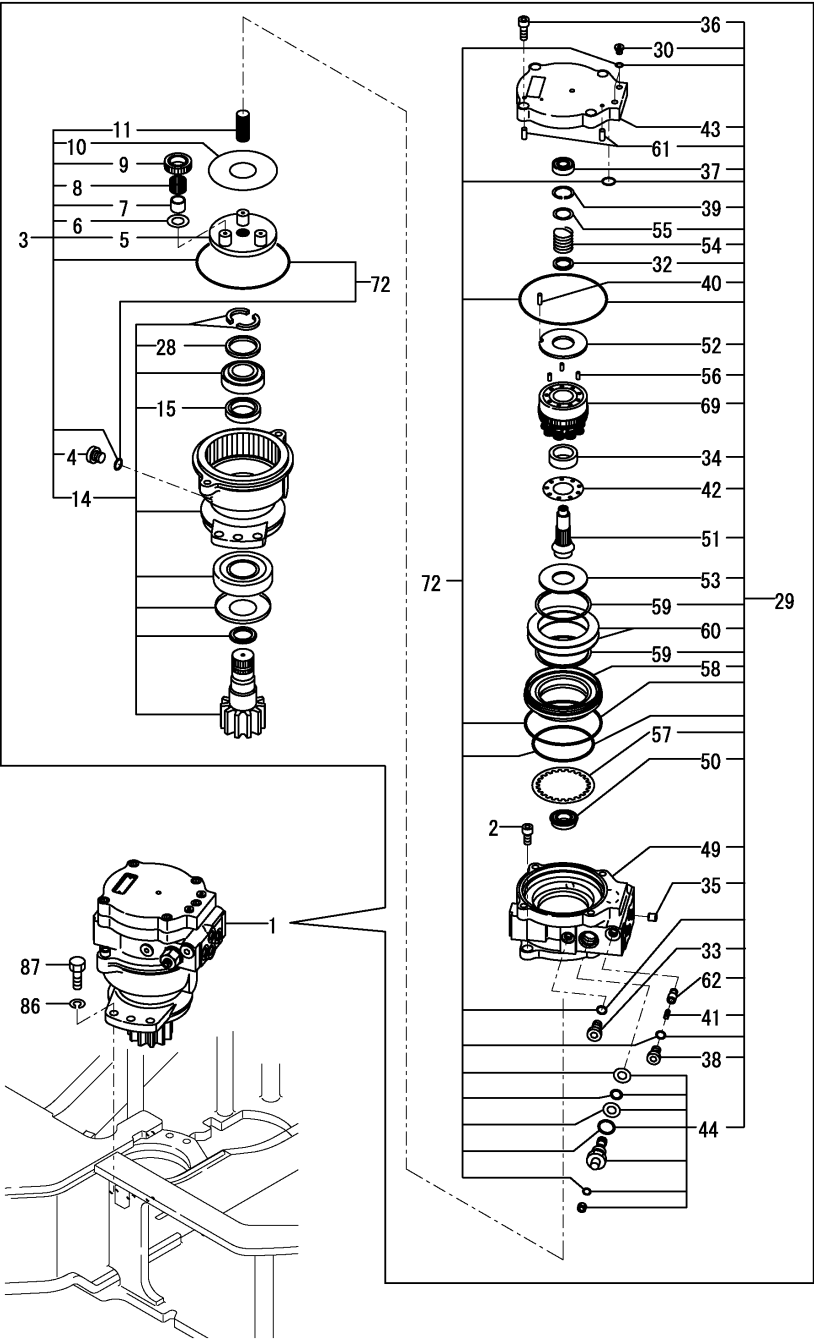
Fig.71. TURNING MOTOR
