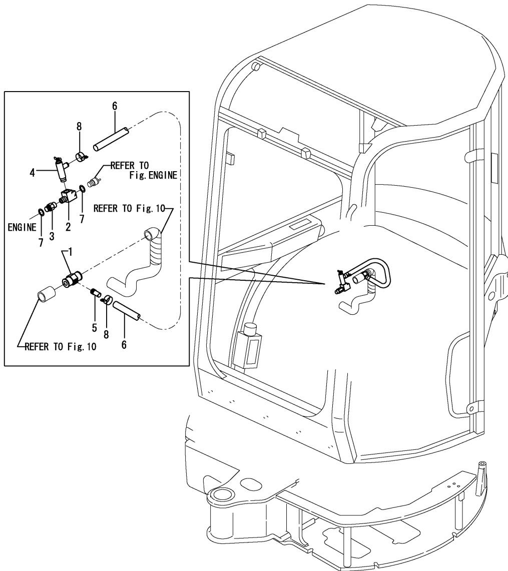
Fig.21. HEATER(PIPING)(TIM CABIN)
