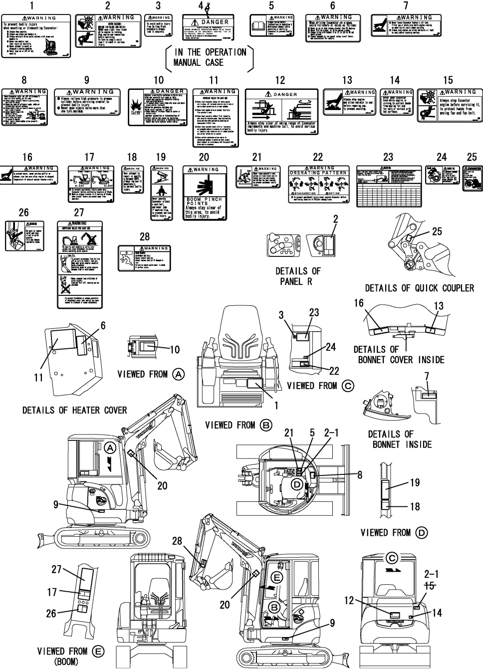
Fig.3. LABEL(SAFETY)(CABIN)
