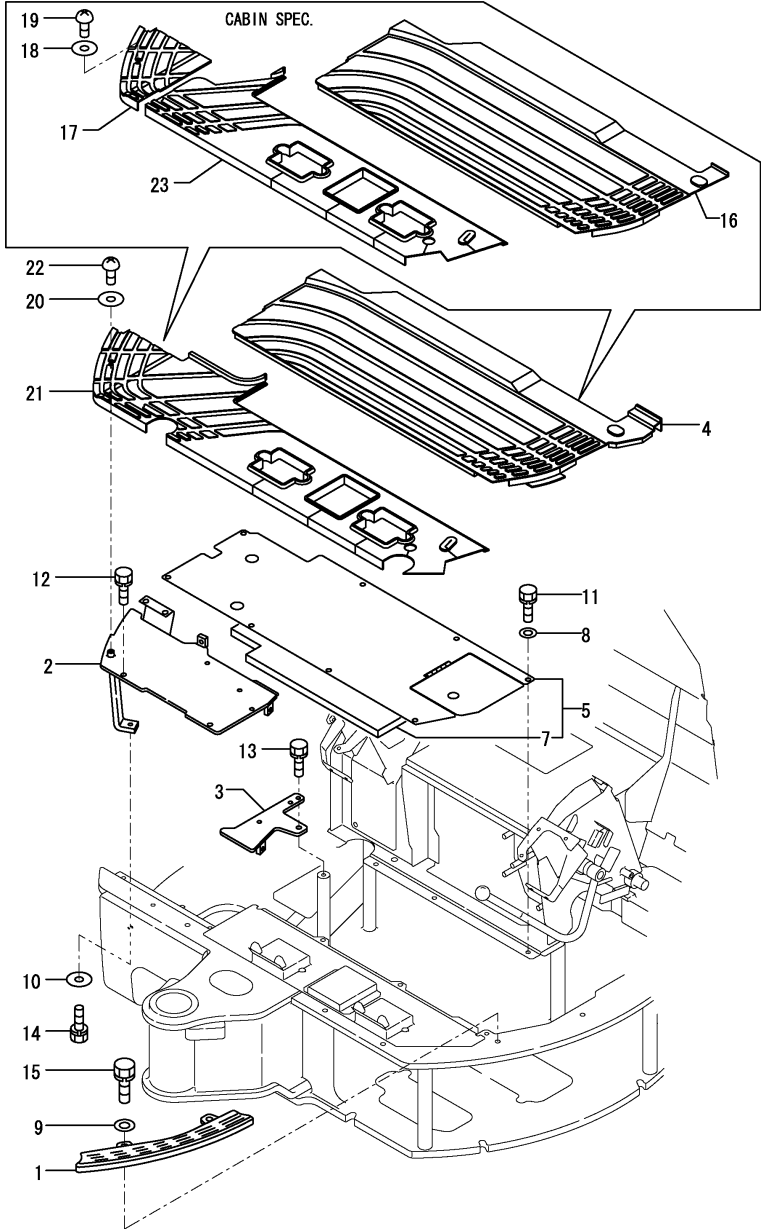
OCS10-M44901 AROUND SEAT Fig.41. STEP & FLOOR MAT
