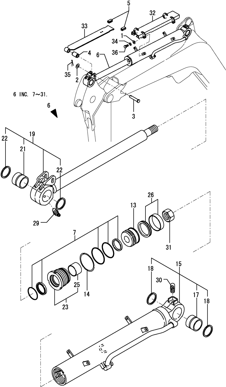
Fig.65. ARM CYLINDER
