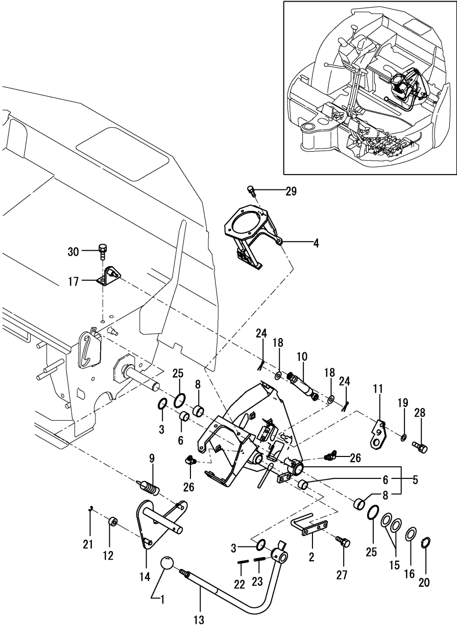
OCS10-M44901 CONTROL EQUIPMENT Fig.27. LOCK LEVER & STAND(LEFT)
