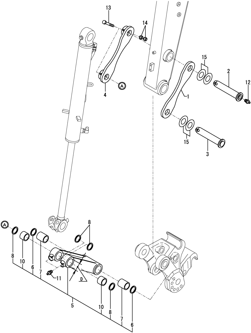
OCS10-M52701 IMPLEMENT Fig.108. BUCKET ARM & LINK
