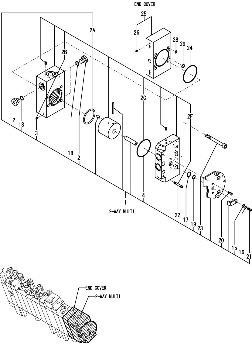
Fig.86. CONTROL VALVE(US,AS,NZ:7/7)
