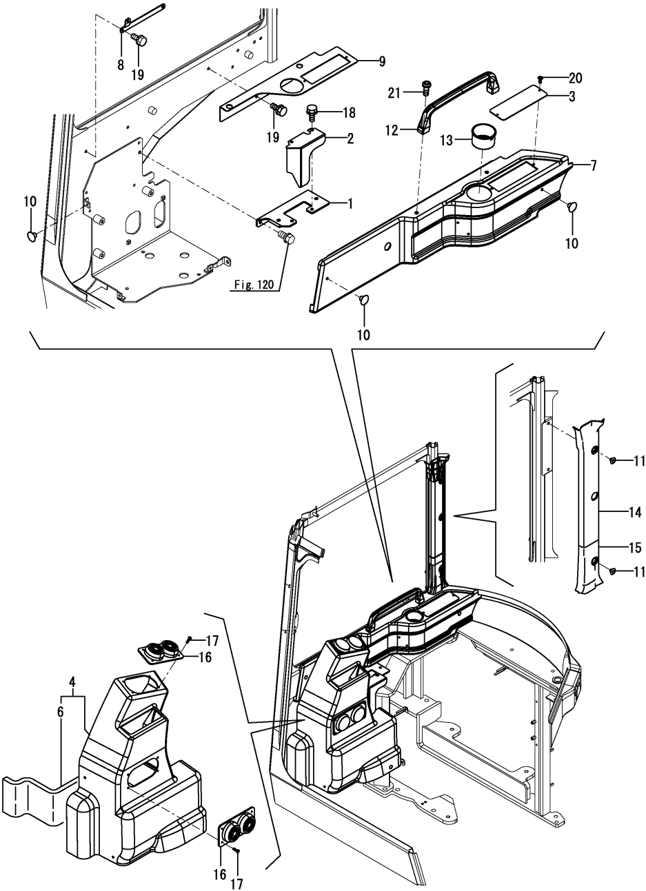
Fig.121. (59A)CABIN(COVER)(FROM M53439)
