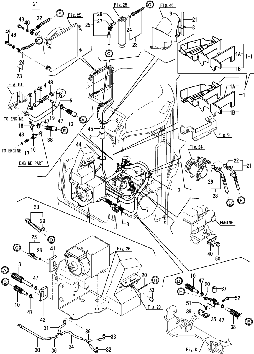
Fig.27. AIR CONDITIONER(PIPING)
