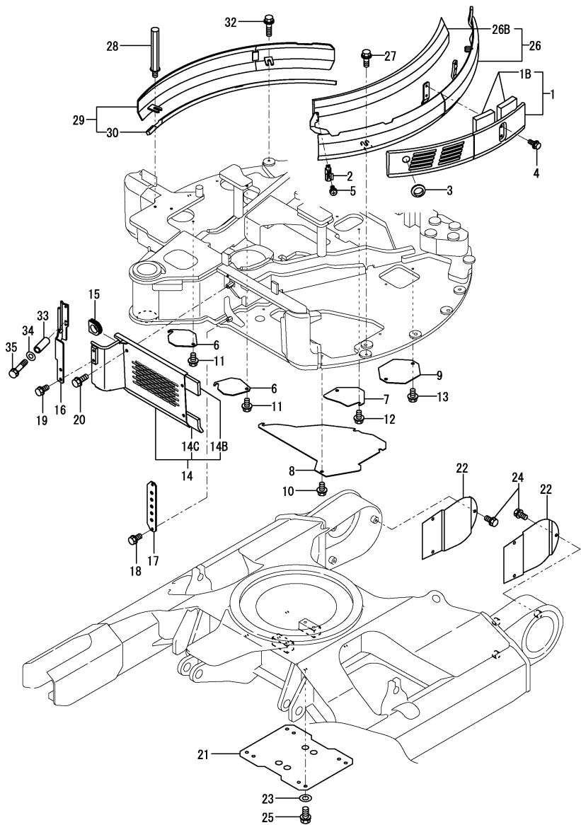
OCS10-M52701 COVER Fig.45. COVER(FRAME)
