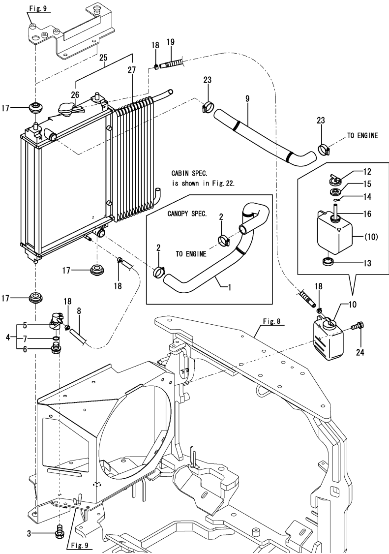
0CS10-M52701 ENGINE RELATED Fig.10. RADIATOR & SUB-TANK
