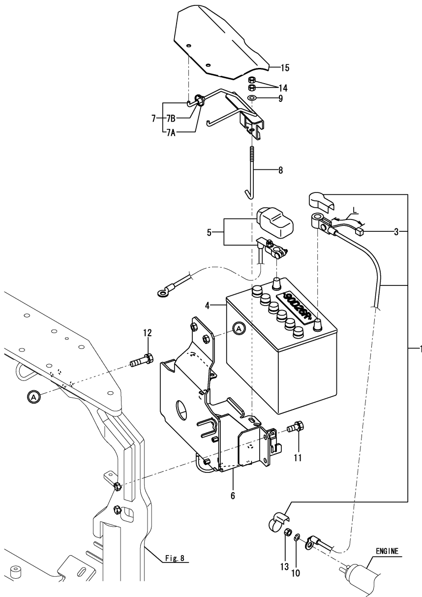
Fig.14. BATTERY
