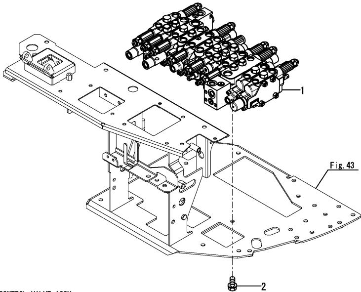
CONTROL VALVE ASSY Fig. 108 Ref. No. 1. INC. Fig. 109~114.
