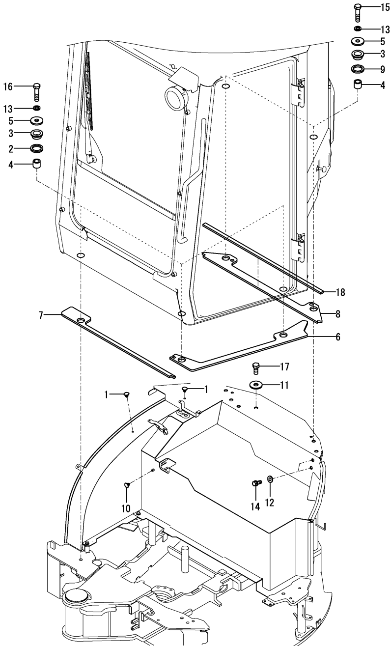
Fig.96. CABINE (ALMOFADA)
