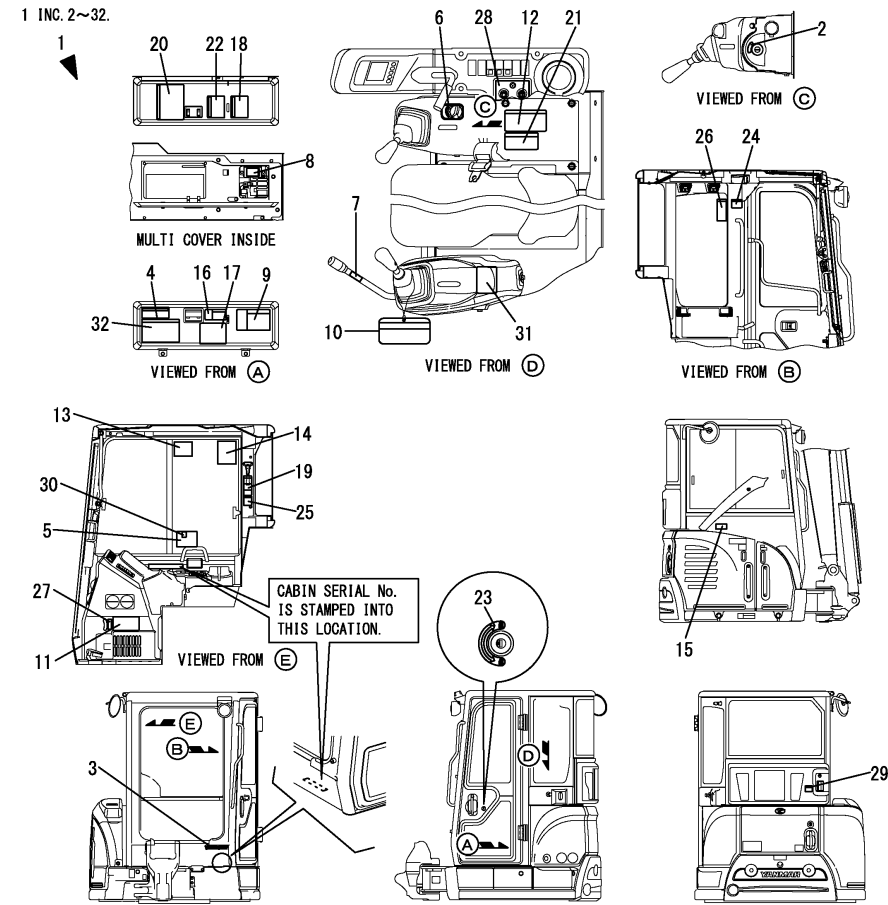
Fig.159. (4A)ETIQUETA(CABINE)(DE MBF001)
