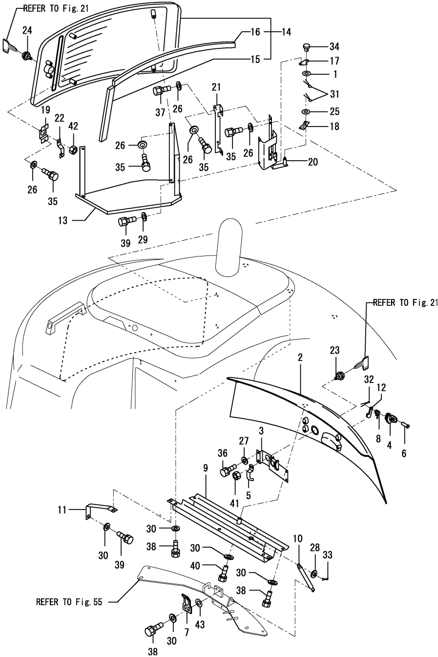
Fig.57. BONNET(3 : SIDE,REAR COVER)
