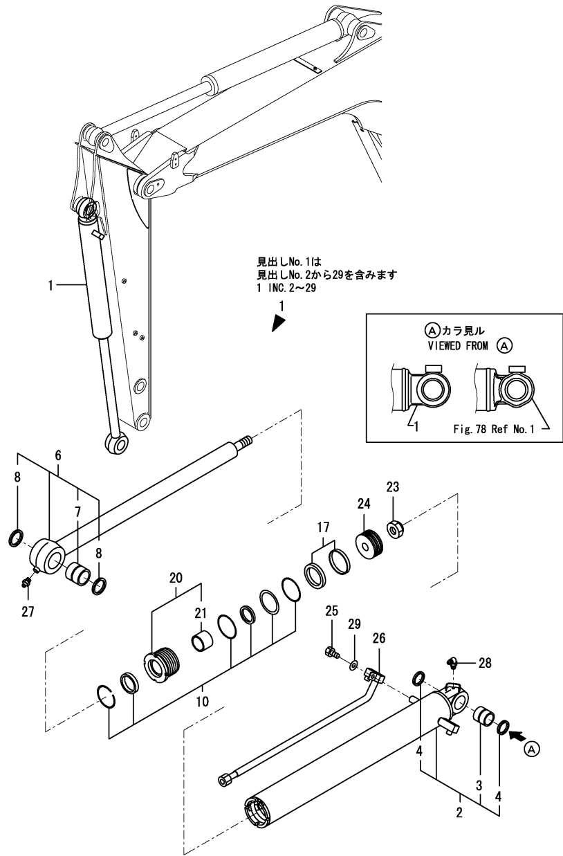
Fig.77. BUCKET CYLINDER
