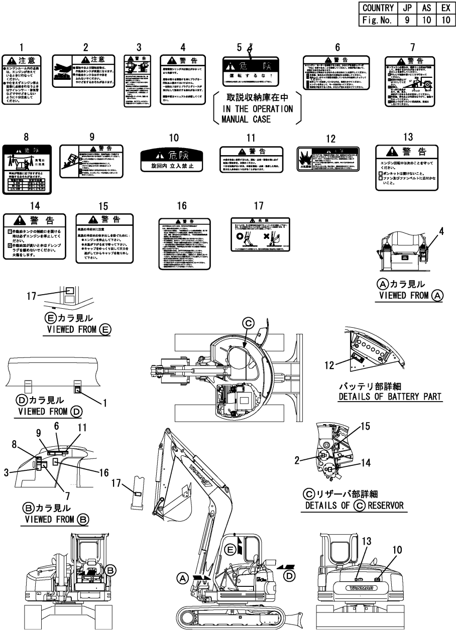
Fig.9. SAFETY LABEL(CANOPY : JP)
