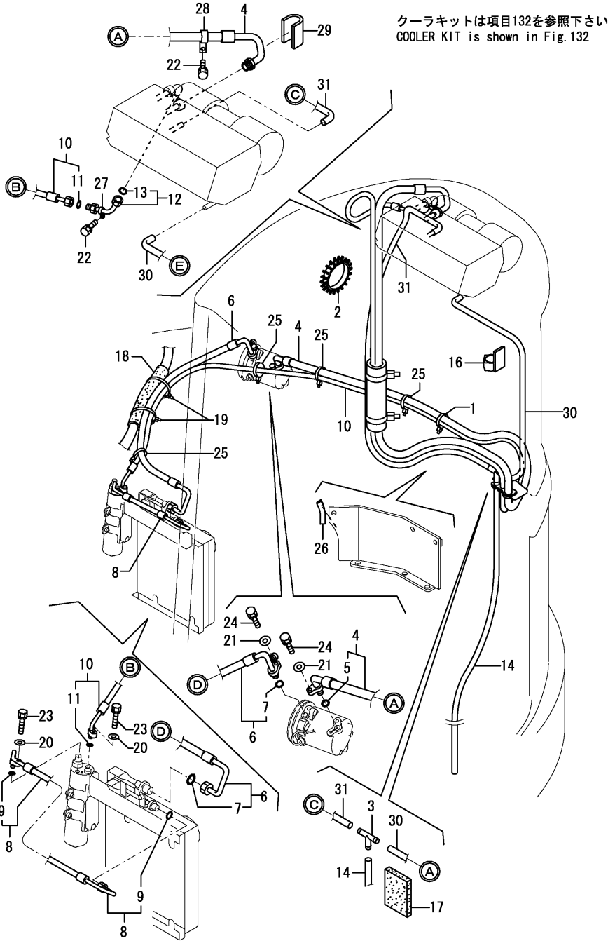
Fig.35. COOLER(PIPING)
