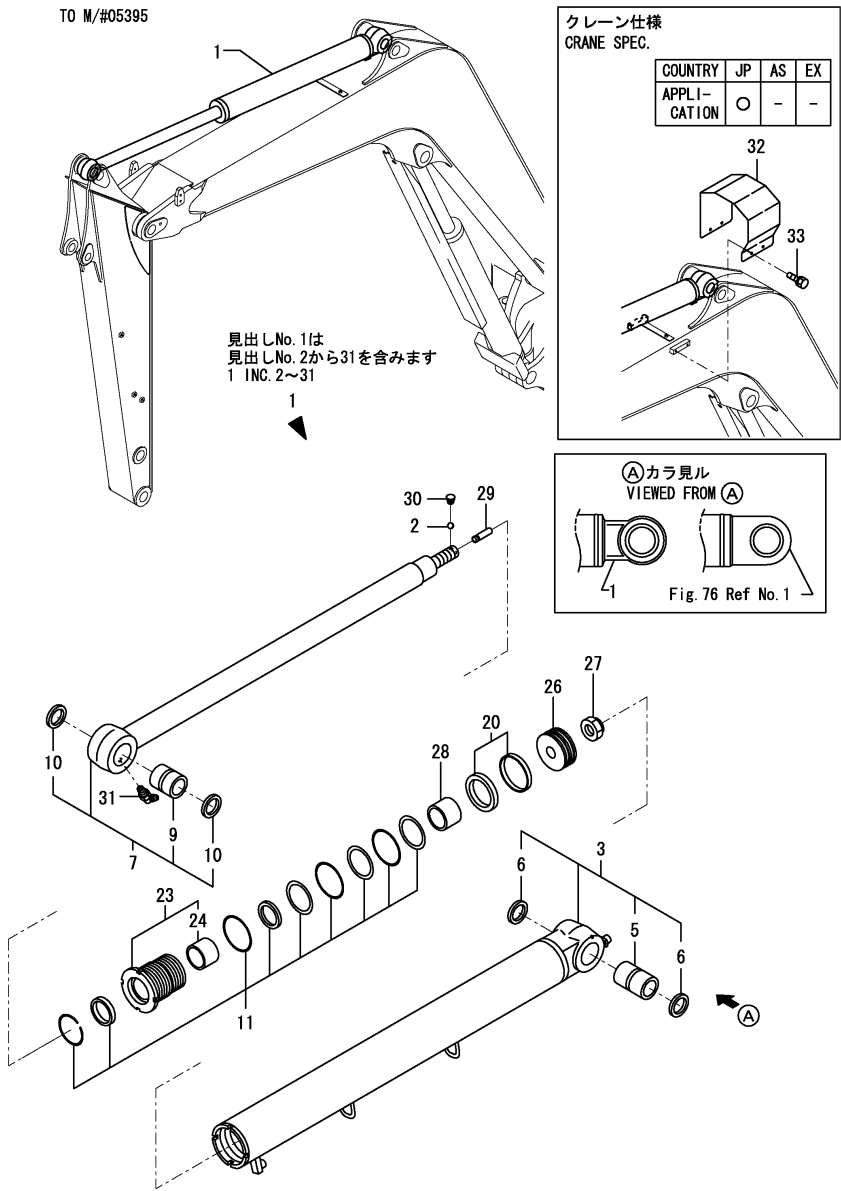
Fig.75. ARM CYLINDER(PREVIOUS)
