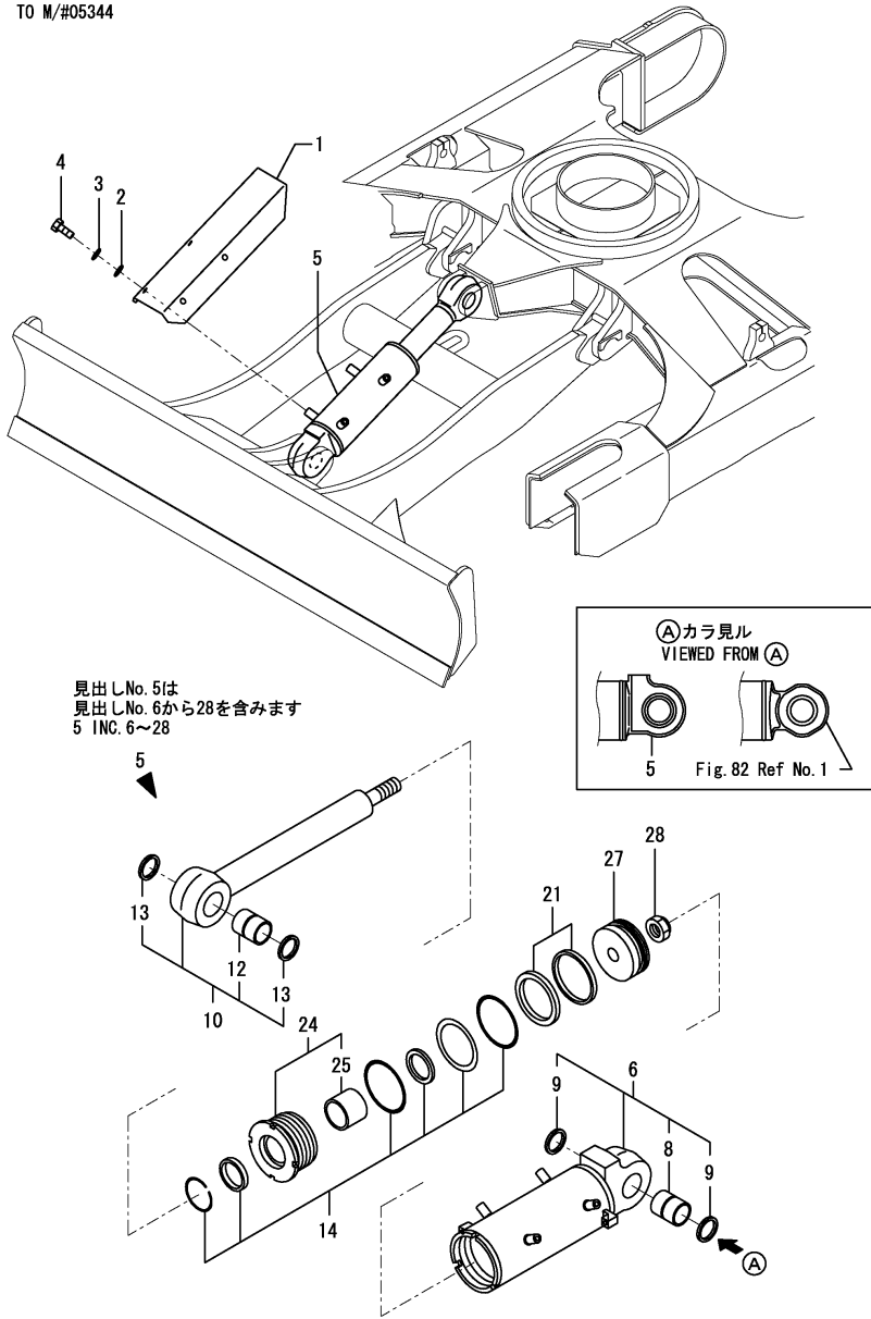
Fig.81. BLADE CYLINDER(PREVIOUS)
