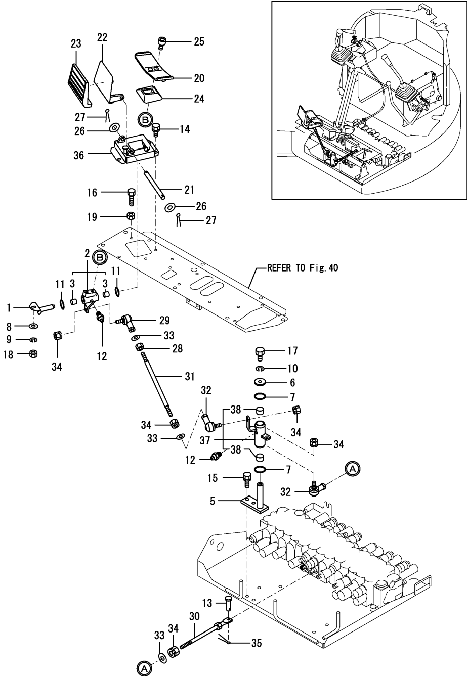
Fig.44. CONTROL EQUIPMENT(SWING)
