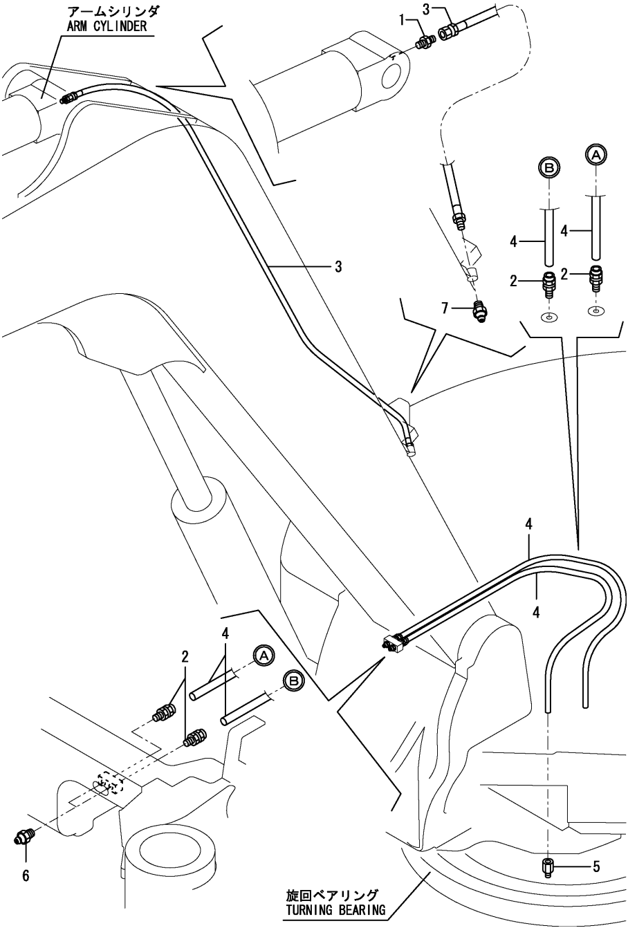
Fig.121. GREASING
