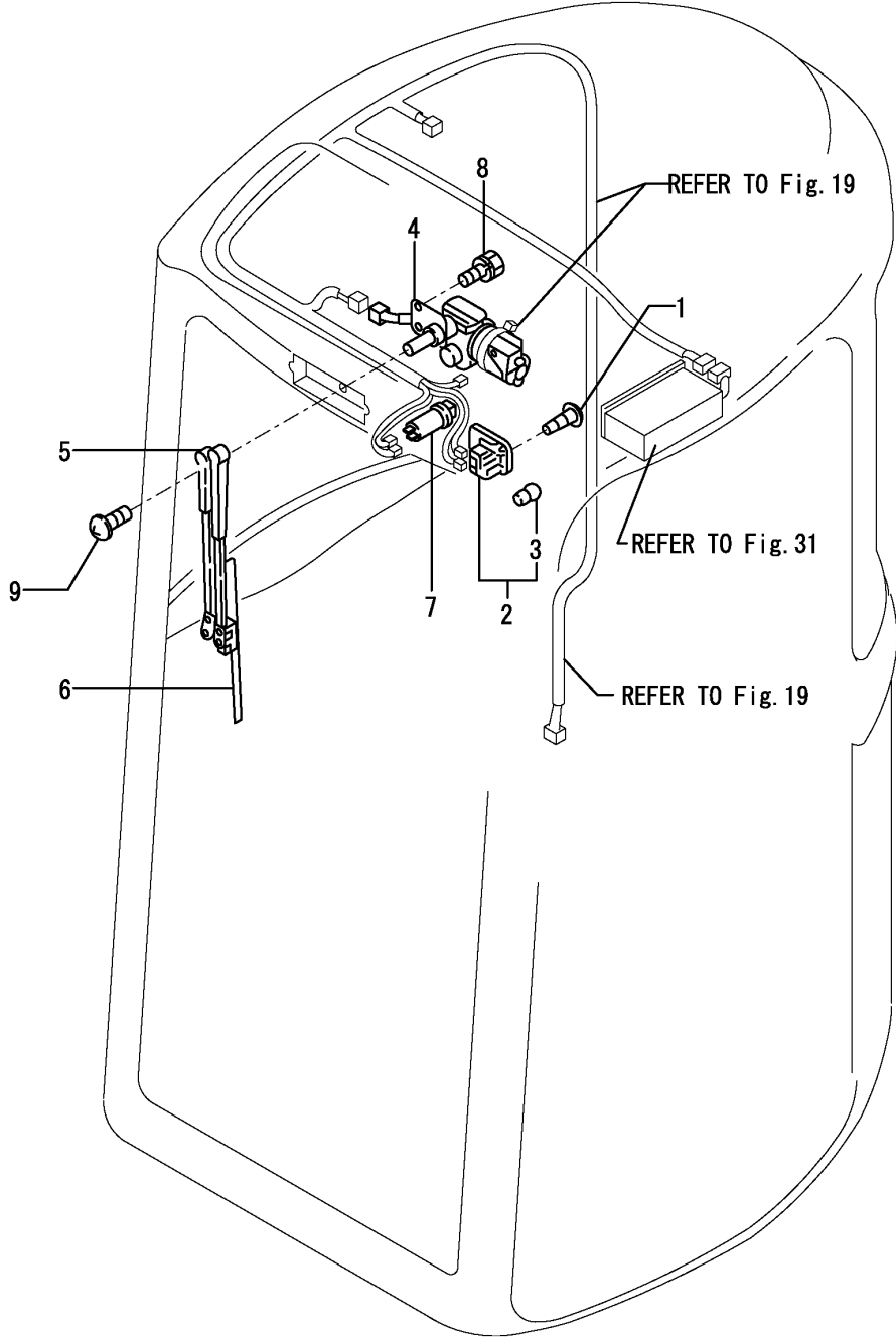
Fig.22. ELECTRIC PART(ROOMLANP,WIPER)
