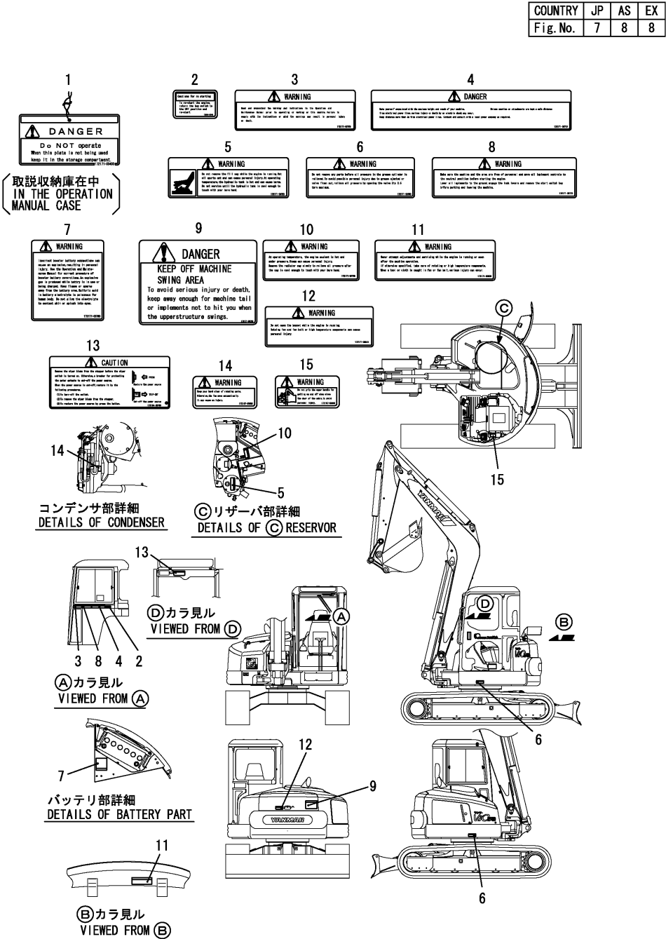
Fig.8. SAFETY LABEL(CABIN : AS,EX)
