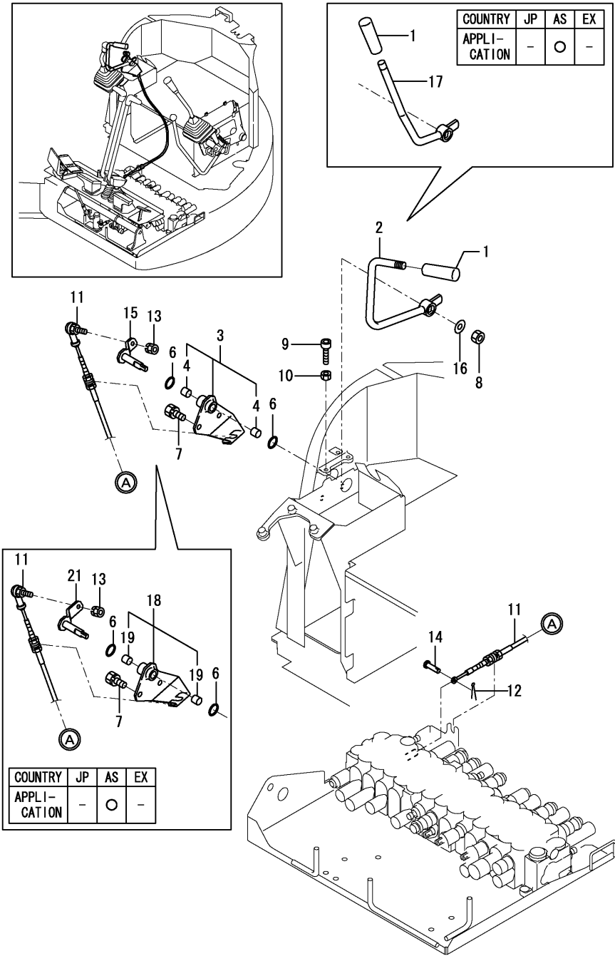
Fig.45. CONTROL EQUIPMENT(BLADE)
