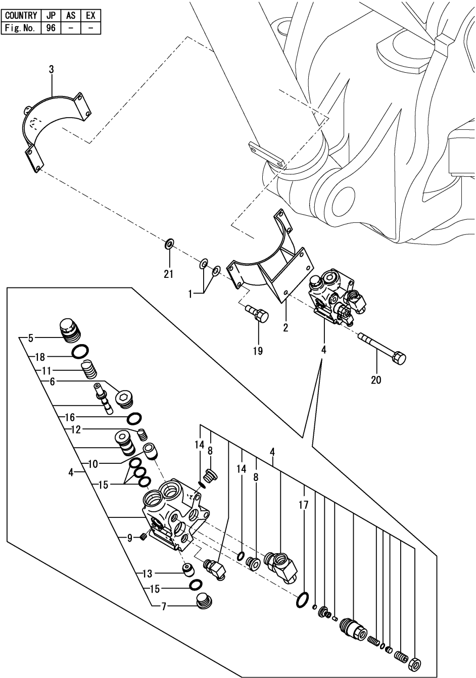
Fig.96. HOLD VALVE(CRANE:BOOM)
