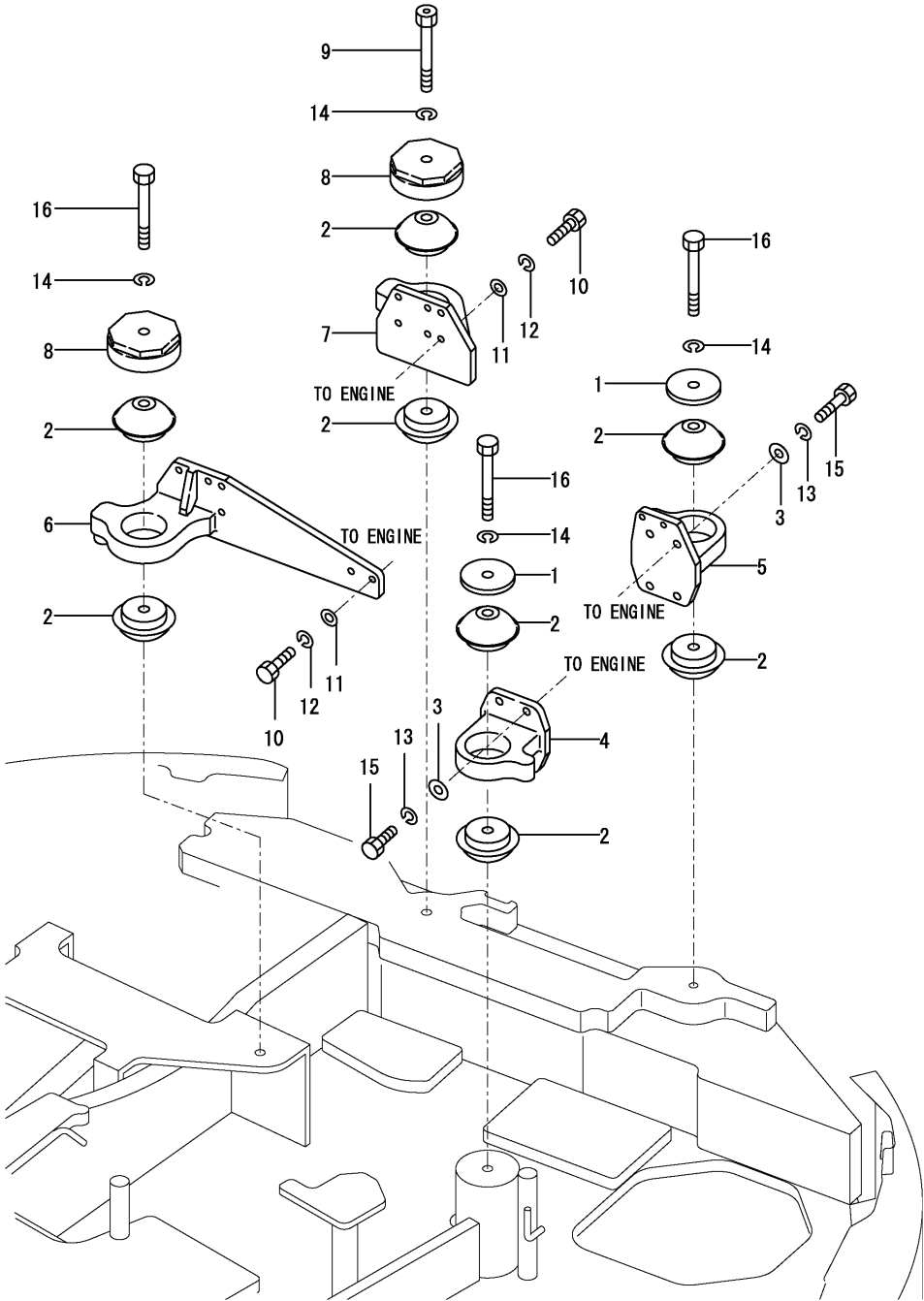
Fig.15. ENGINE MOUNT
