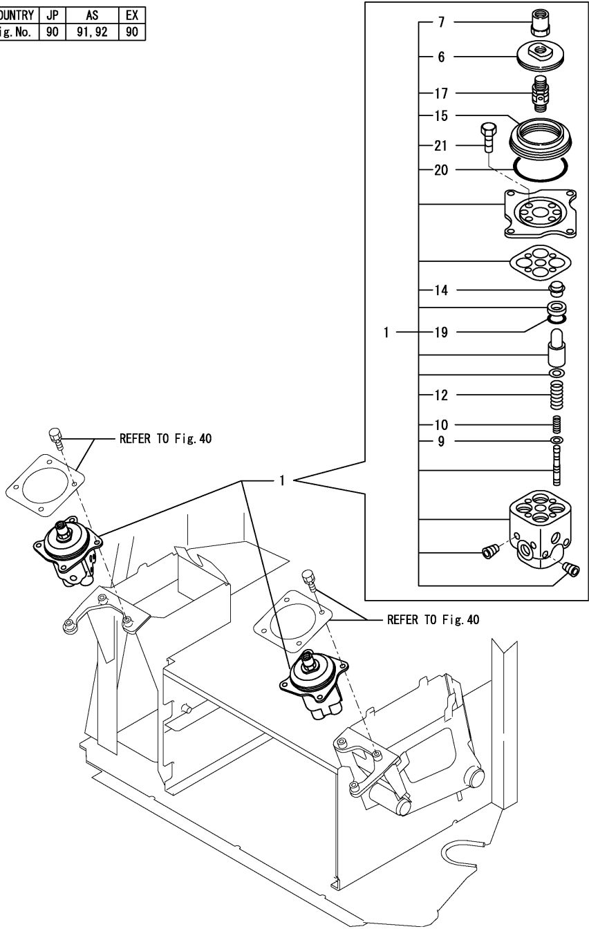
Fig.90. REMOTE CONTROL VALVE(JP,EX)
