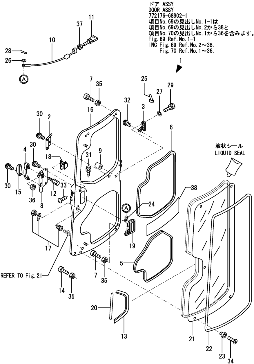
Fig.69. CABIN DOOR(BODY)
