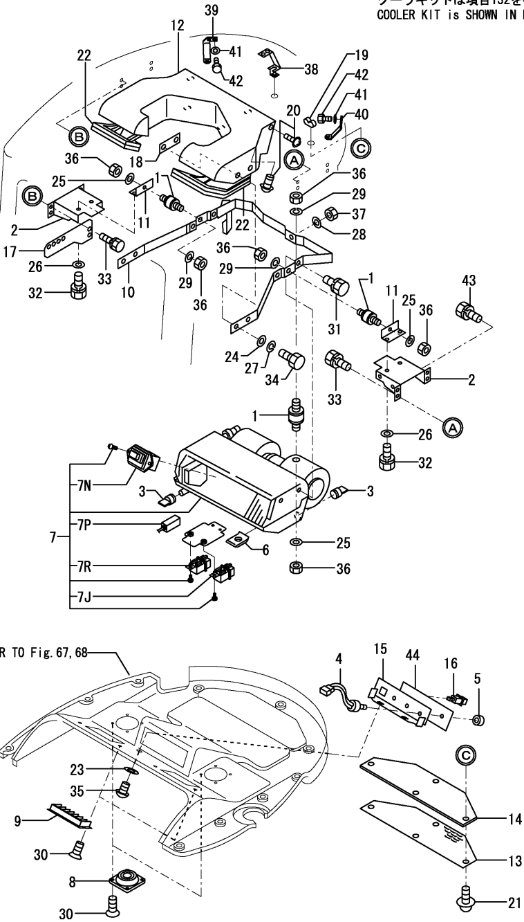
Fig.34. COOLER(CABIN RELATED)
