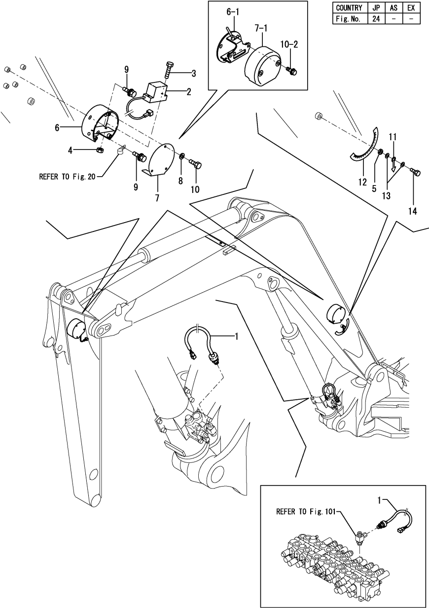
Fig.24. ELECRTC PART(CRANE : 2)
