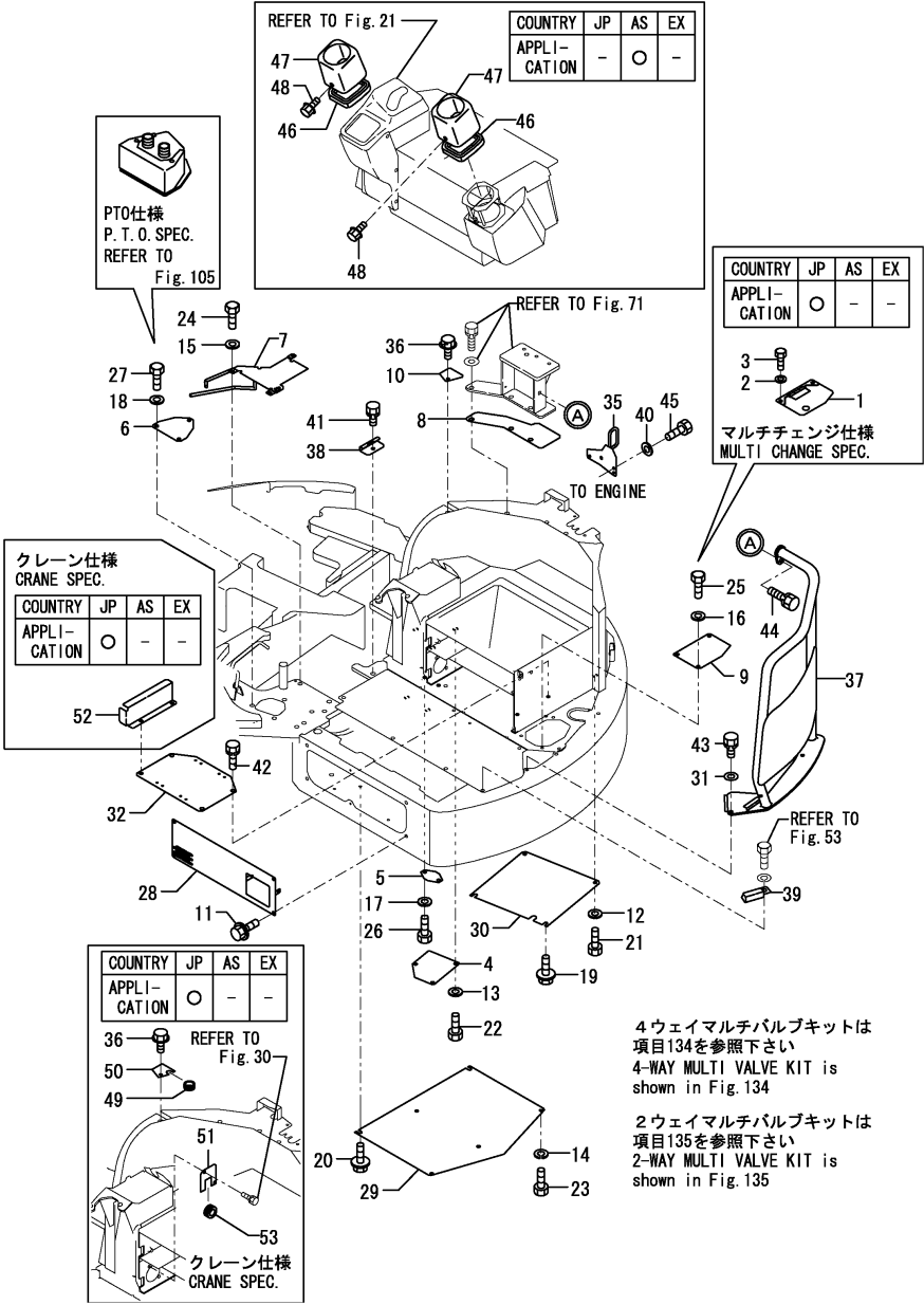
Fig.51. FRAME COVER(TURNING:CANOPY)
