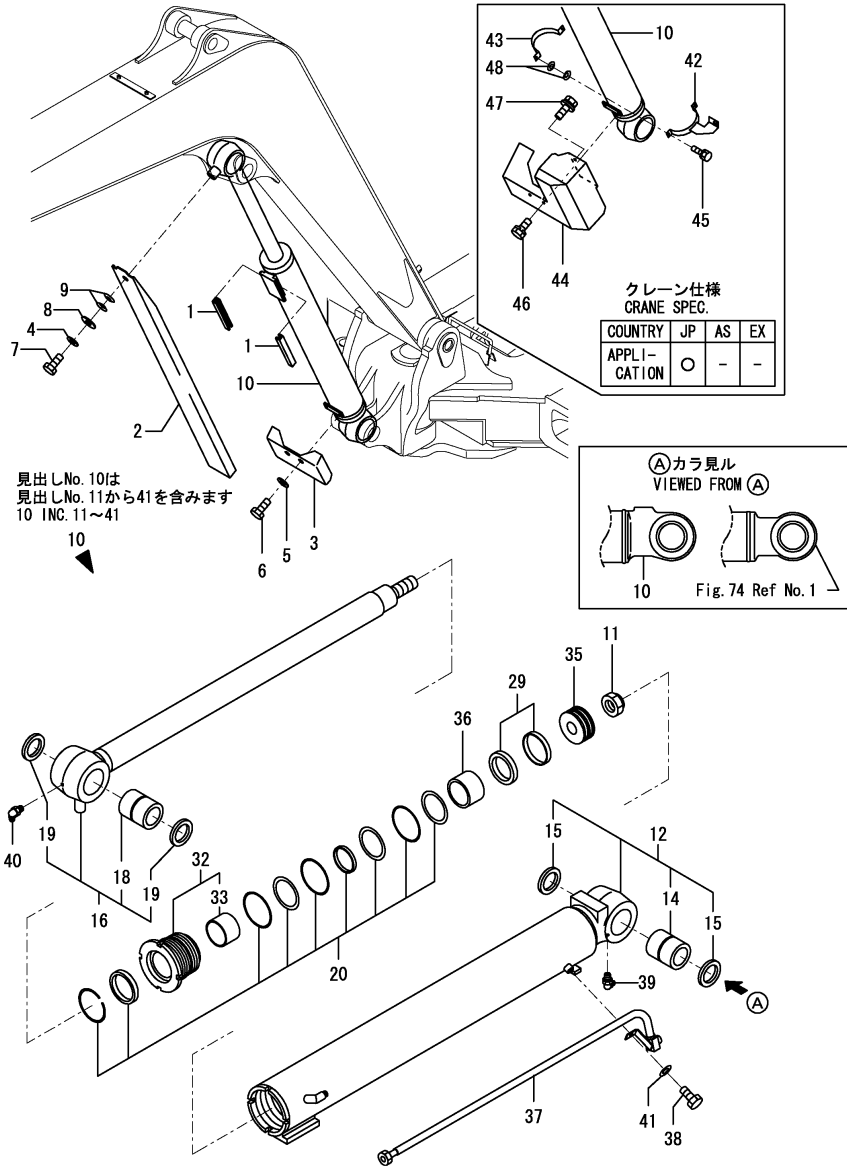
Fig.73. BOOM CYLINDER(PREVIOUS)
