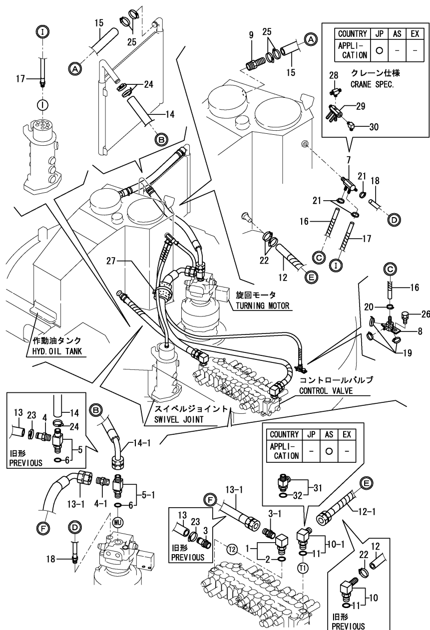
Fig.103. HYD. OIL PIPING(RETURN : 1)
