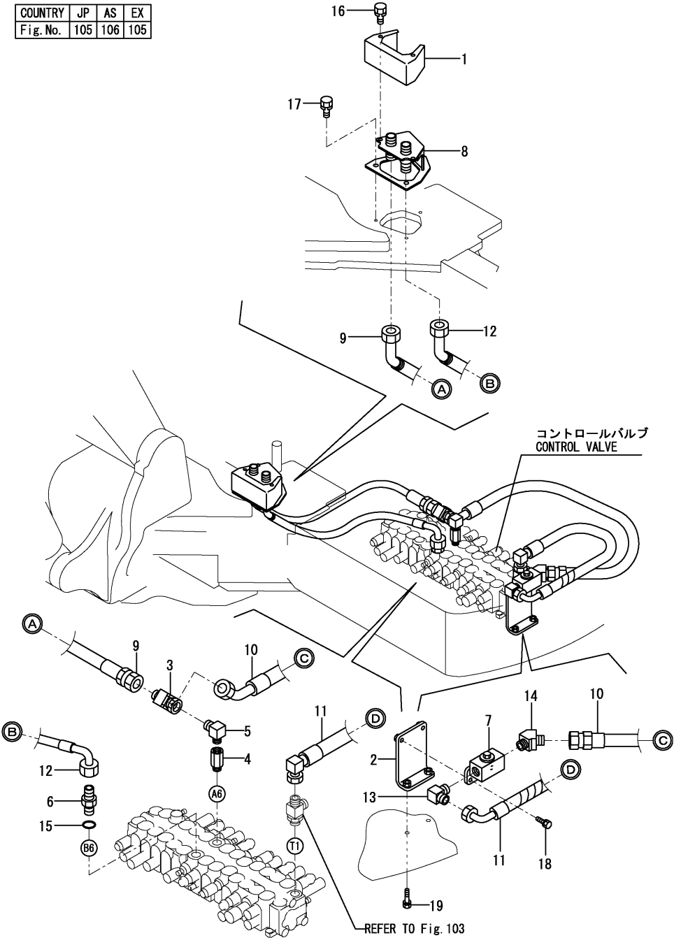
Fig.106. HYD. OIL PIPING(P.T.O.,FRAME END : AS SPEC.)
