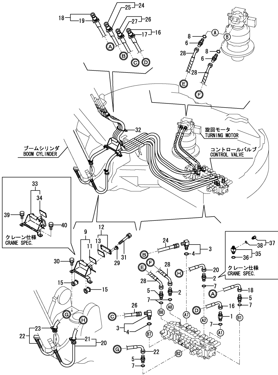
Fig.101. HYD. OIL PIPING(CONTROL VALVE - TURNING MOTOR,BOOM)
