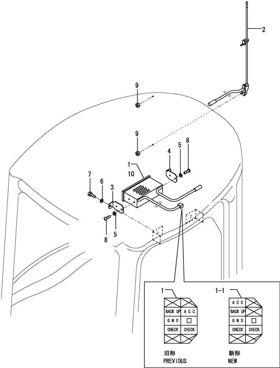
Fig.31. RADIO
