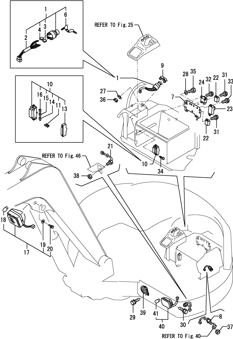
Fig.21. ELECTRIC PART(EQUIPMENT)
