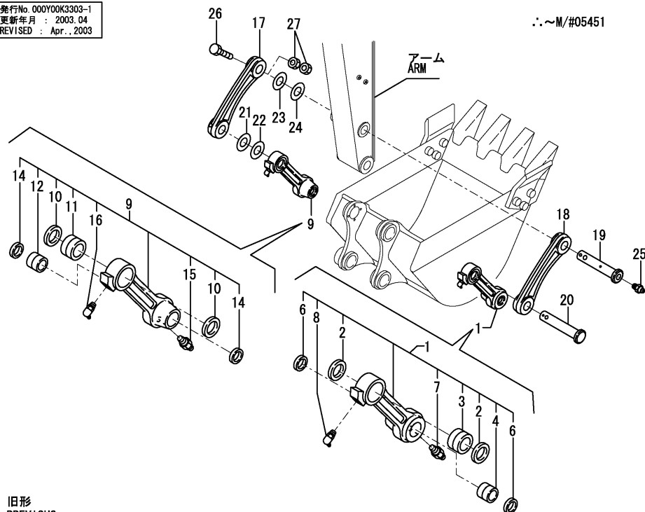
Fig.127. BUCKET ARM & LINK
