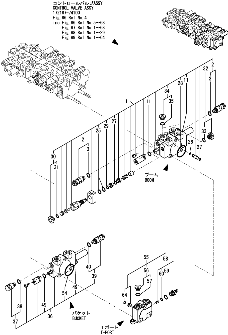
Fig.89. CONTROL VALVE(4)
