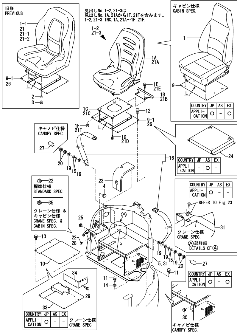
Fig.54. SEAT & SEAT MOUNT
