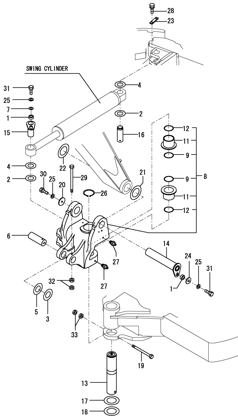
Fig.81. BOOM BRACKET
