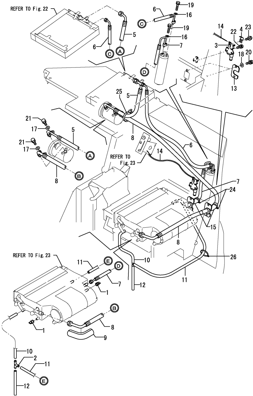
Fig.24. AIR CONDITIONER(PIPING)
