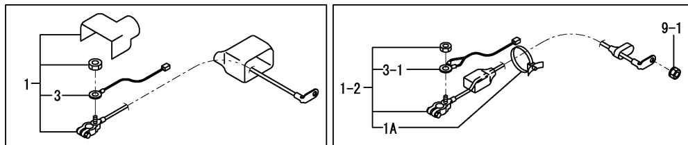
Fig.12. BATTERY
