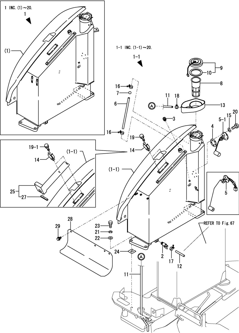
Fig.10. FUEL TANK
