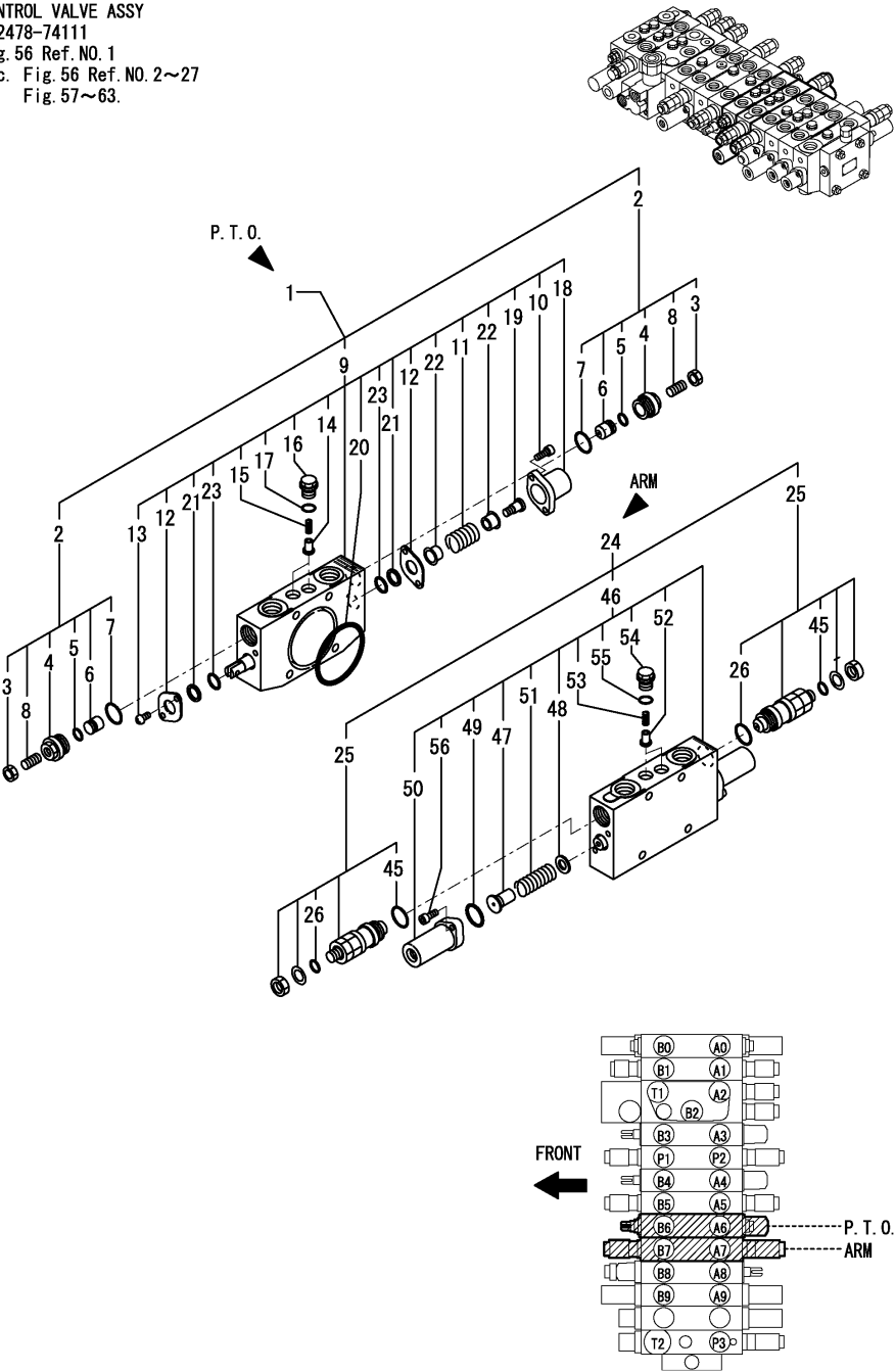
Fig.61. CONTROL VALVE(6/8)
