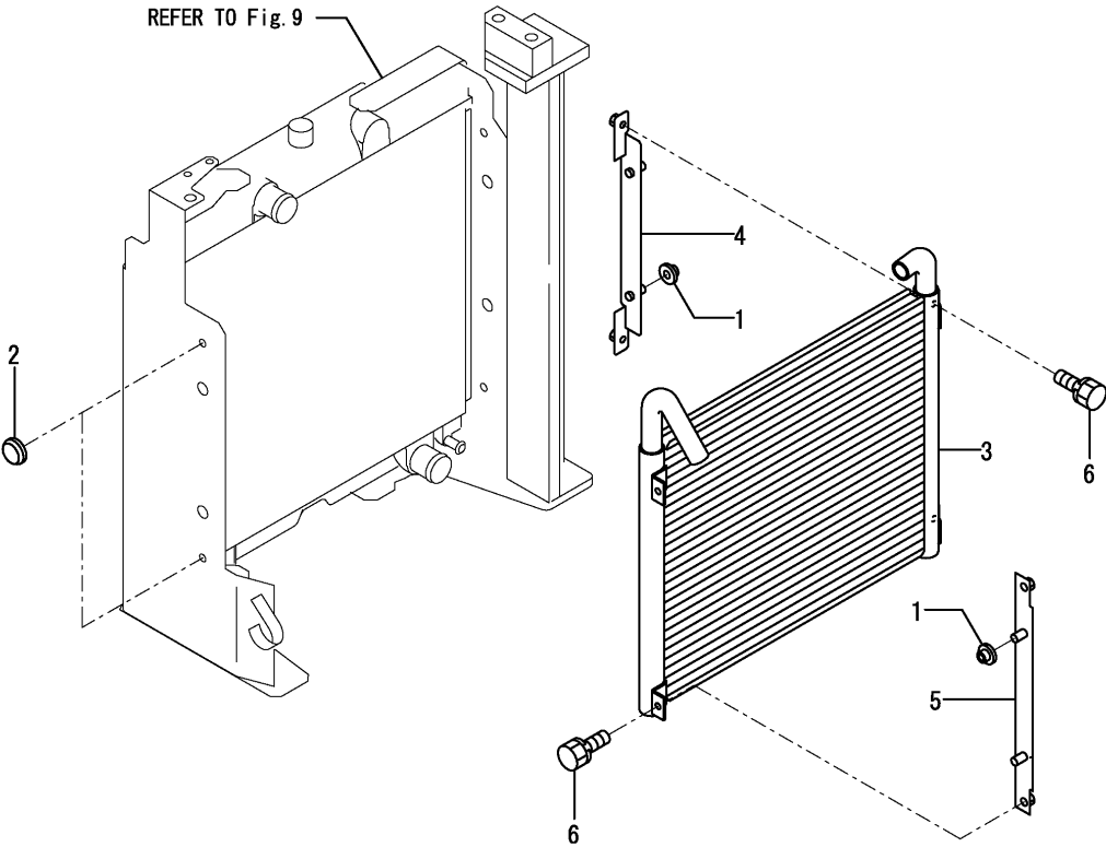
Fig.66. OIL COOLER
