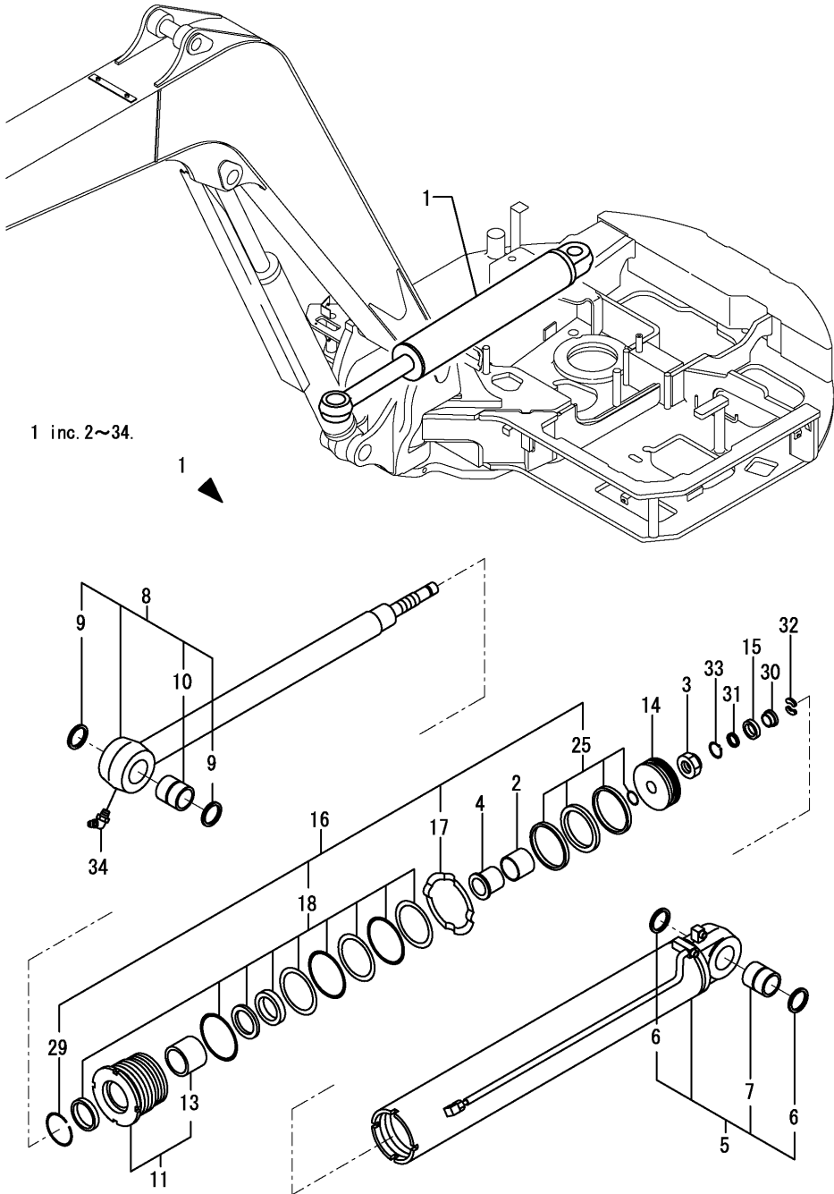
Fig.50. SWING CYLINDER
