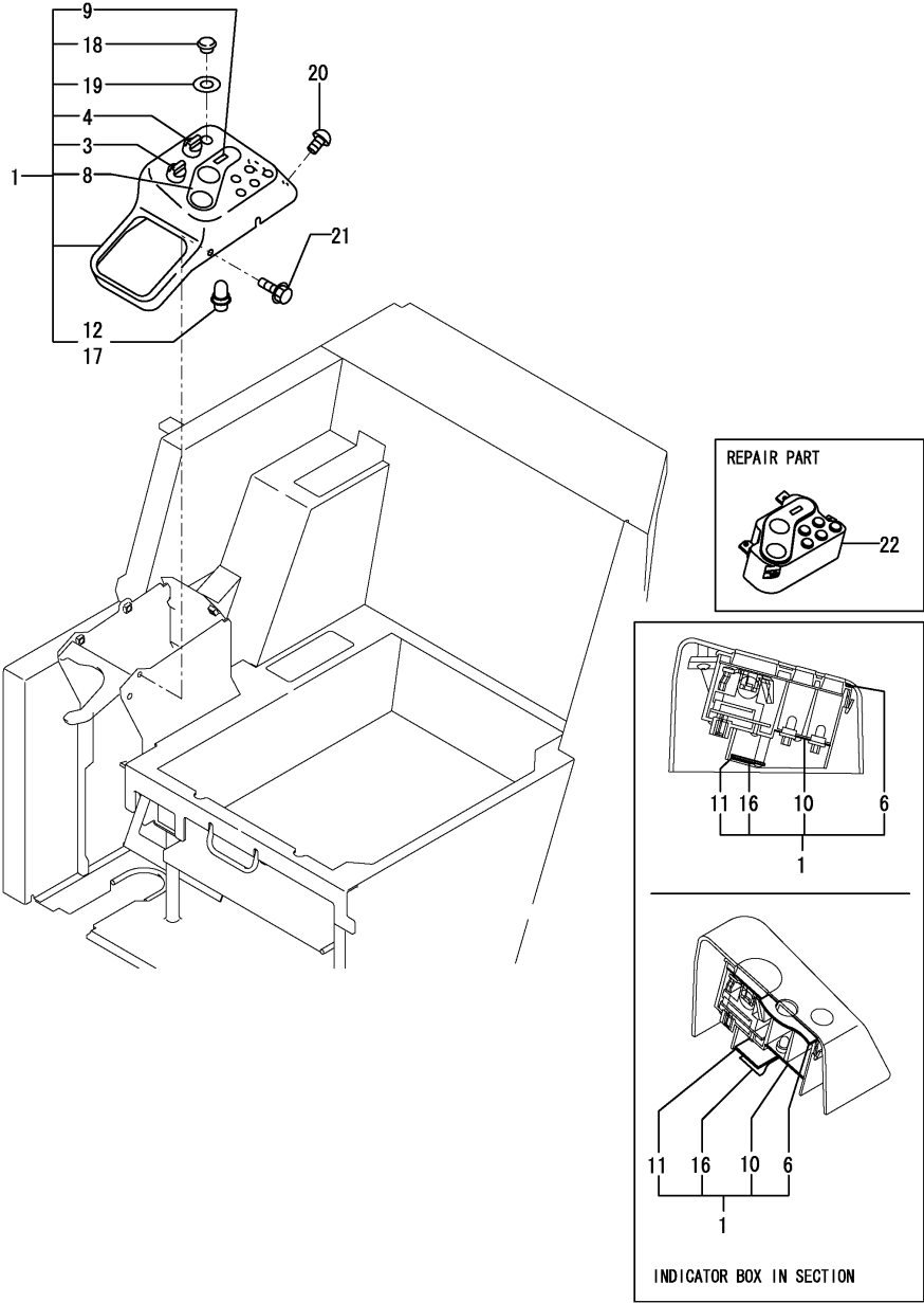
0CS10-M43501 ELECTRICAL PARTS Fig.18. INDICATOR BOX(TO M13433)
