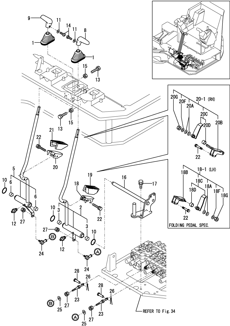
Fig.29. TRAVEL
