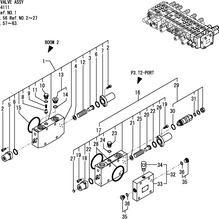
Fig.63. CONTROL VALVE(8/8)
