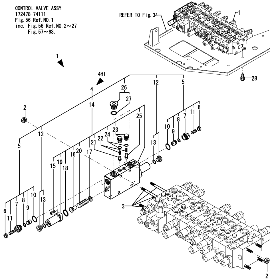
Fig.56. CONTROL VALVE(1/8)
