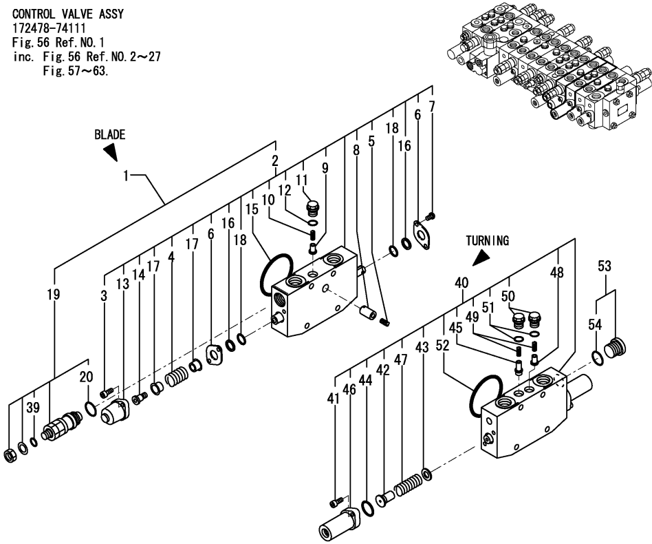
Fig.62. CONTROL VALVE(7/8)
