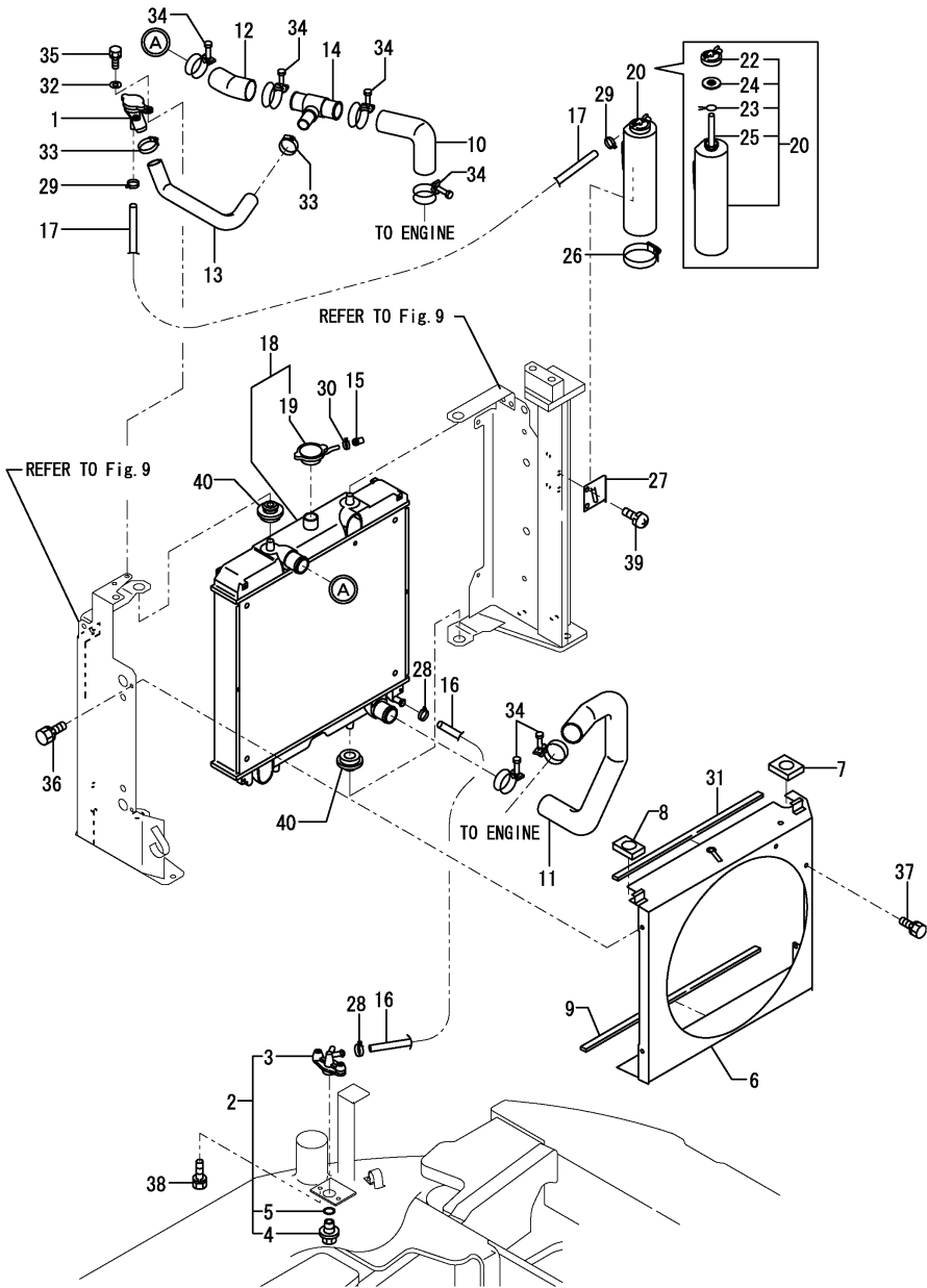
OCS10-M43501 ENGINE RELATED Fig.8. RADIATOR & SUB TANK
