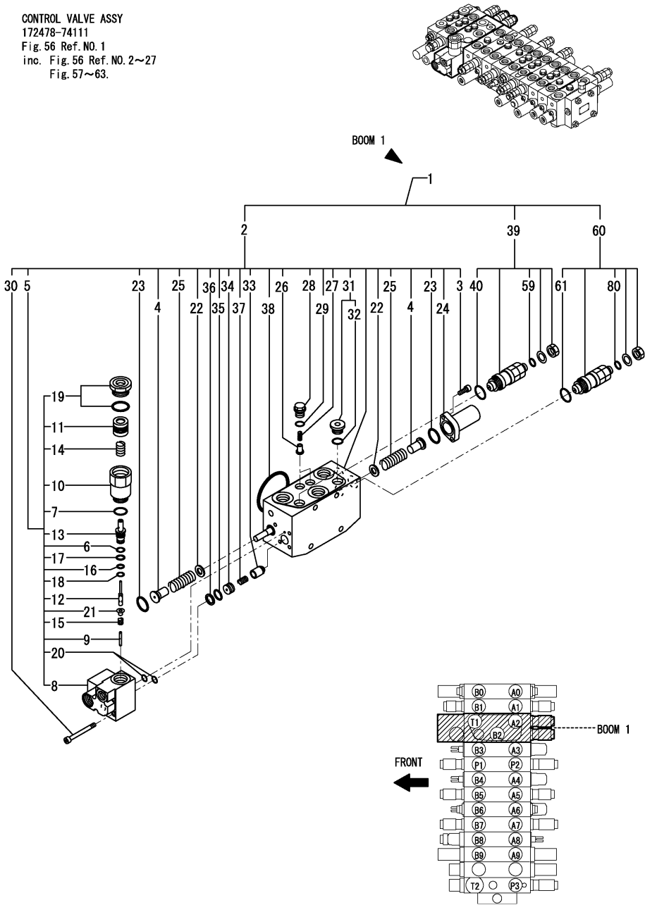
Fig.58. CONTROL VALVE(3/8)
