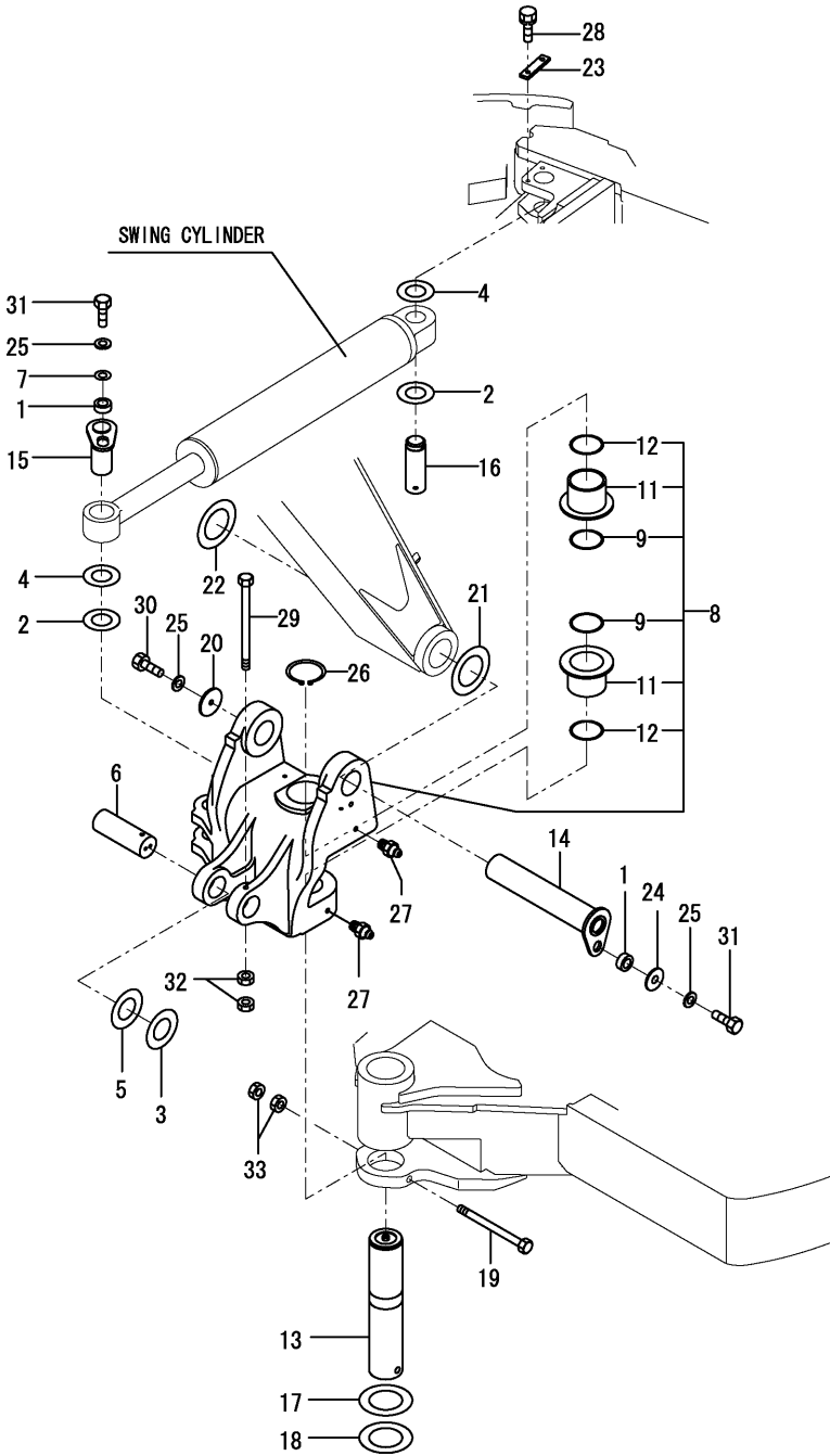
Fig.86. BOOM BRACKET
