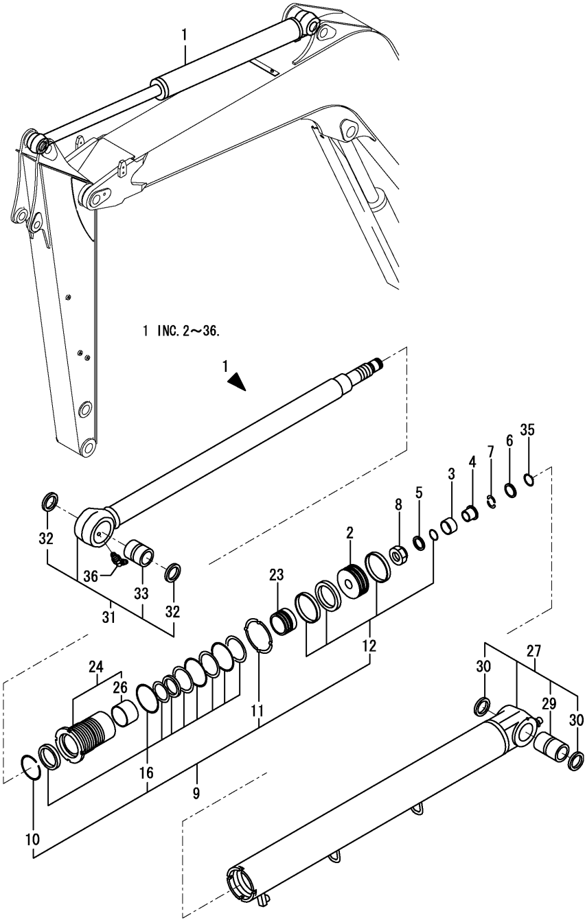
Fig.53. ARM CYLINDER
