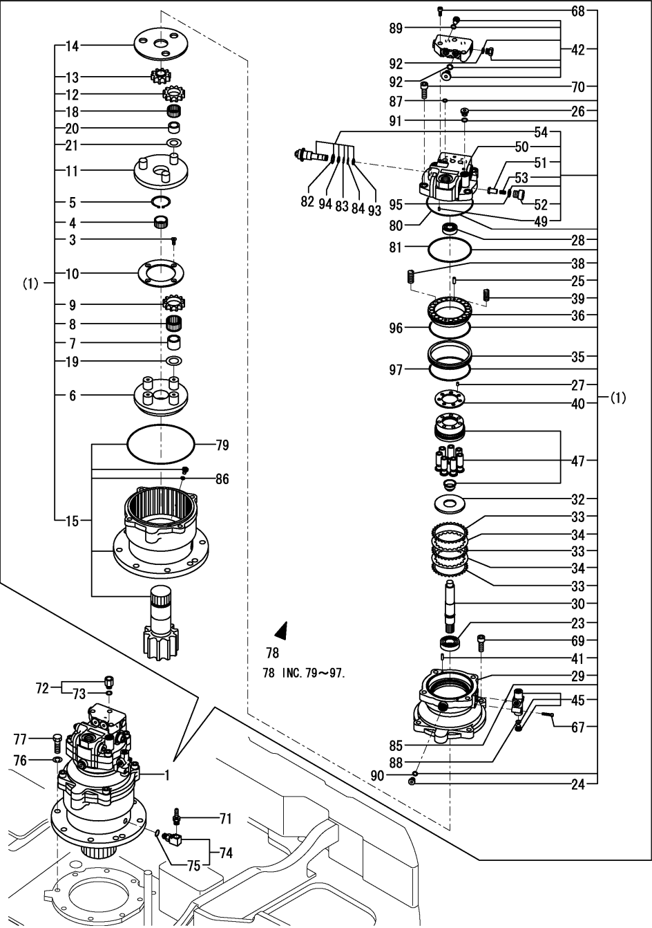
Fig.59. TURNING MOTOR
