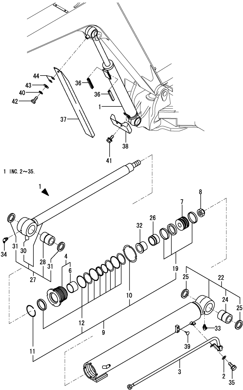
Fig.52. BOOM CYLINDER
