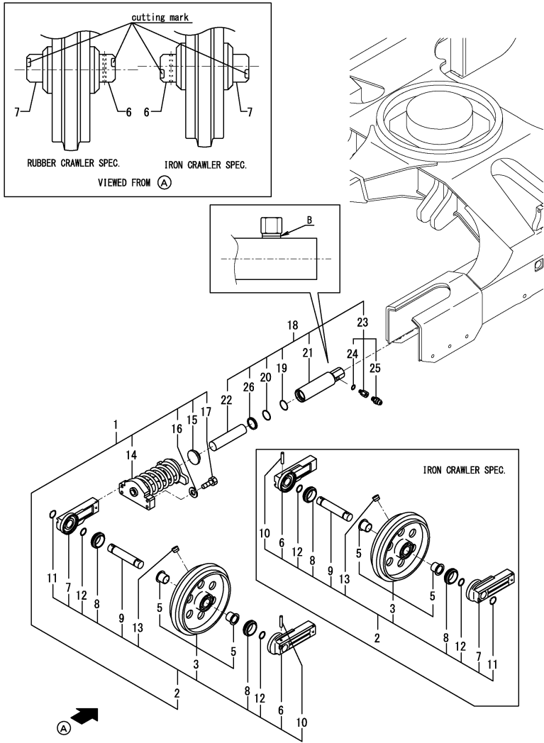
Fig.26. IDLER & ADJUST
