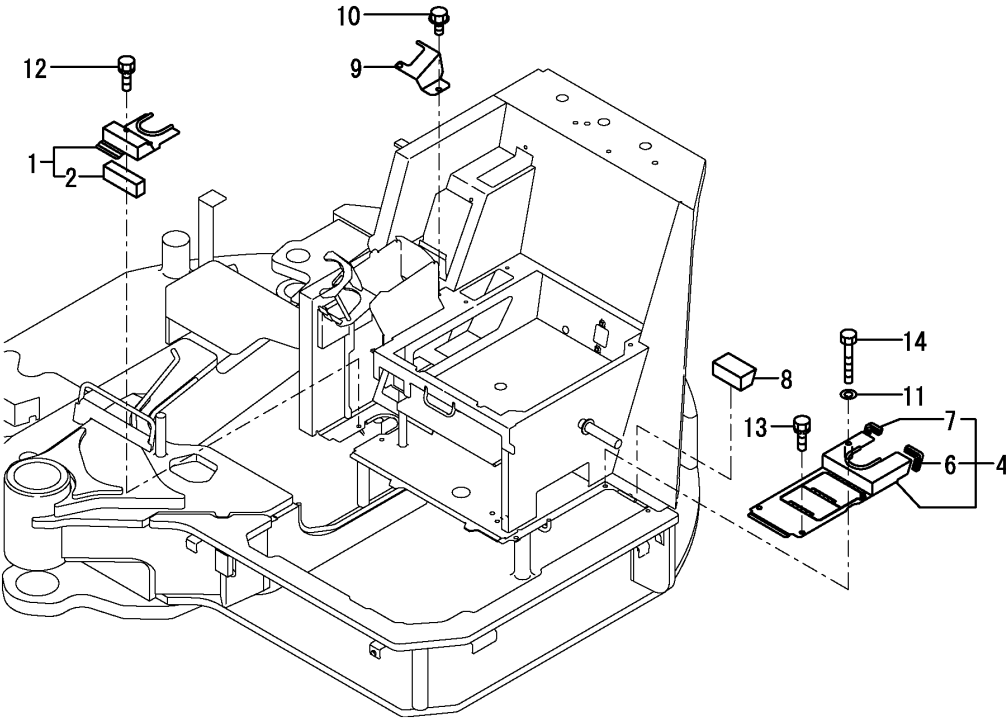
Fig.37. COVER(AROUND THE CONTROL)
