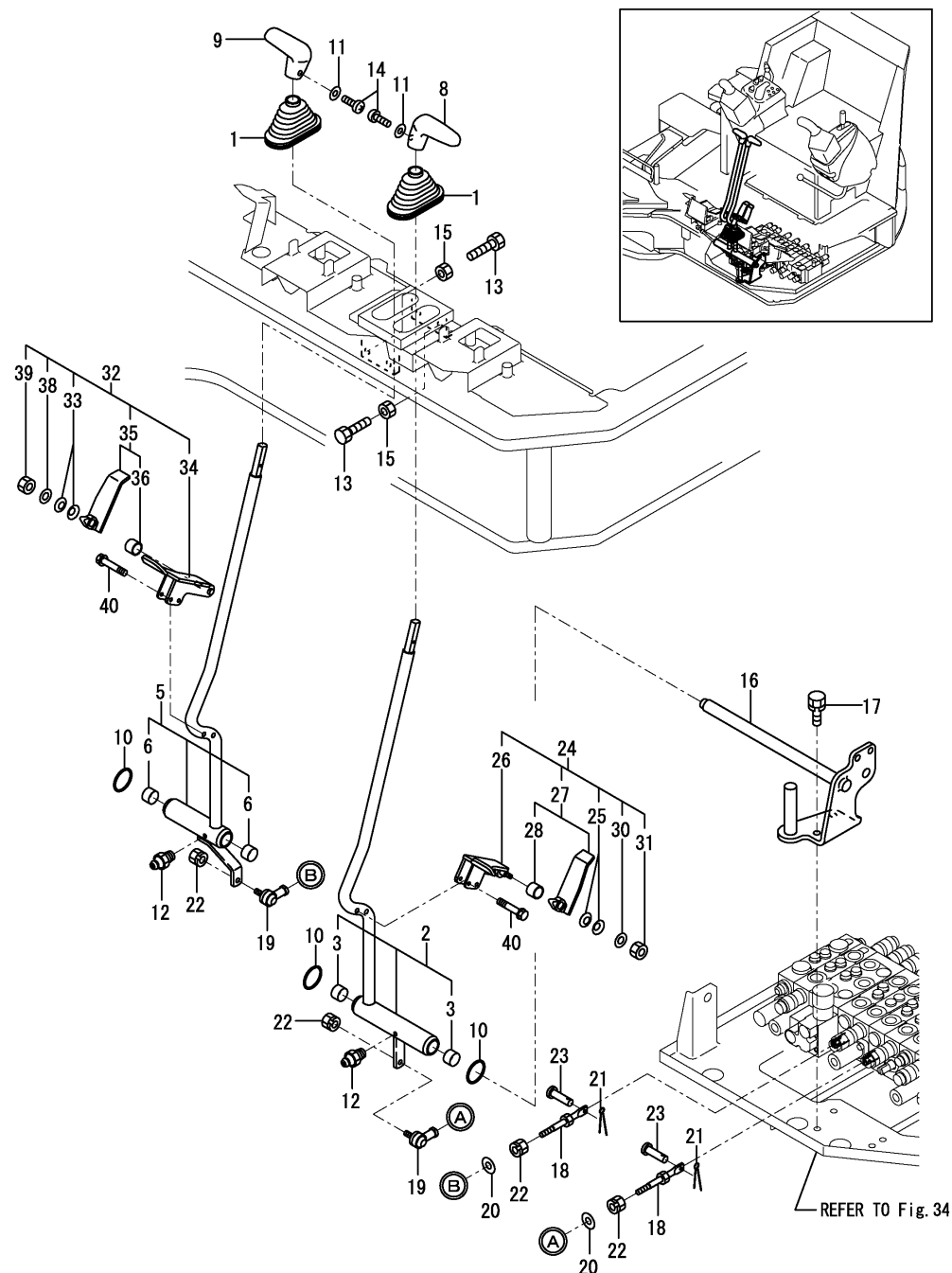
Fig.29. CONTROL EQUIPMENT(TRAVEL)
