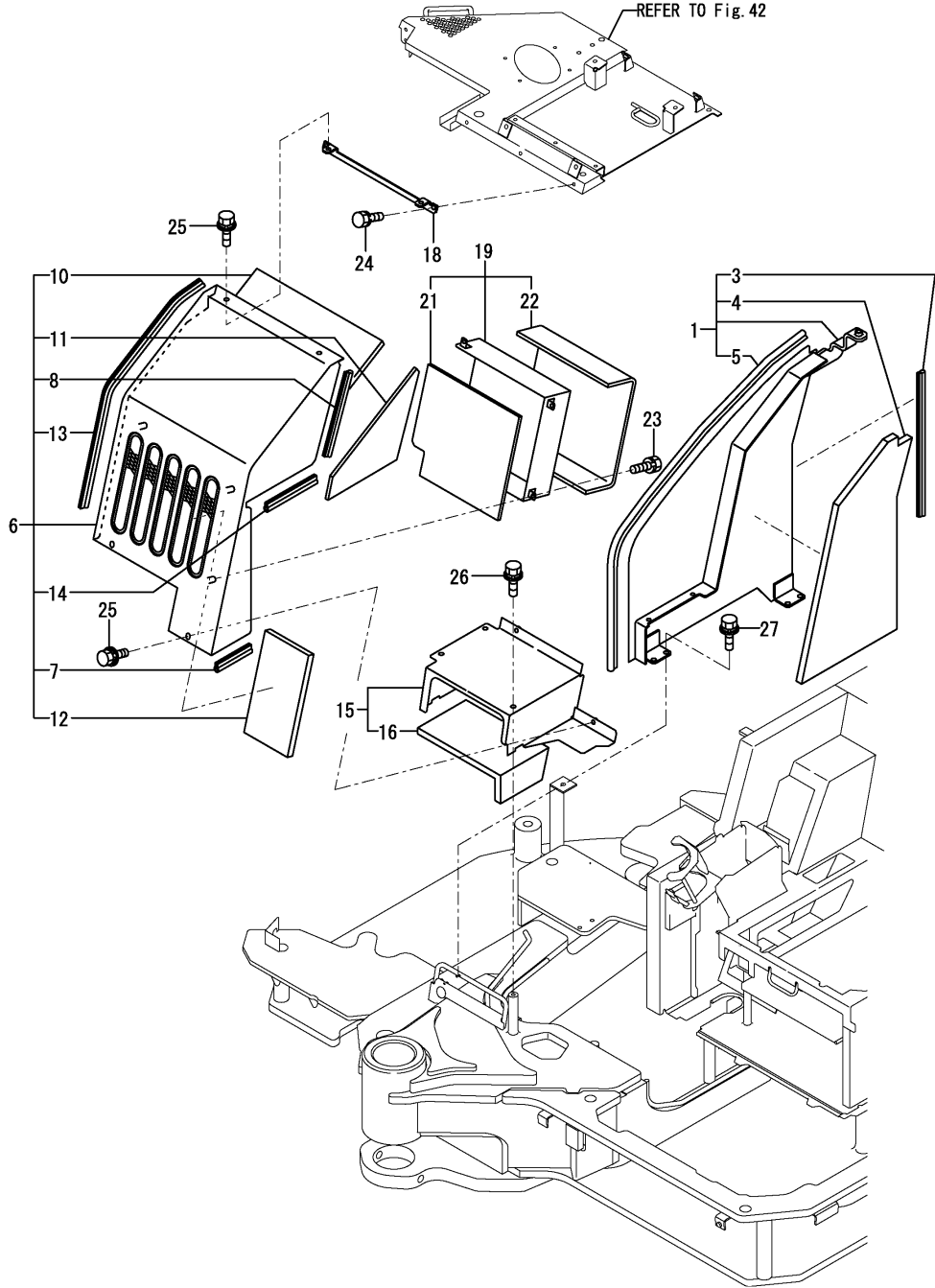
Fig.44. HOOD(FRONT)
