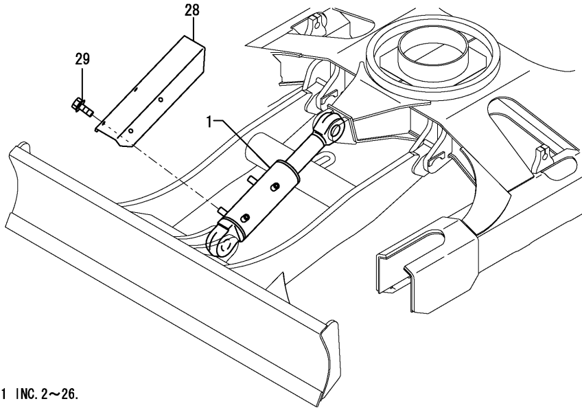
Fig.56. BLADE CYLINDER
