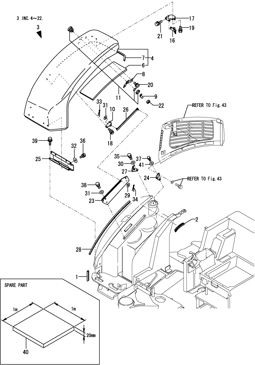
Fig.41. HOOD(BODY)
