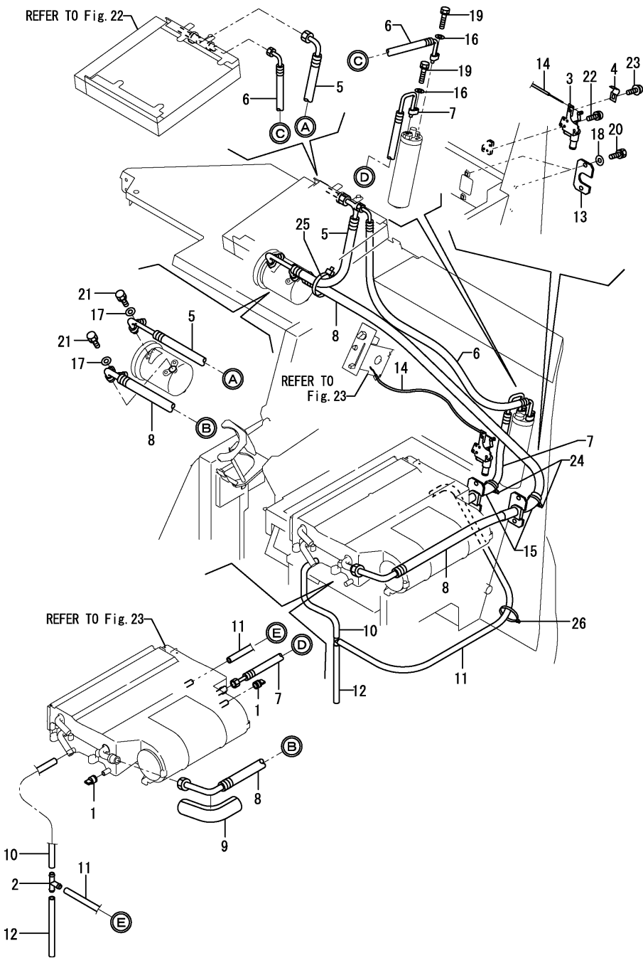
Fig.24. AIR CONDITIONER(PIPING)
