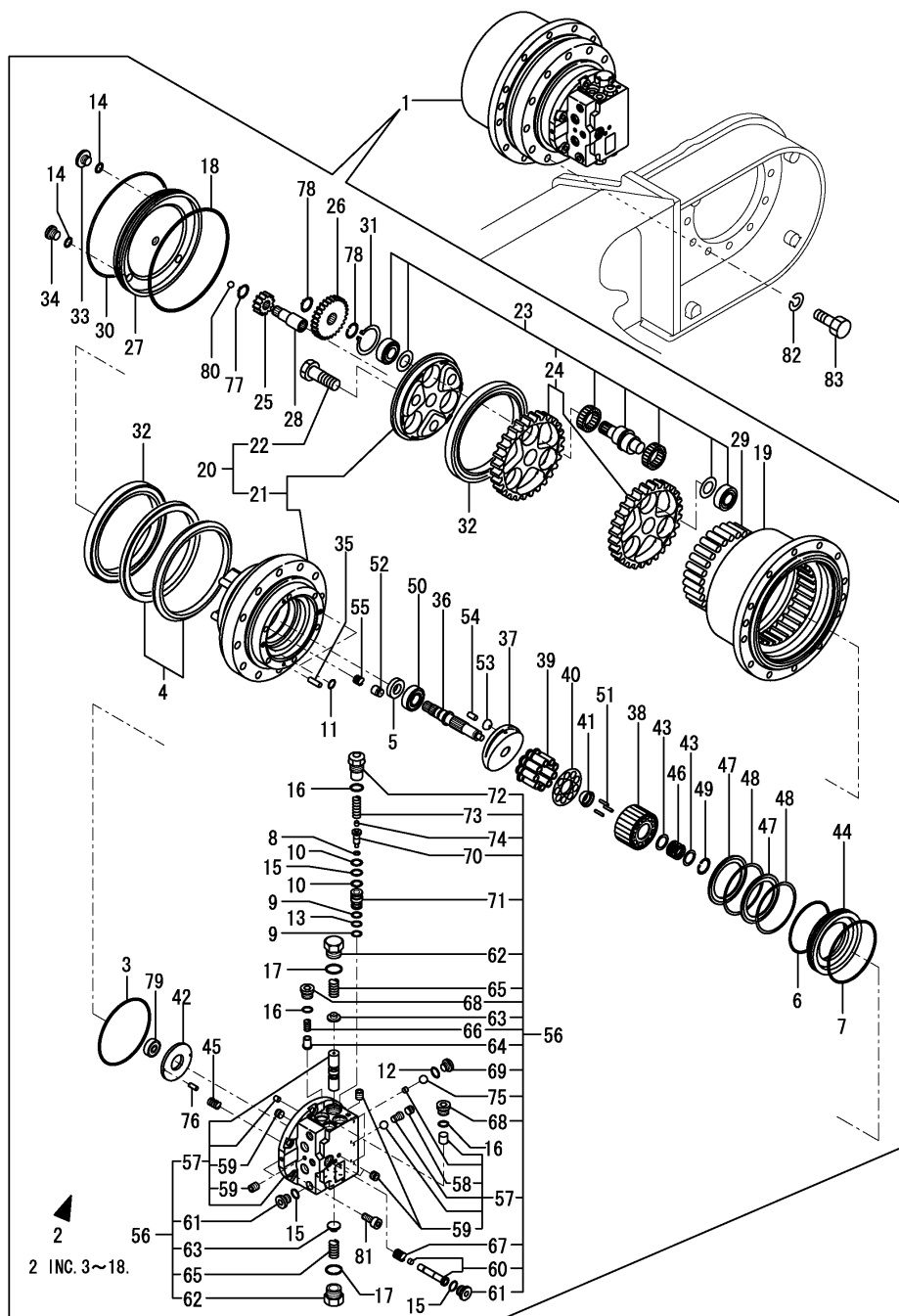
Fig.58. TRAVEL MOTOR(TO M15128)
