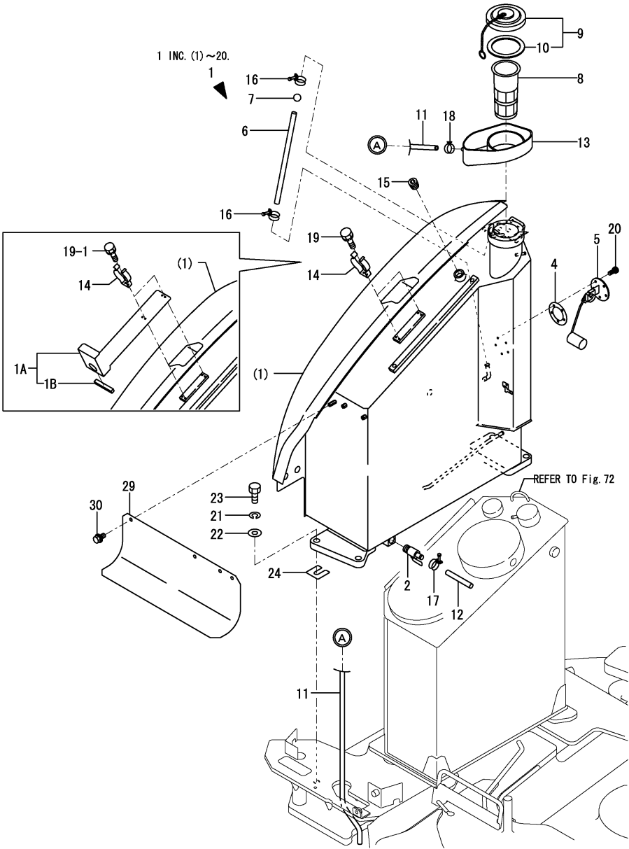
Fig.10. FUEL TANK
