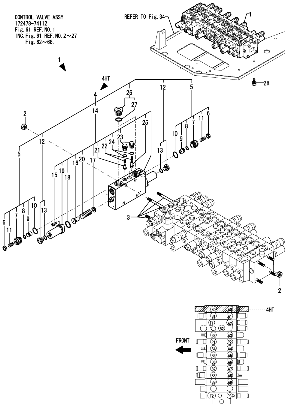
Fig.61. CONTROL VALVE(1/8)
