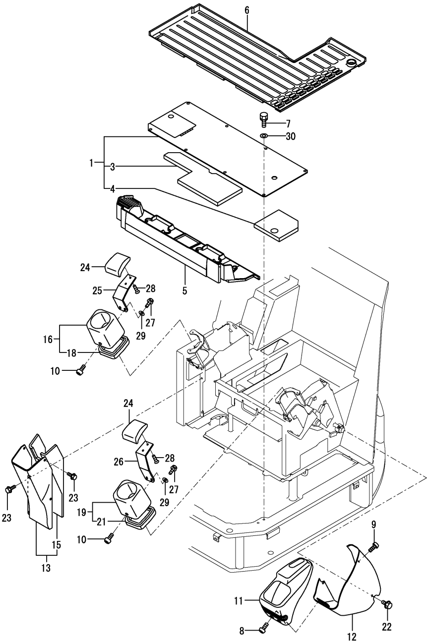
Fig.39. STEP & INSTRUMENT PANEL
