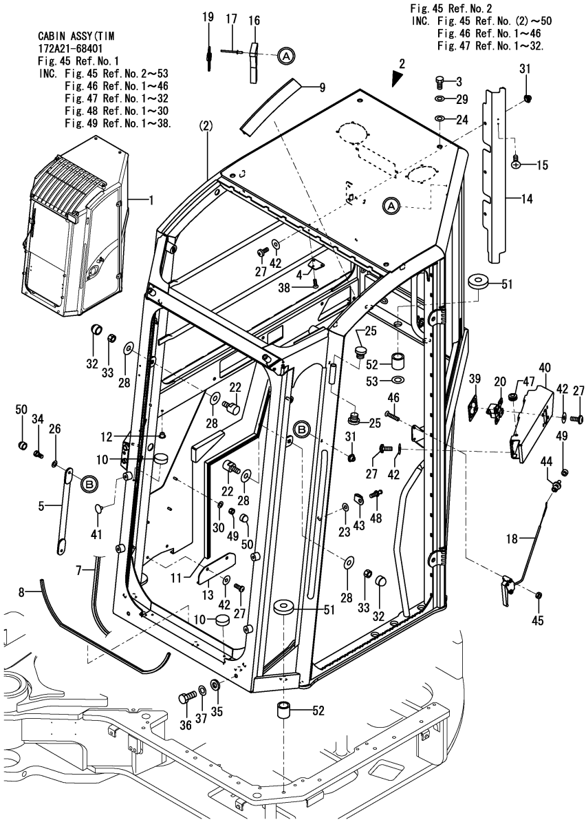
Fig.45. TIM CABIN(BODY, ACCESSORY)
