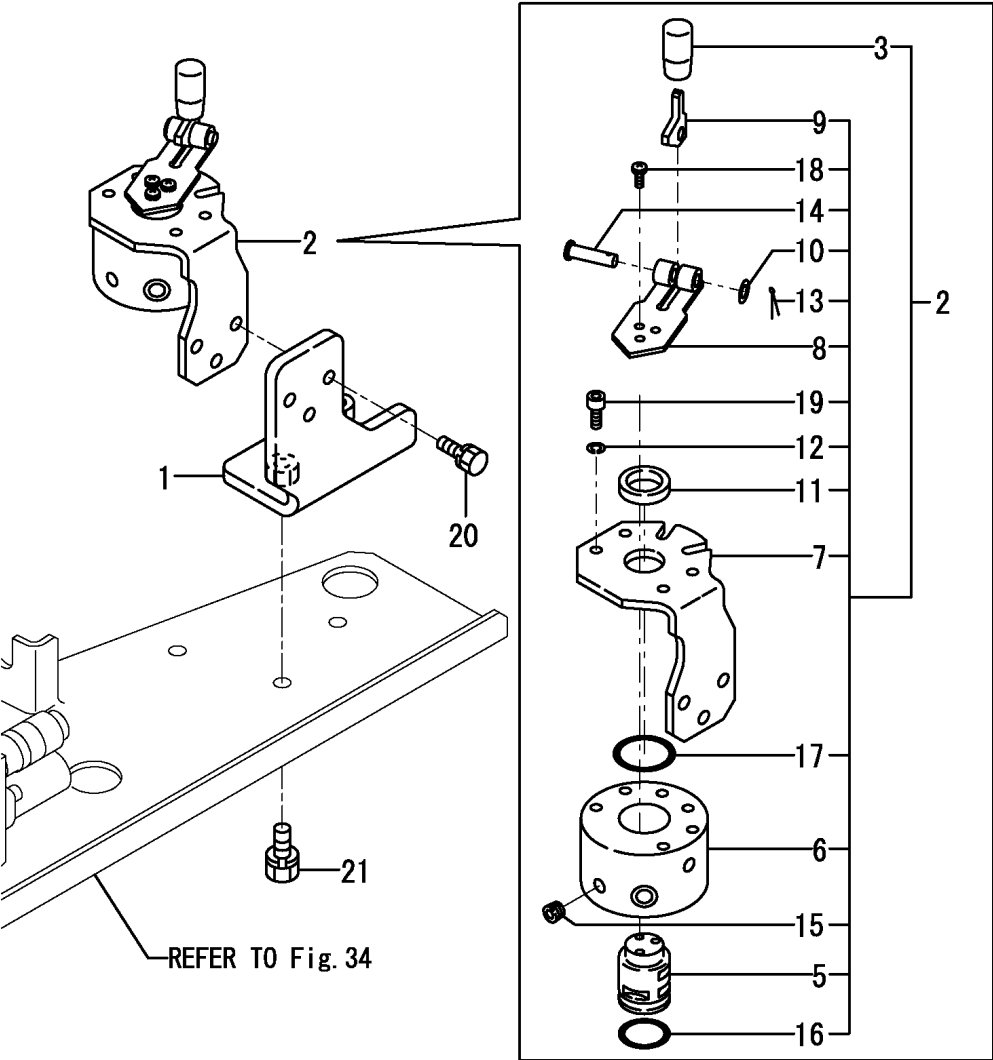
Fig.69. 2-WAY VALVE
