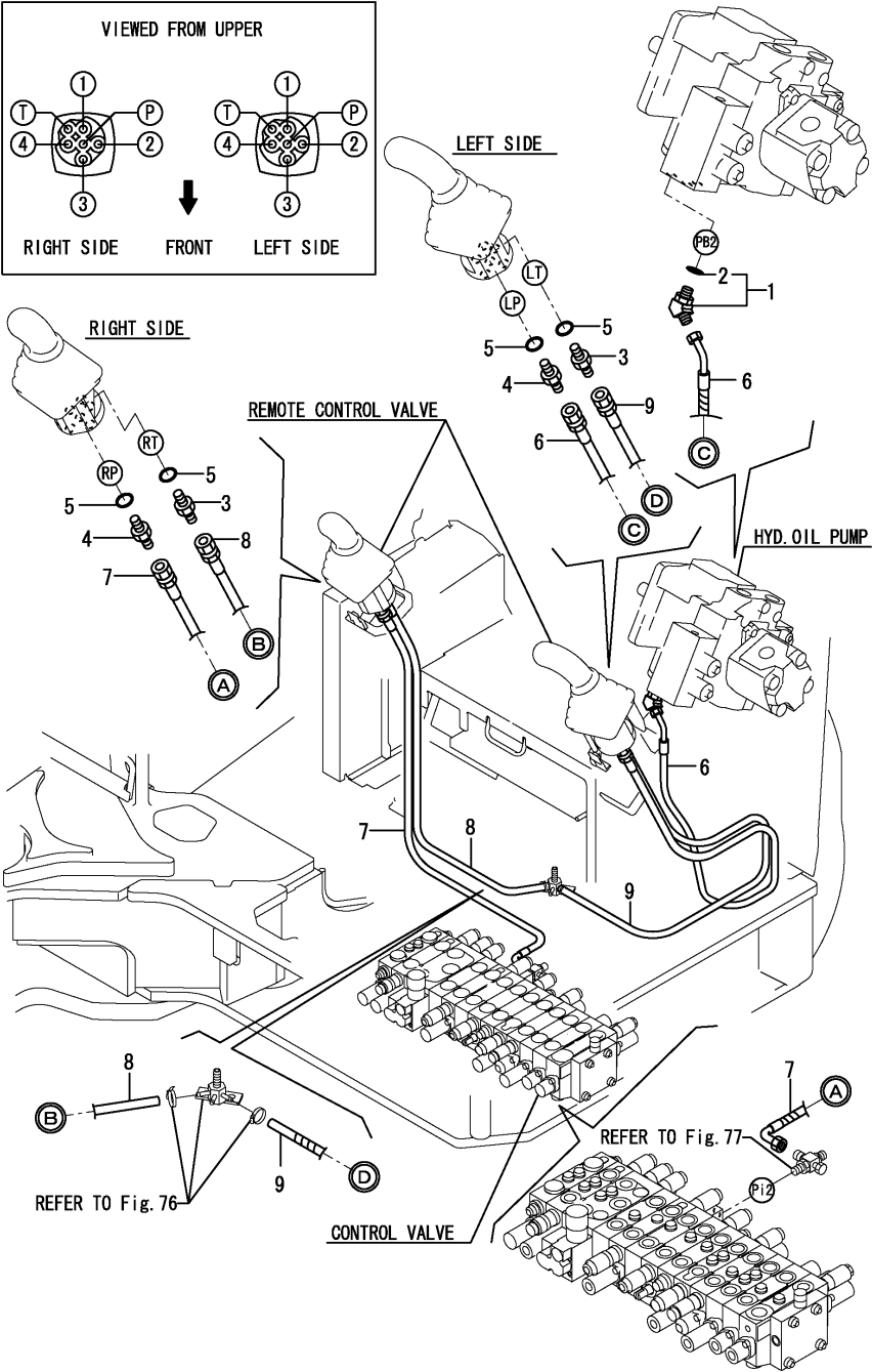
Fig.83. CONTROL PIPING(RETURN)
