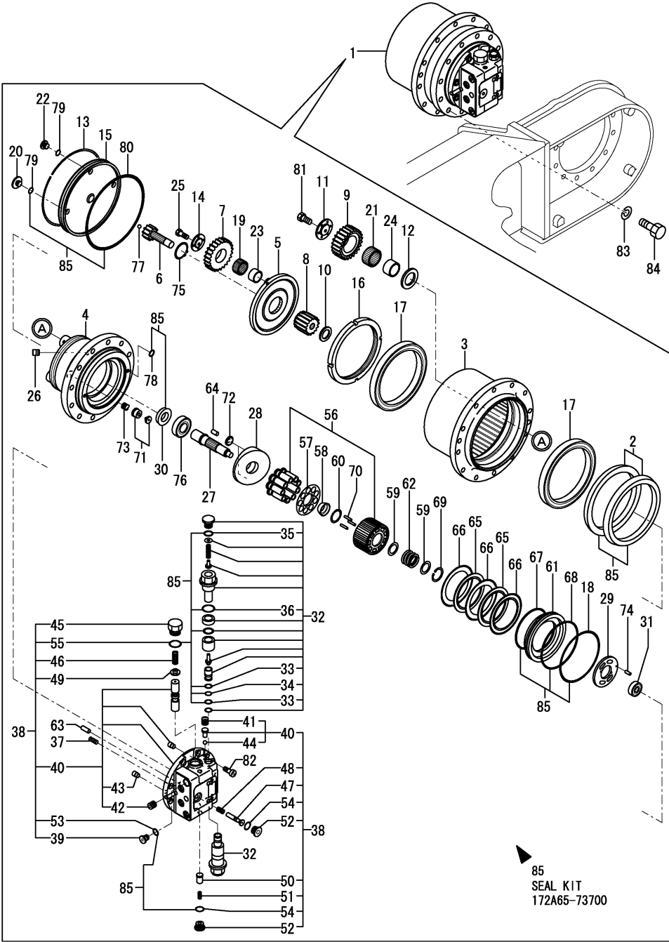
Fig.93. (58A)TRAVEL MOTOR(FROM M15129)
