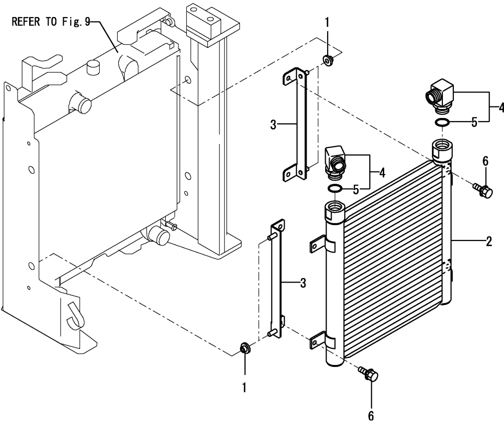
Fig.71. OIL COOLER
