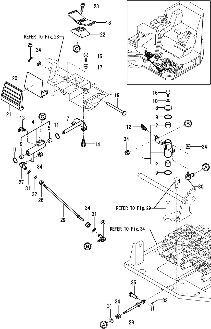
Fig.31. CONTROL EQUIPMENT(SWING PEDAL)
