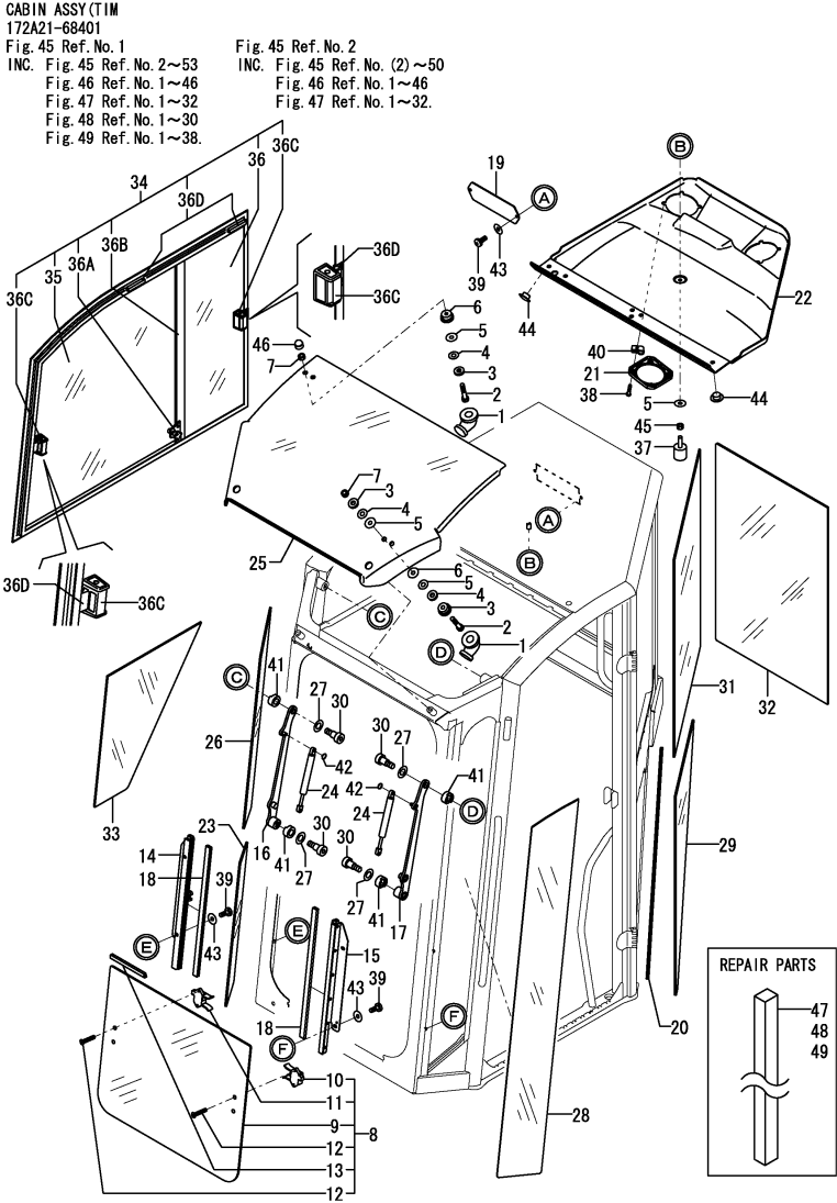
Fig.46. TIM CABIN(GLASS)
