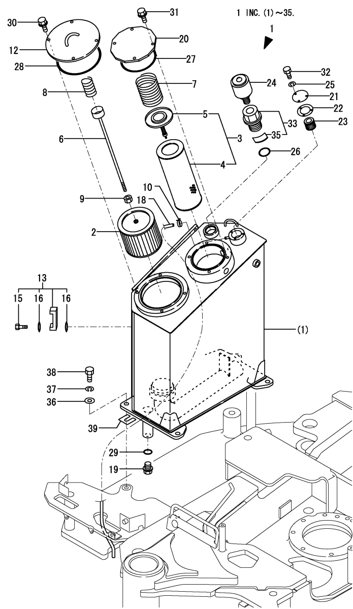
Fig.72. HYD.OIL TANK
