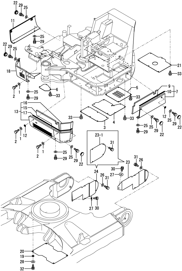
OCS10-M53500 COVER Fig.36. COVER(FRAME)
