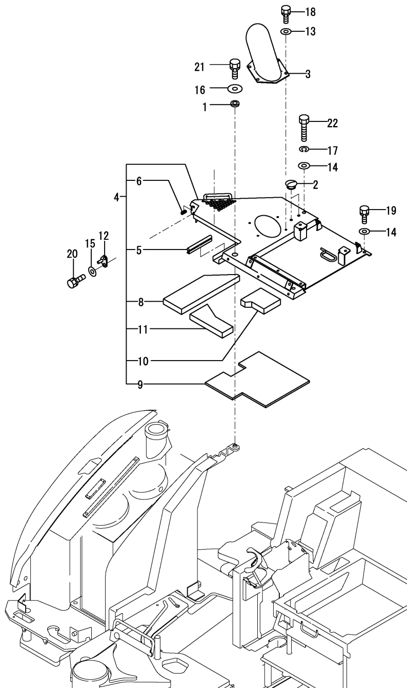
Fig.42. HOOD(UPPER COVER)
