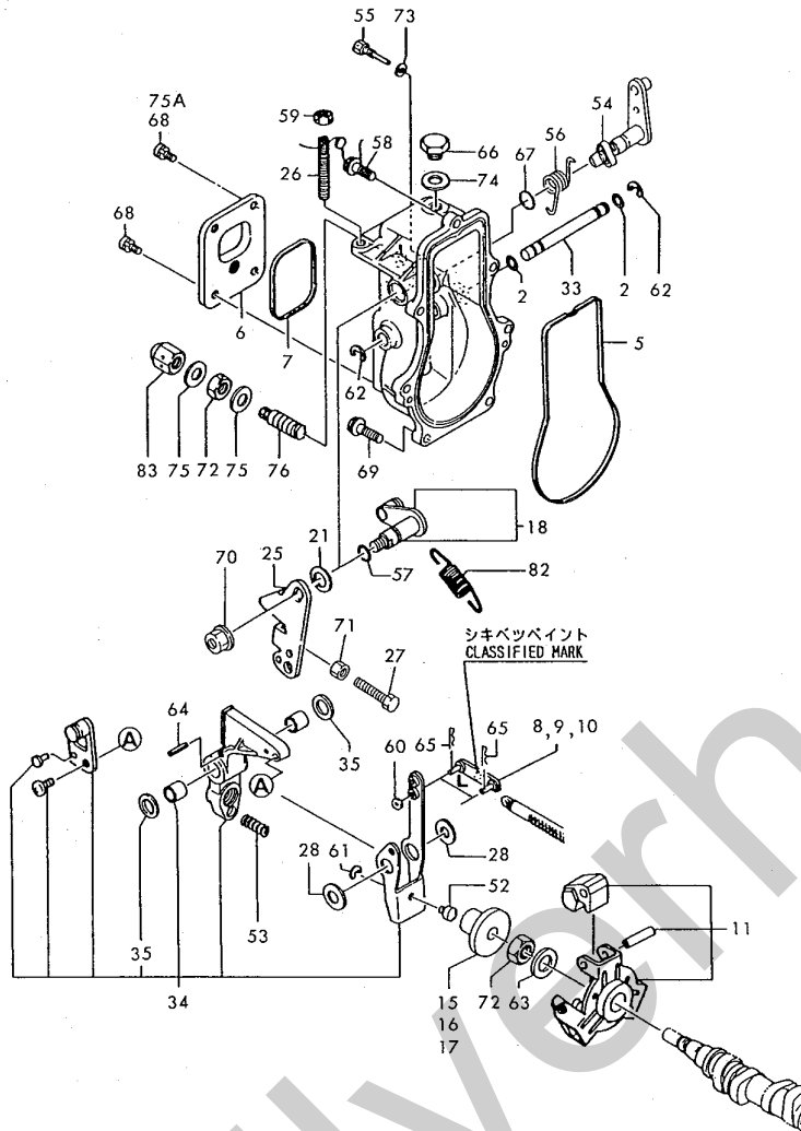
Fig. 16 ガバナ GOVERNOR
