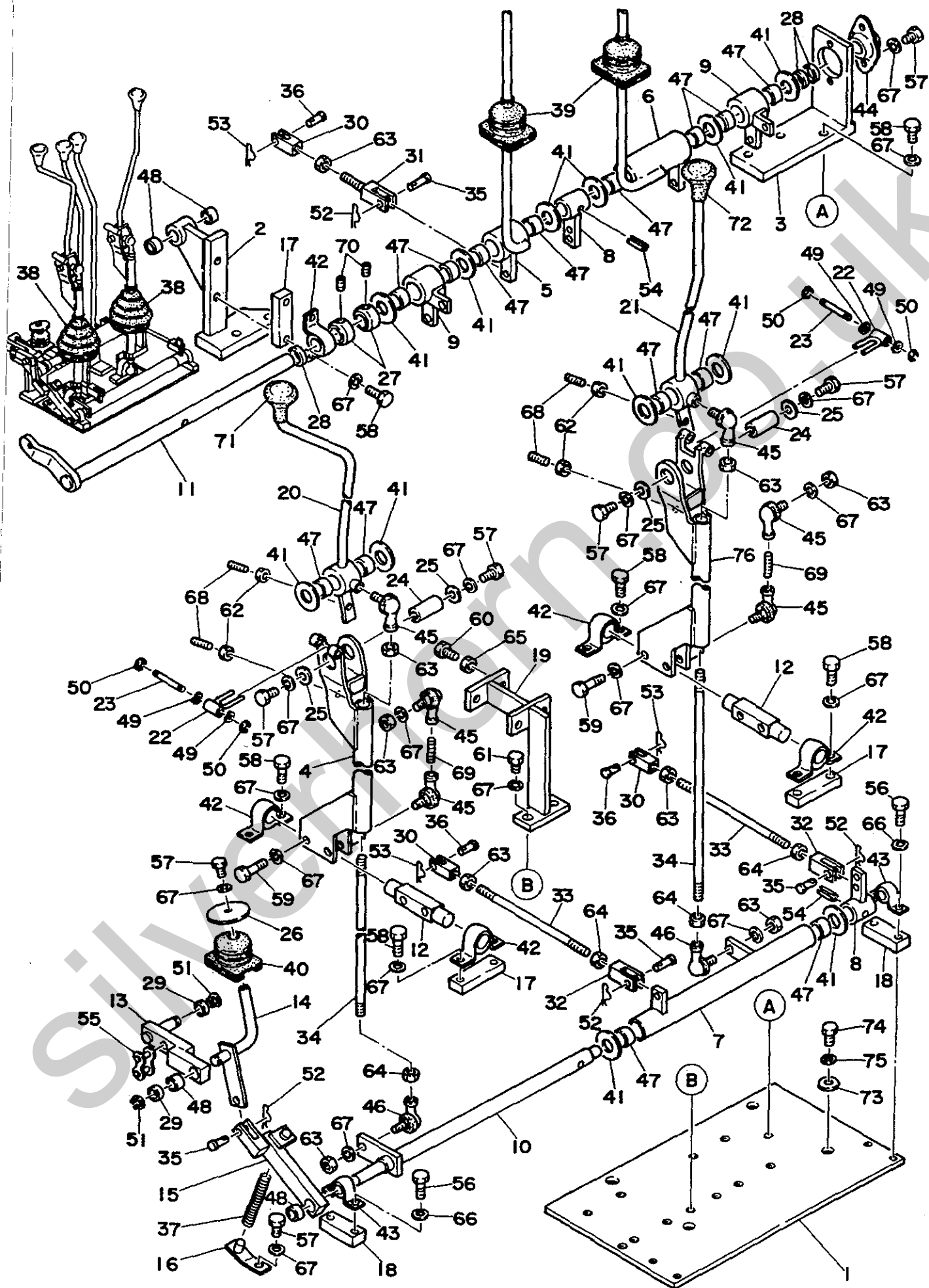
FIG. 13-1 CONTROL LEVER
