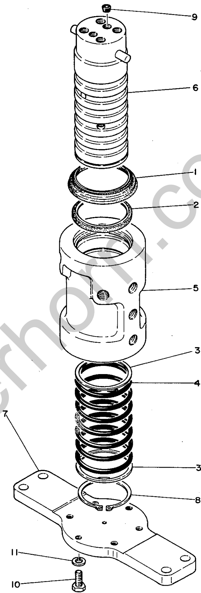
FIG. 27 SWIVEL JOINT
