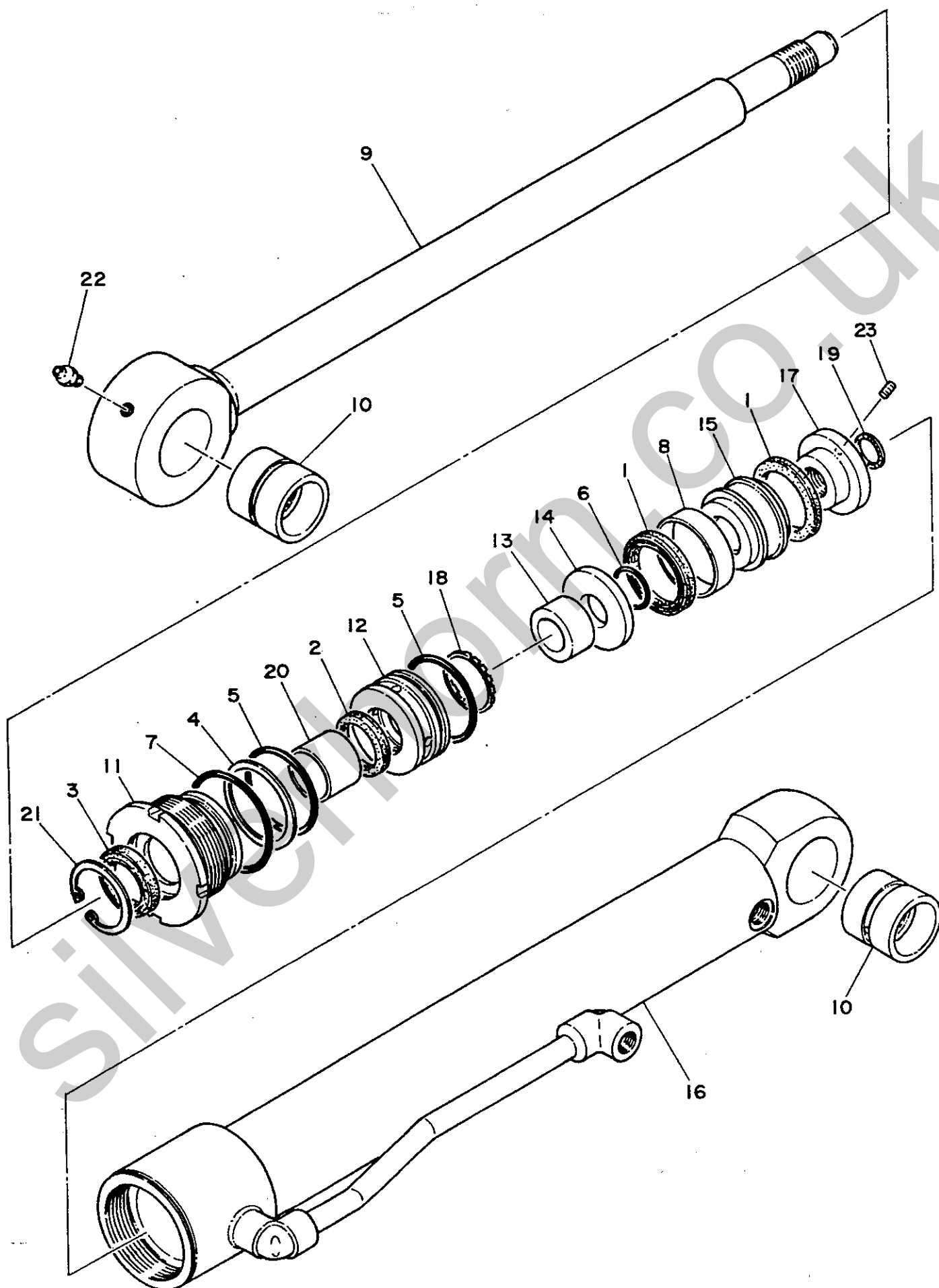
FIG. 33 SWING CYLINDER
