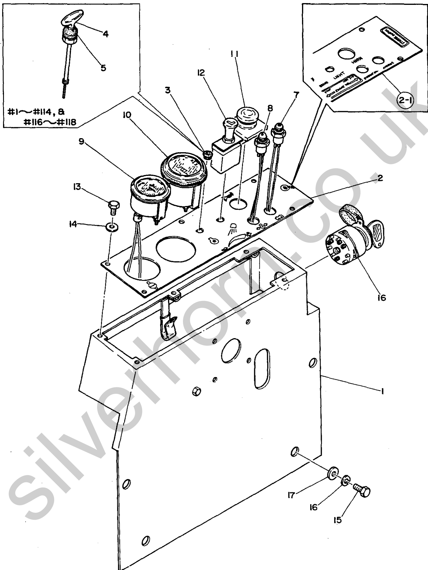
FIG. 14 CONTROL BOX
