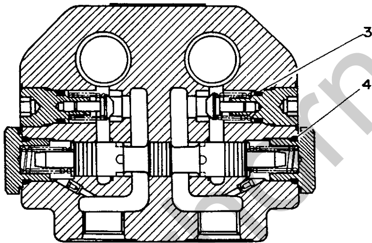
CONTERBALANCE VALVE #104 ~ #137
