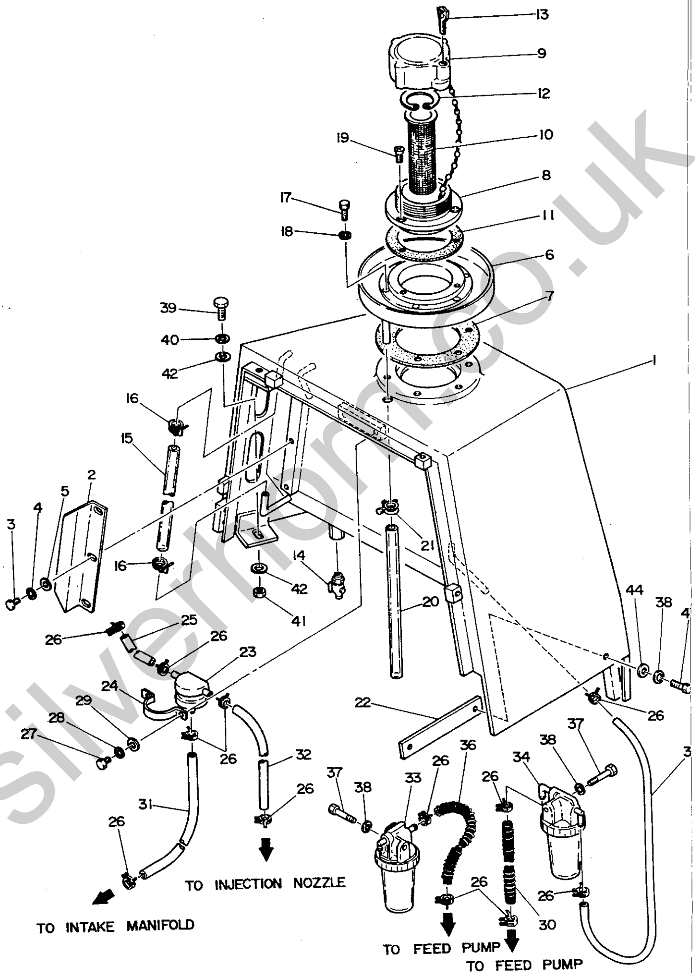
FIG. 12 FUEL TANK
