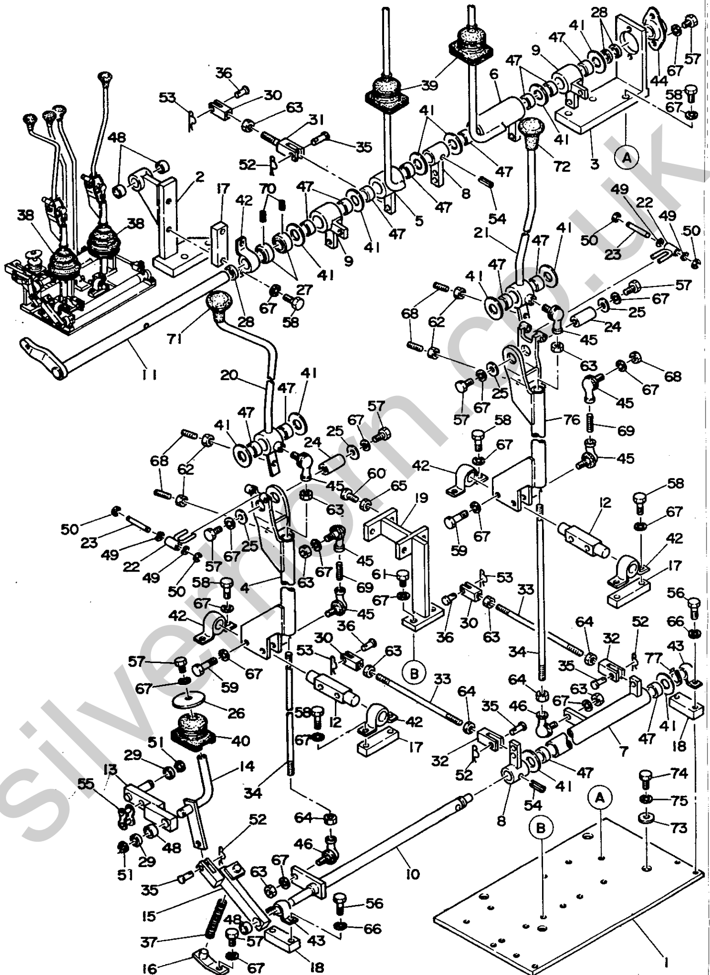
FIG. 13-2 CONTROL LEVER
