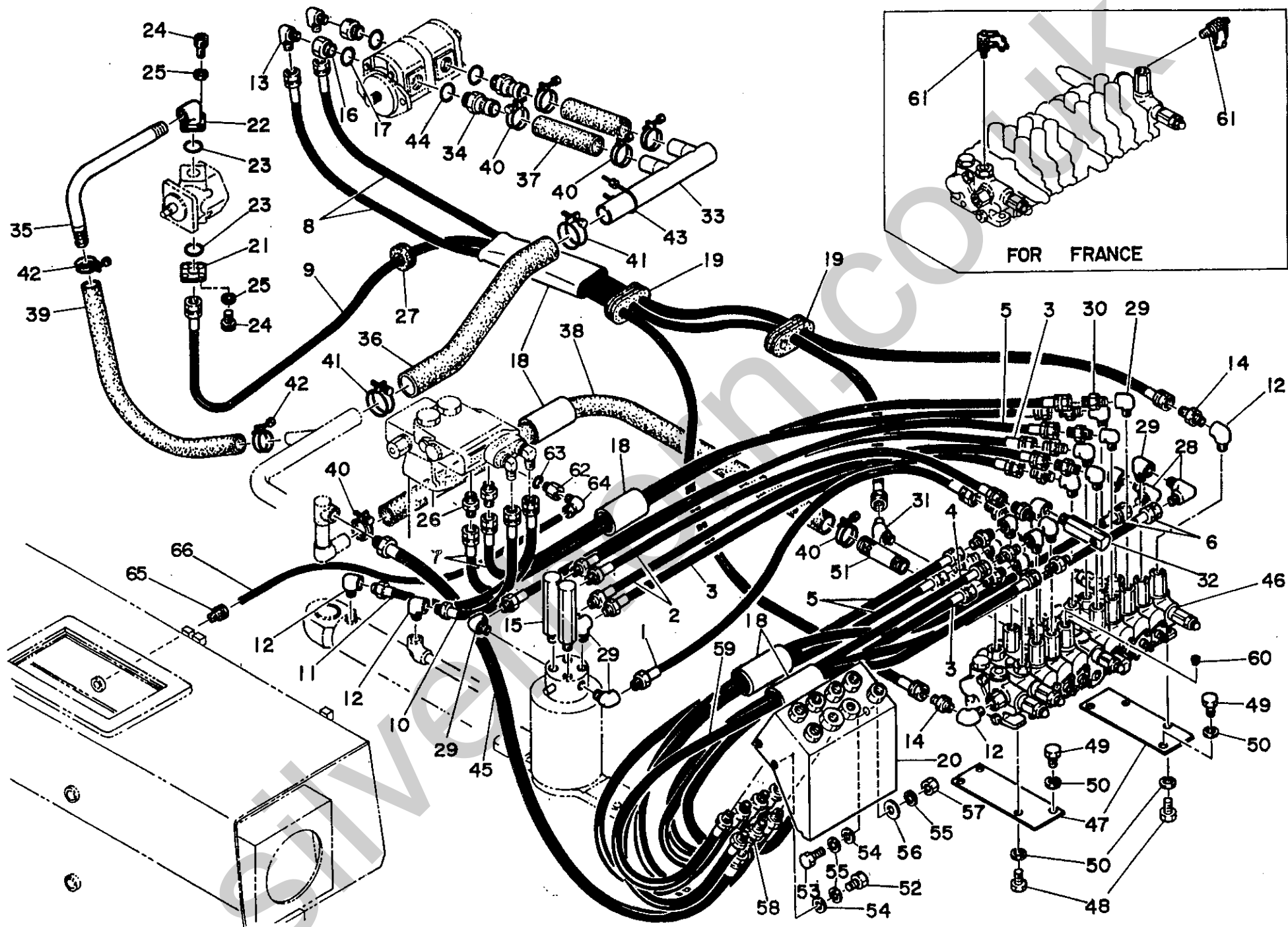
FIG. 10 PIPING, UPPER
