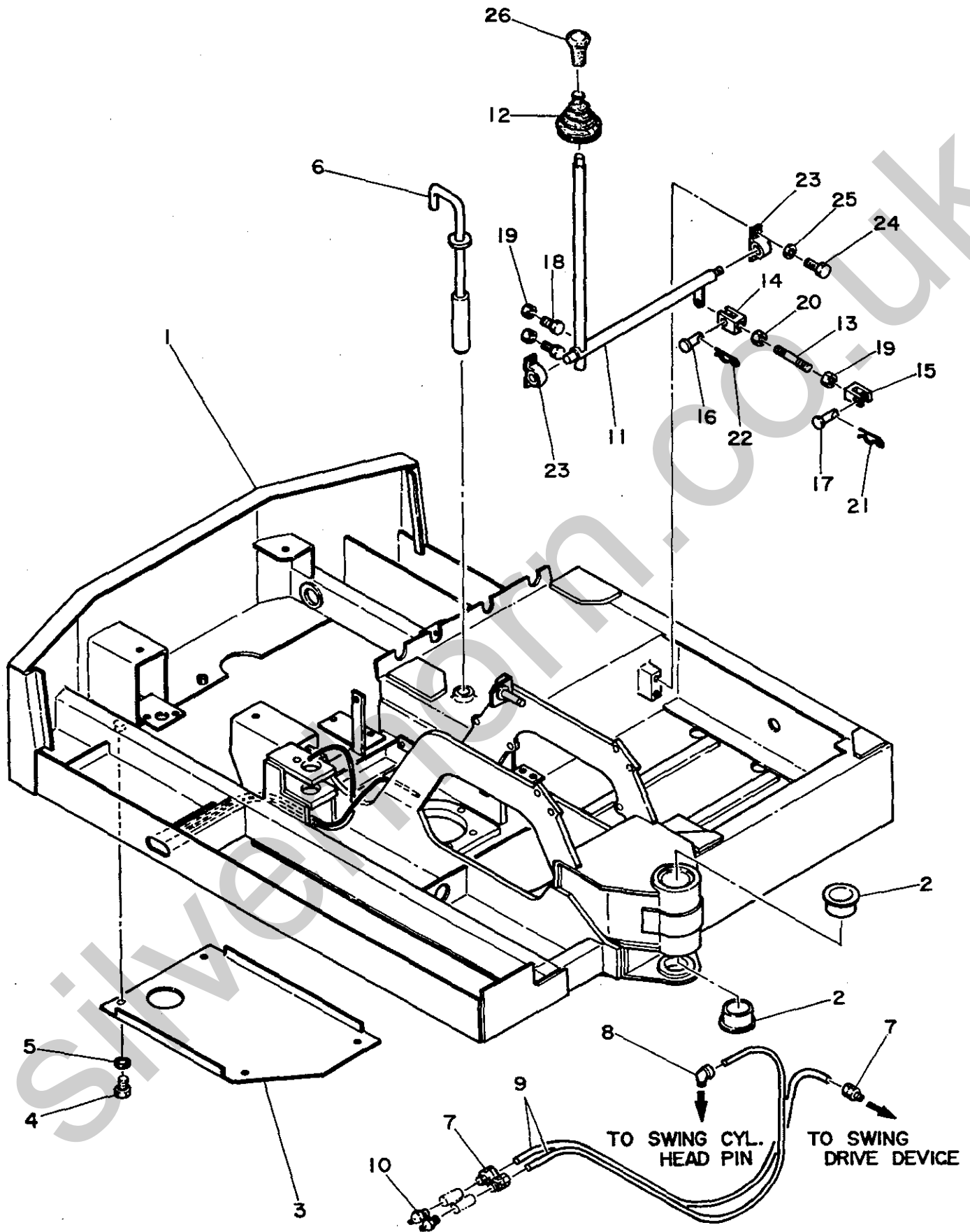
FIG. 08 TURNTABLE
