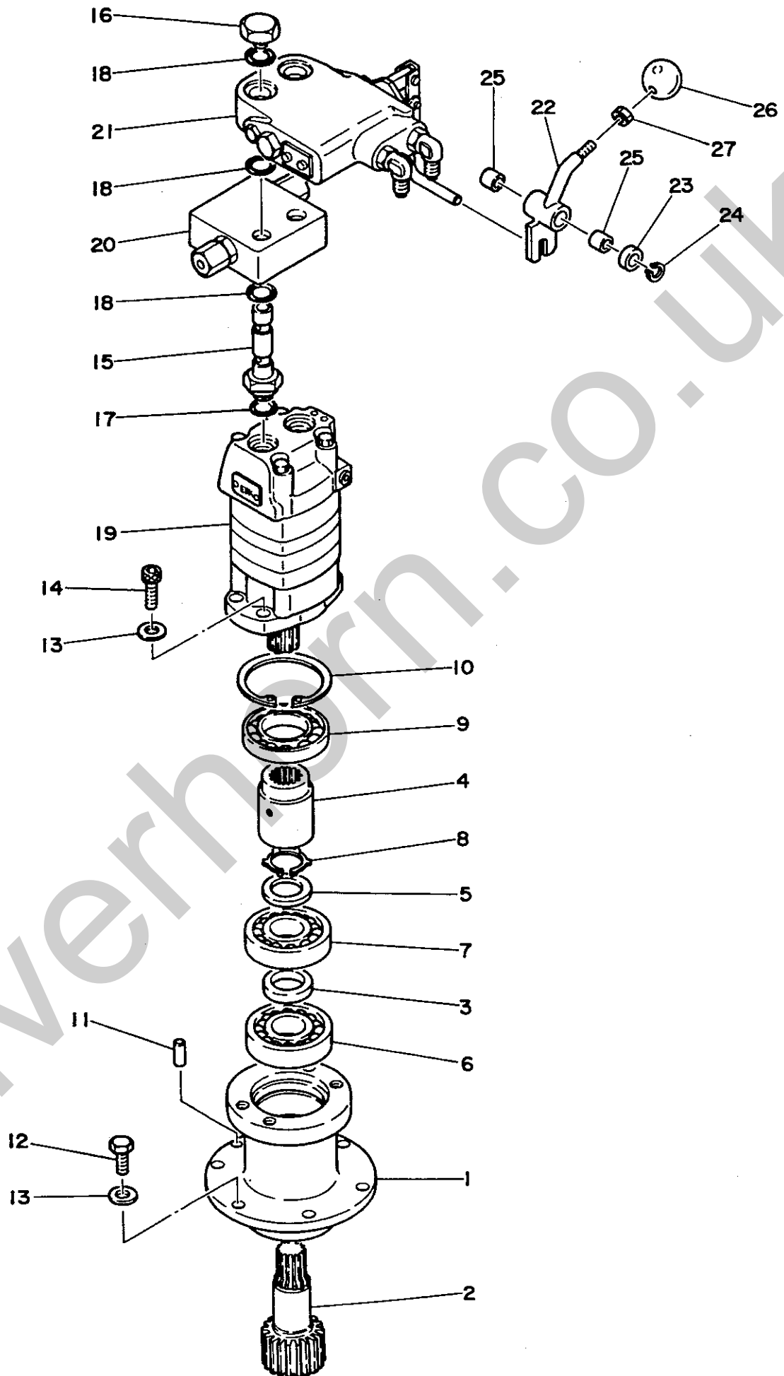
FIG. 09 SLEW GEARBOX
