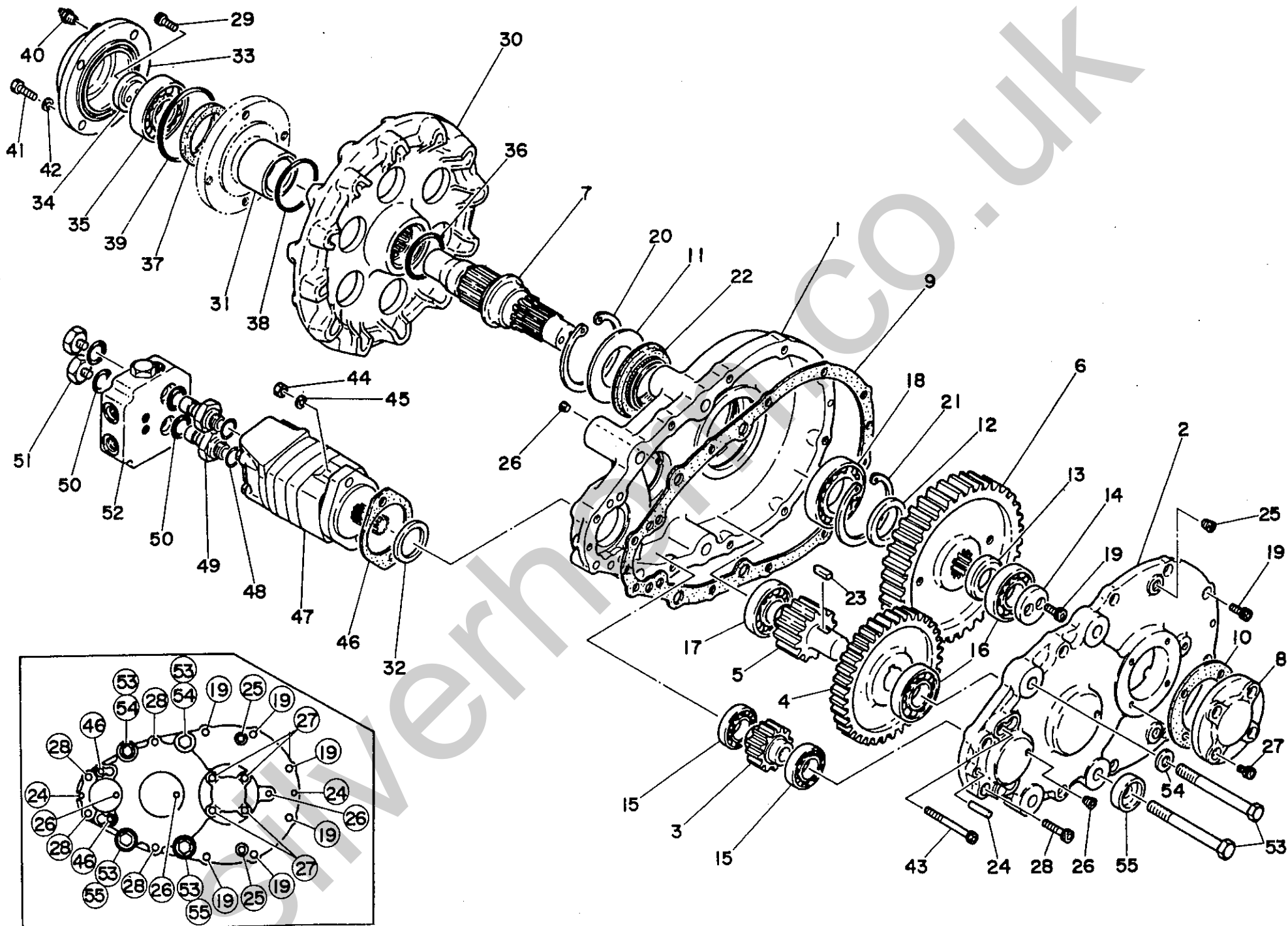
FIG. 06 TRACK GEARBOX
