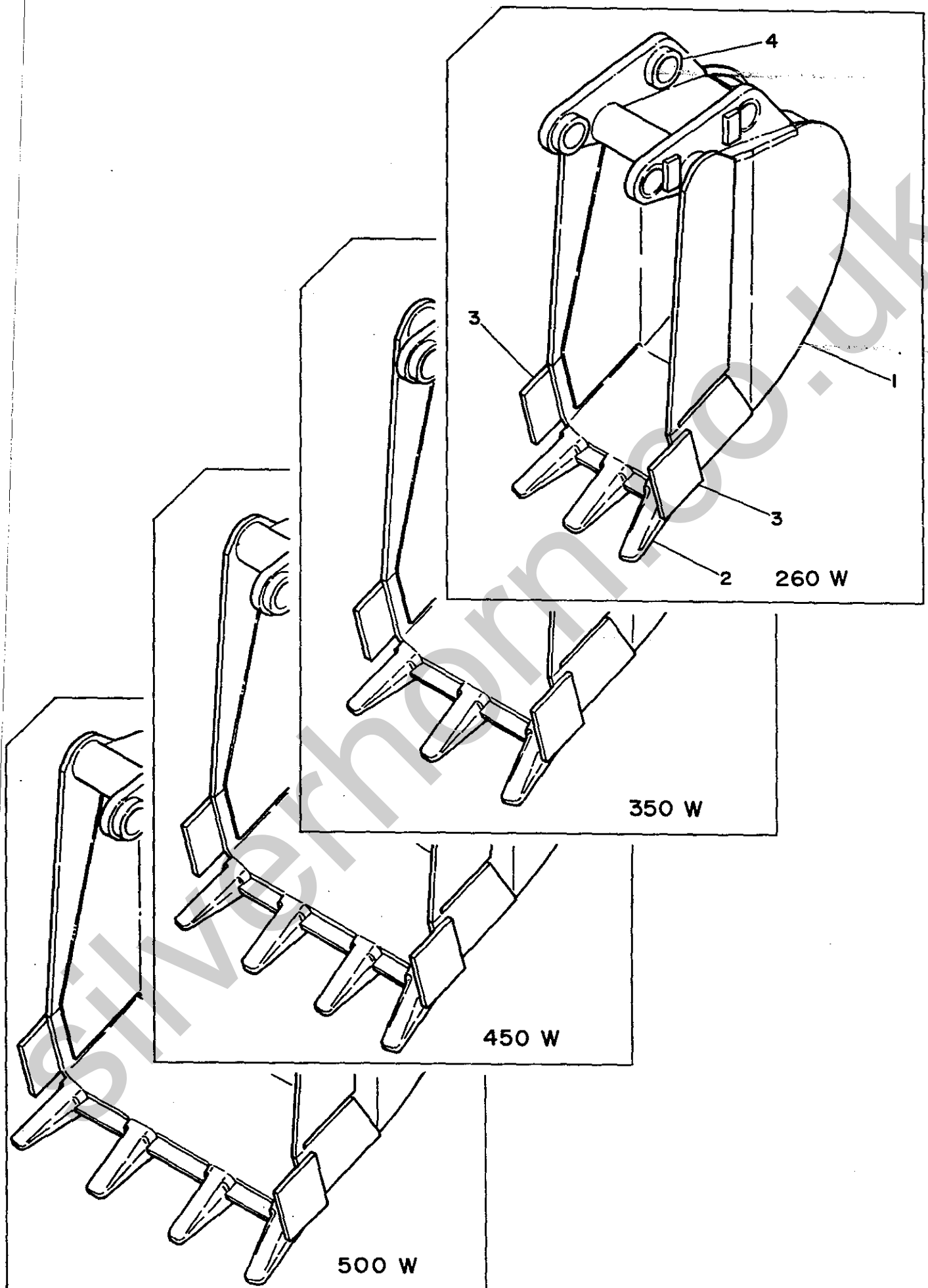
FIG. 40 BUCKET
