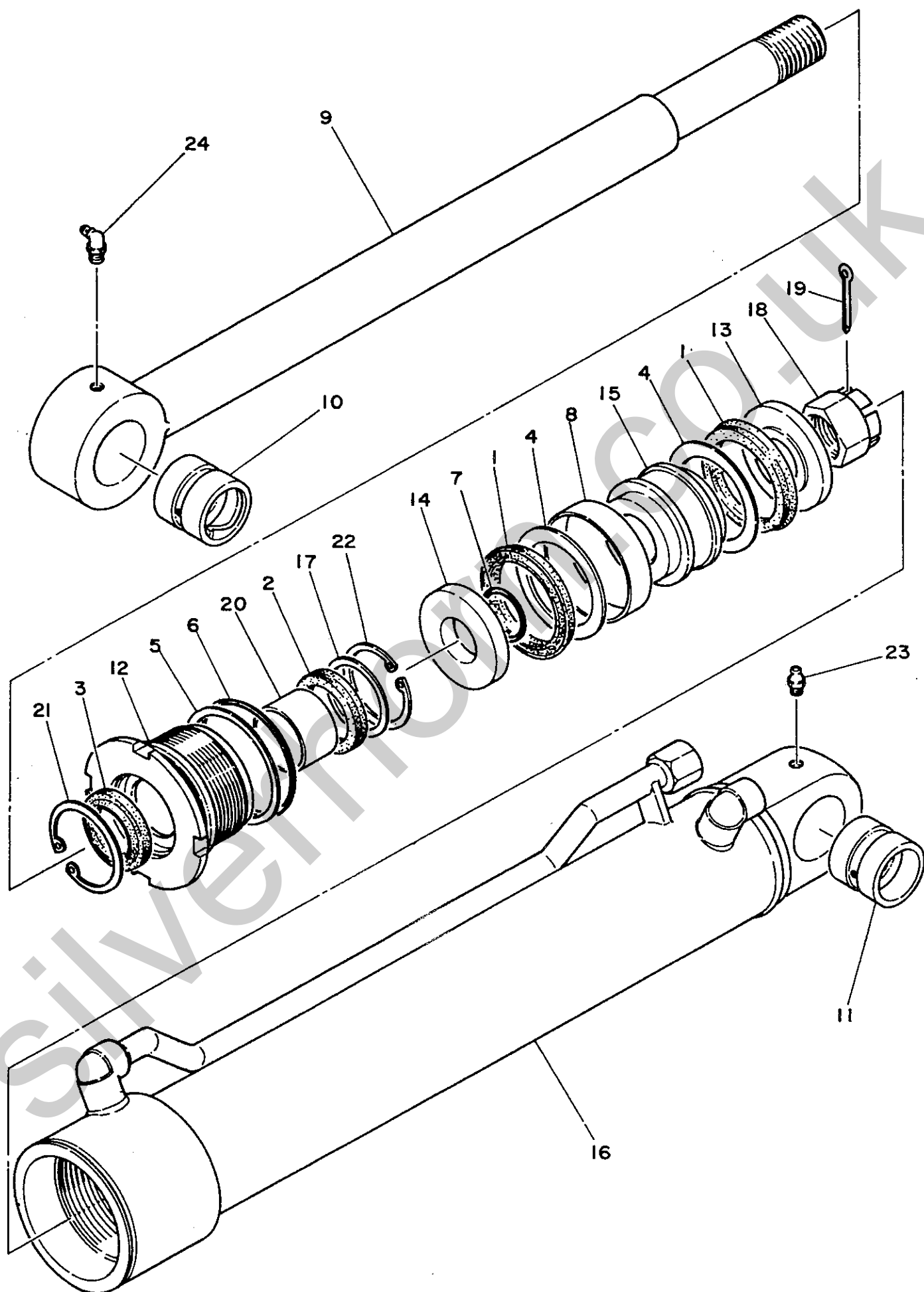
FIG. 30 ARM CYLINDER
