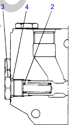
断面 "C-C" SECTION "C-C"
