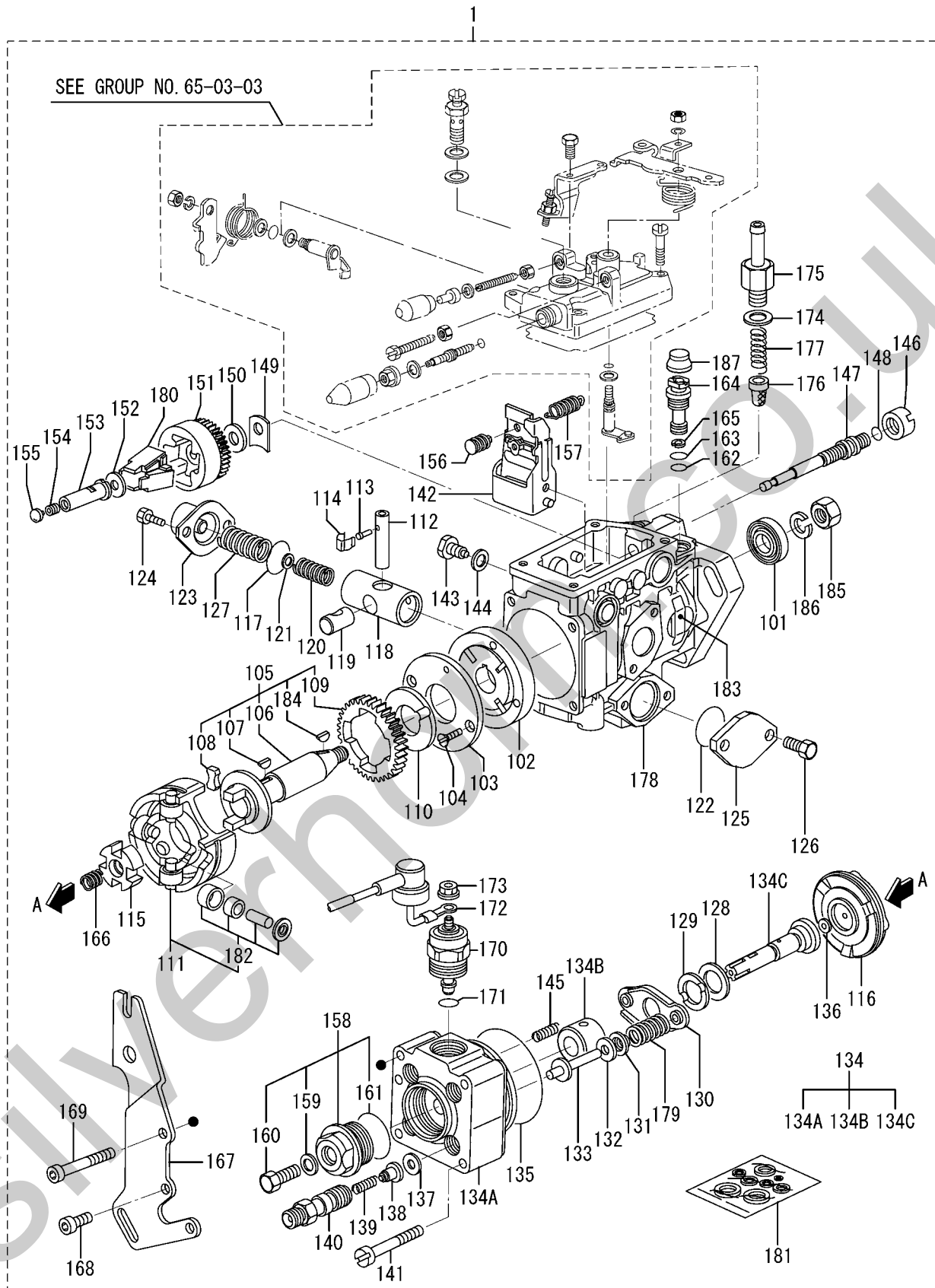
Ref. No. 134 Distributor head(Part Number 14640-14220) Consists of 3 parts that are referred to by No. 134A, 134B, and 134C.
