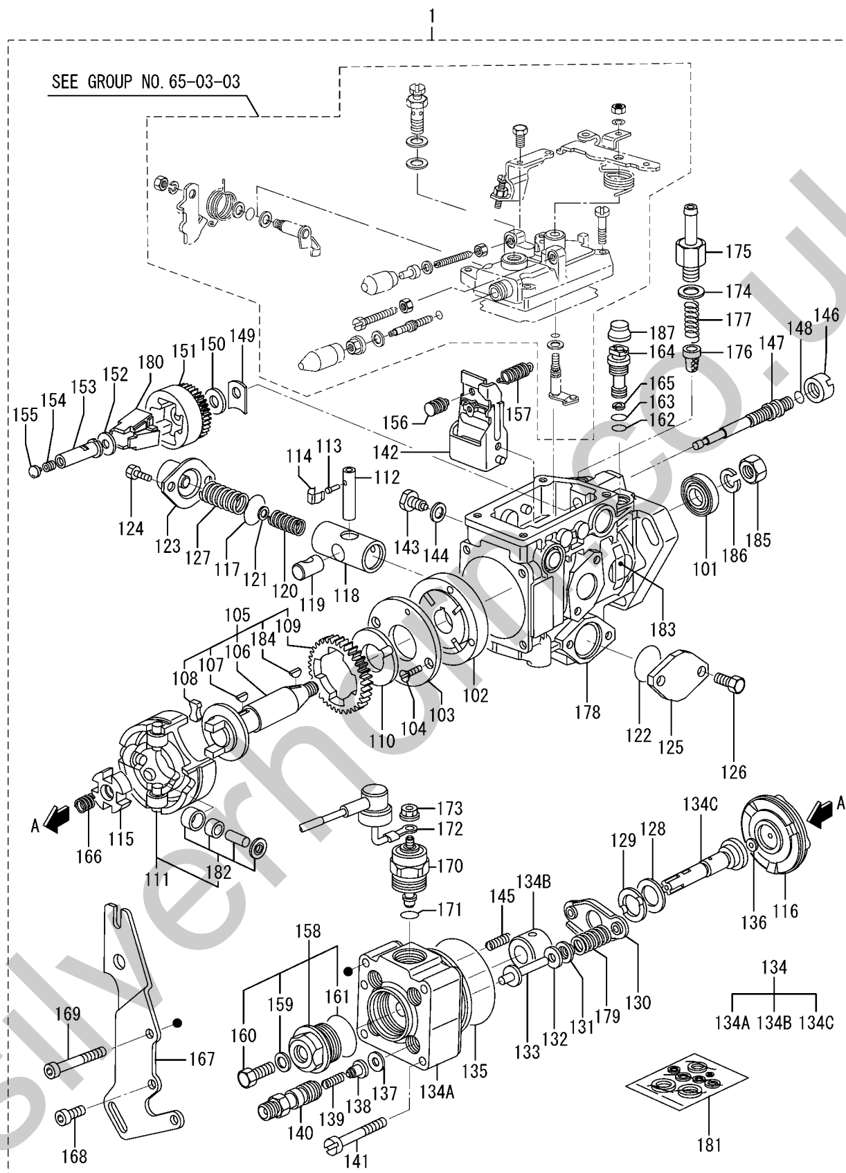
Ref. No. 134 Distributor head (Part Number 14640-14220) Consists of 3 parts that are referred to by No. 134A, 134B, and 134C.
