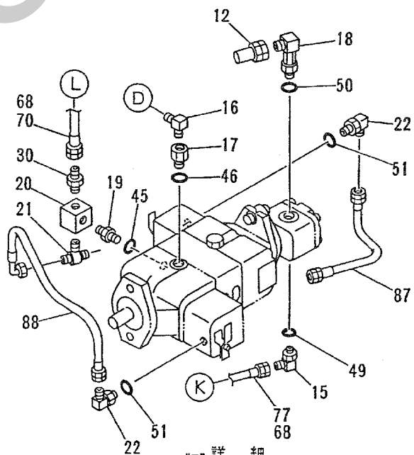
"E" 詳細 DETAIL
