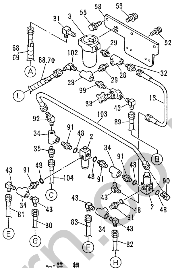
"D" 詳細 DETAIL
