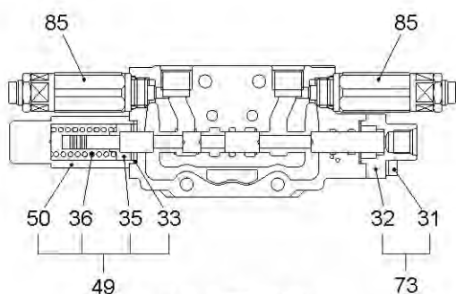
"I-I" SECTION
