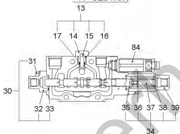
"K-K" SECTION
