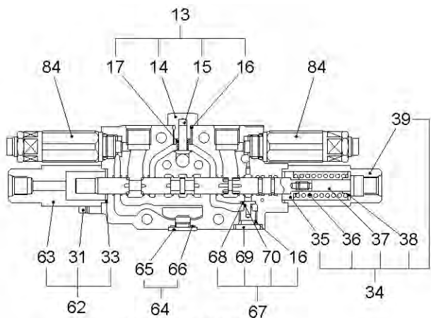
"G-G" SECTION
