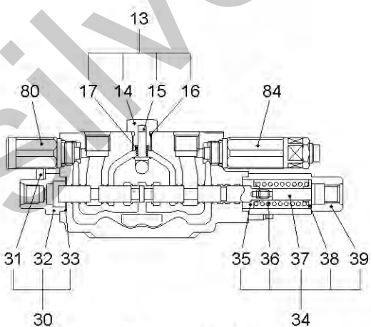
"M-M" SECTION
